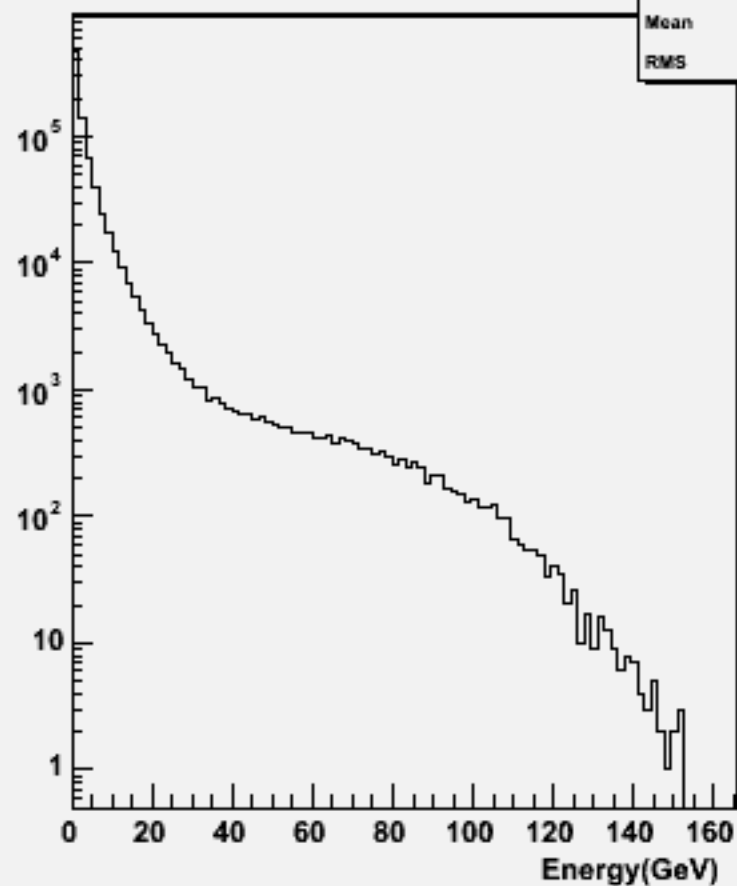
Particle Energy : w101756 ccude1n1_o
