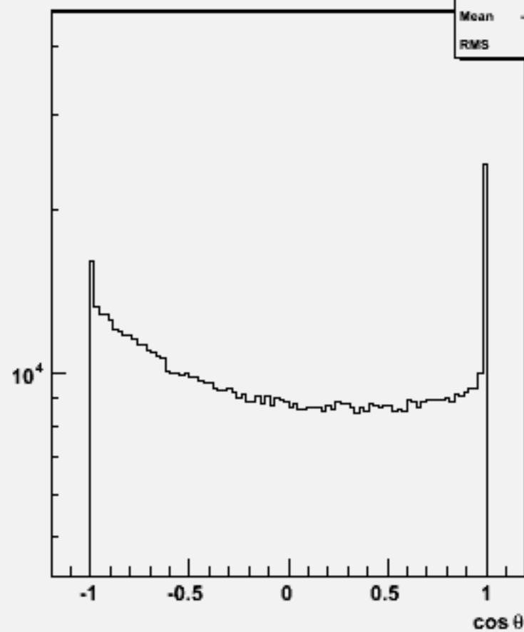
Particle cos \theta : w101756 ccude1n1_o
