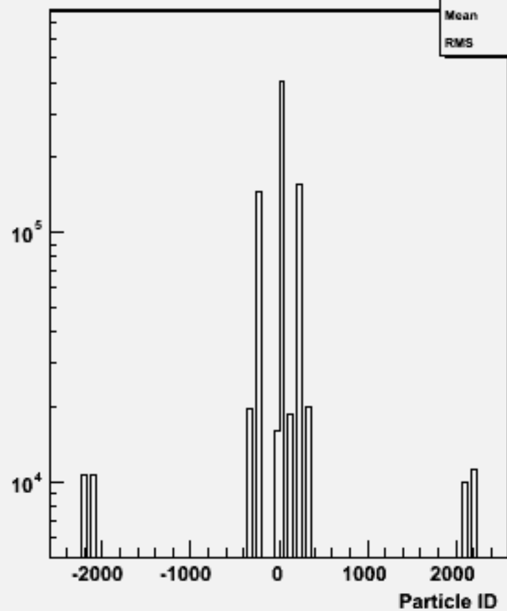
Particle ID : w101756 ccude1n1_o
