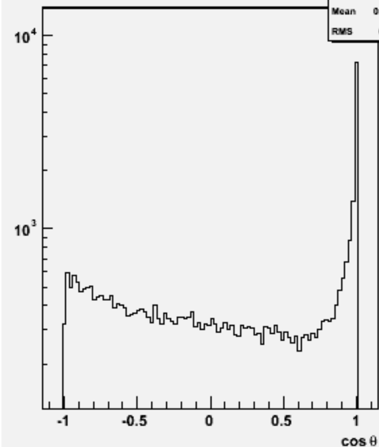
Jet cos \theta (All jets)w101756 ccude1n1_o
