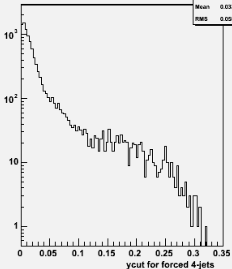
Ycut for 4-jets :w101756 ccude1n1_o
