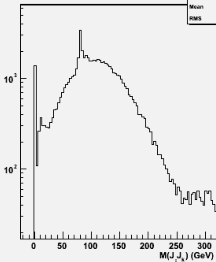
2jets mass(All comb)w101756 ccude1n1_o
