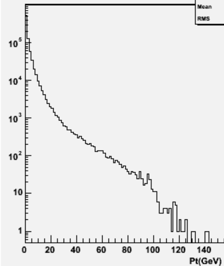
Particle Pt : w101756 ccude1n1_o
