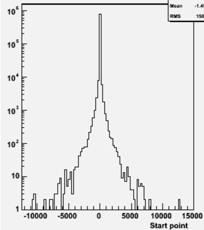
Start point Z : w101756 ccude1n1_o
