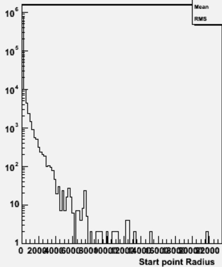
Start point R : w101756 ccude1n1_o
