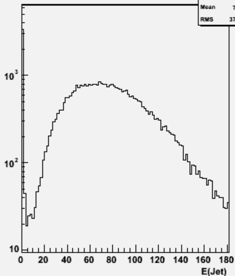
Jet energies(All jets)w101756 ccude1n1_o
