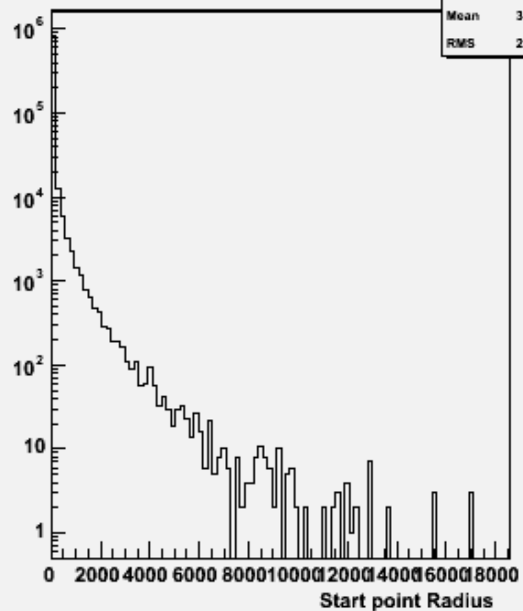
Start point R : w101753 ccn3e3sc_o
