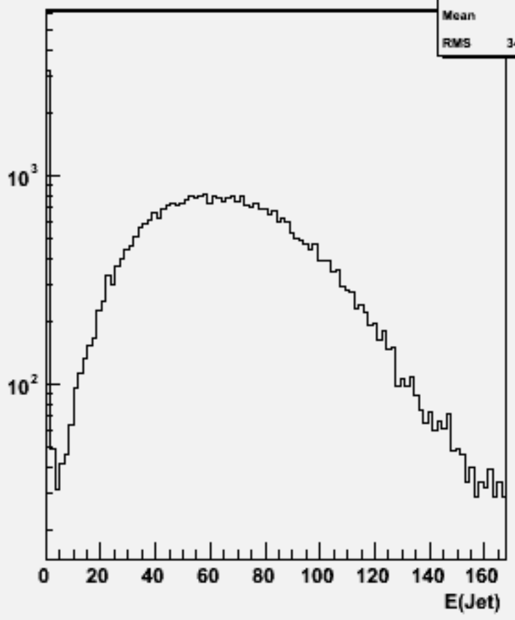
Jet energies(All jets)w101753 ccn3e3sc_o
