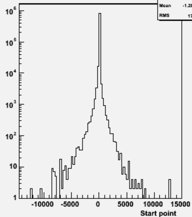
Start point Z : w101753 ccn3e3sc_o
