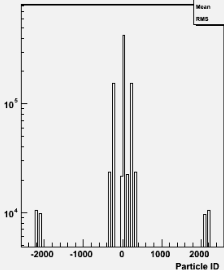
Particle ID : w101753 ccn3e3sc_o
