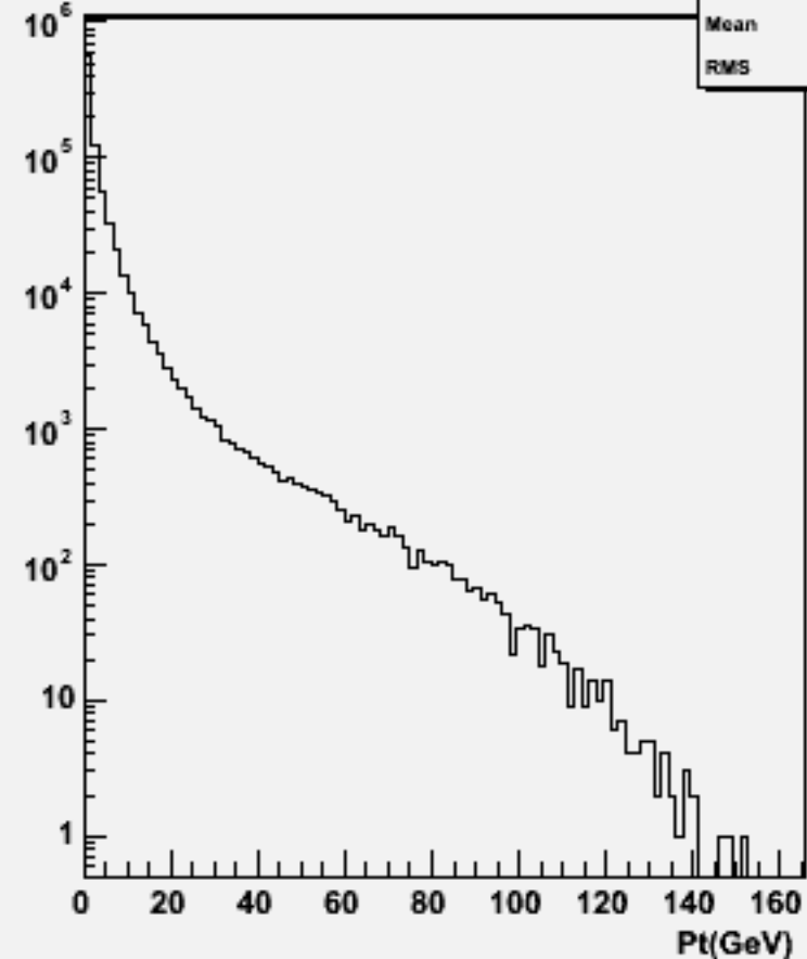
Particle Pt : w101753 ccn3e3sc_o
