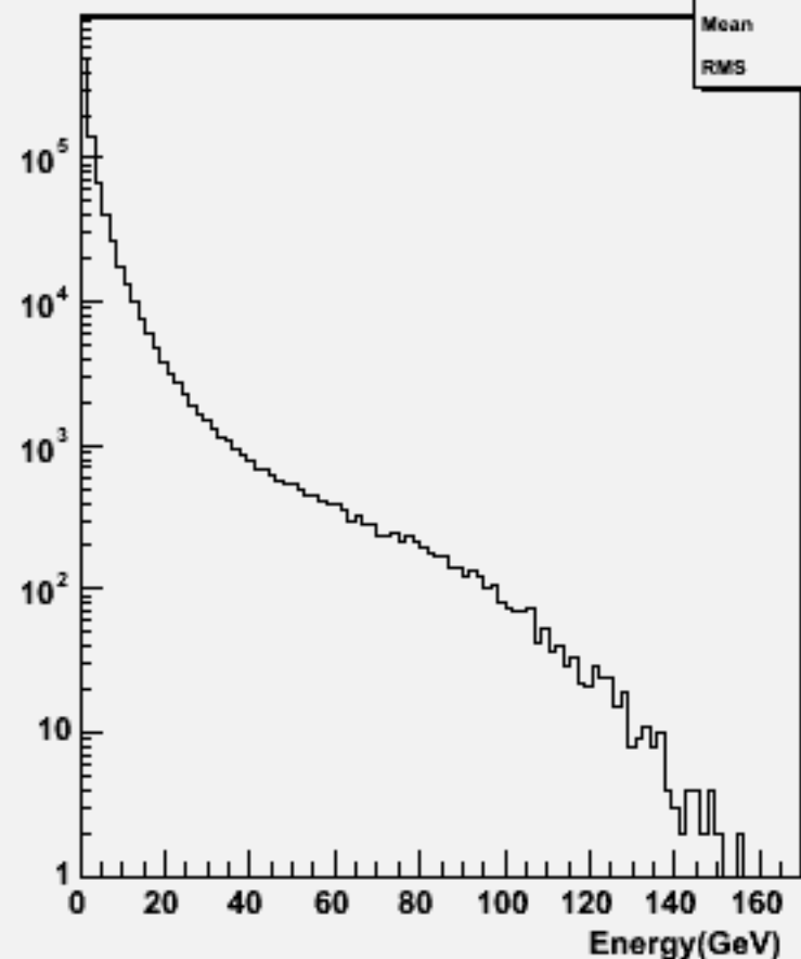
Particle Energy : w101753 ccn3e3sc_o
