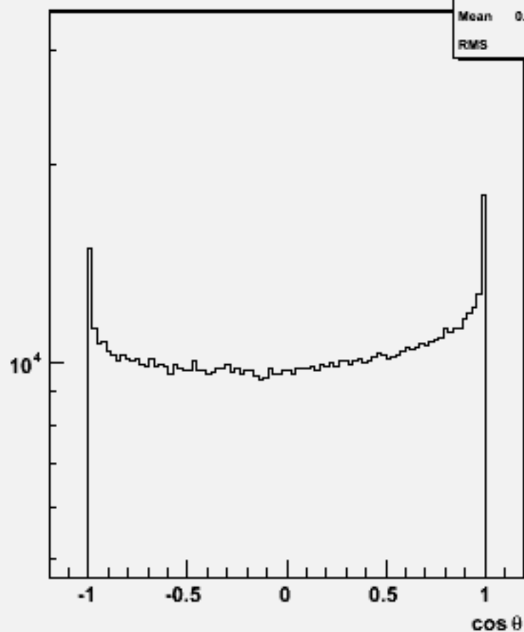
Particle cosθ : w101753 ccn3e3sc_o
