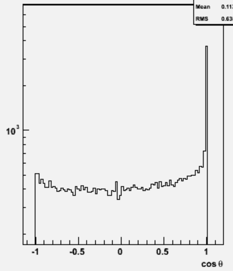
Jet cosθ (All jets)w101753 ccn3e3sc_o
