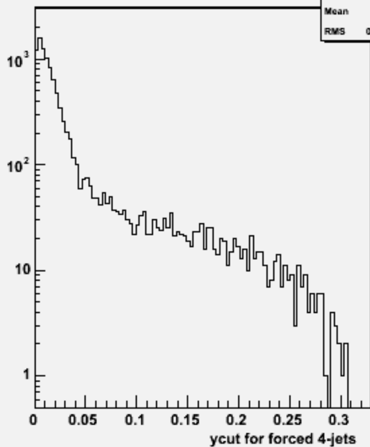
Ycut for 4-jets :w101752 ccn3e3sc_o
