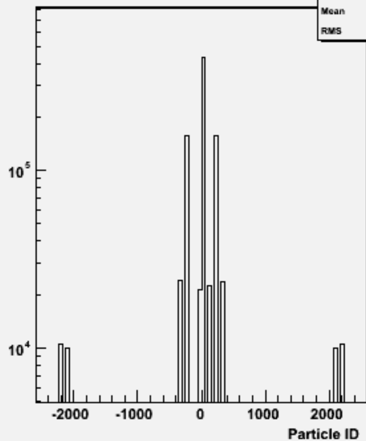
Particle ID : w101752 ccn3e3sc_o
