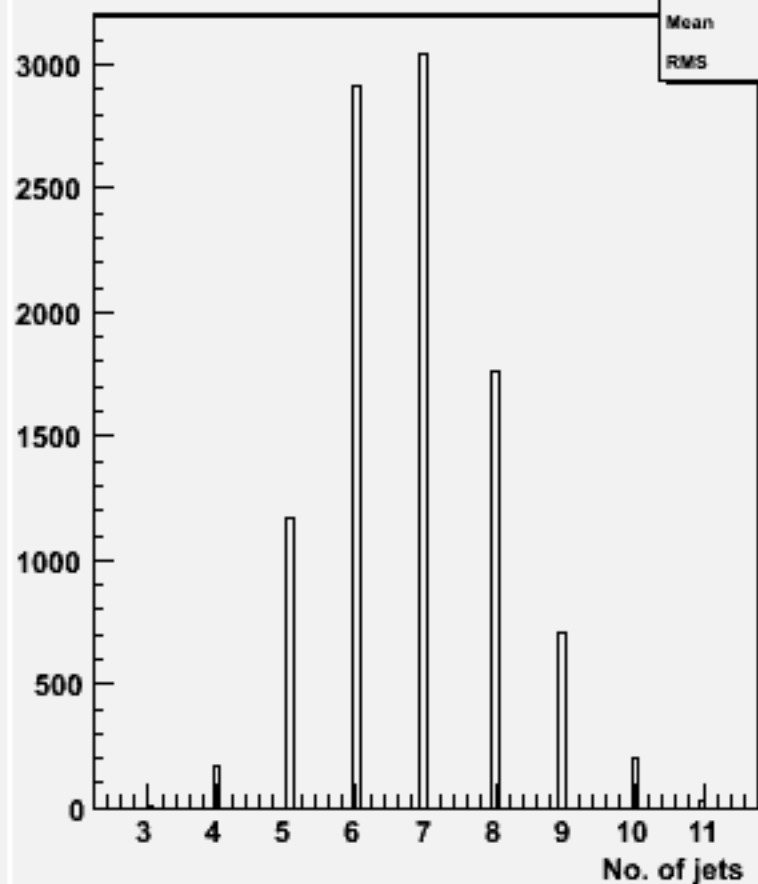
No. jets (ycut=0.001) : w101752 ccn3e3sc_o
