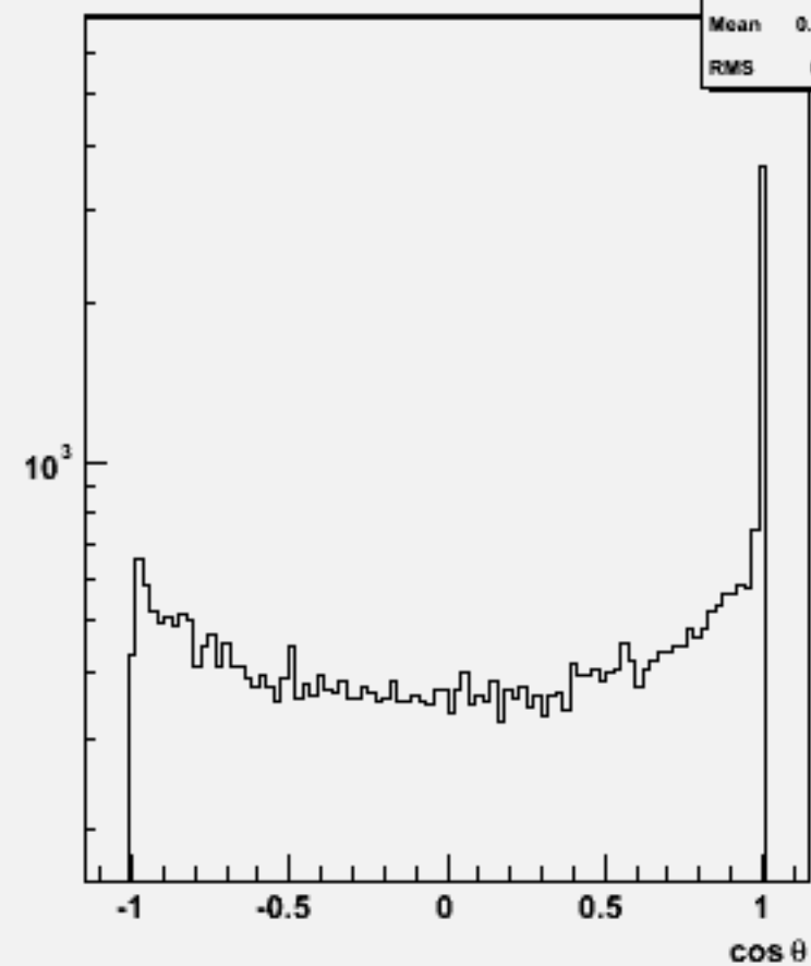
Jet cosθ (All jets)w101752 ccn3e3sc_o
