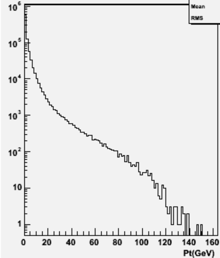
Particle Pt : w101752 ccn3e3sc_o
