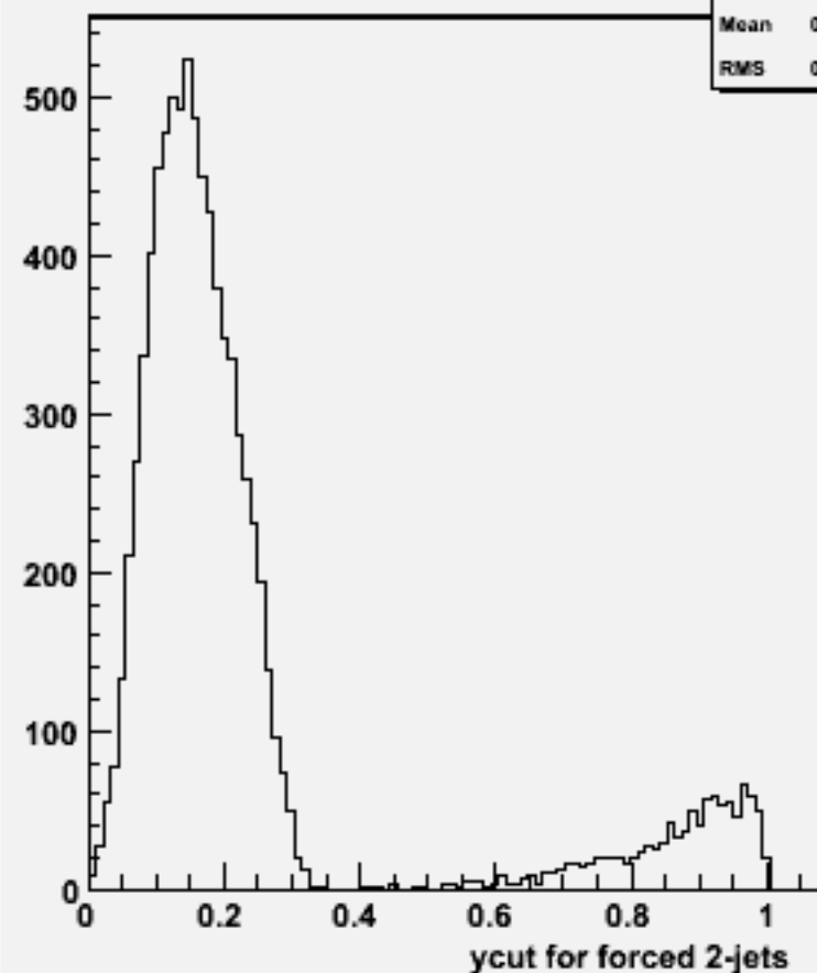
Ycut for 2-jets :w101752 ccn3e3sc_o
