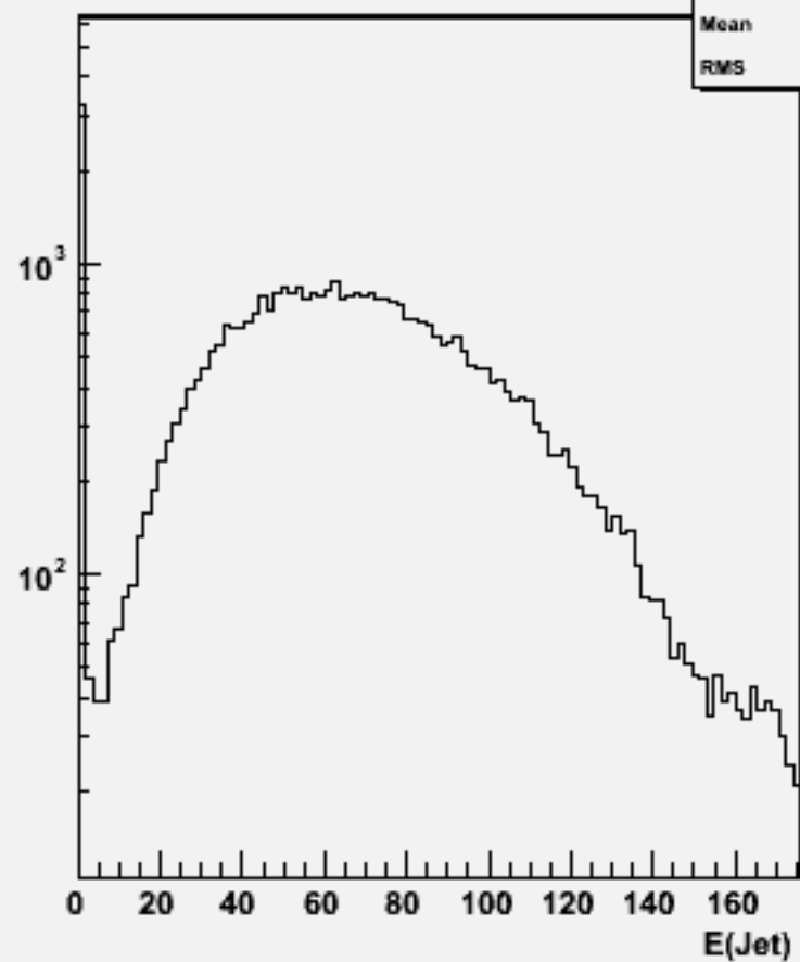
Jet energies(All jets)w101752 ccn3e3sc_o
