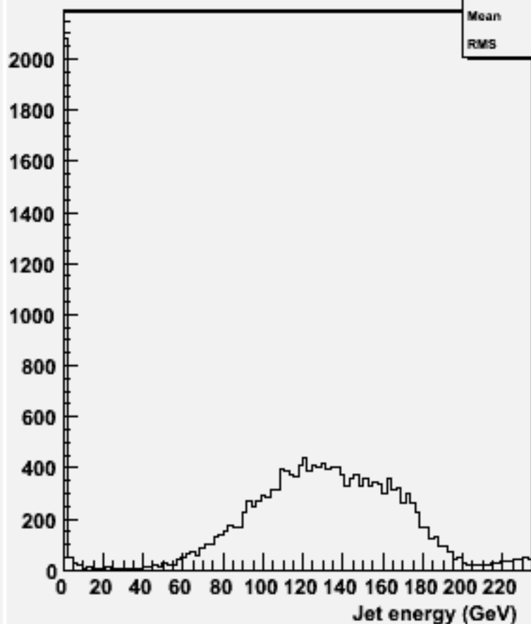
energy for 2-jets :w101752 ccn3e3sc_o
