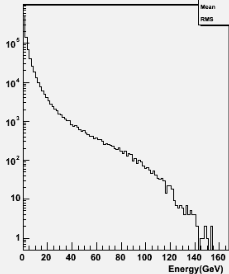
Particle Energy : w101752 ccn3e3sc_o
