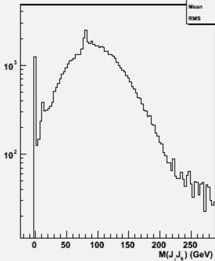
2jets mass(All comb)w101752 ccn3e3sc_o
