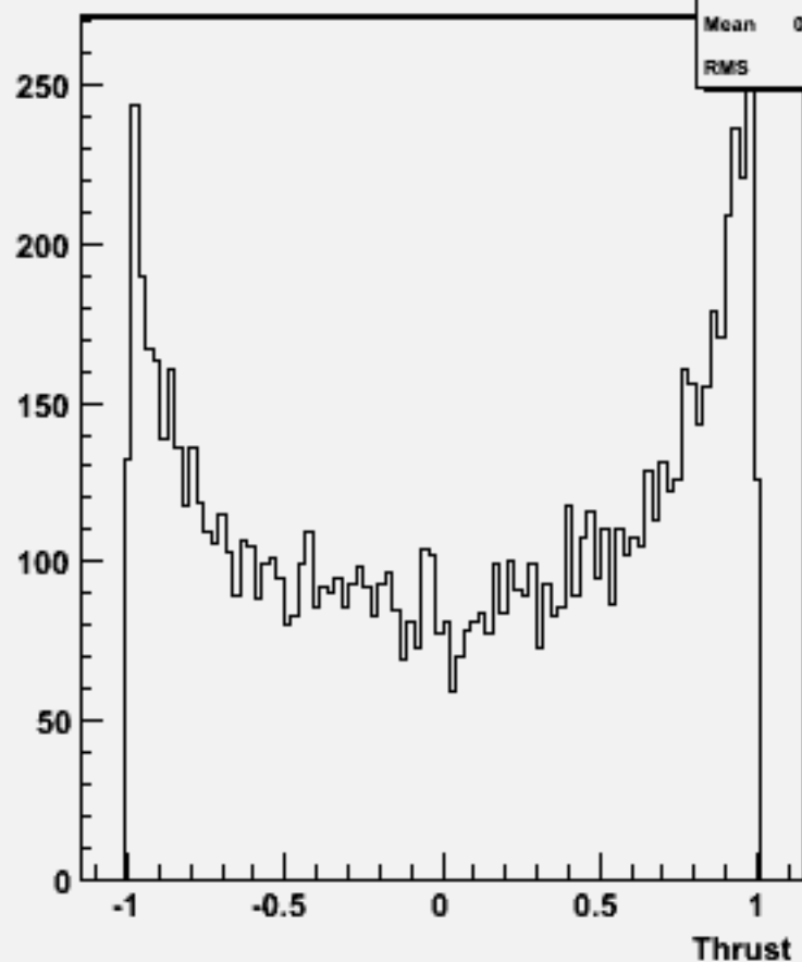
cos \Theta (thrust) w101752 ccn3e3sc_o
