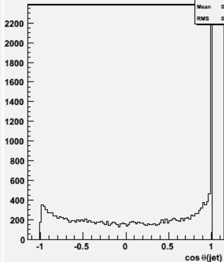
cos \theta for 2-jets :w101752 ccn3e3sc_o
