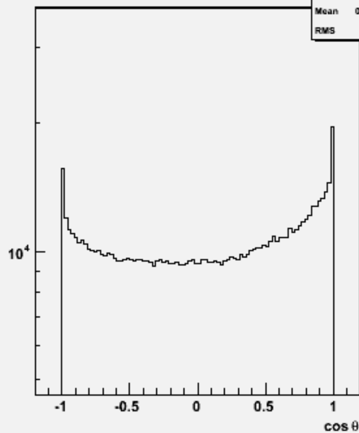
Particle cos \theta : w101752 ccn3e3sc_o
