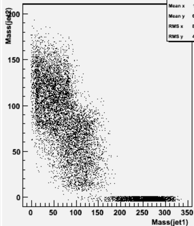
Jet mass for forced 2-jets : w101752 ccn3e3sc_o
