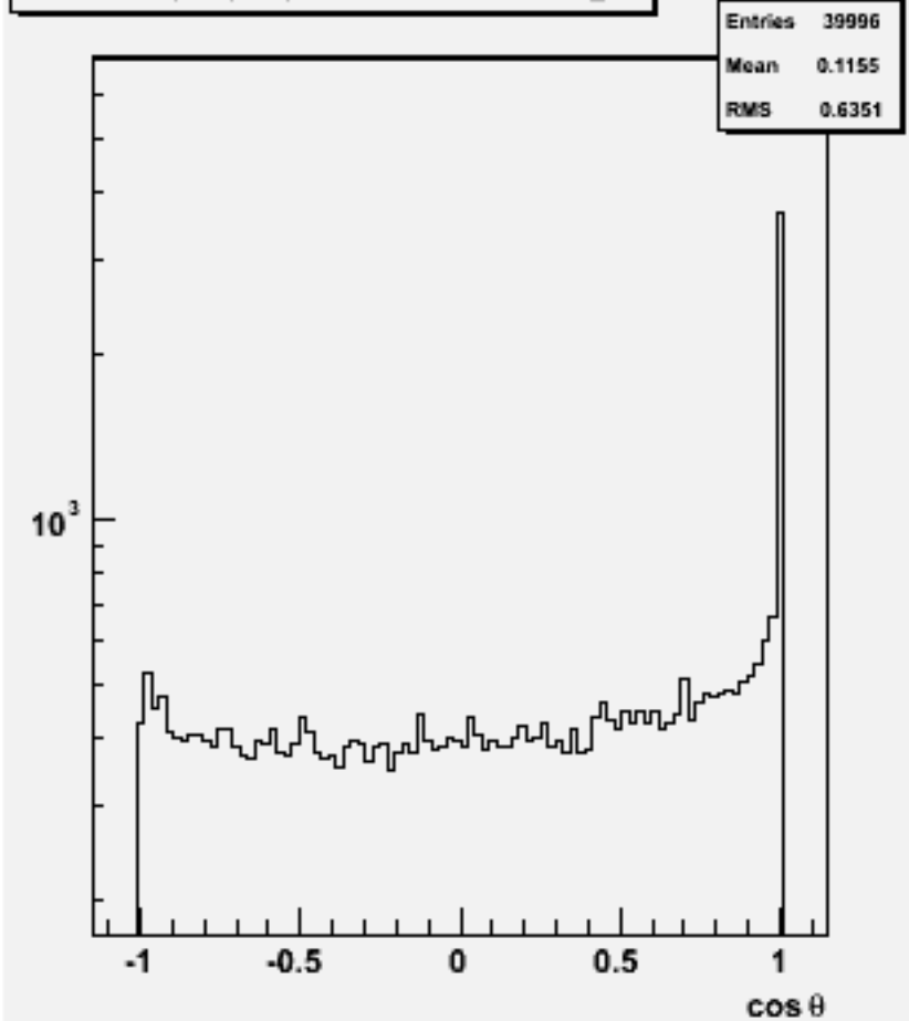
Jet cosθ (All jets)w101749 ccn3e3du_o
