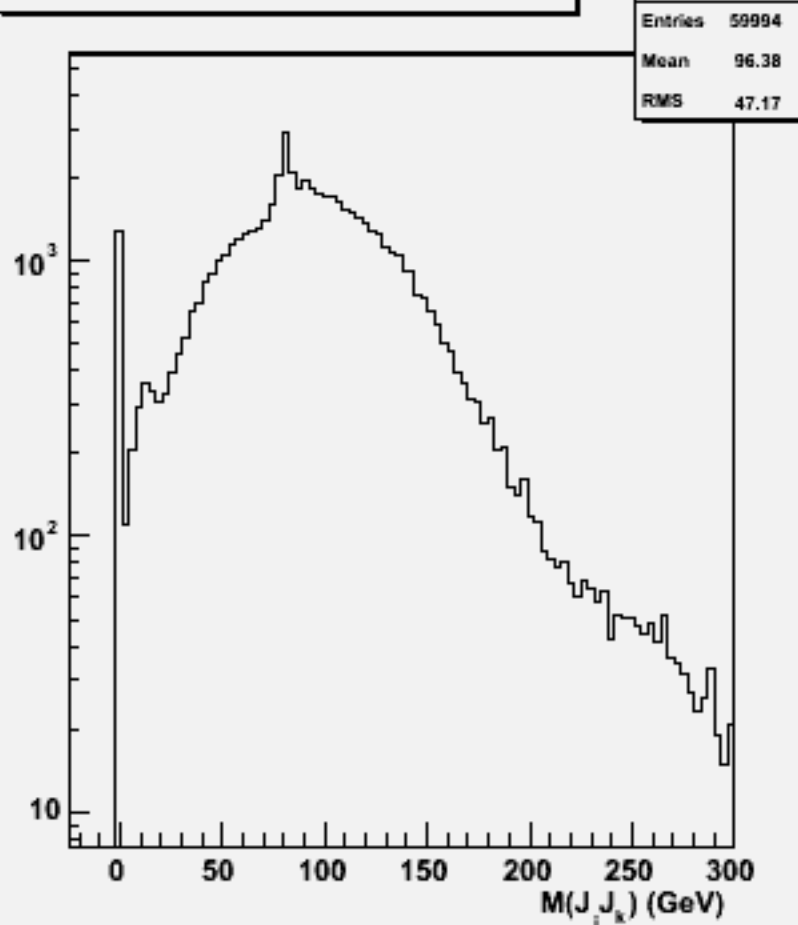
2jets mass(All comb)w101749 ccn3e3du_o
