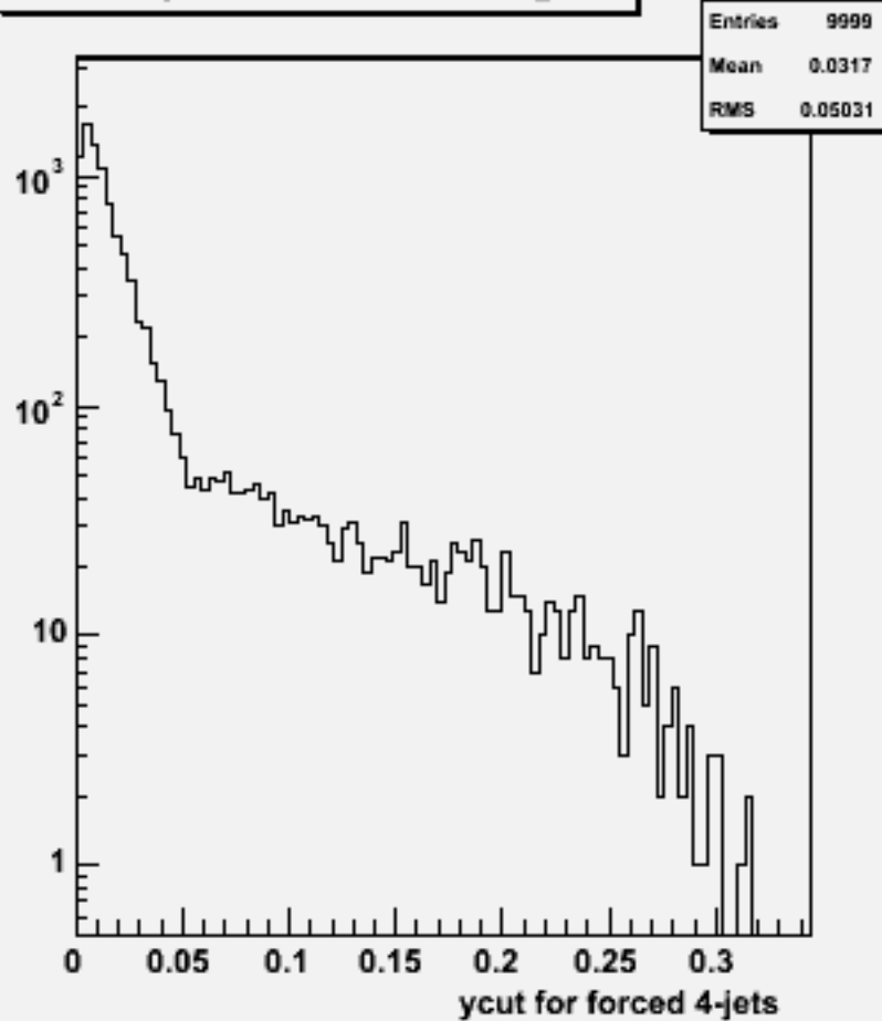
Ycut for 4-jets :w101749 ccn3e3du_o
