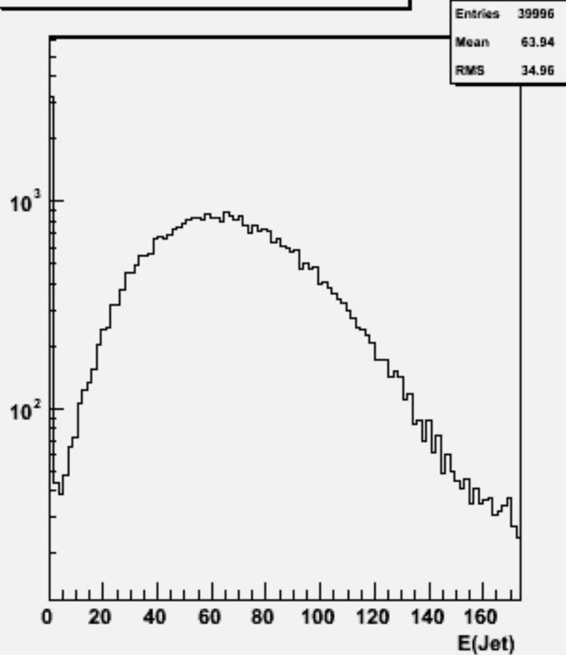
Jet energies(All jets)w101749 ccn3e3du_o
