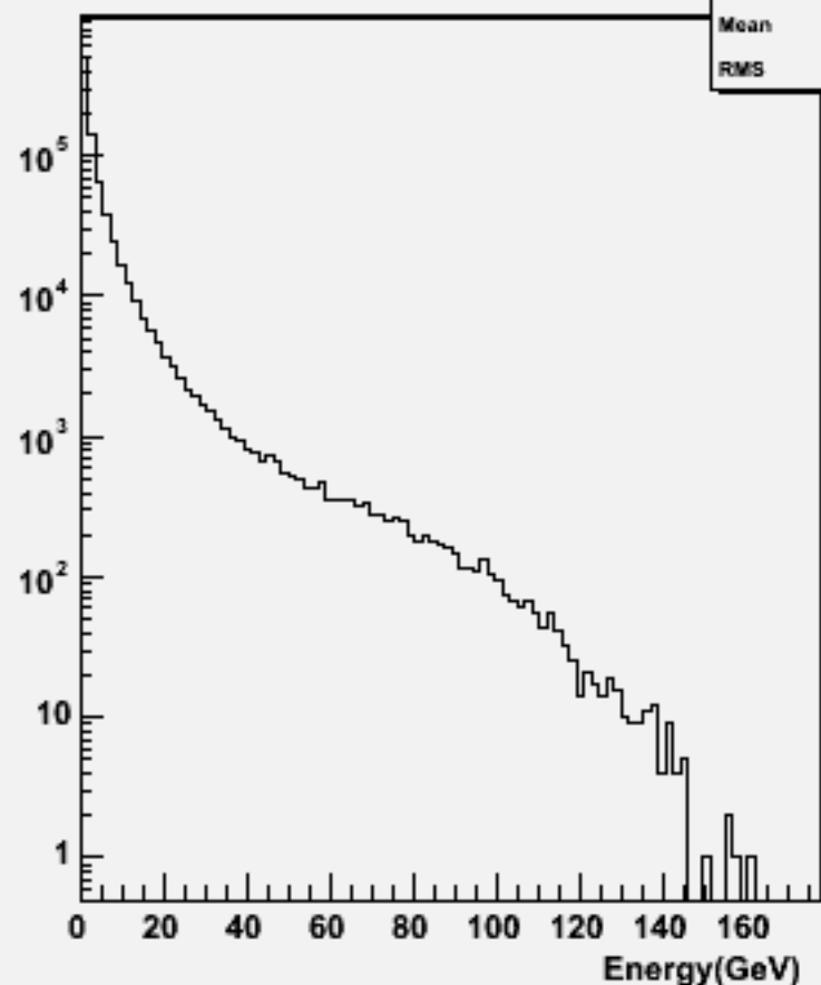
Particle Energy : w101749 ccn3e3du_o
