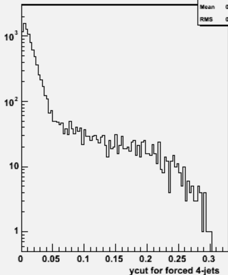
Ycut for 4-jets :w101748 ccn3e3du_o
