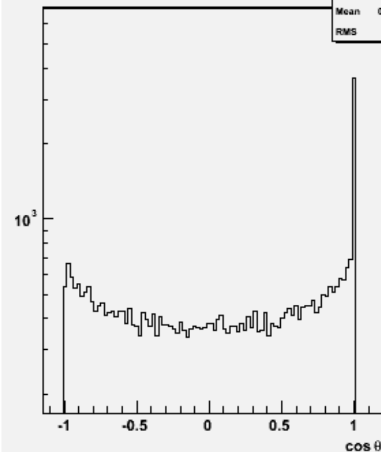
Jet cos \theta (All jets)w101748 ccn3e3du_o
