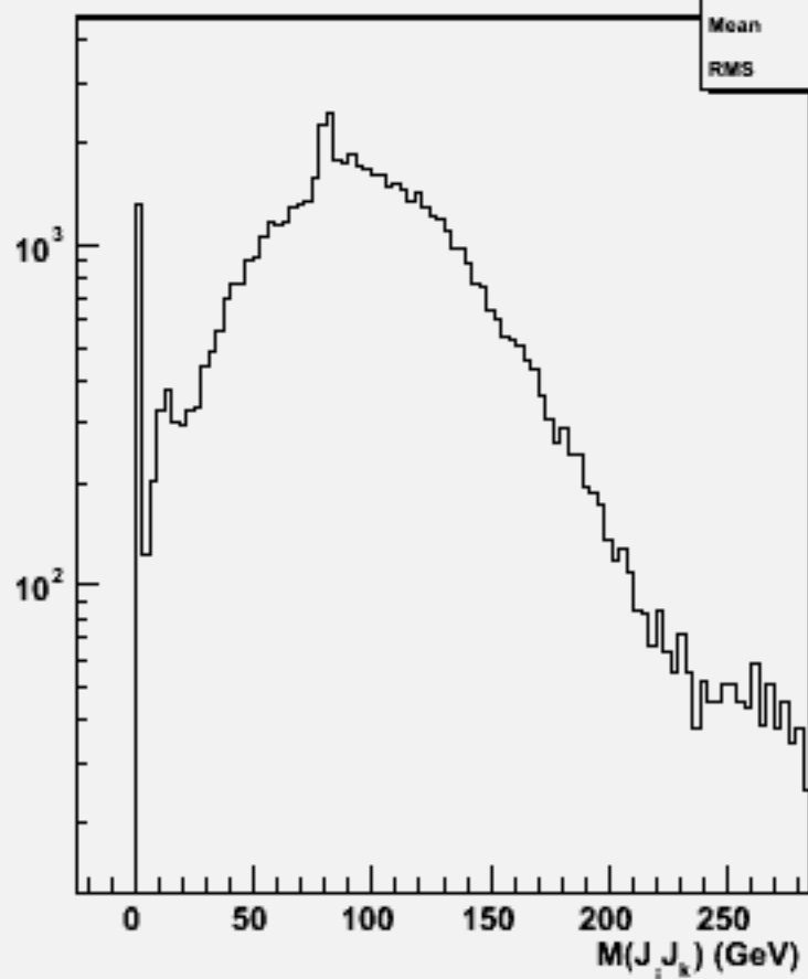
2jets mass(All comb)w101748 ccn3e3du_o
