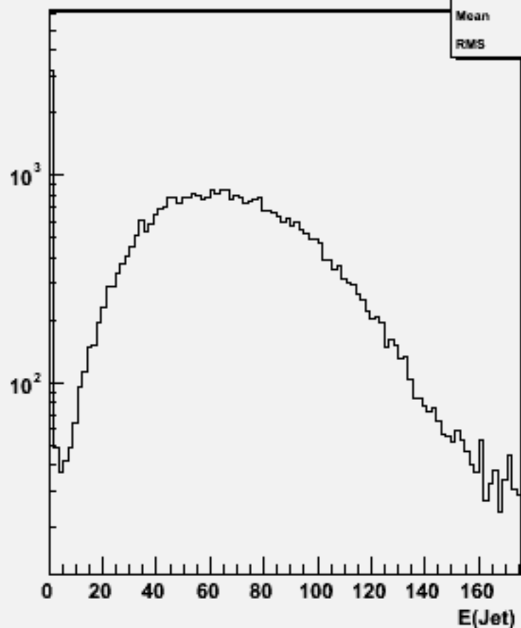
Jet energies(All jets)w101748 ccn3e3du_o
