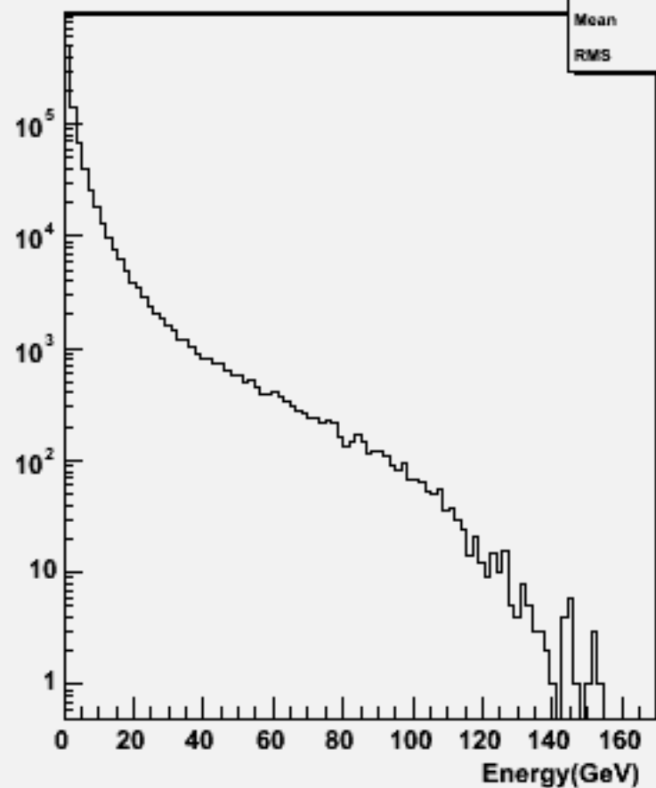
Particle Energy : w101748 ccn3e3du_o
