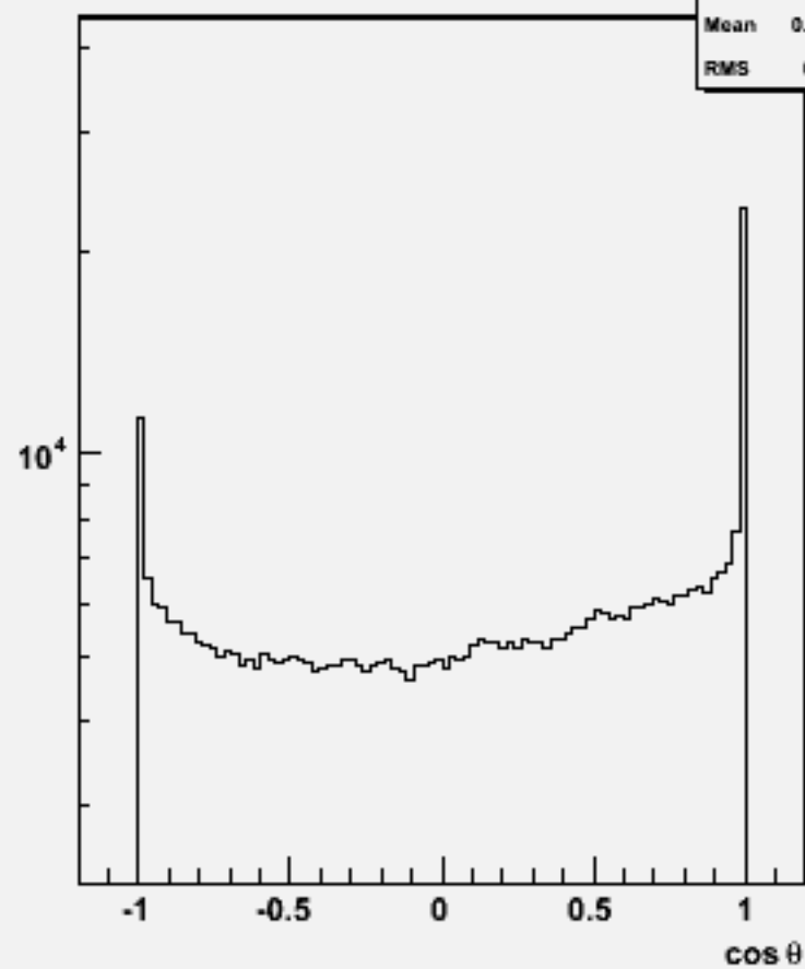
Particle cos \theta : w101738 ccn3e3e1n1_o
