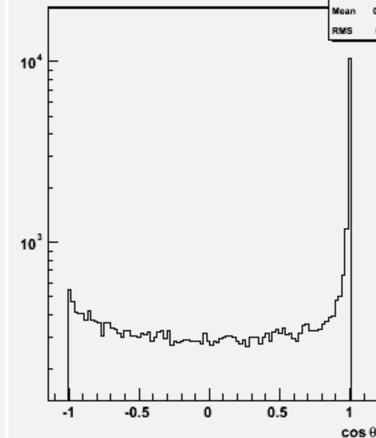
Jet cos \theta (All jets)w101738 ccn3e3e1n1_o
