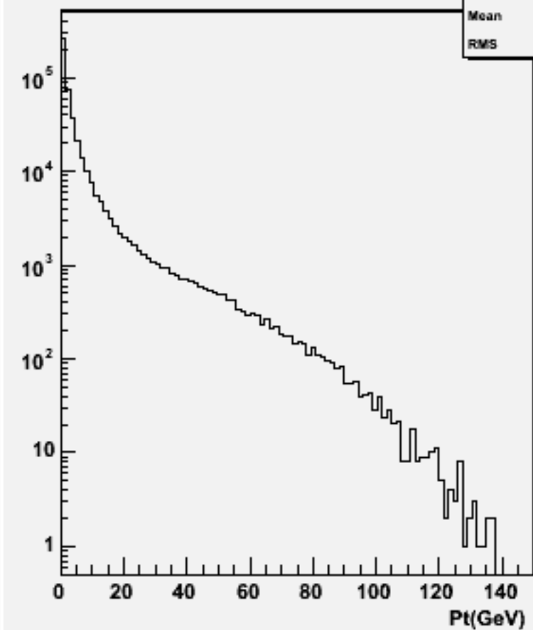
Particle Pt : w101738 ccn3e3e1n1_o
