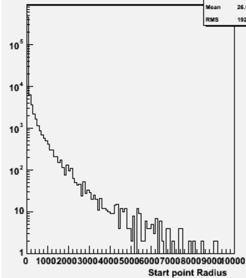
Start point R : w101738 ccn3e3e1n1_o
