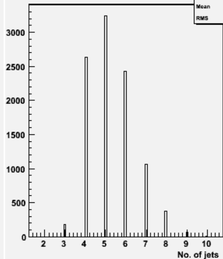
No. jets (ycut=0.001) : w101738 ccn3e3e1n1_o
