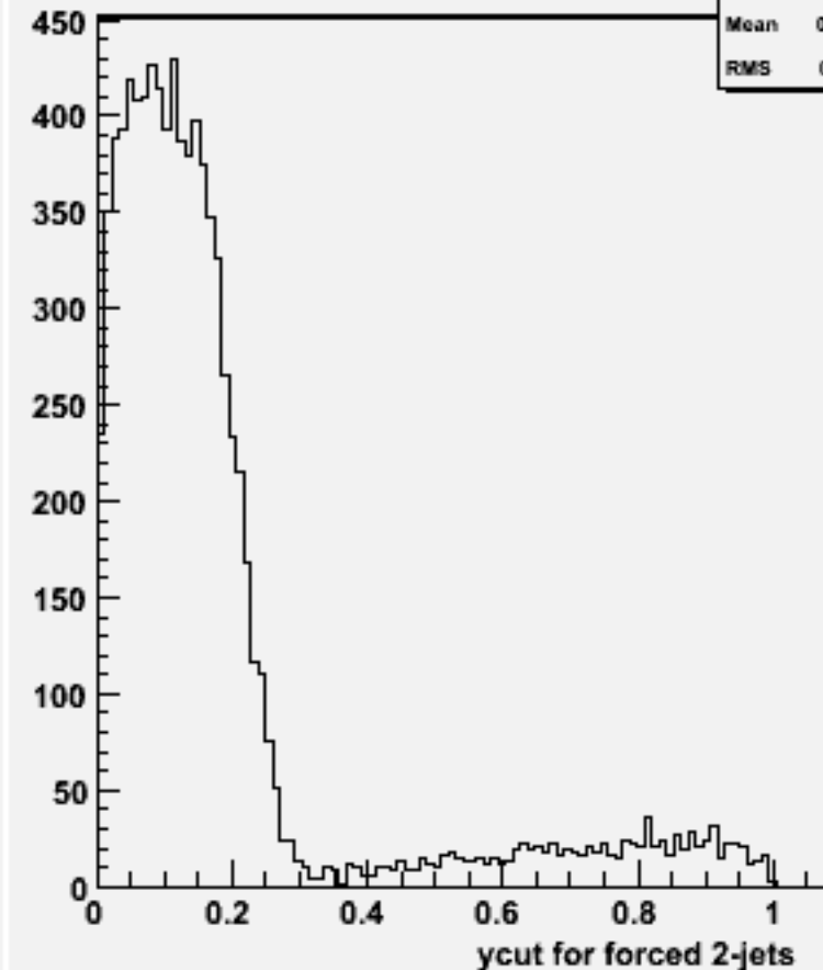
Ycut for 2-jets :w101738 ccn3e3e1n1_o
