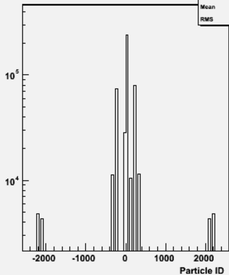
Particle ID : w101738 ccn3e3e1n1_o
