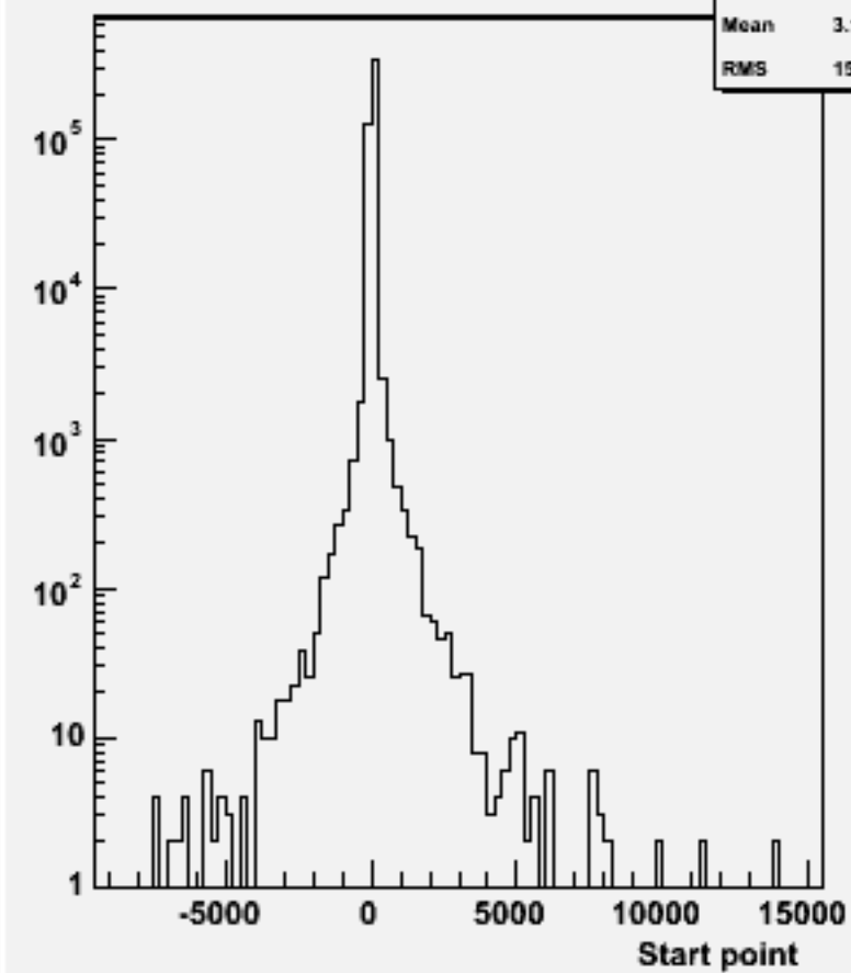
Start point Z : w101738 ccn3e3e1n1_o
