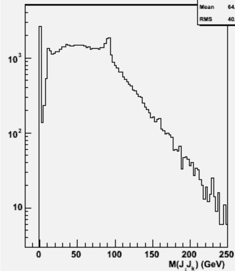
2jets mass(All comb)w101738 ccn3e3e1n1_o
