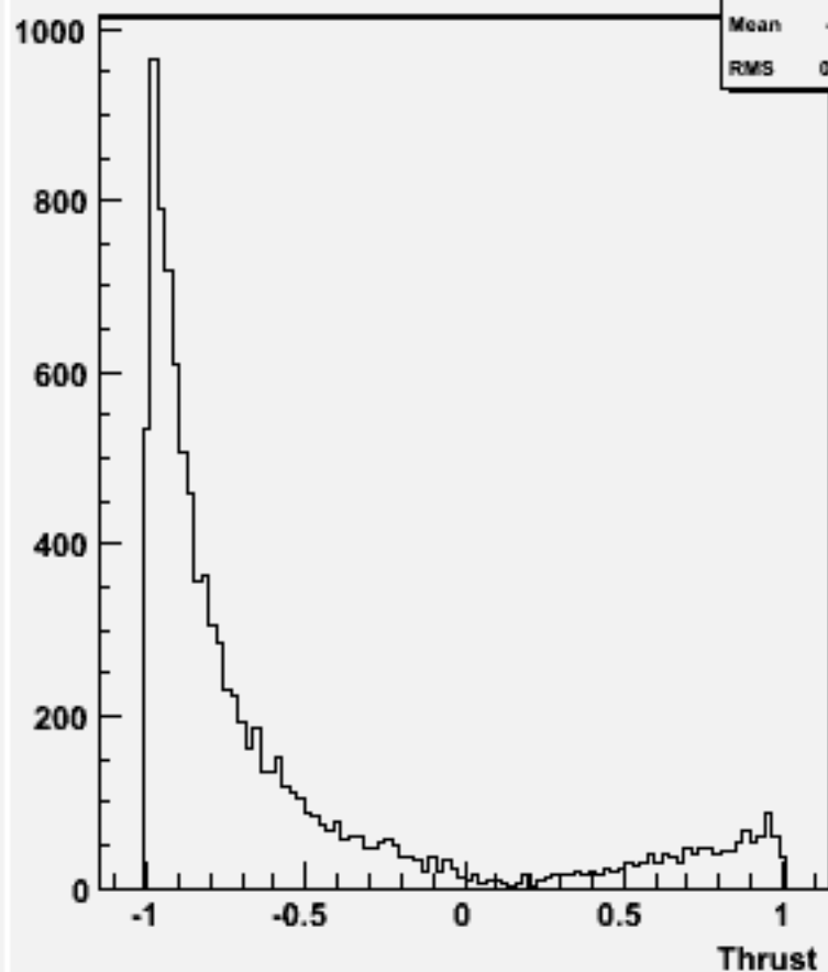
cos \Theta (thrust) w101738 ccn3e3e1n1_o
