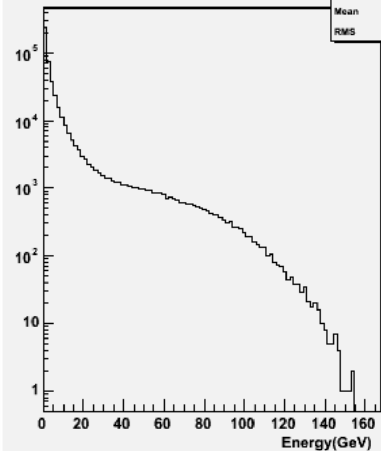
Particle Energy : w101738 ccn3e3e1n1_o
