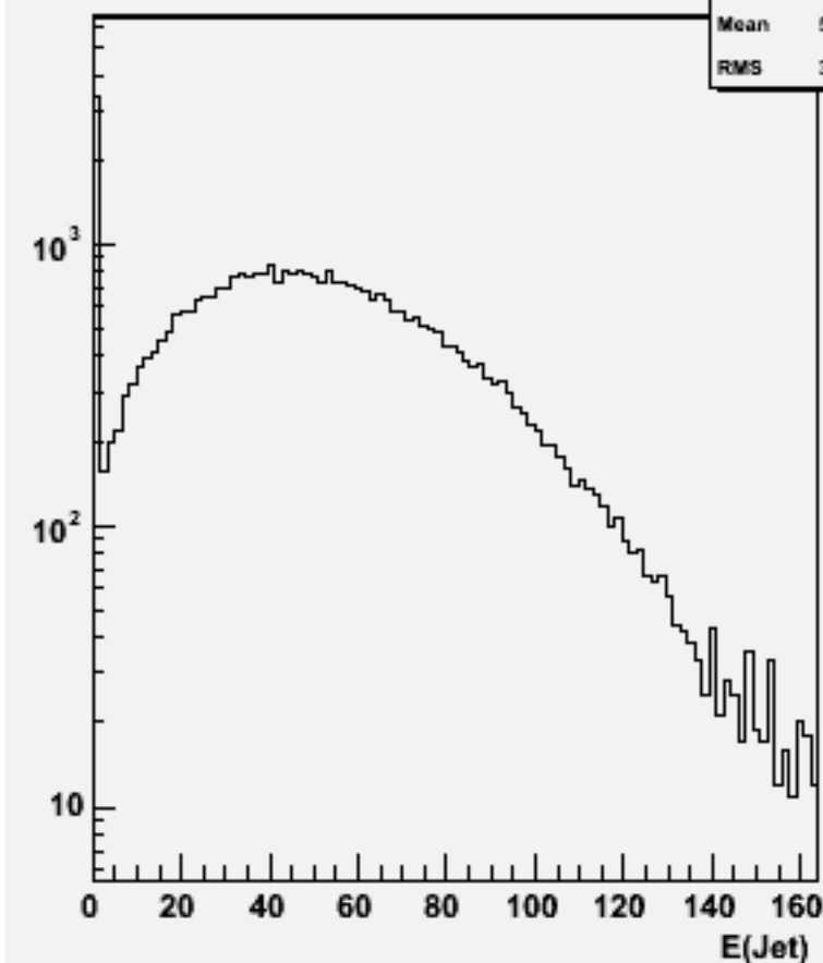
Jet energies(All jets)w101738 ccn3e3e1n1_o
