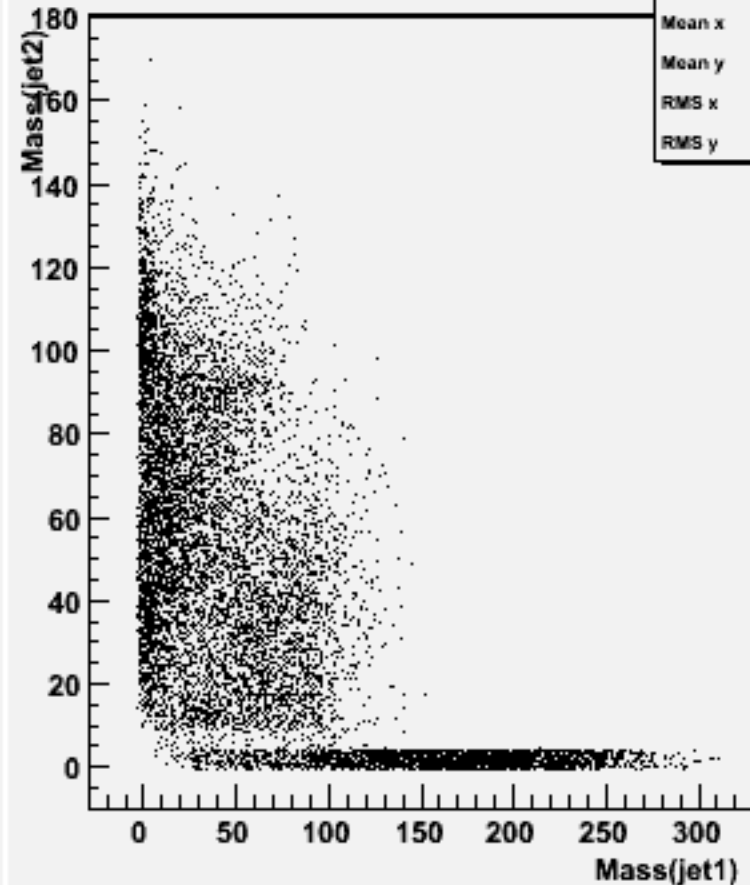
Jet mass for forced 2-jets : w101738 ccn3e3e1n1_o
