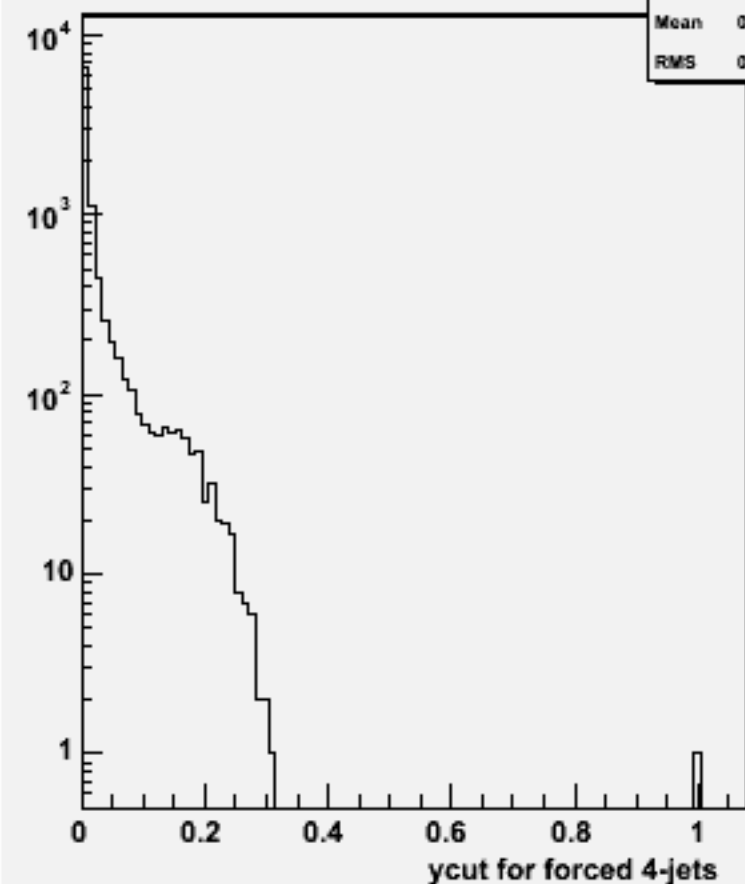
Ycut for 4-jets :w101738 ccn3e3e1n1_o
