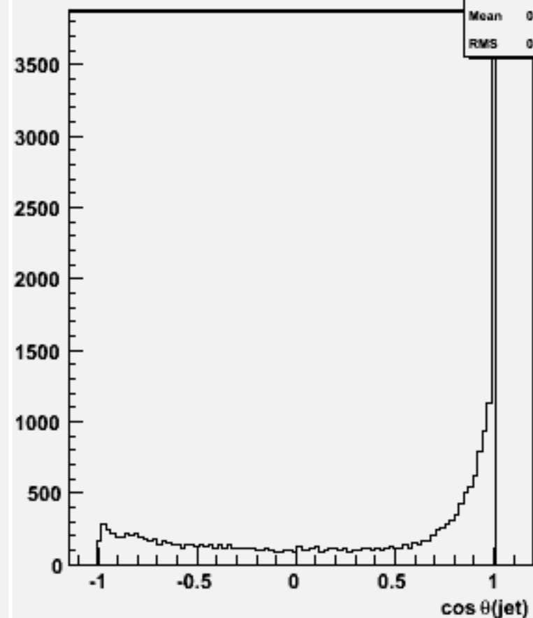
cos \theta for 2-jets :w101738 ccn3e3e1n1_o
