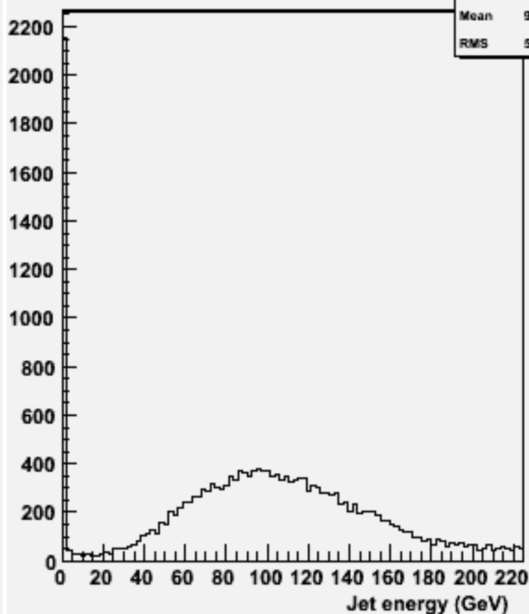
energy for 2-jets :w101738 ccn3e3e1n1_o
