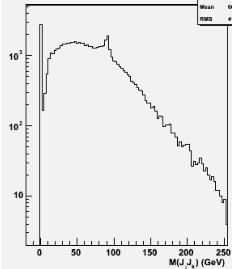
2jets mass(All comb)w101737 ccn3e3e1n1_o
