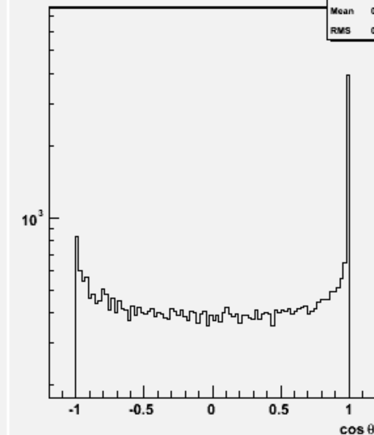
Jet cos \theta (All jets)w101737 ccn3e3e1n1_o
