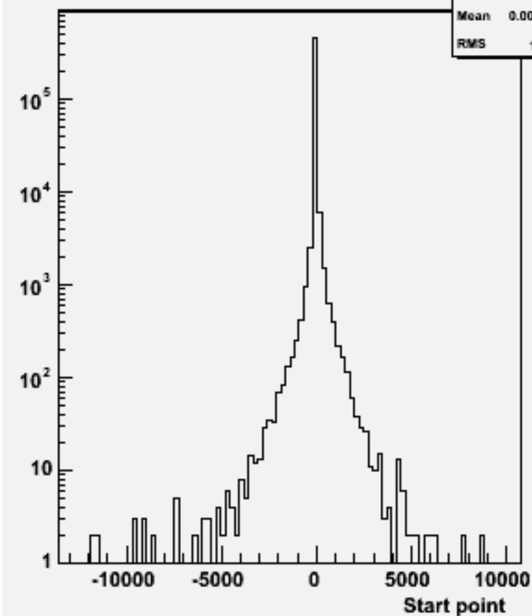
Start point Z : w101737 ccn3e3e1n1_o
