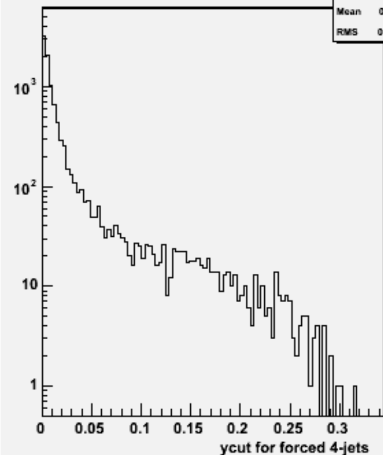
Ycut for 4-jets :w101737 ccn3e3e1n1_o
