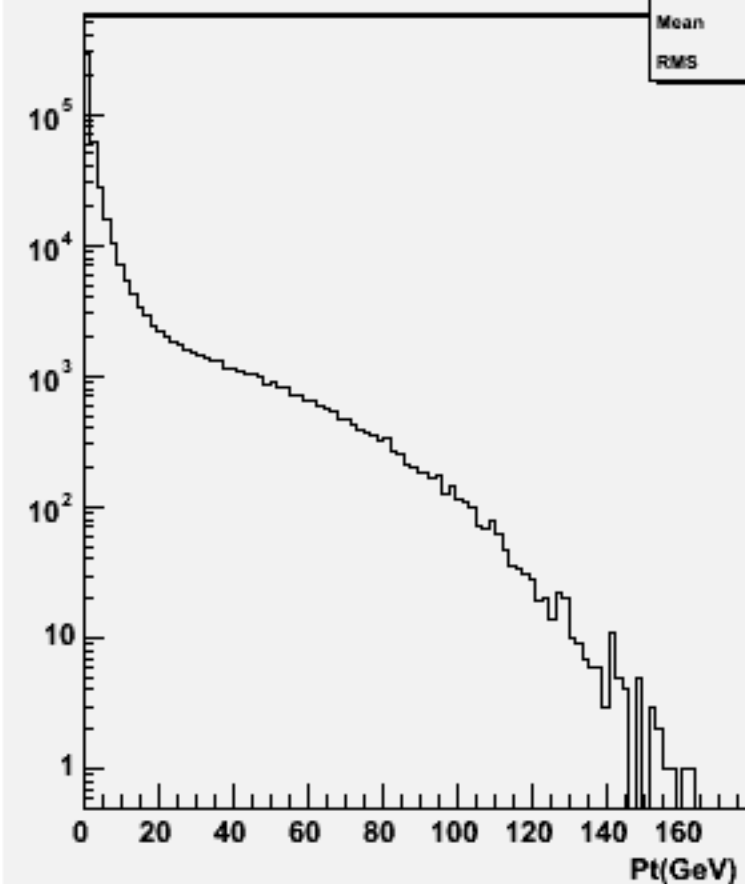
Particle Pt : w101737 ccn3e3e1n1_o
