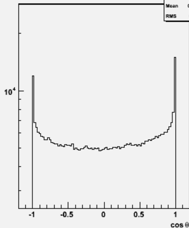
Particle \cos\theta : w101737 ccn3e3e1n1_o
