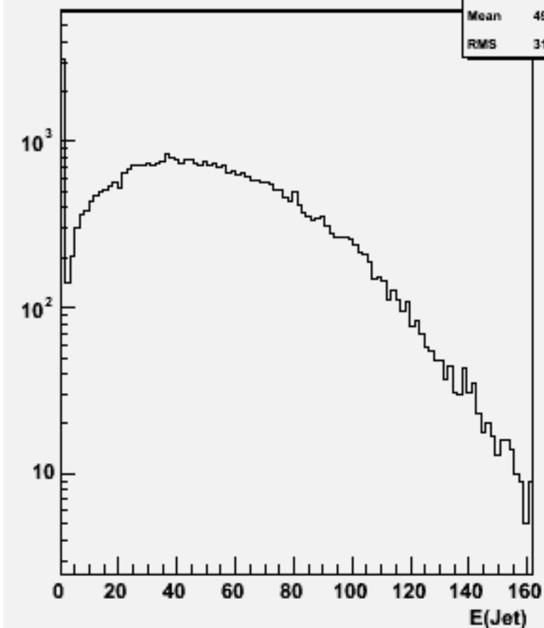
Jet energies(All jets)w101737 ccn3e3e1n1_o
