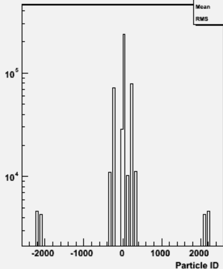
Particle ID : w101737 ccn3e3e1n1_o
