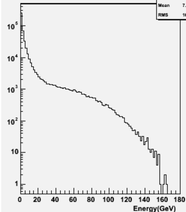
Particle Energy : w101737 ccn3e3e1n1_o
