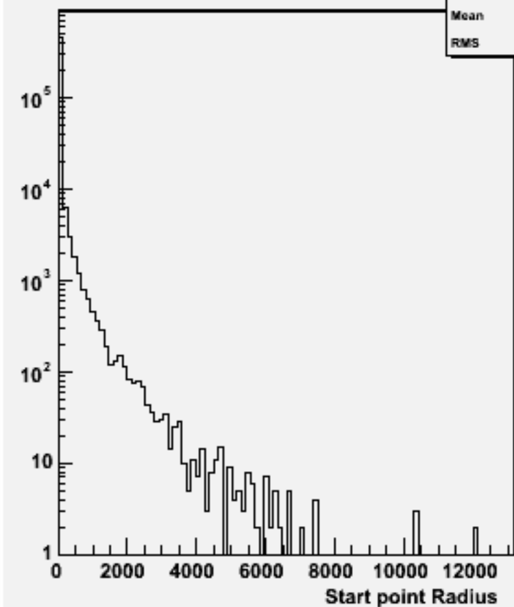
Start point R : w101737 ccn3e3e1n1_o
