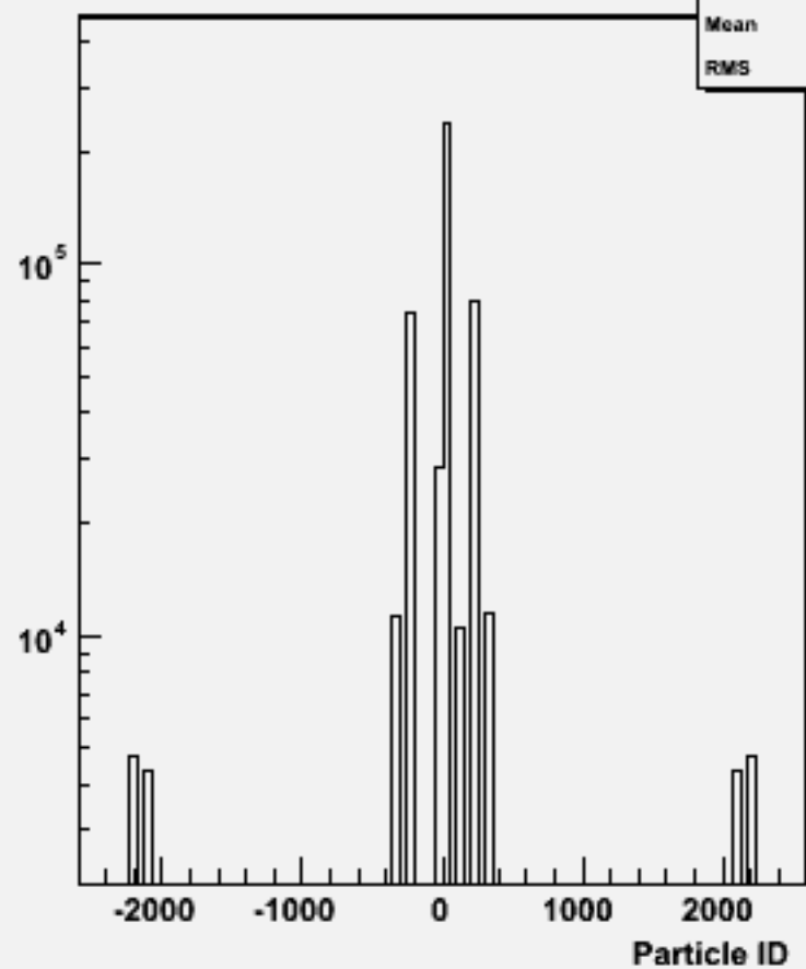
Particle ID : w101736 ccn3e3e1n1_o
