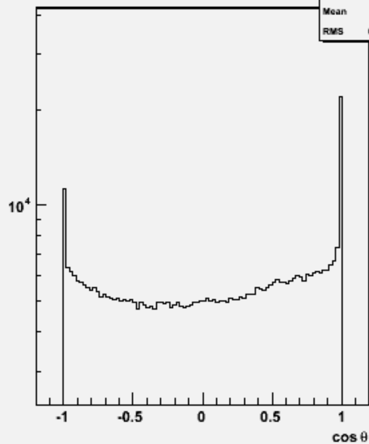
Particle cos \theta : w101736 ccn3e3e1n1_o
