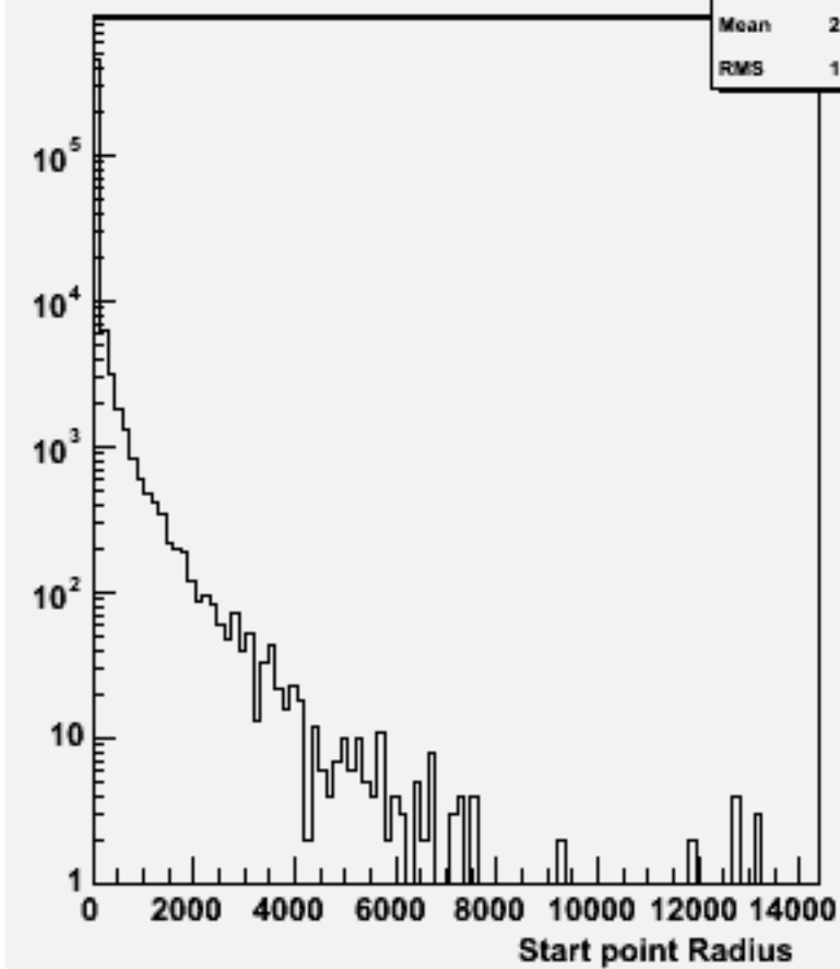
Start point R : w101736 ccn3e3e1n1_o
