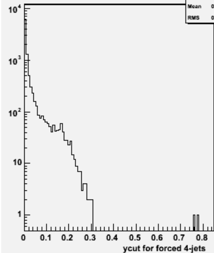
Ycut for 4-jets :w101736 ccn3e3e1n1_o
