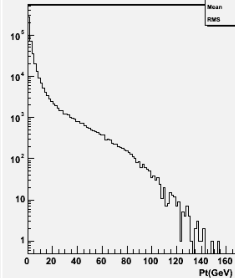
Particle Pt : w101736 ccn3e3e1n1_o
