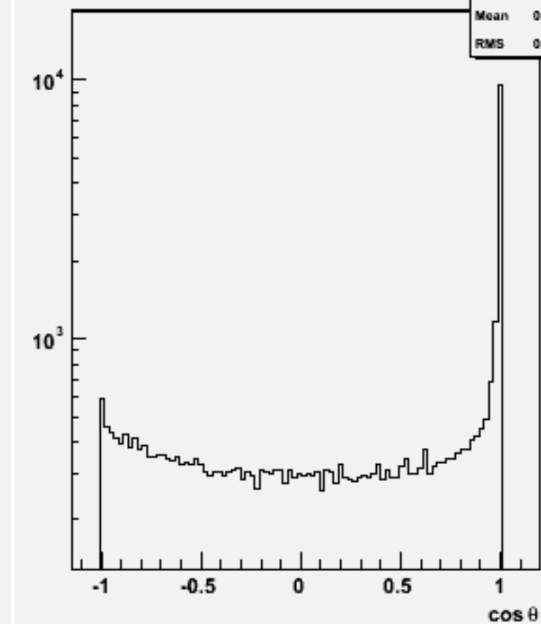
Jet cos \theta (All jets)w101736 ccn3e3e1n1_o
