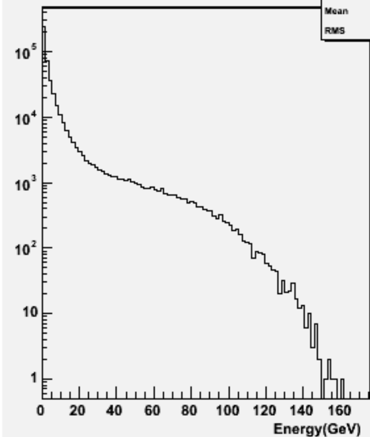
Particle Energy : w101736 ccn3e3e1n1_o
