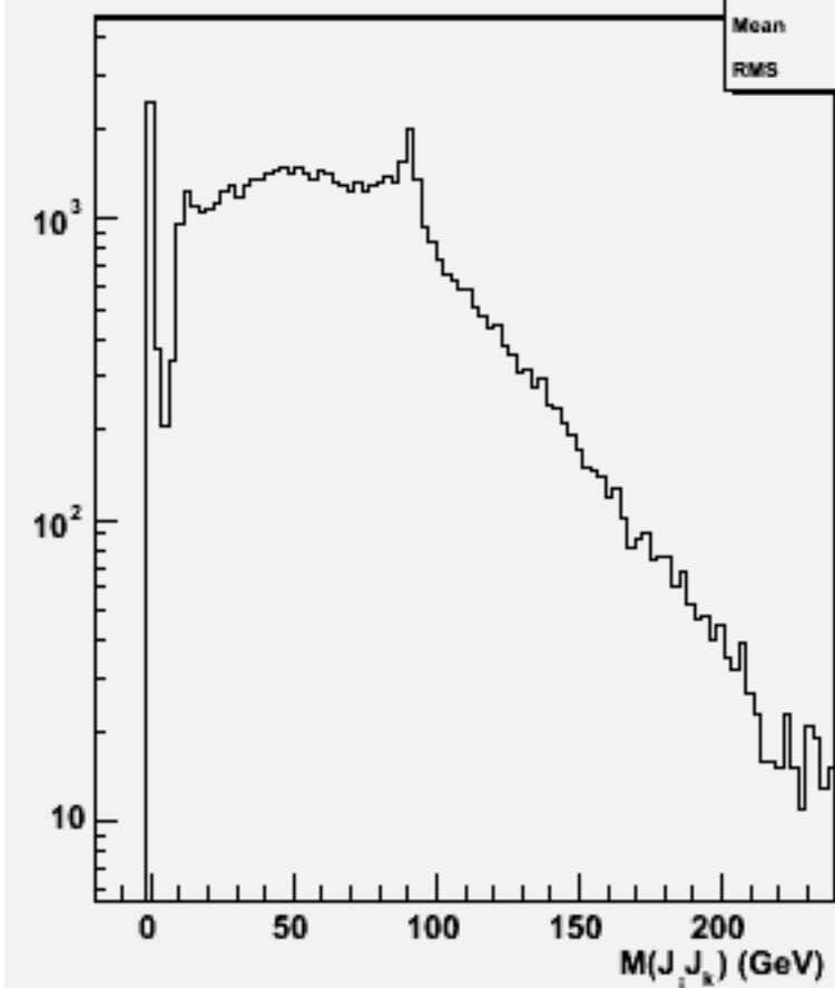
2jets mass(All comb)w101736 ccn3e3e1n1_o
