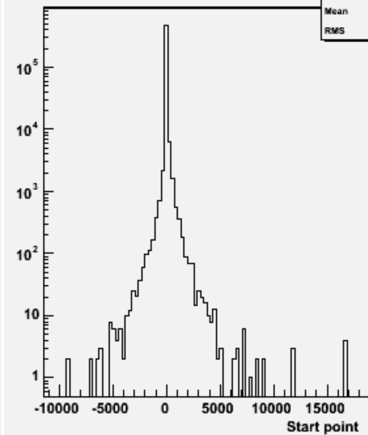
Start point Z : w101736 ccn3e3e1n1_o
