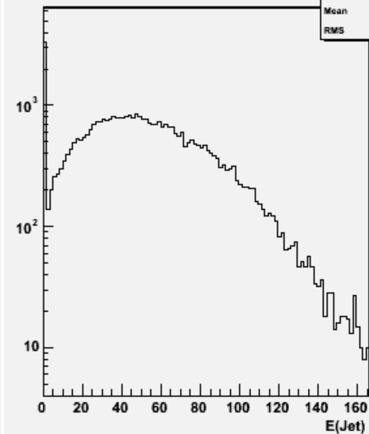
Jet energies(All jets)w101736 ccn3e3e1n1_o
