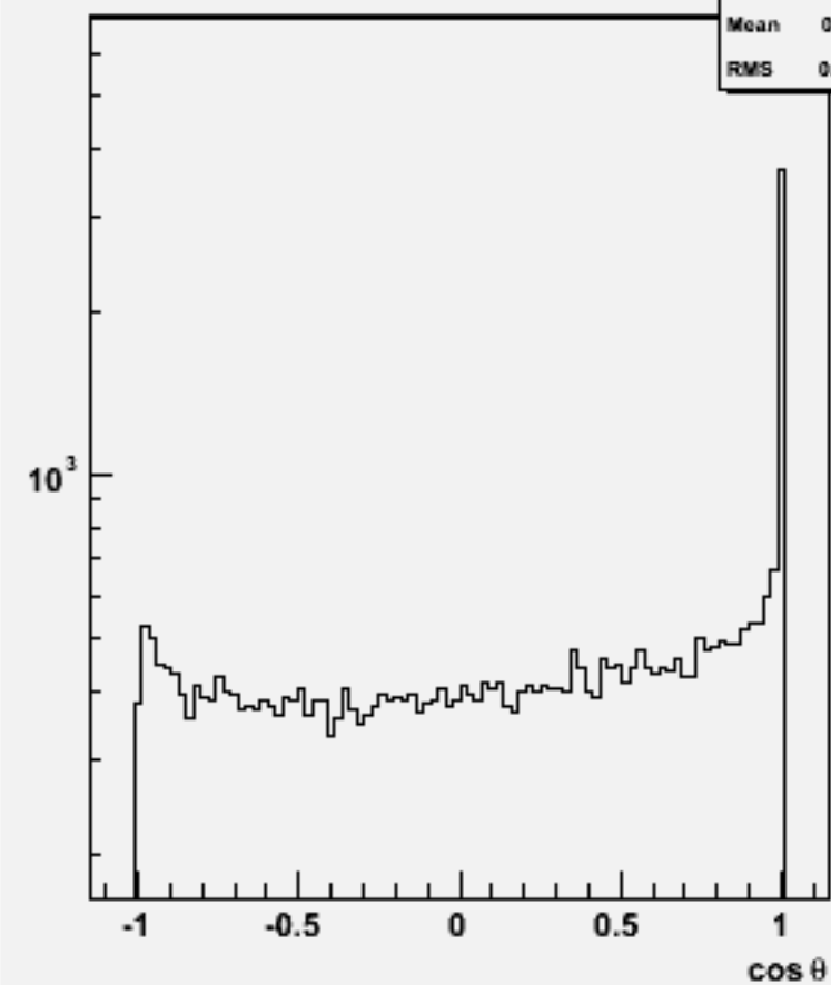
Jet cosθ (All jets)w101733 ccn2e2sc_o
