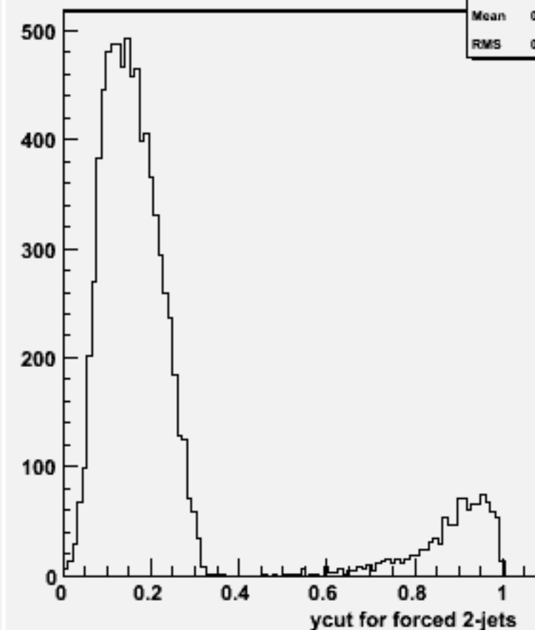
Ycut for 2-jets :w101733 ccn2e2sc_o
