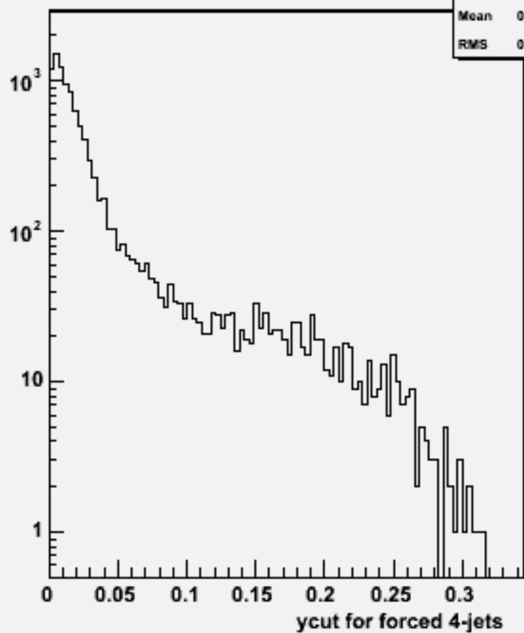
Ycut for 4-jets :w101733 ccn2e2sc_o
