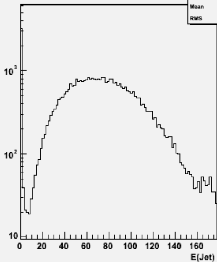
Jet energies(All jets)w101733 ccn2e2sc_o
