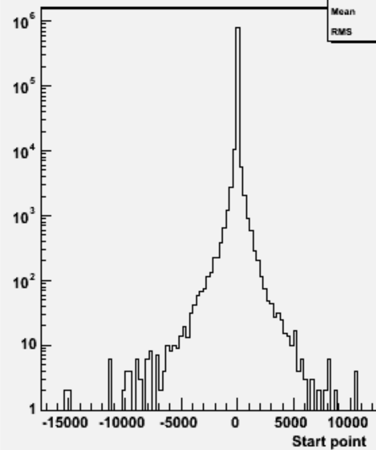
Start point Z : w101733 ccn2e2sc_o
