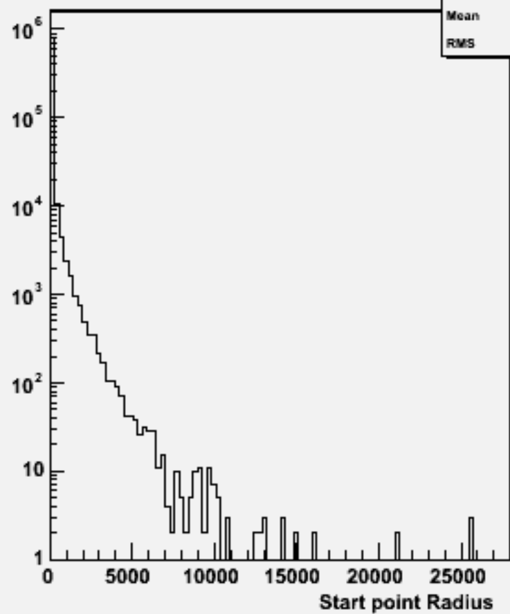
Start point R : w101733 ccn2e2sc_o
