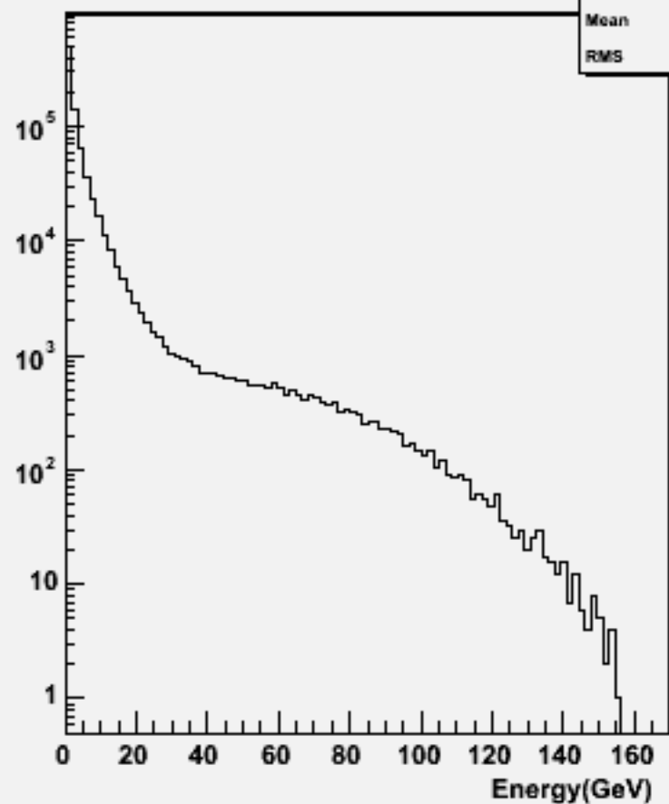
Particle Energy : w101733 ccn2e2sc_o
