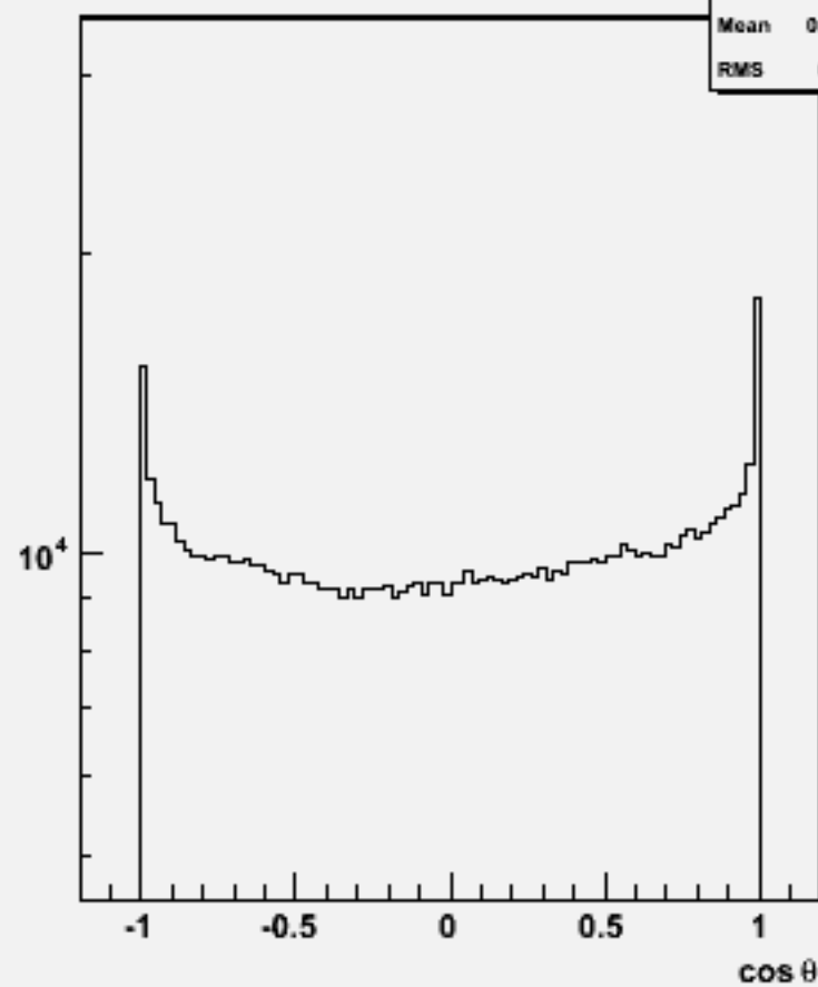
Particle cos \theta : w101733 ccn2e2sc_o
