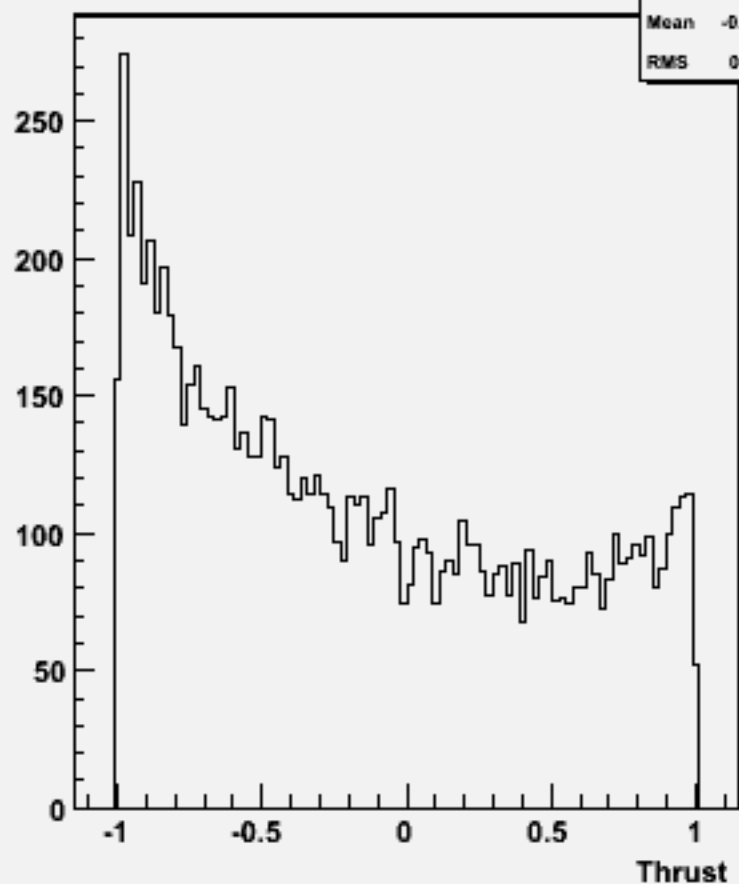
cos \Theta (thrust) w101733 ccn2e2sc_o
