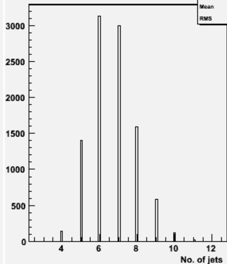
No. jets (ycut=0.001) : w101733 ccn2e2sc_o
