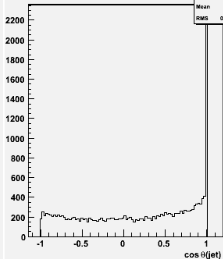
cos \theta for 2-jets :w101733 ccn2e2sc_o
