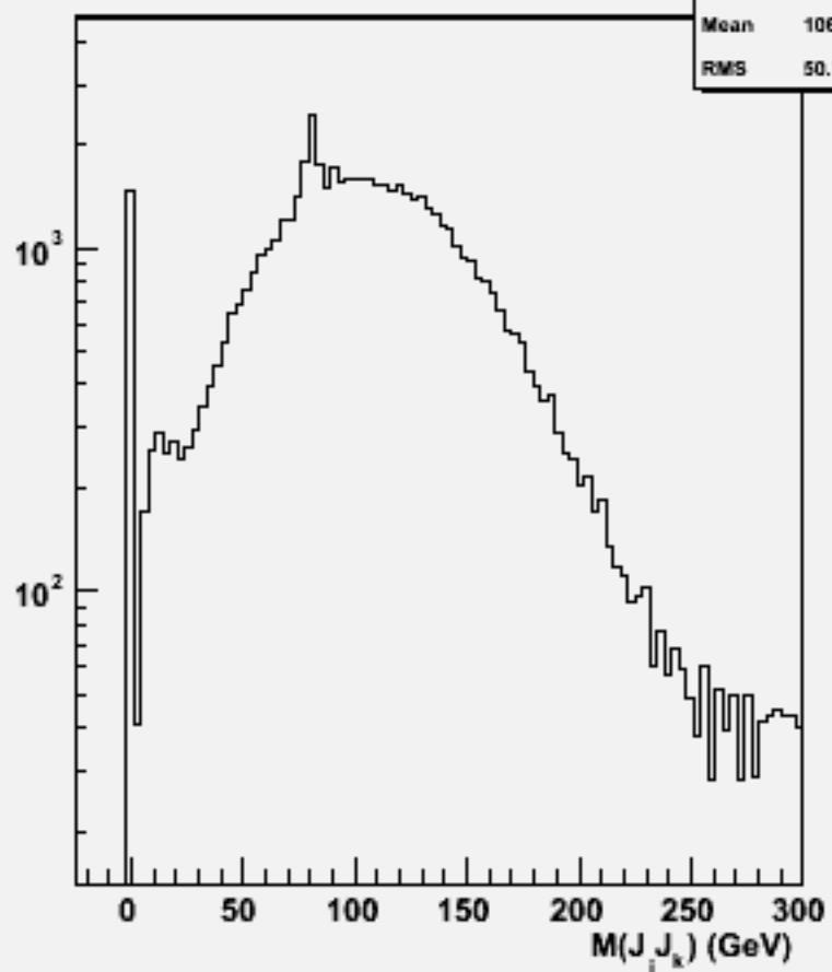
2jets mass(All comb)w101733 ccn2e2sc_o
