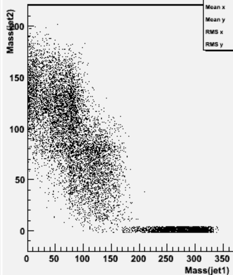
Jet mass for forced 2-jets : w101733 ccn2e2sc_o
