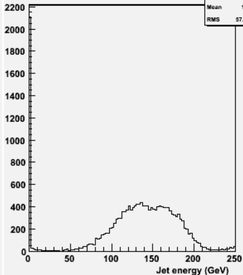
energy for 2-jets :w101733 ccn2e2sc_o
