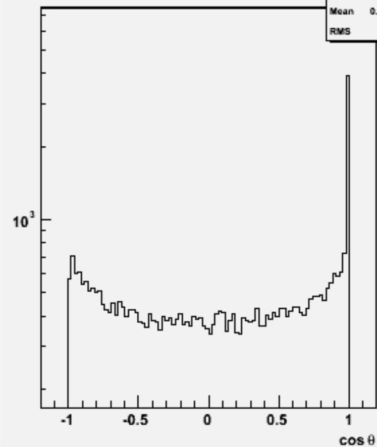
Jet cosθ (All jets)w101732 ccn2e2sc_o
