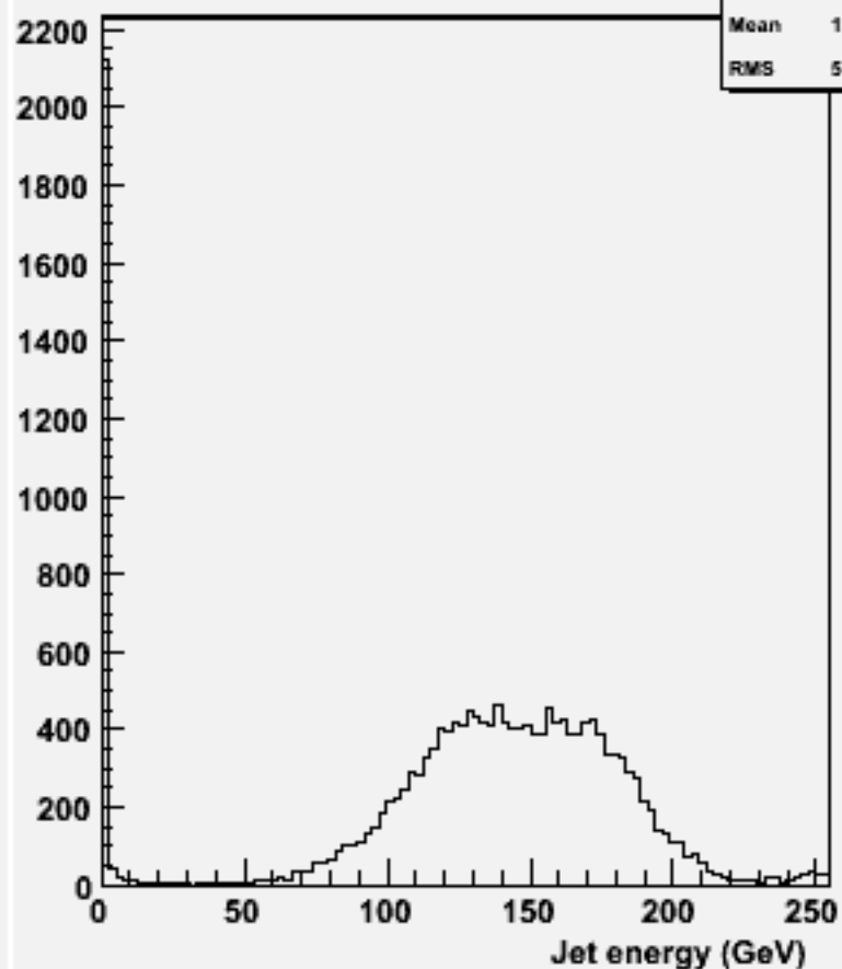
energy for 2-jets :w101732 ccn2e2sc_o
