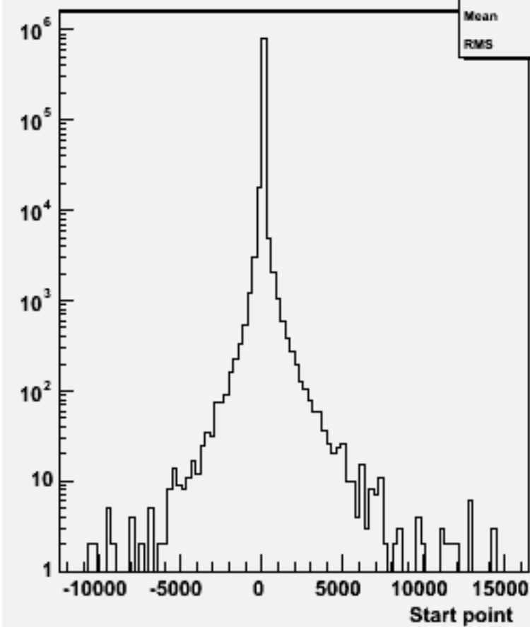
Start point Z : w101732 ccn2e2sc_o
