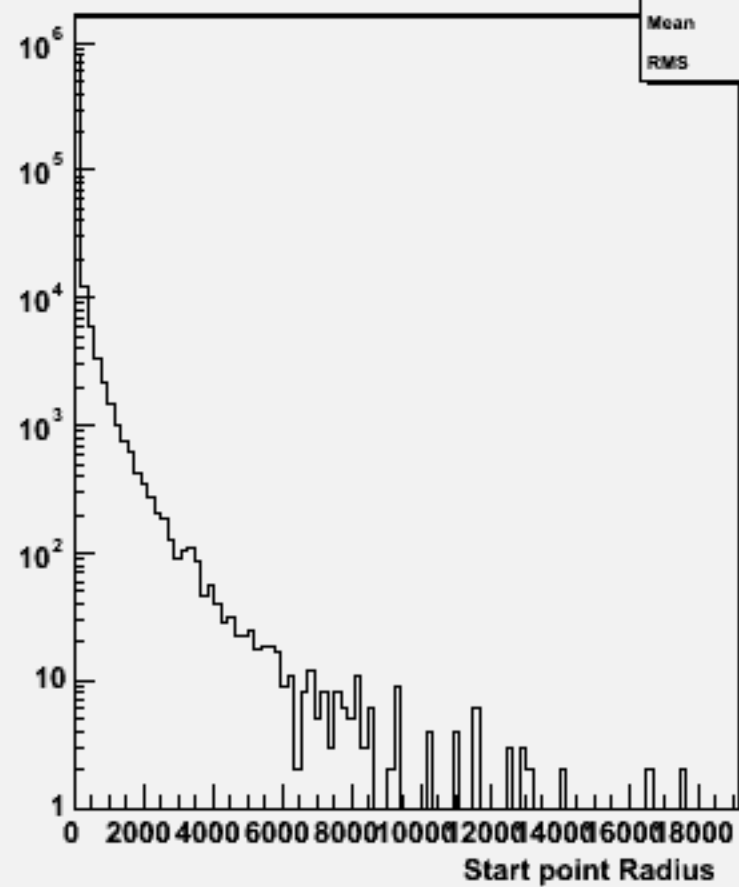
Start point R : w101732 ccn2e2sc_o
