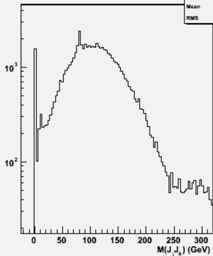
2jets mass(All comb)w101732 ccn2e2sc_o
