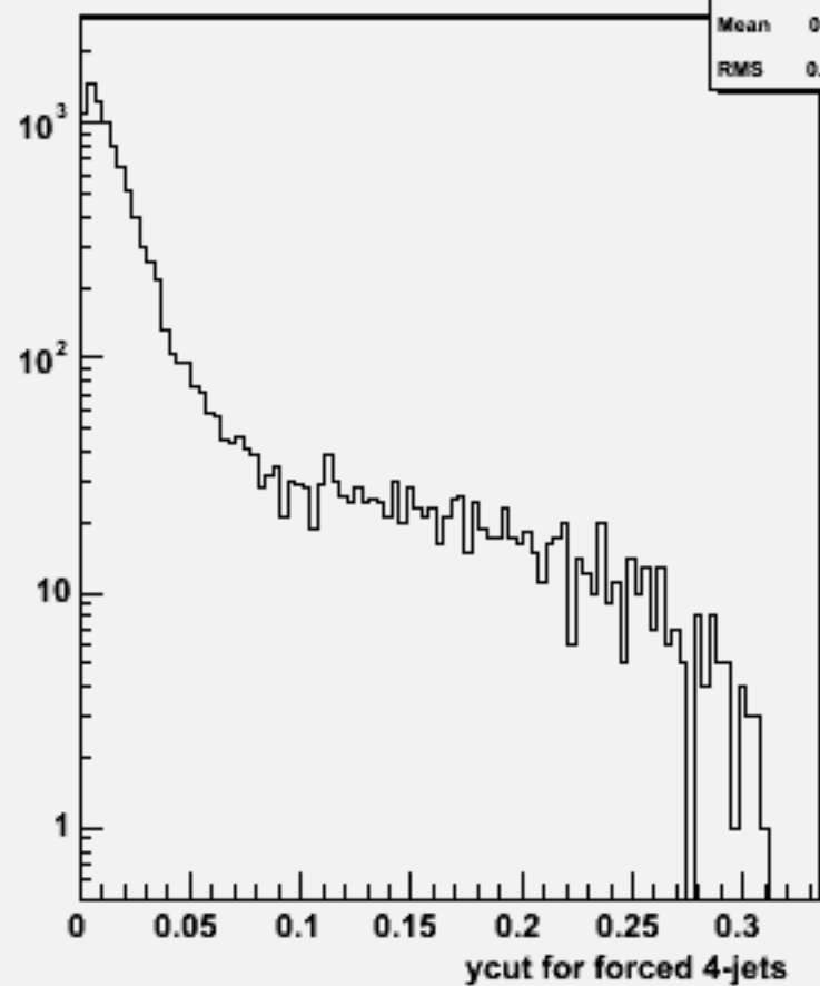
Ycut for 4-jets :w101732 ccn2e2sc_o
