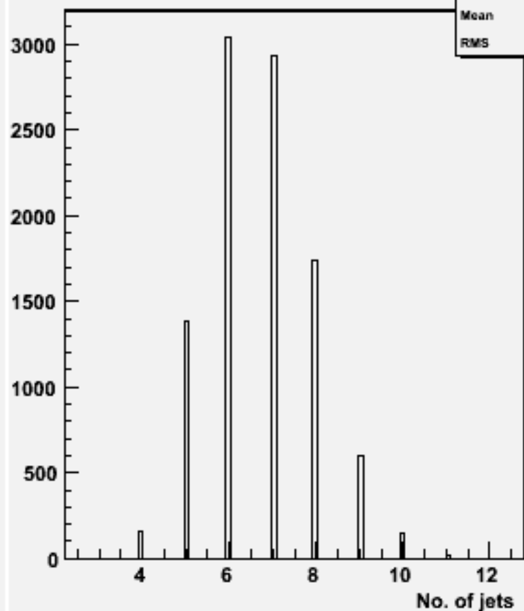
No. jets (ycut=0.001) : w101732 ccn2e2sc_o
