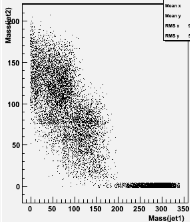
Jet mass for forced 2-jets : w101732 ccn2e2sc_o
