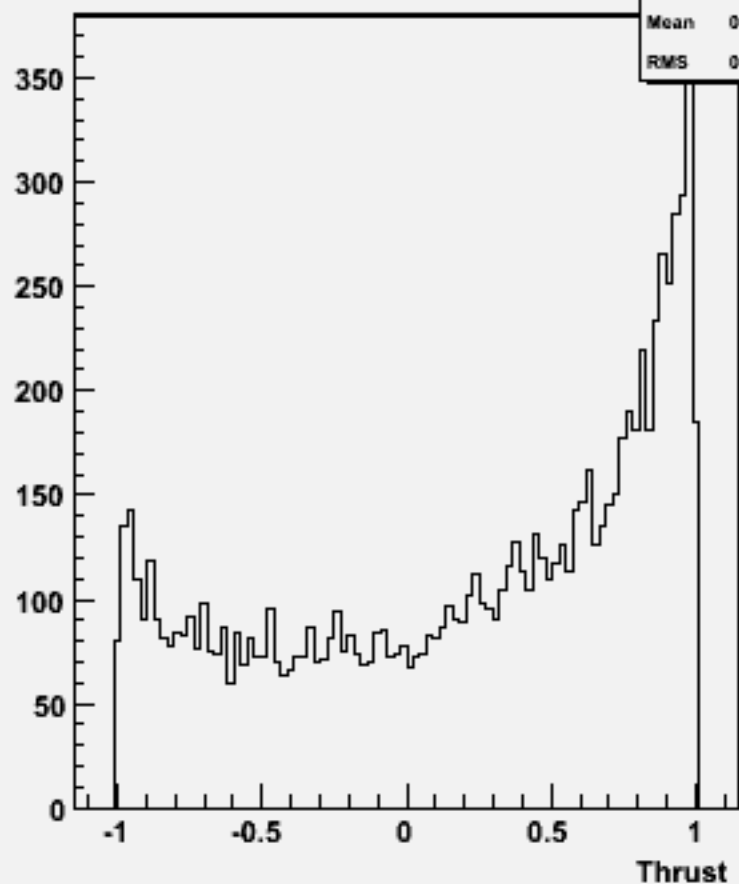
cos \Theta (thrust) w101732 ccn2e2sc_o
