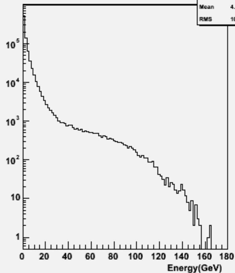
Particle Energy : w101732 ccn2e2sc_o
