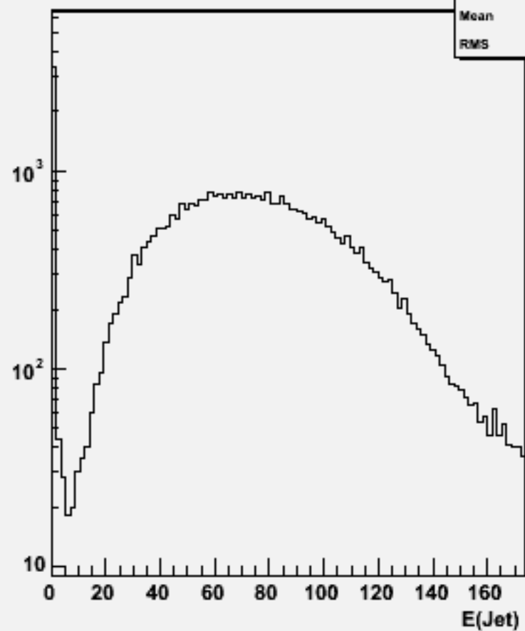
Jet energies(All jets)w101732 ccn2e2sc_o
