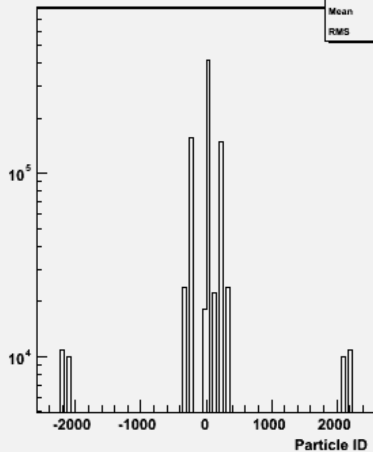
Particle ID : w101732 ccn2e2sc_o
