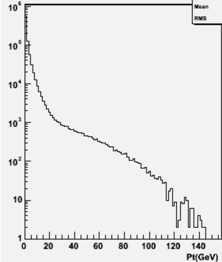
Particle Pt : w101732 ccn2e2sc_o
