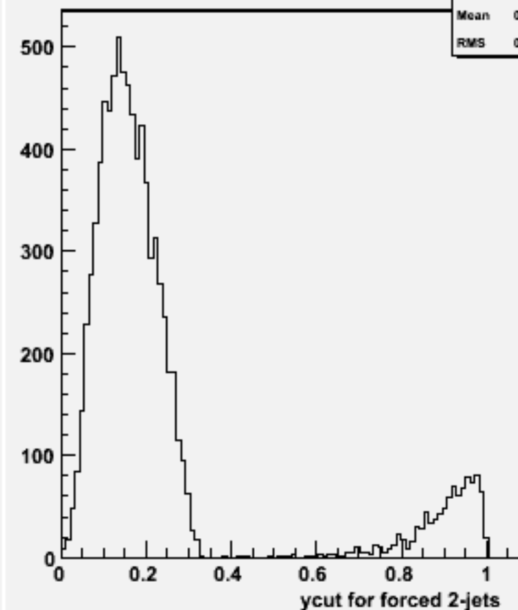
Ycut for 2-jets :w101732 ccn2e2sc_o
