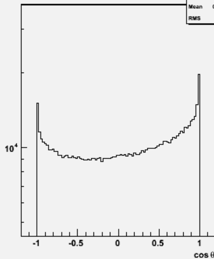
Particle cos \theta : w101732 ccn2e2sc_o
