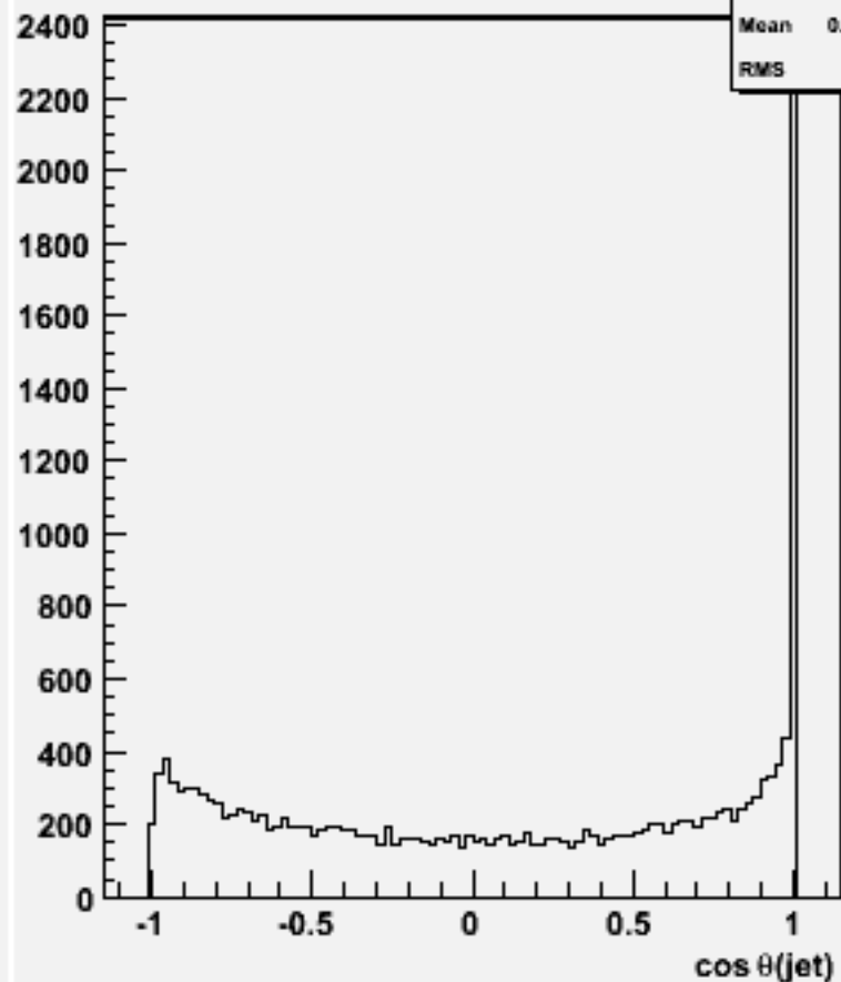
cos \theta for 2-jets :w101732 ccn2e2sc_o
