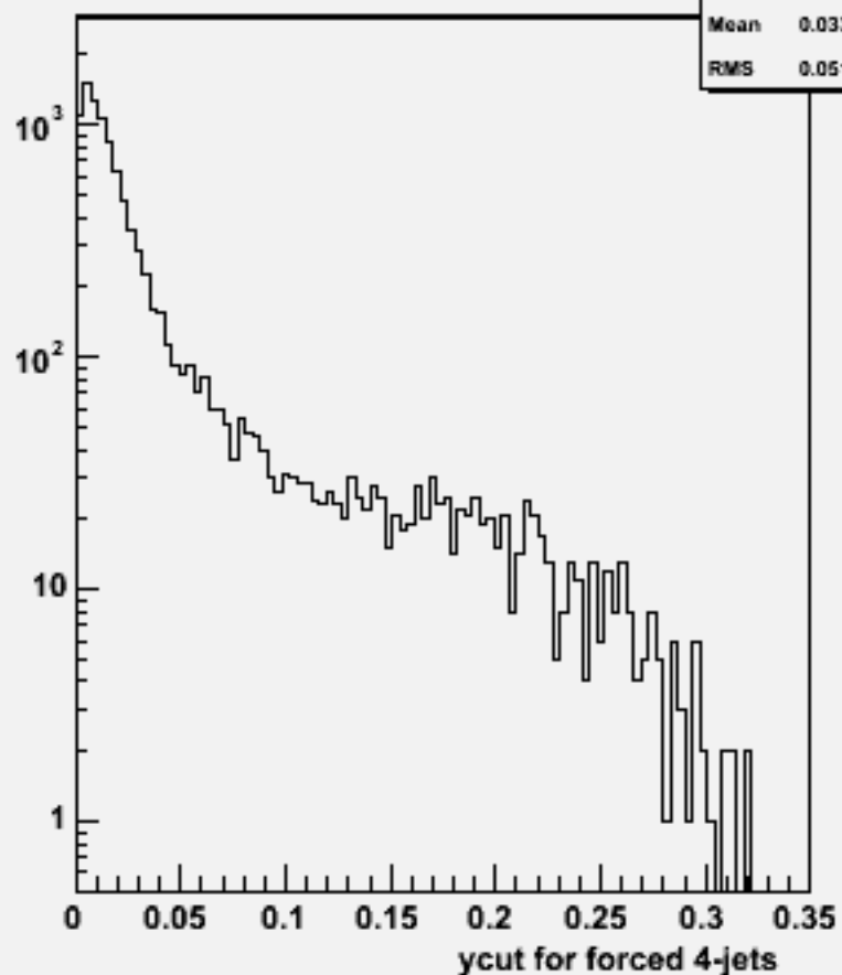
Ycut for 4-jets :w101729 ccn2e2du_o
