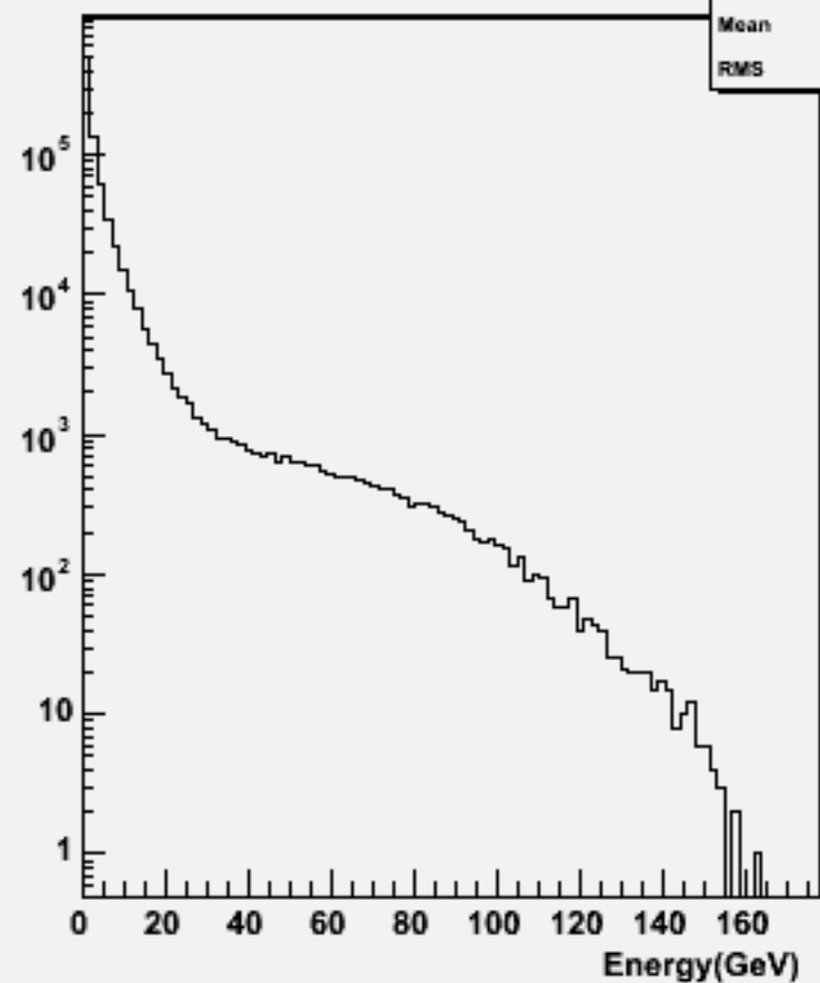
Particle Energy : w101729 ccn2e2du_o
