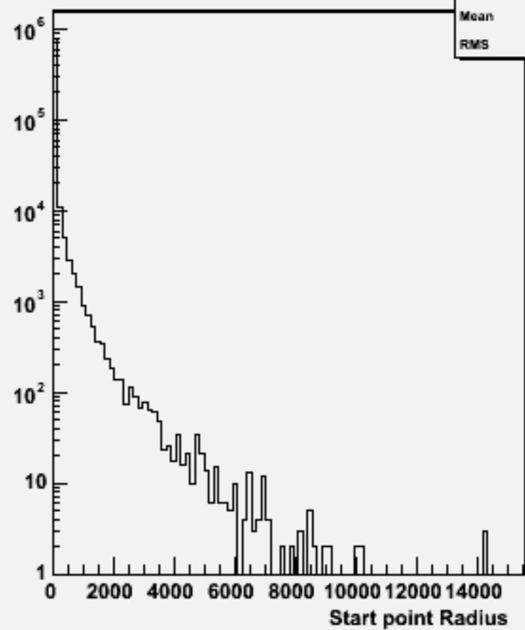
Start point R : w101729 ccn2e2du_o
