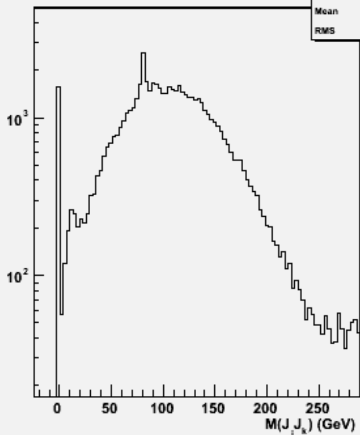
2jets mass(All comb)w101729 ccn2e2du_o
