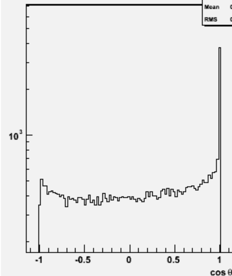
Jet cos \theta (All jets)w101729 ccn2e2du_o
