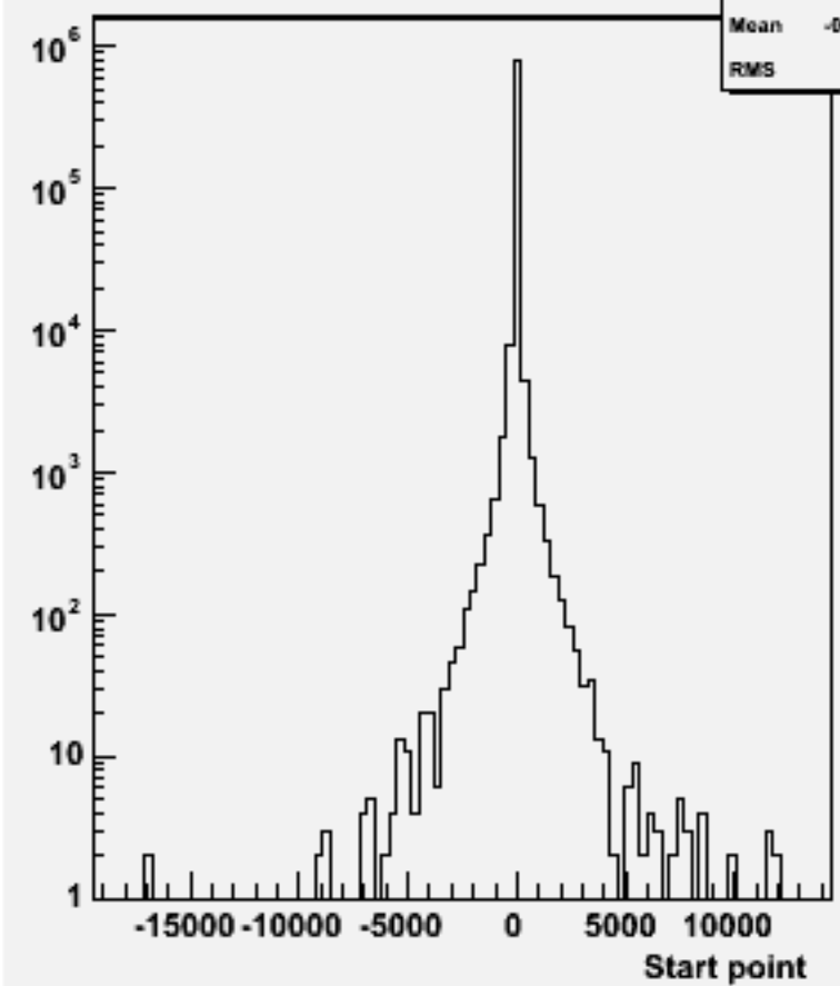
Start point Z : w101729 ccn2e2du_o
