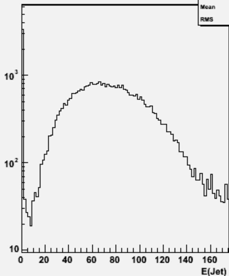
Jet energies(All jets)w101729 ccn2e2du_o
