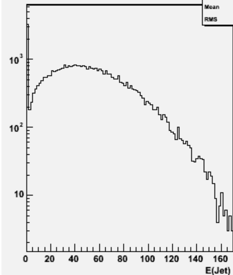
Jet energies(All jets)w101725 ccn2e2e3n3_o
