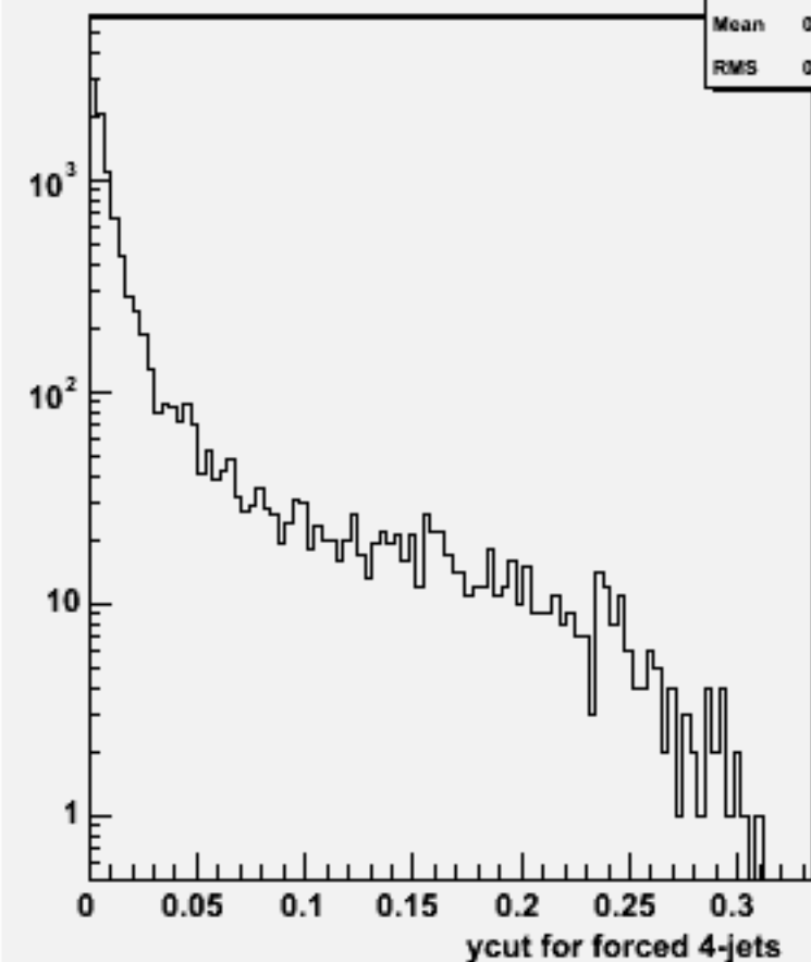
Ycut for 4-jets :w101725 ccn2e2e3n3_o
