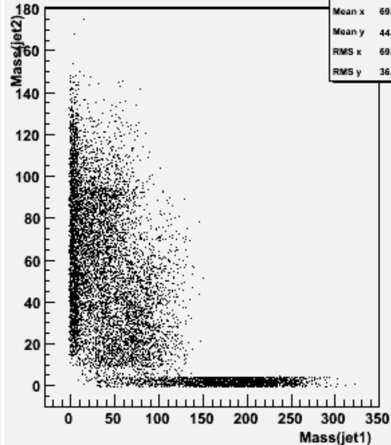
Jet mass for forced 2-jets : w101725 ccn2e2e3n3_o
