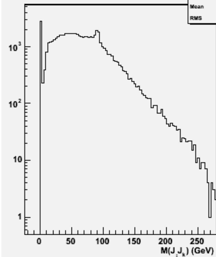
2jets mass(All comb)w101725 ccn2e2e3n3_o
