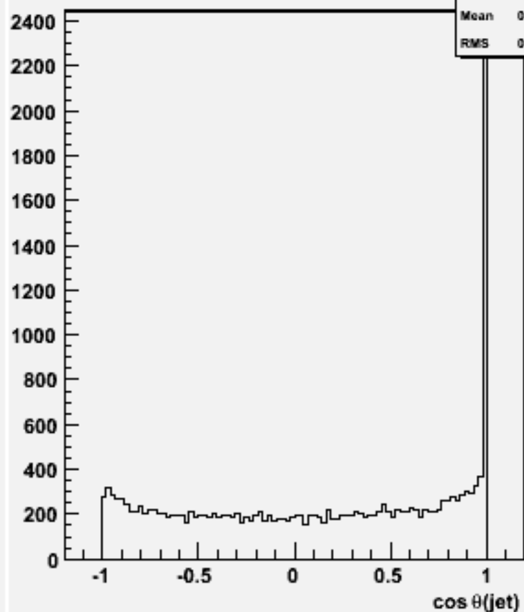
cos \theta for 2-jets :w101725 ccn2e2e3n3_o
