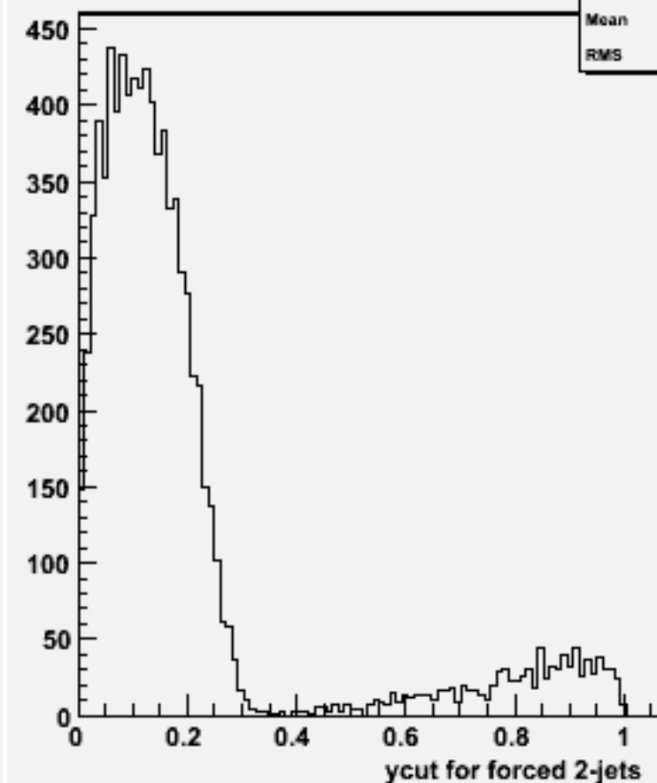
Ycut for 2-jets :w101725 ccn2e2e3n3_o
