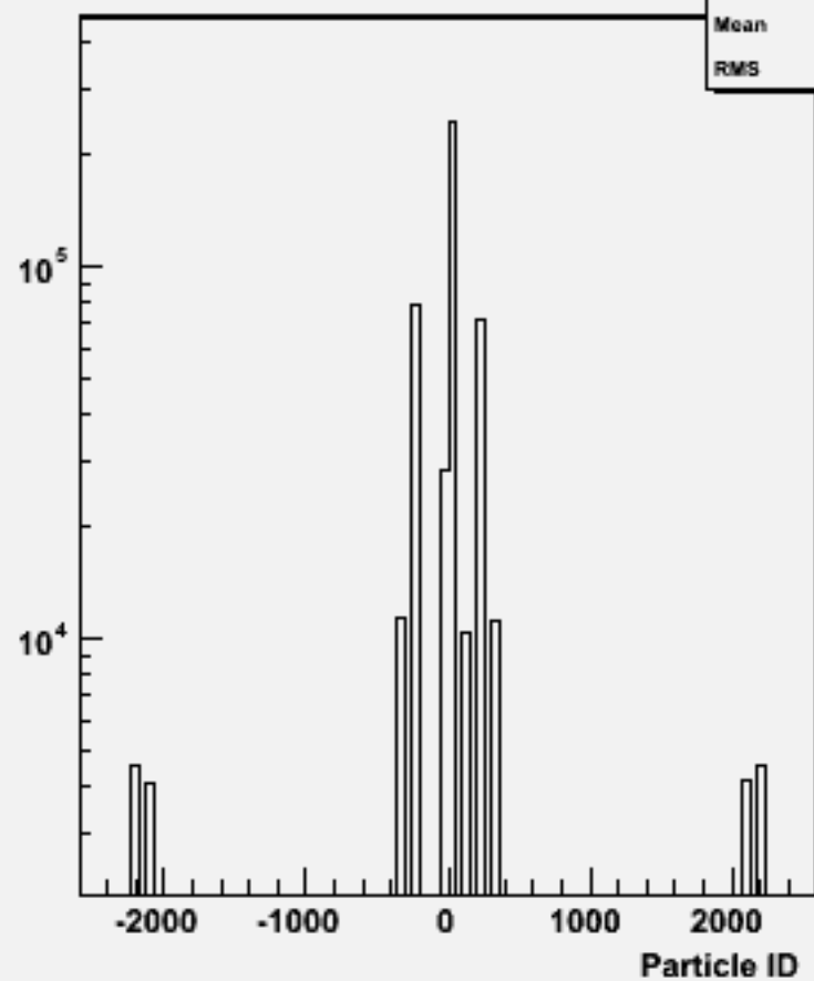
Particle ID : w101725 ccn2e2e3n3_o
