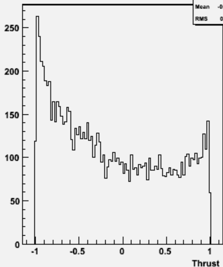
cos \Theta (thrust) w101725 ccn2e2e3n3_o
