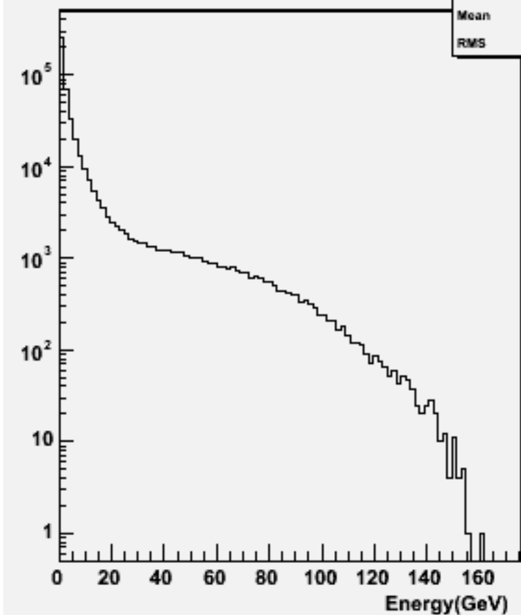
Particle Energy : w101725 ccn2e2e3n3_o
