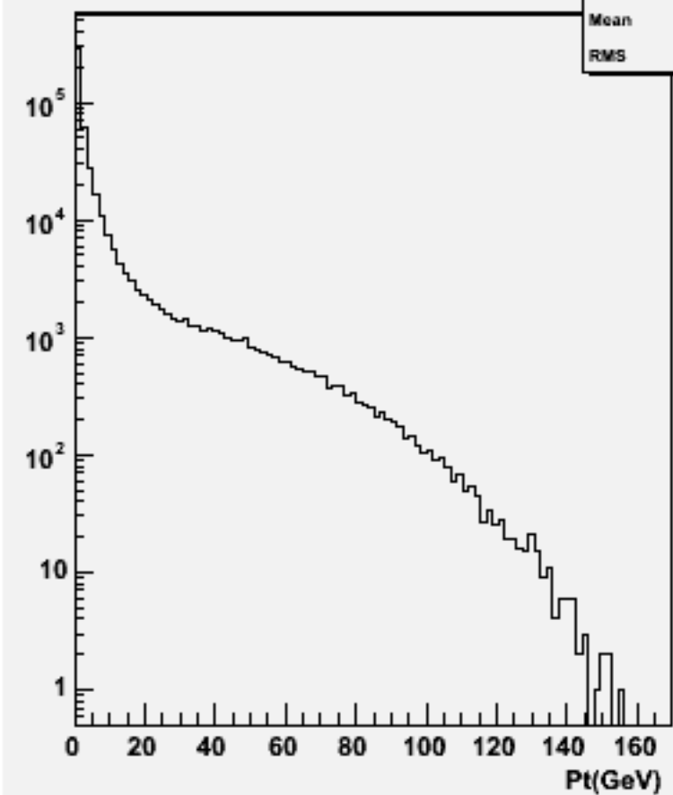
Particle Pt : w101725 ccn2e2e3n3_o
