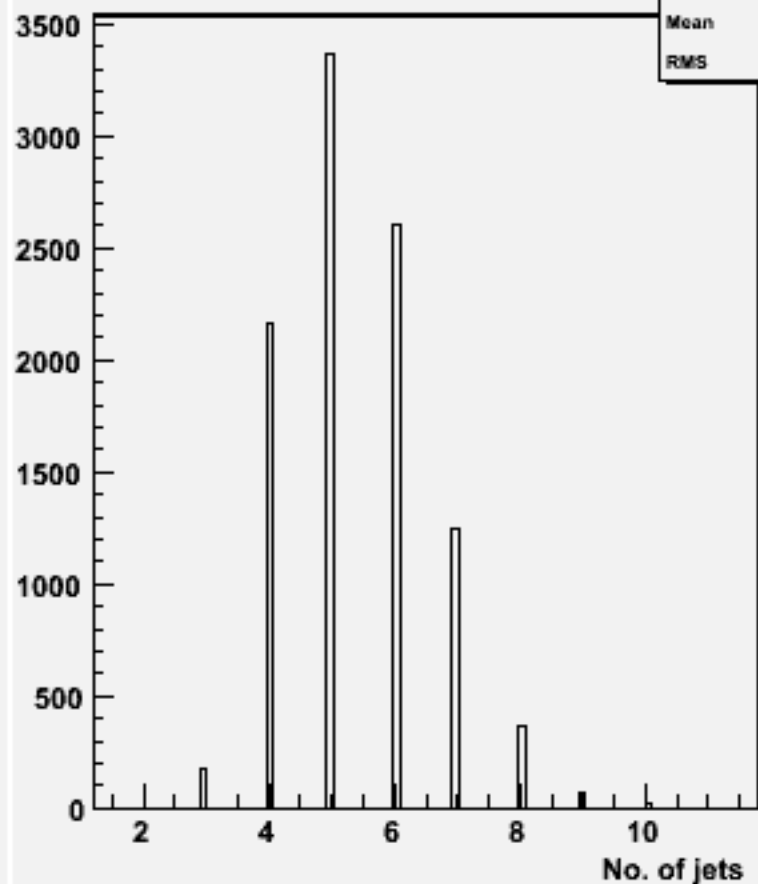
No. jets (ycut=0.001) : w101725 ccn2e2e3n3_o
