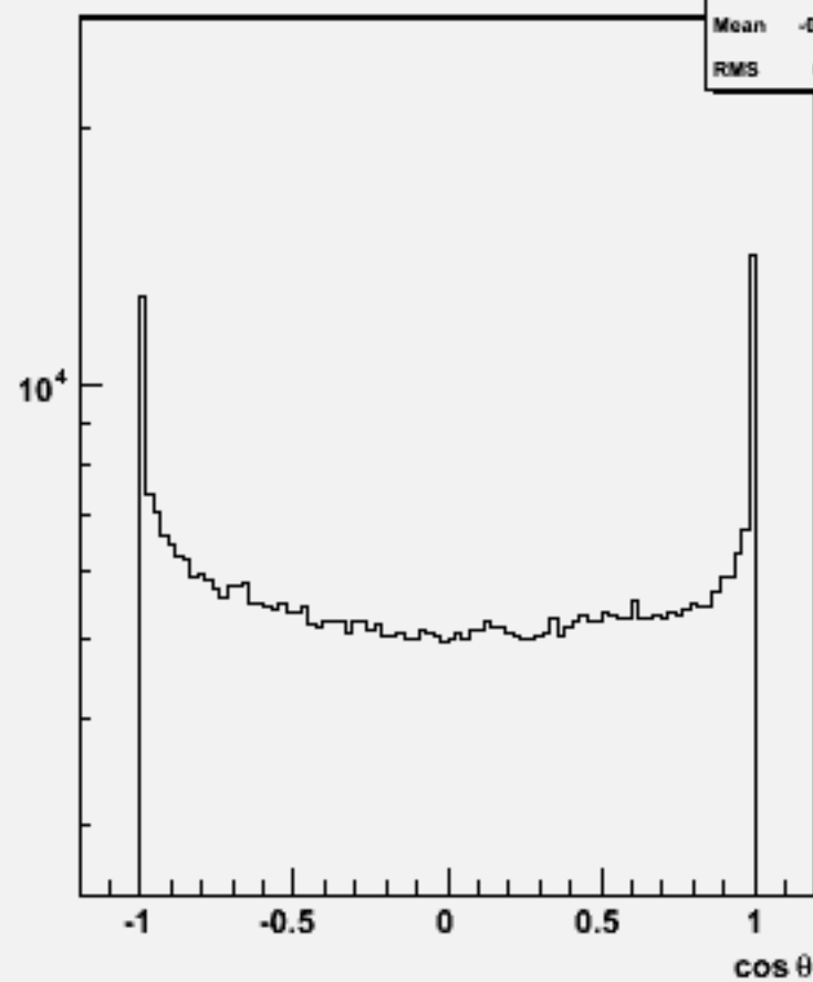
Particle cos θ : w101725 ccn2e2e3n3_o
