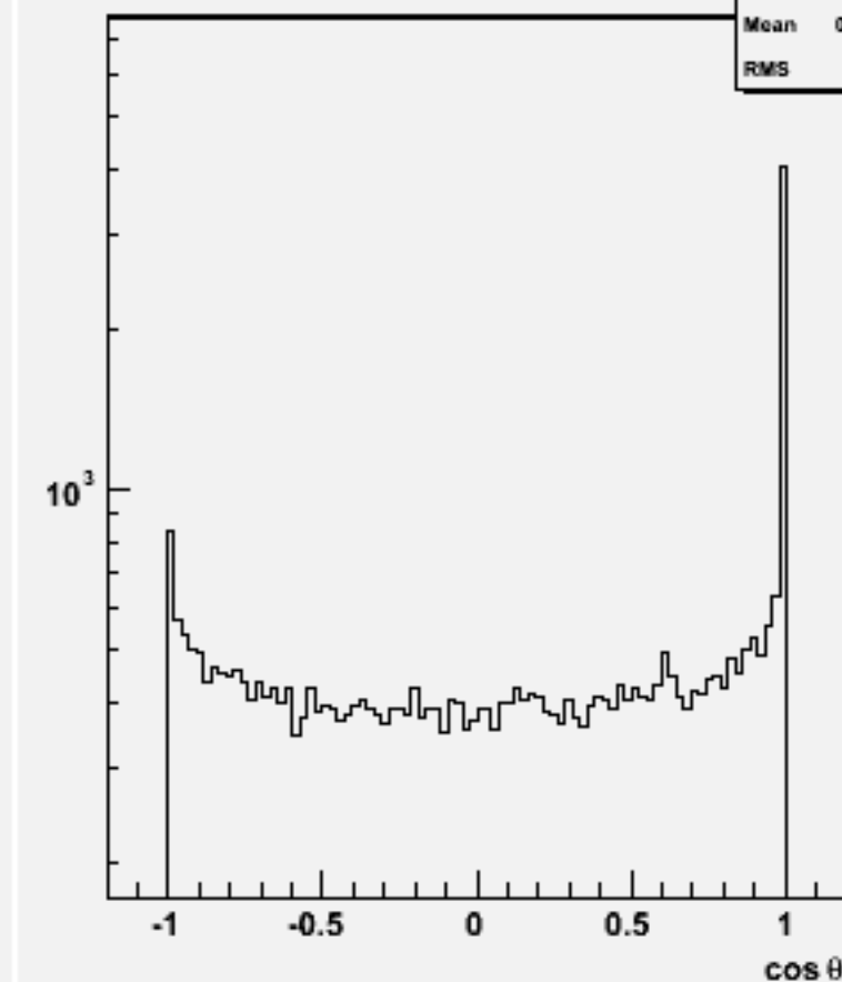
Jet cos \theta (All jets)w101725 ccn2e2e3n3_o
