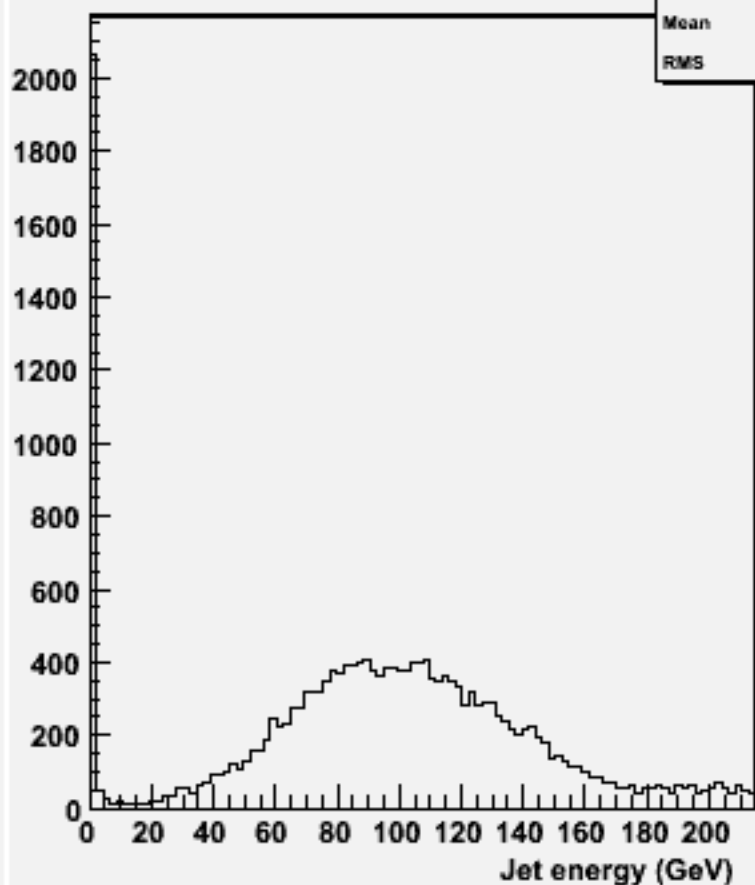
energy for 2-jets :w101725 ccn2e2e3n3_o
