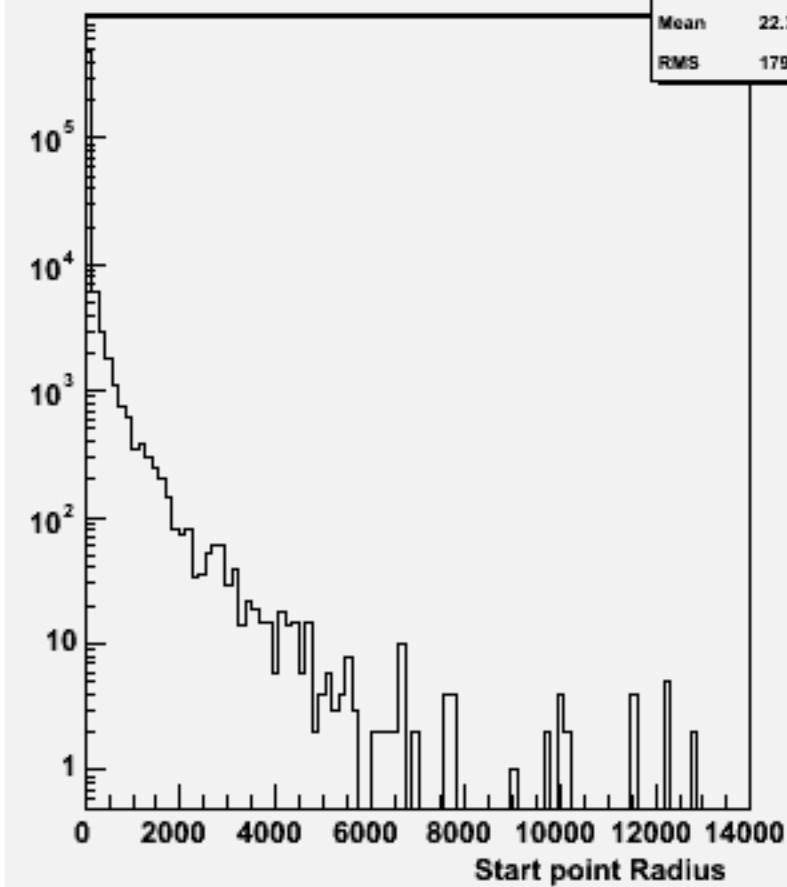
Start point R : w101724 ccn2e2e3n3_o
