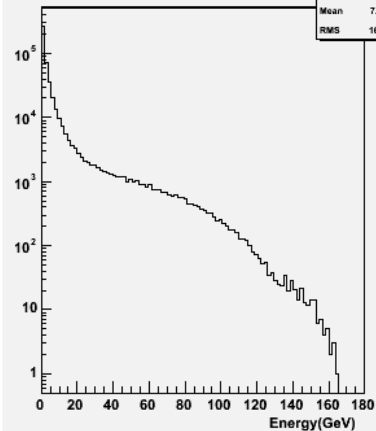
Particle Energy : w101724 ccn2e2e3n3_o
