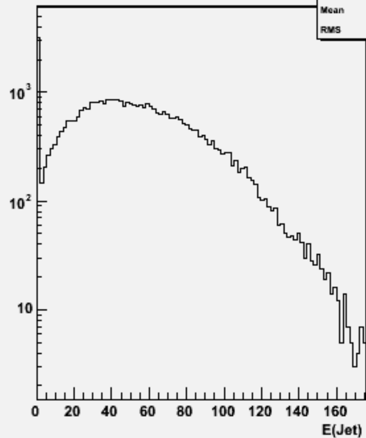
Jet energies(All jets)w101724 ccn2e2e3n3_o
