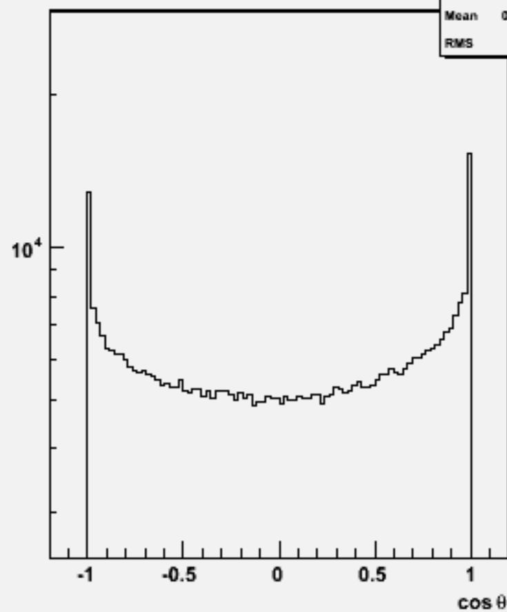
Particle \cos\theta : w101724 ccn2e2e3n3_o
