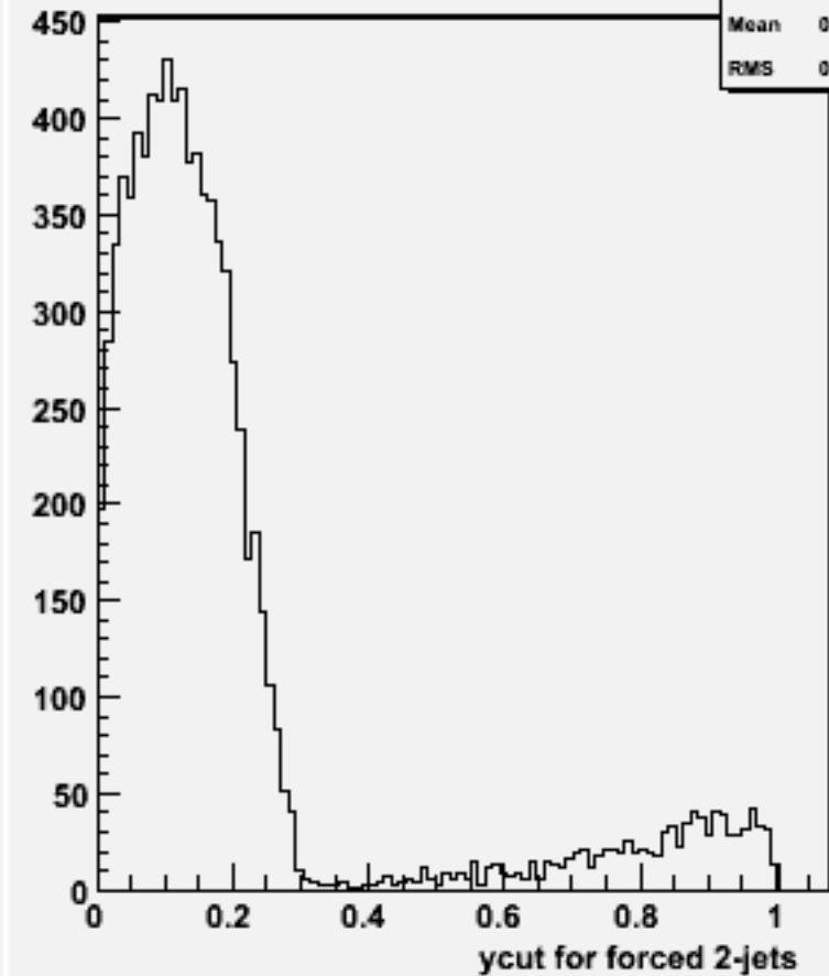
Ycut for 2-jets :w101724 ccn2e2e3n3_o
