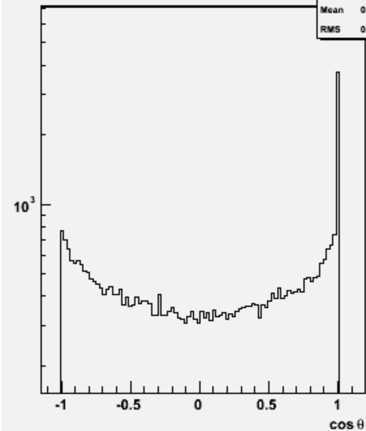
Jet cos \theta (All jets)w101724 ccn2e2e3n3_o
