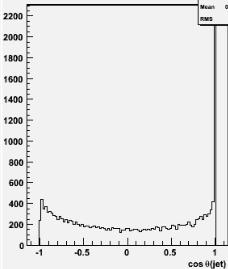
cos \theta for 2-jets :w101724 ccn2e2e3n3_o
