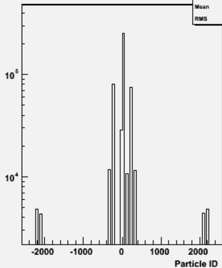
Particle ID : w101724 ccn2e2e3n3_o
