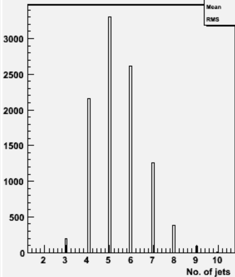
No. jets (ycut=0.001) : w101724 ccn2e2e3n3_o
