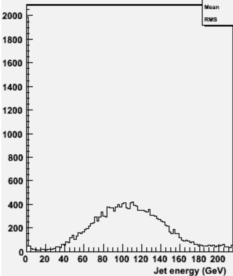
energy for 2-jets :w101724 ccn2e2e3n3_o
