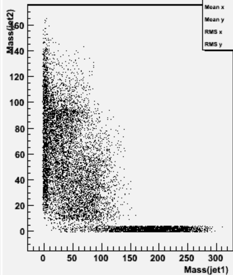
Jet mass for forced 2-jets : w101724 ccn2e2e3n3_o
