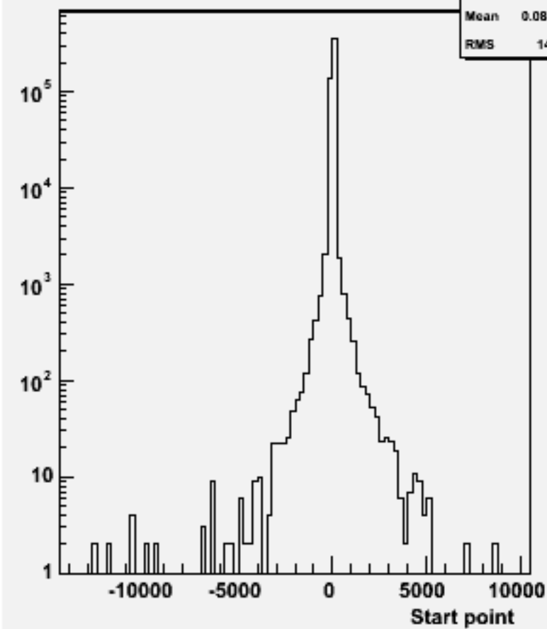
Start point Z : w101724 ccn2e2e3n3_o
