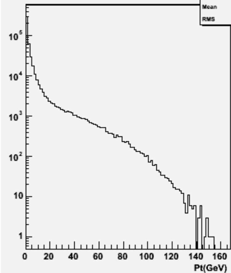
Particle Pt : w101724 ccn2e2e3n3_o
