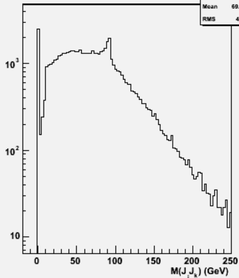
2jets mass(All comb)w101724 ccn2e2e3n3_o
