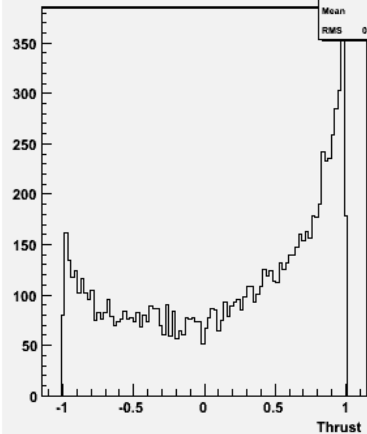
cos \Theta (thrust) w101724 ccn2e2e3n3_o
