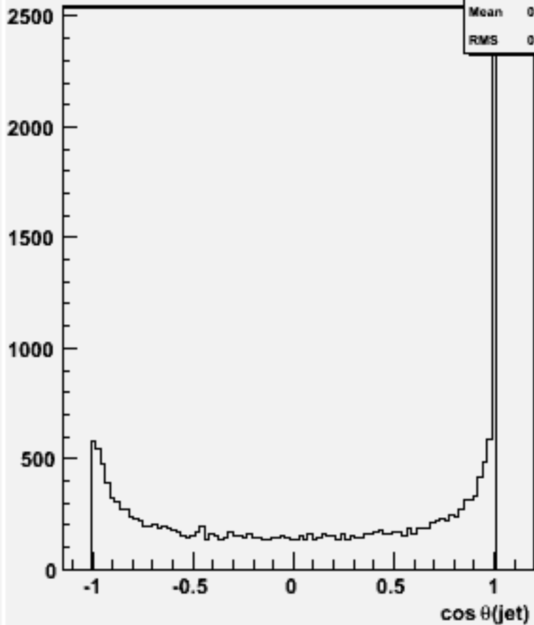
cos \theta for 2-jets :w101721 ccn2e2e2n2_o
