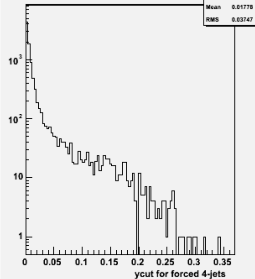
Ycut for 4-jets :w101721 ccn2e2e2n2_o
