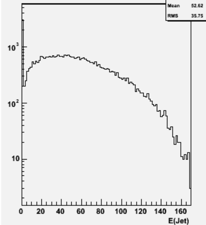
Jet energies(All jets)w101721 ccn2e2e2n2_o
