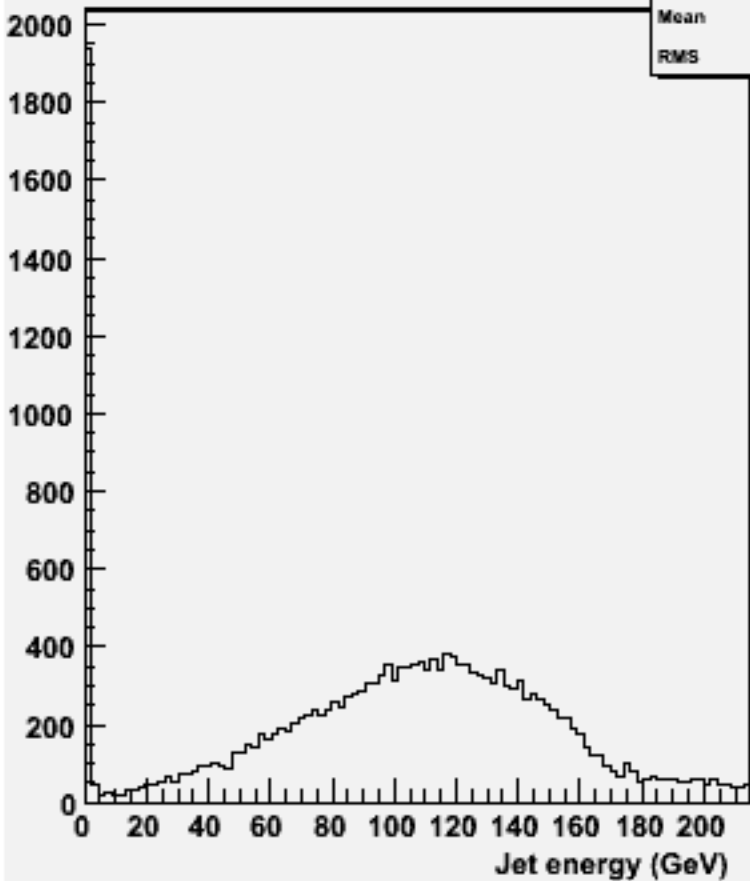
energy for 2-jets :w101721 ccn2e2e2n2_o
