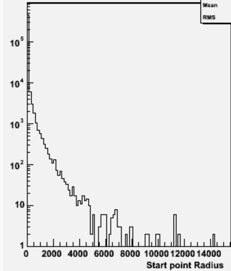
Start point R : w101721 ccn2e2e2n2_o
