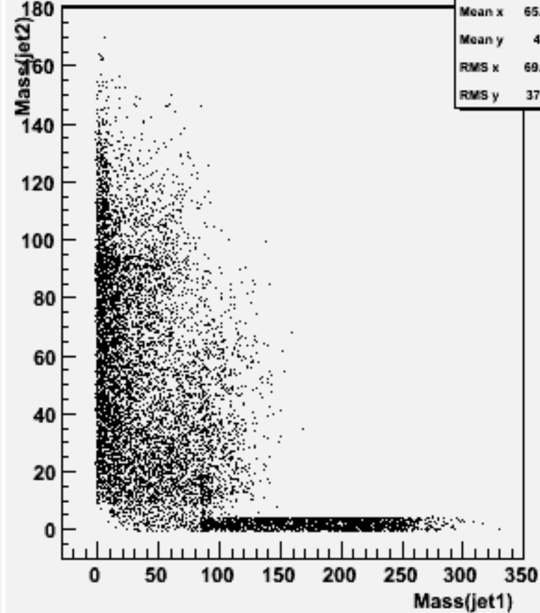
Jet mass for forced 2-jets : w101721 ccn2e2e2n2_o
