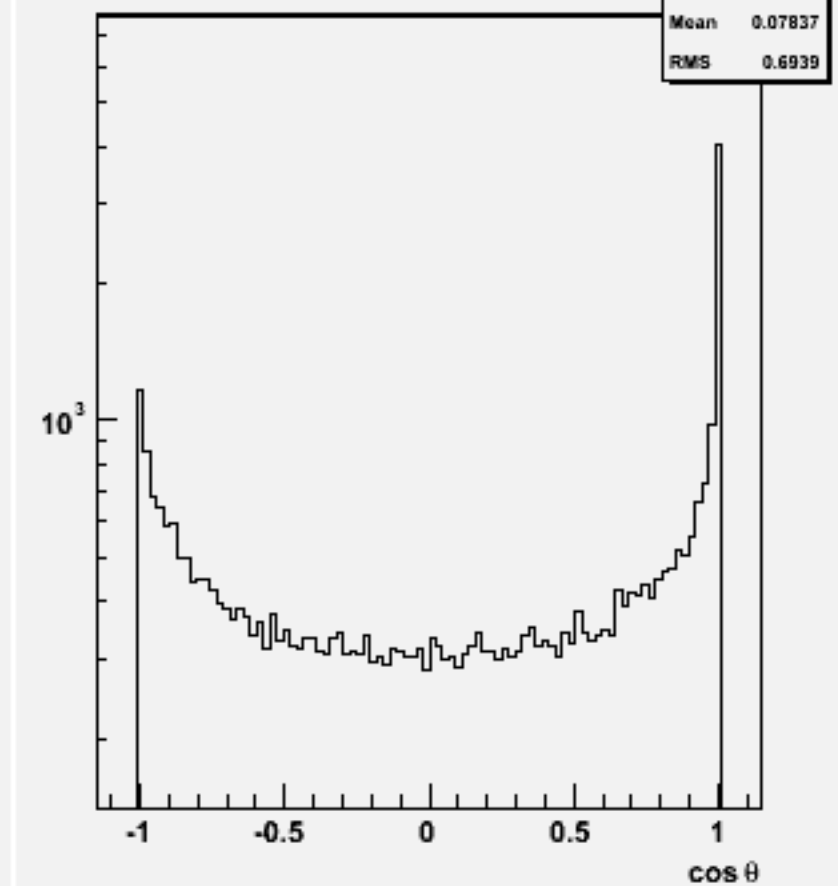
Jet cos \theta (All jets)w101721 ccn2e2e2n2_o
