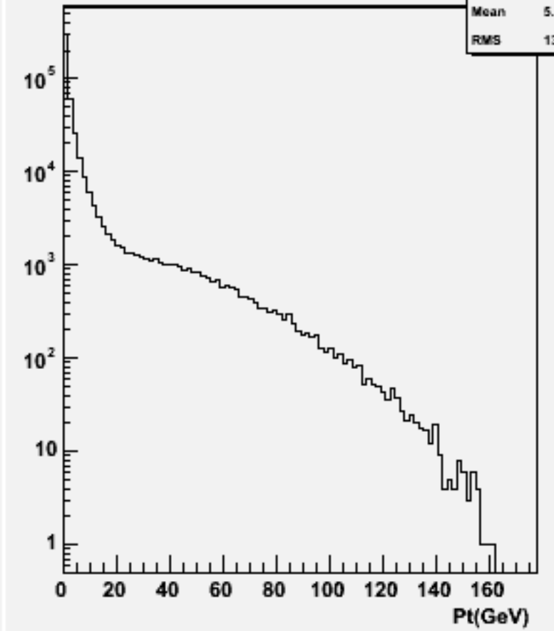
Start point Z : w101721 ccn2e2e2n2_o
