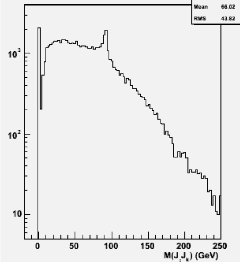
2jets mass(All comb)w101721 ccn2e2e2n2_o
