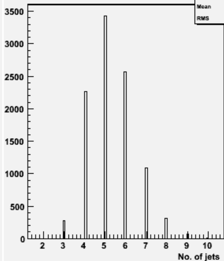
No. jets (ycut=0.001) : w101720 ccn2e2e2n2_o
