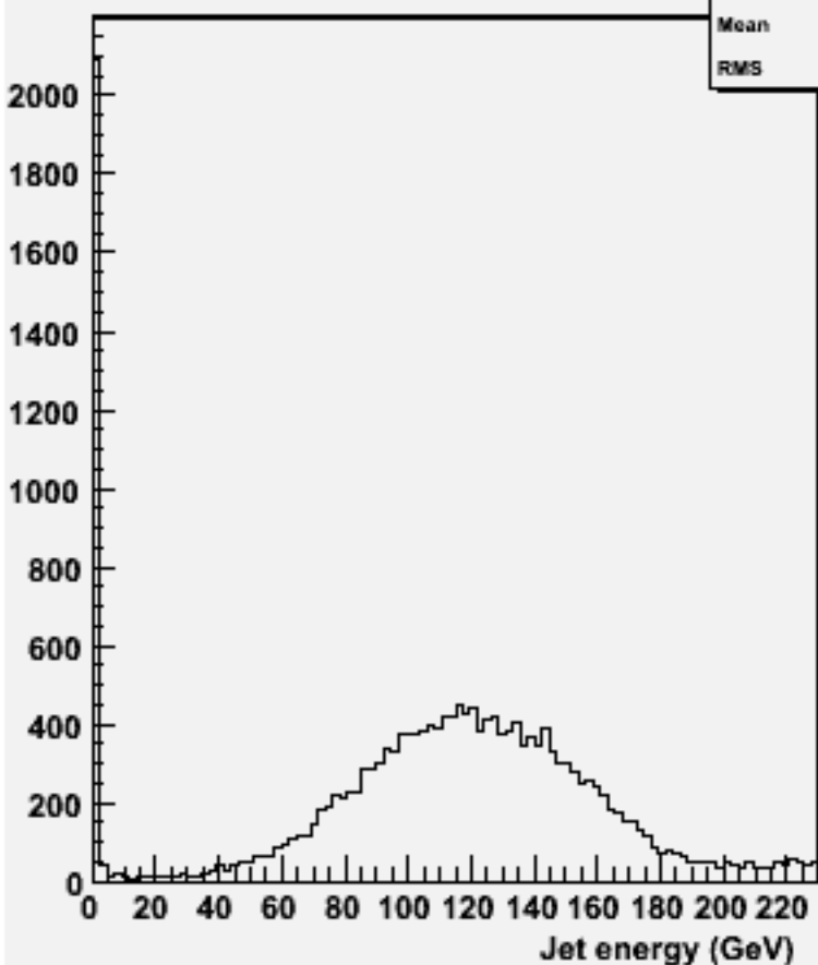
energy for 2-jets :w101720 ccn2e2e2n2_o
