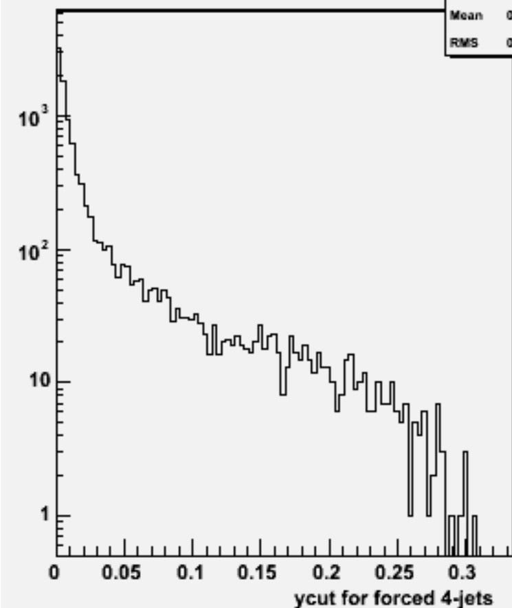
Ycut for 4-jets :w101720 ccn2e2e2n2_o
