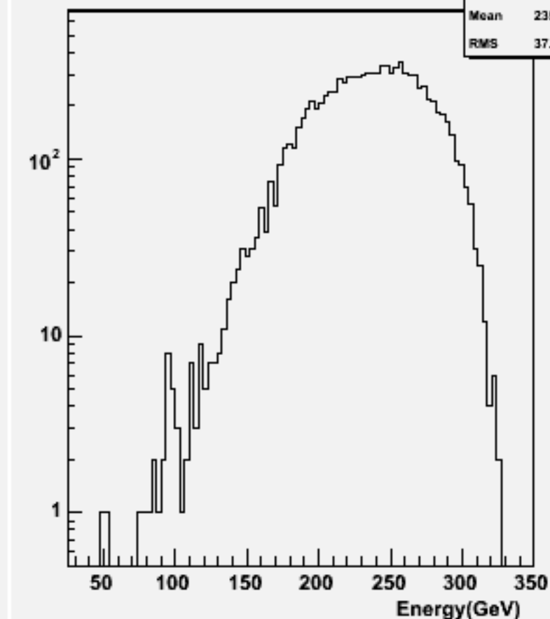
Thrust w101720 ccn2e2e2n2_o
