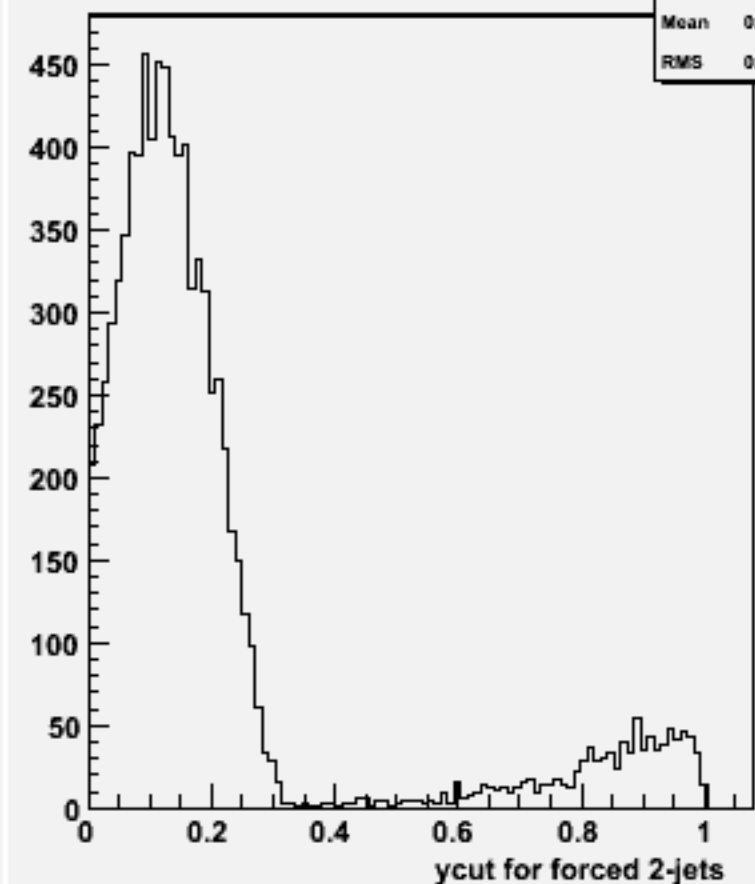
Ycut for 2-jets :w101720 ccn2e2e2n2_o
