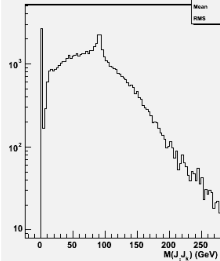
2jets mass(All comb)w101720 ccn2e2e2n2_o
