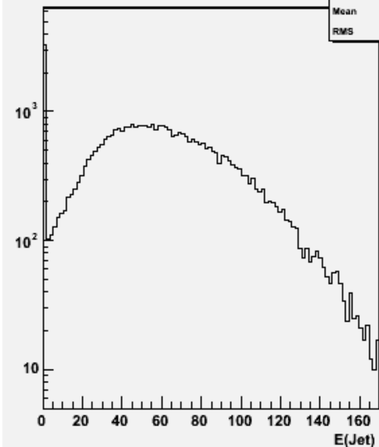
Jet energies(All jets)w101720 ccn2e2e2n2_o
