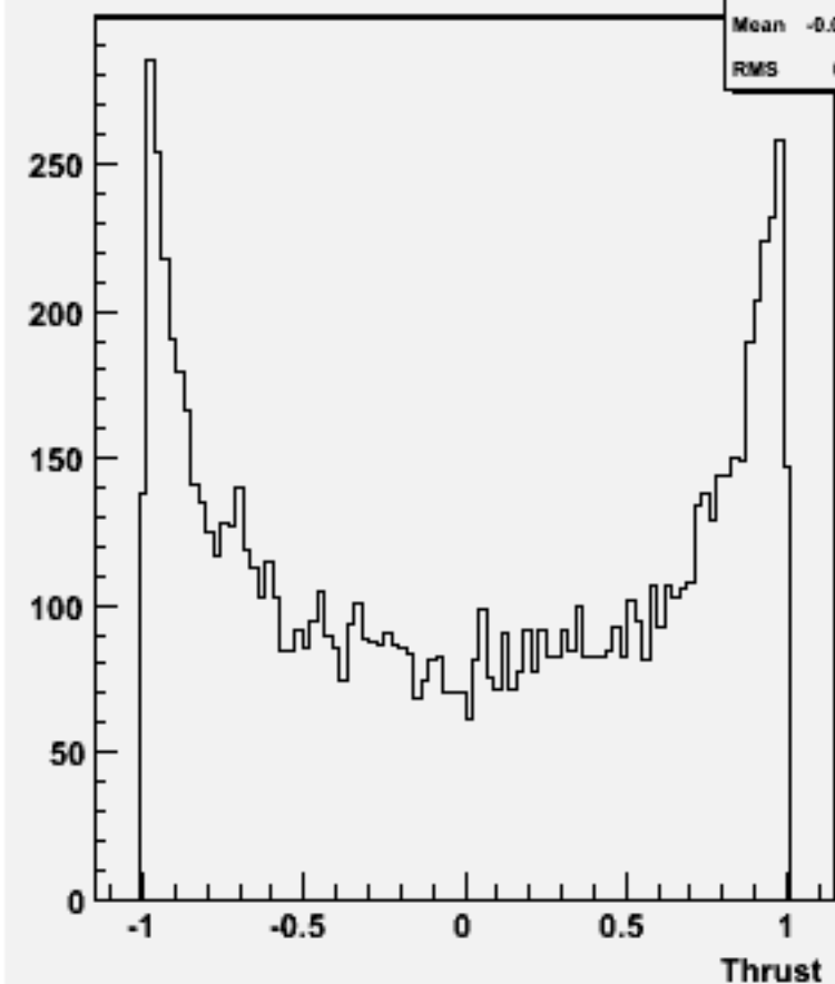
cos \Theta (thrust) w101720 ccn2e2e2n2_o
