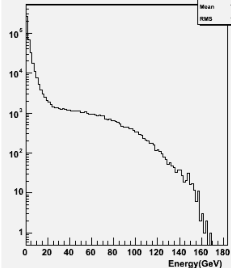
Particle Energy : w101720 ccn2e2e2n2_o
