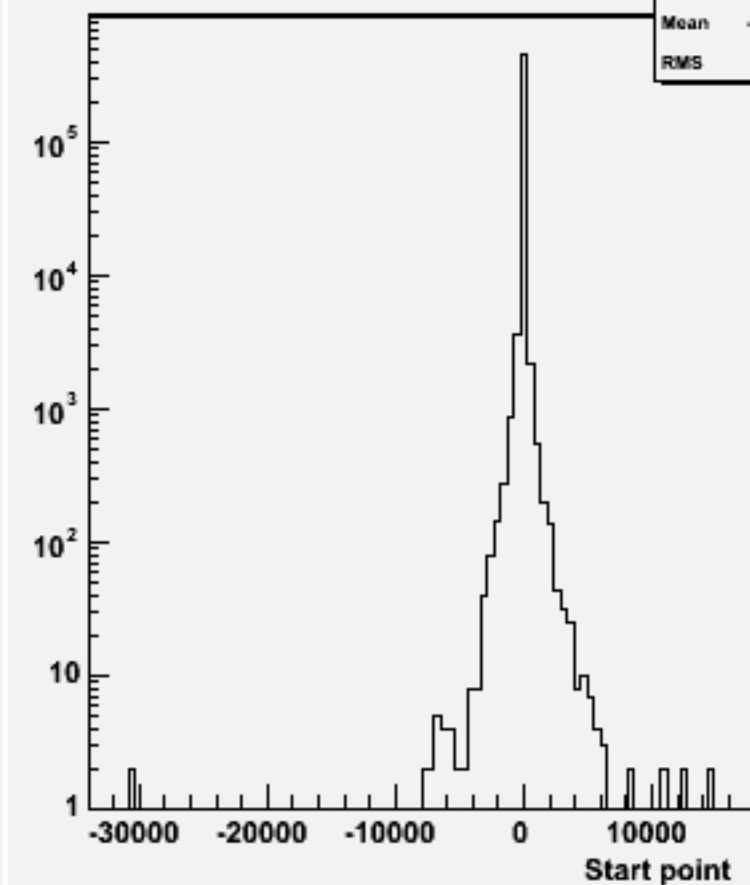
Start point Z : w101720 ccn2e2e2n2_o
