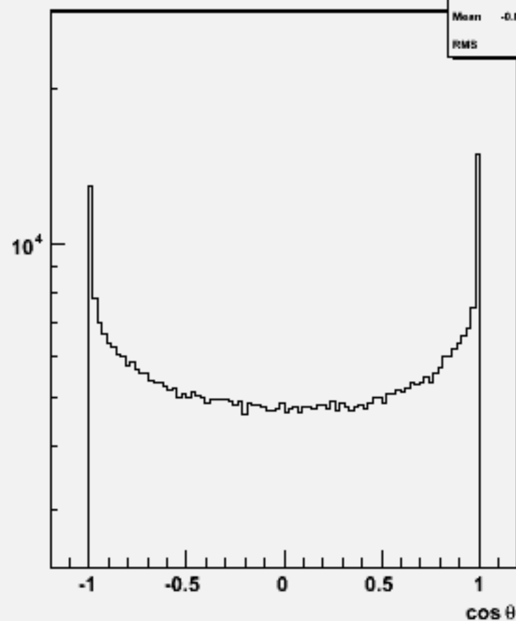
Particle cos θ : w101720 ccn2e2e2n2_o
