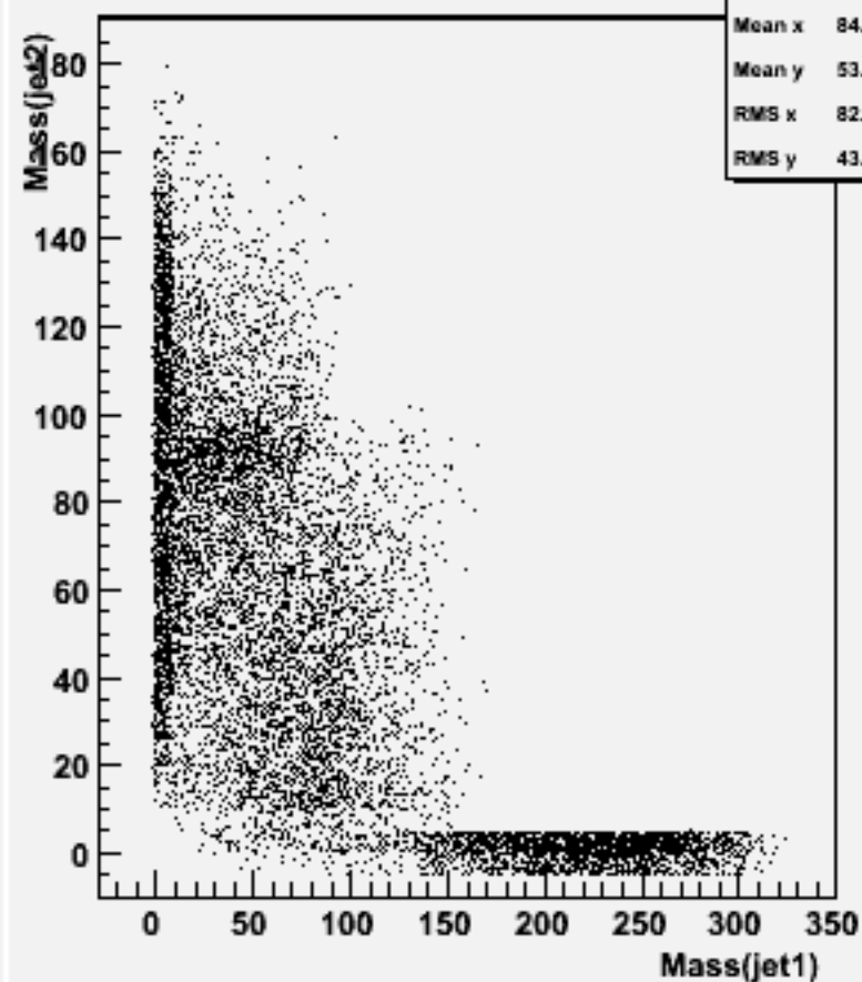
Jet mass for forced 2-jets : w101720 ccn2e2e2n2_o
