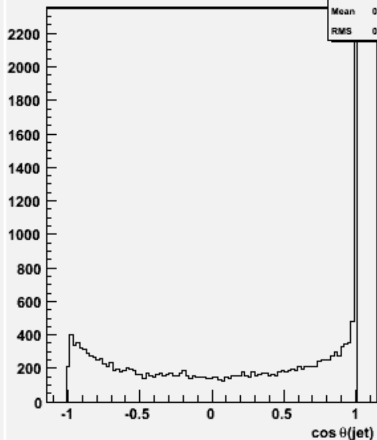
cos \theta for 2-jets :w101720 ccn2e2e2n2_o
