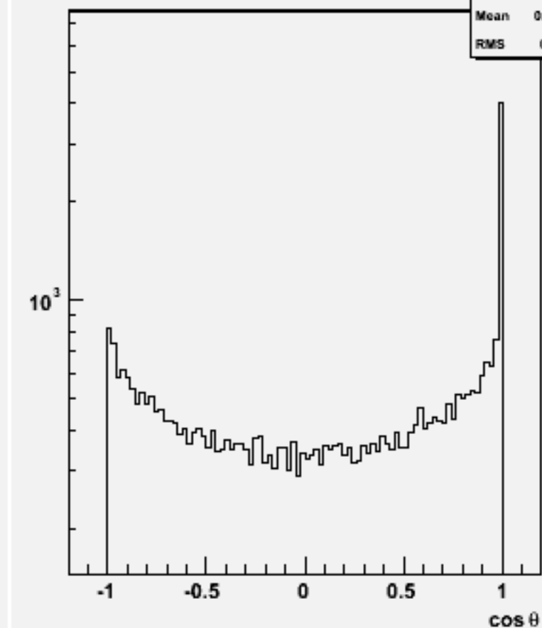
Jet cos \theta (All jets)w101720 ccn2e2e2n2_o
