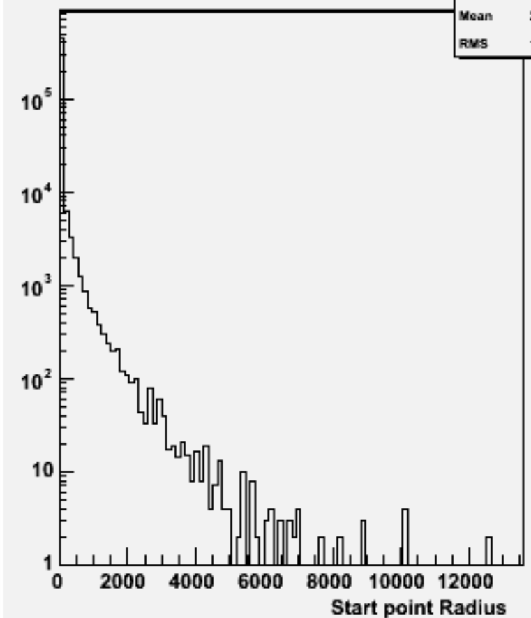
Start point R : w101720 ccn2e2e2n2_o
