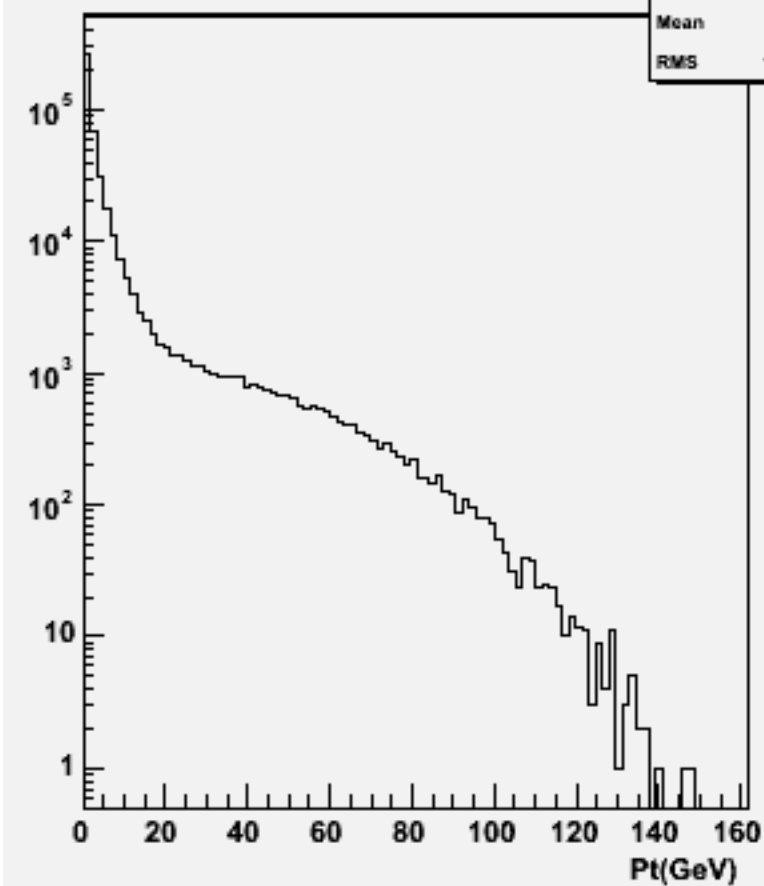
Particle Pt : w101718 ccn2e2e1n1_o
