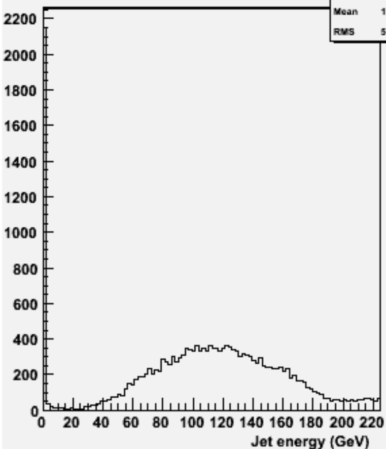
energy for 2-jets :w101718 ccn2e2e1n1_o
