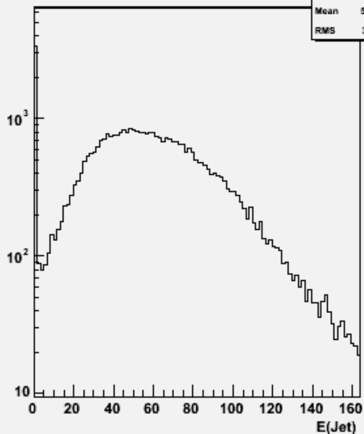
Jet energies(All jets)w101718 ccn2e2e1n1_o
