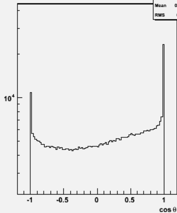
Particle \cos\theta : w101718 ccn2e2e1n1_o
