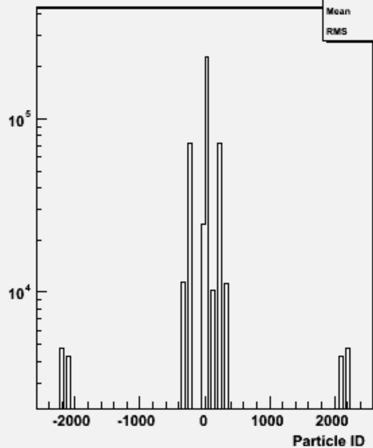
Particle ID : w101718 ccn2e2e1n1_o
