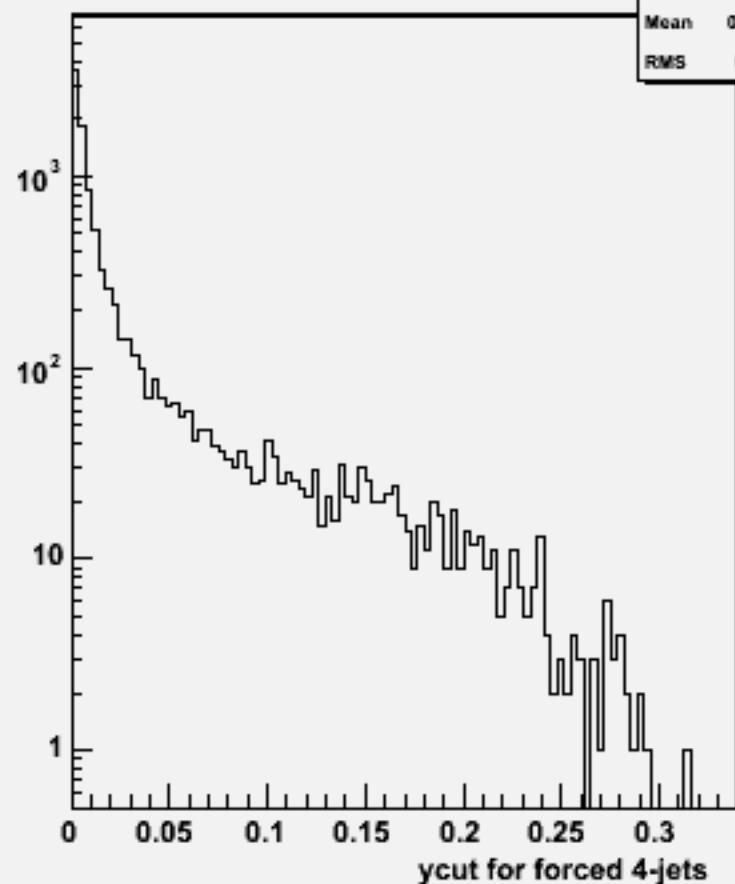
Ycut for 4-jets :w101718 ccn2e2e1n1_o
