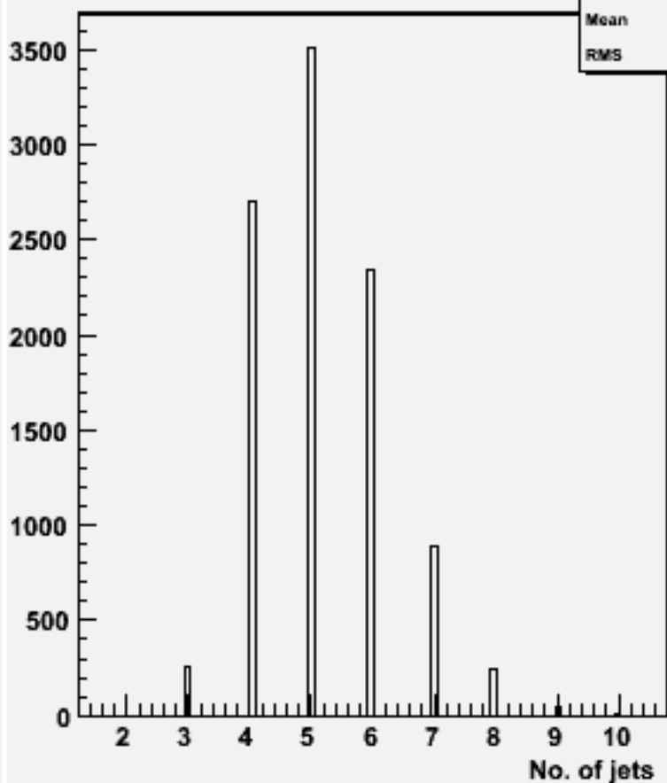
No. jets (ycut=0.001) : w101718 ccn2e2e1n1_o
