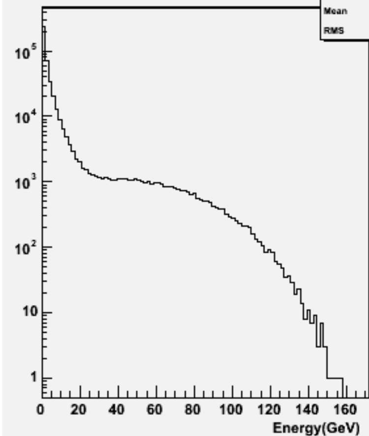
Particle Energy : w101718 ccn2e2e1n1_o
