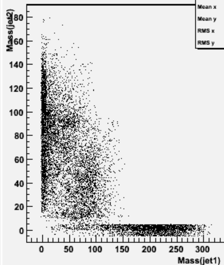
Jet mass for forced 2-jets : w101718 ccn2e2e1n1_o
