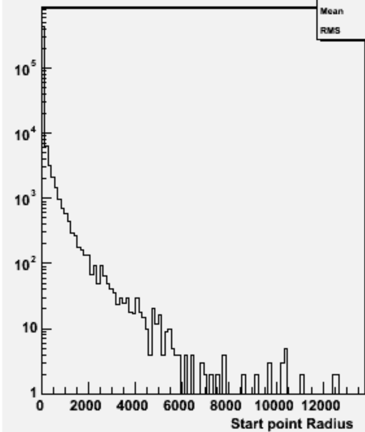
Start point R : w101718 ccn2e2e1n1_o
