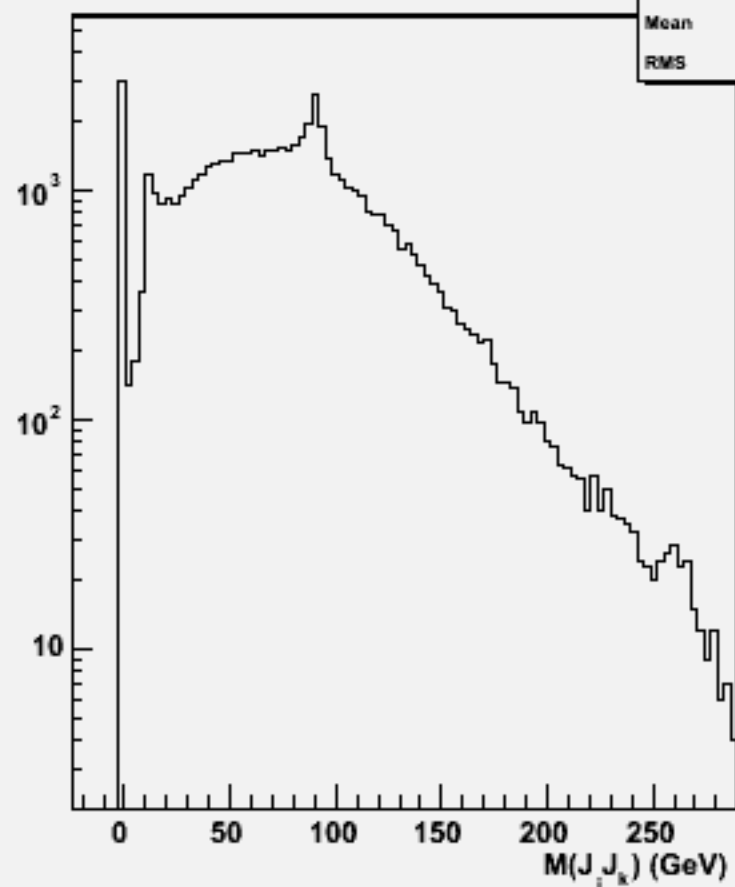
2jets mass(All comb)w101718 ccn2e2e1n1_o
