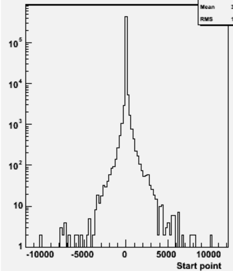
Start point Z : w101718 ccn2e2e1n1_o
