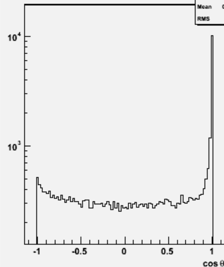
Jet cos \theta (All jets)w101718 ccn2e2e1n1_o
