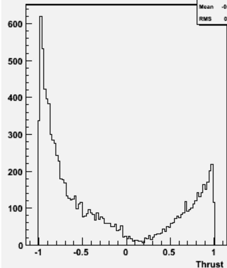
cos \Theta (thrust) w101718 ccn2e2e1n1_o
