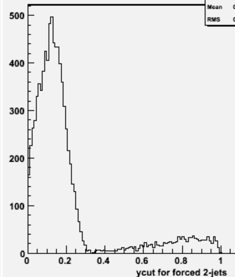
Ycut for 2-jets :w101718 ccn2e2e1n1_o
