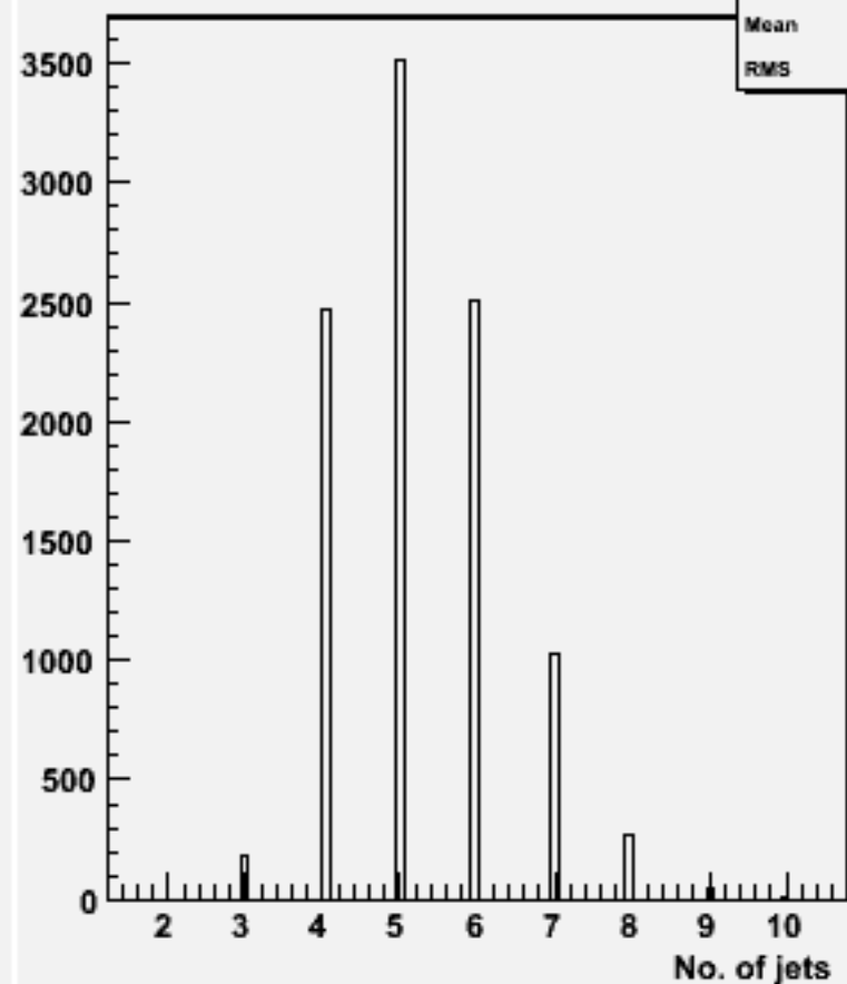
No. jets (ycut=0.001) : w101717 ccn2e2e1n1_o
