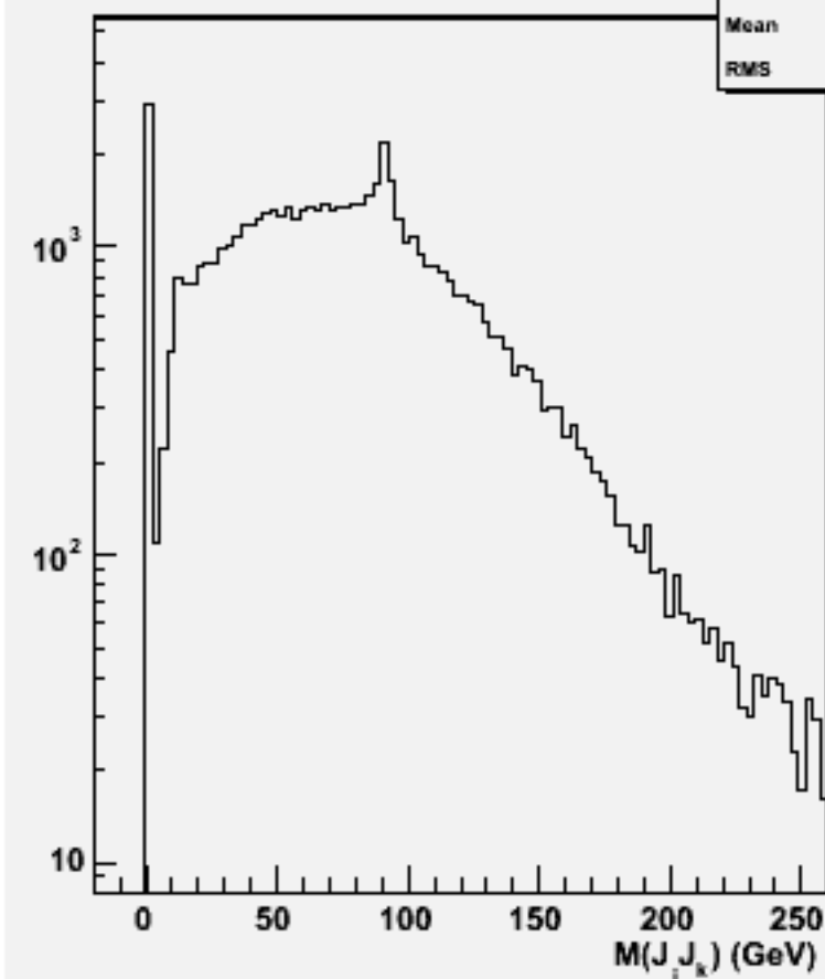
2jets mass(All comb)w101717 ccn2e2e1n1_o
