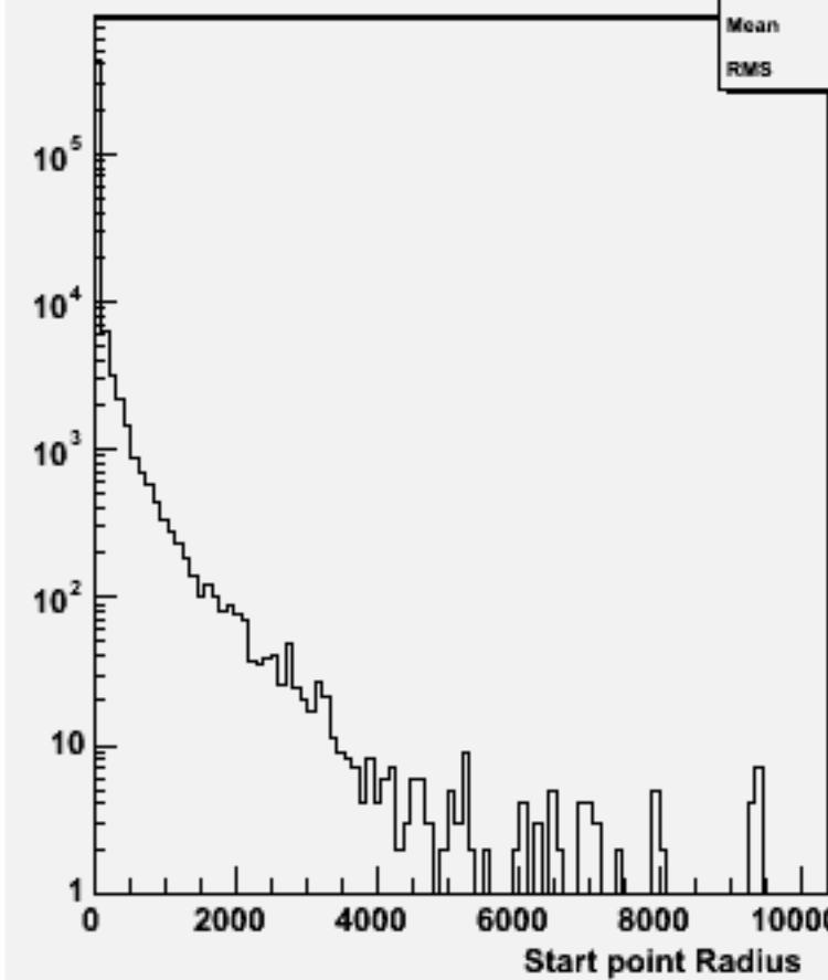
Start point R : w101717 ccn2e2e1n1_o
