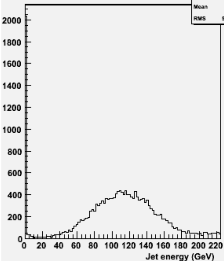
energy for 2-jets :w101717 ccn2e2e1n1_o
