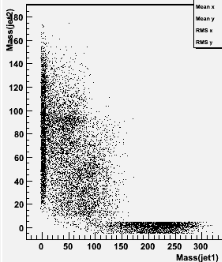
Jet mass for forced 2-jets : w101717 ccn2e2e1n1_o
