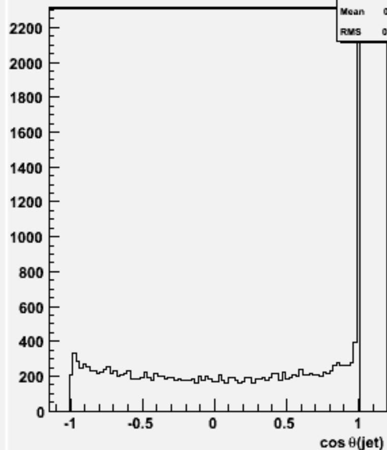
cos \theta for 2-jets :w101717 ccn2e2e1n1_o
