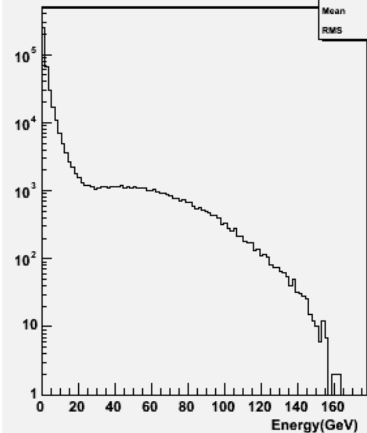
Particle Energy : w101717 ccn2e2e1n1_o
