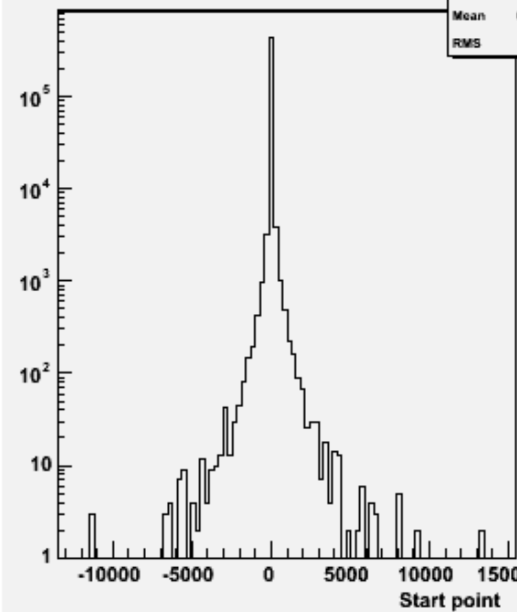
Start point Z : w101717 ccn2e2e1n1_o
