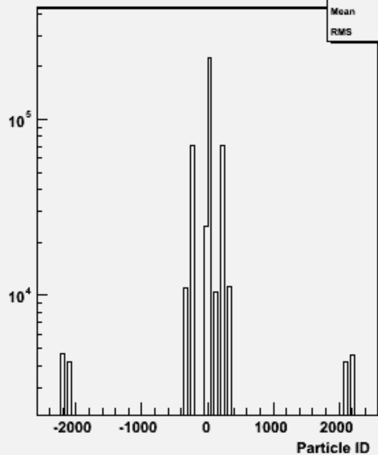
Particle ID : w101717 ccn2e2e1n1_o
