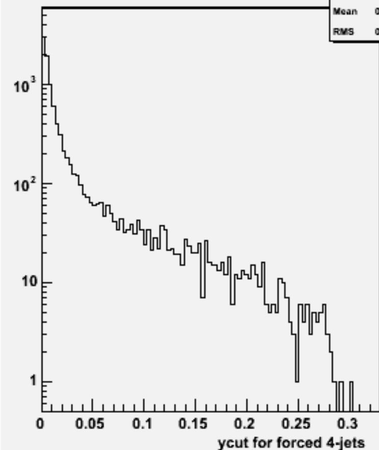
Ycut for 4-jets :w101717 ccn2e2e1n1_o
