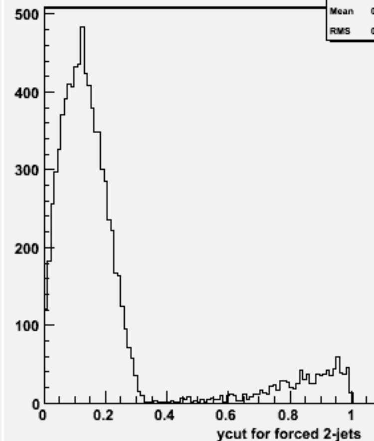
Ycut for 2-jets :w101717 ccn2e2e1n1_o
