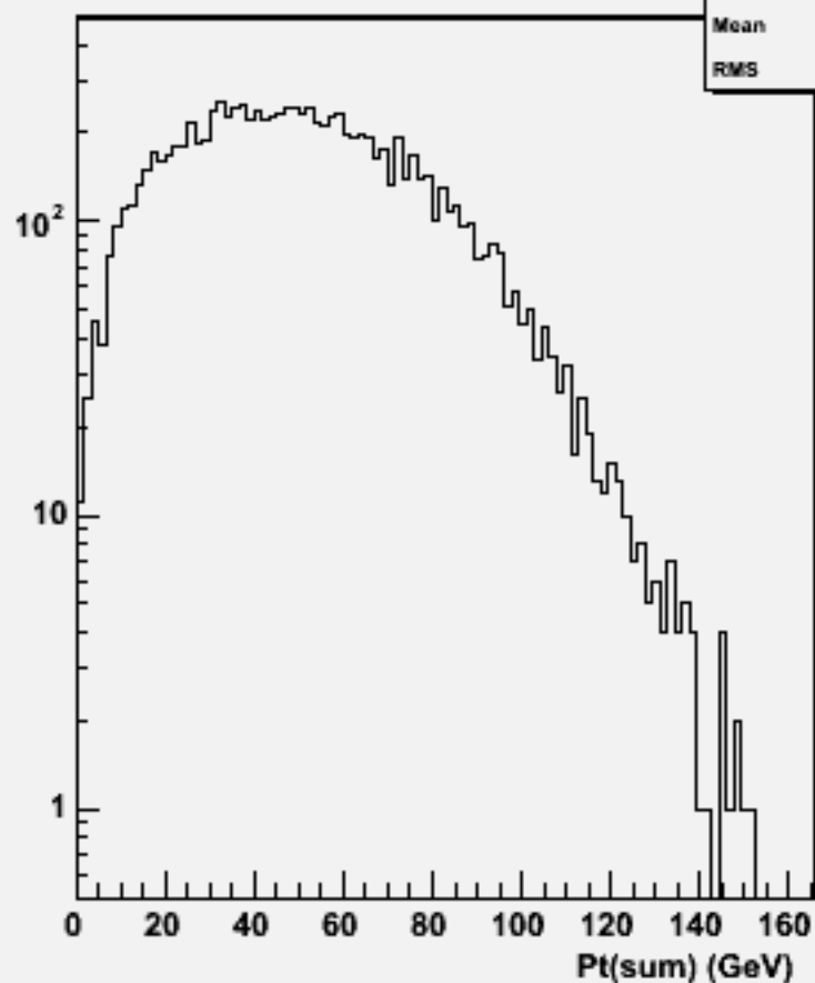
Pt Sum: w101717 ccn2e2e1n1_o
