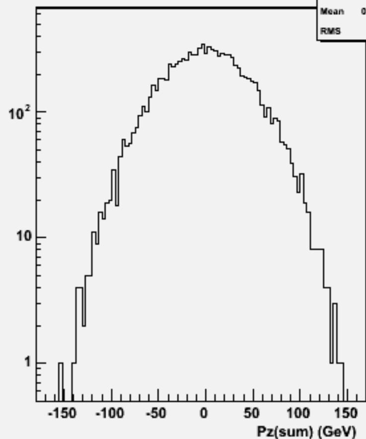
Pz Sum: w101717 ccn2e2e1n1_o
