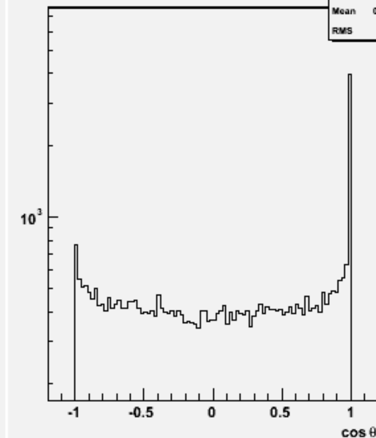
Jet cos \theta (All jets)w101717 ccn2e2e1n1_o
