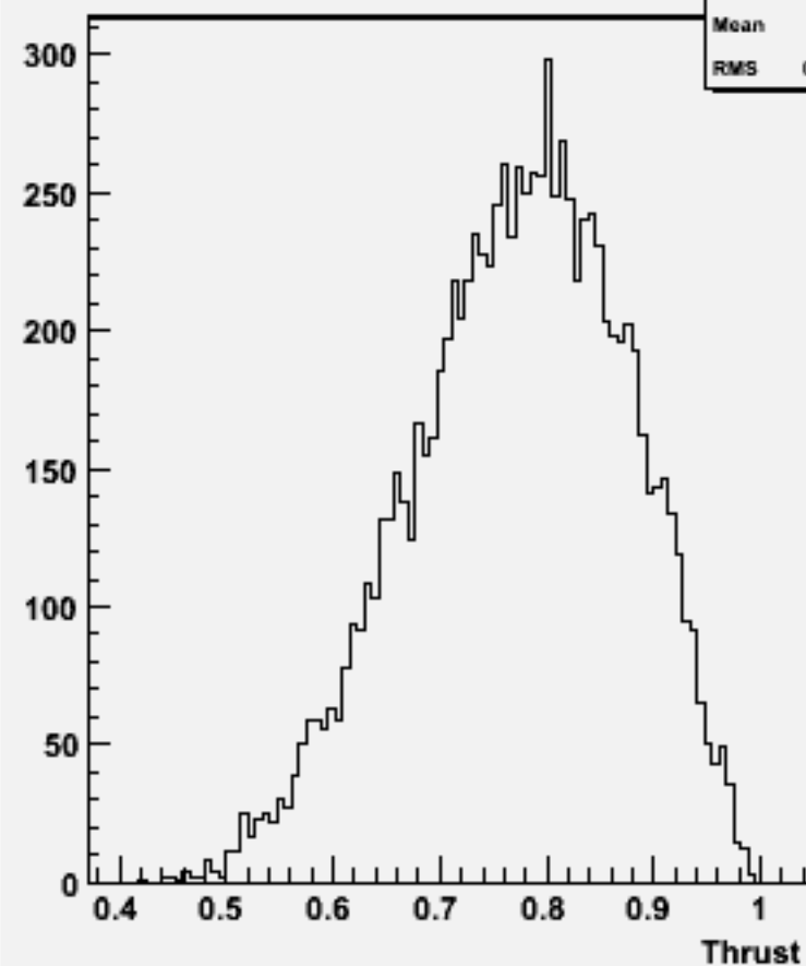
Thrust w101717 ccn2e2e1n1_o
