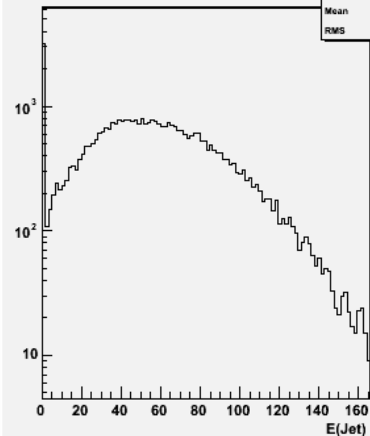
Jet energies(All jets)w101717 ccn2e2e1n1_o
