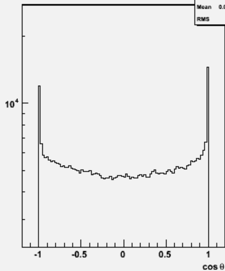
Particle cosθ : w101717 ccn2e2e1n1_o
