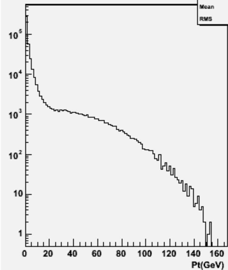
Particle Pt : w101717 ccn2e2e1n1_o
