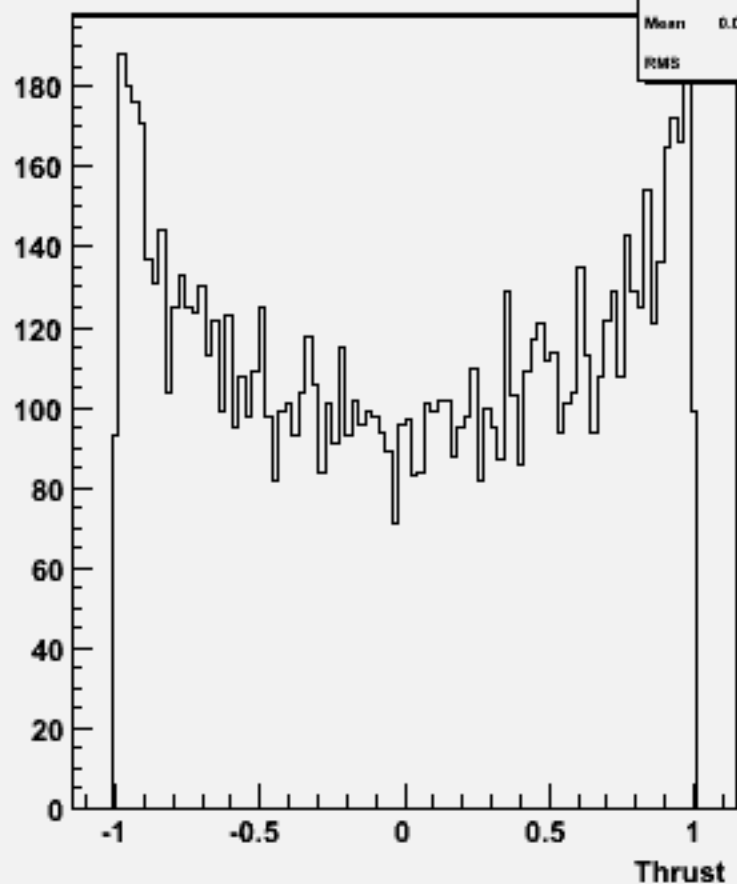
cos \Theta (thrust) w101717 ccn2e2e1n1_o
