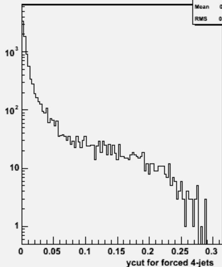
Ycut for 4-jets :w101716 ccn2e2e1n1_o
