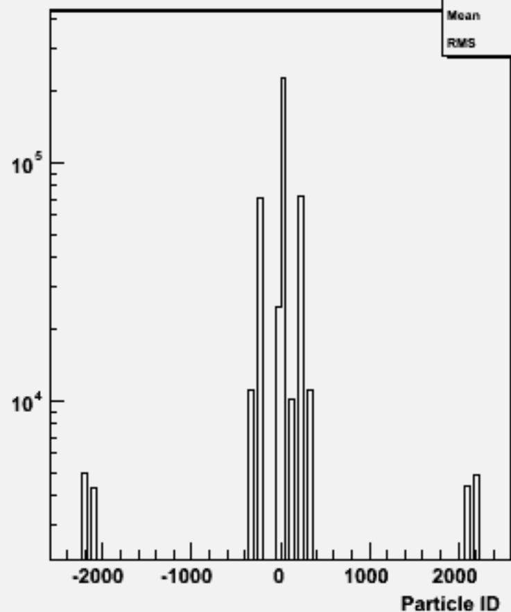
Particle ID : w101716 ccn2e2e1n1_o
