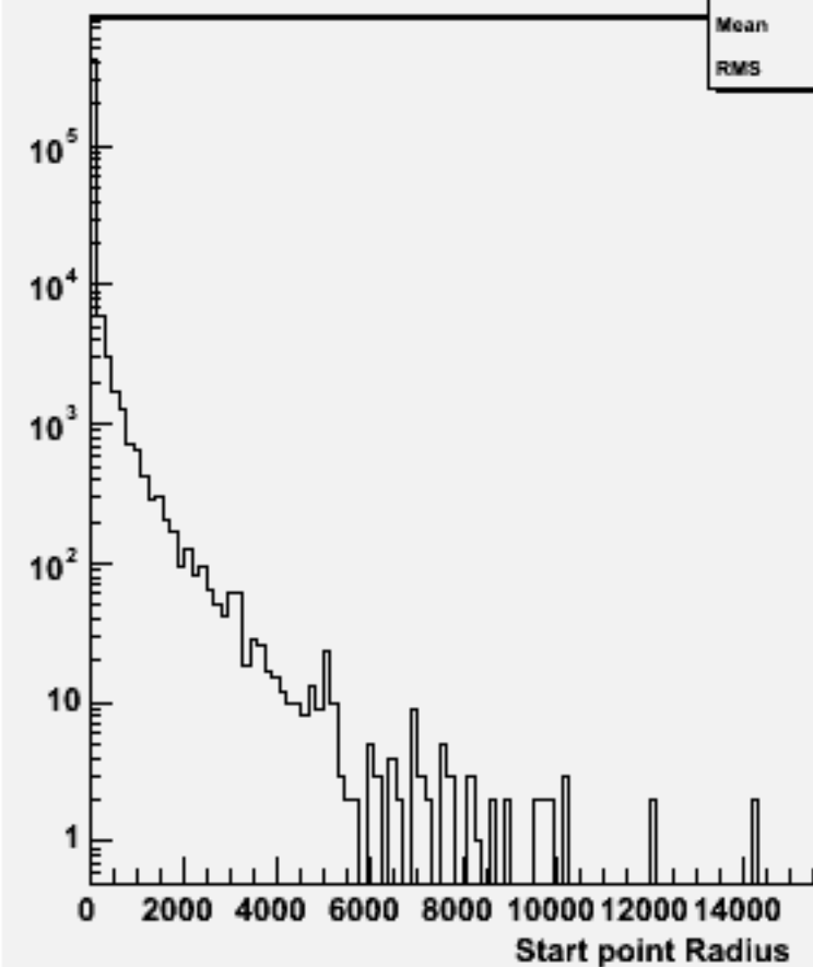
Start point R : w101716 ccn2e2e1n1_o
