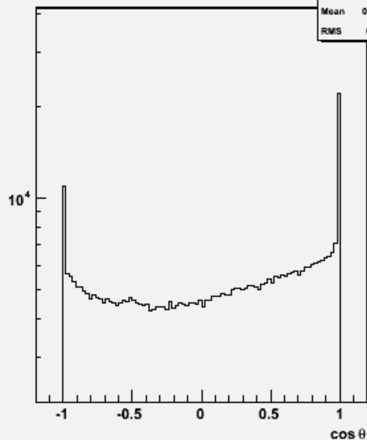
Particle cos θ : w101716 ccn2e2e1n1_o
