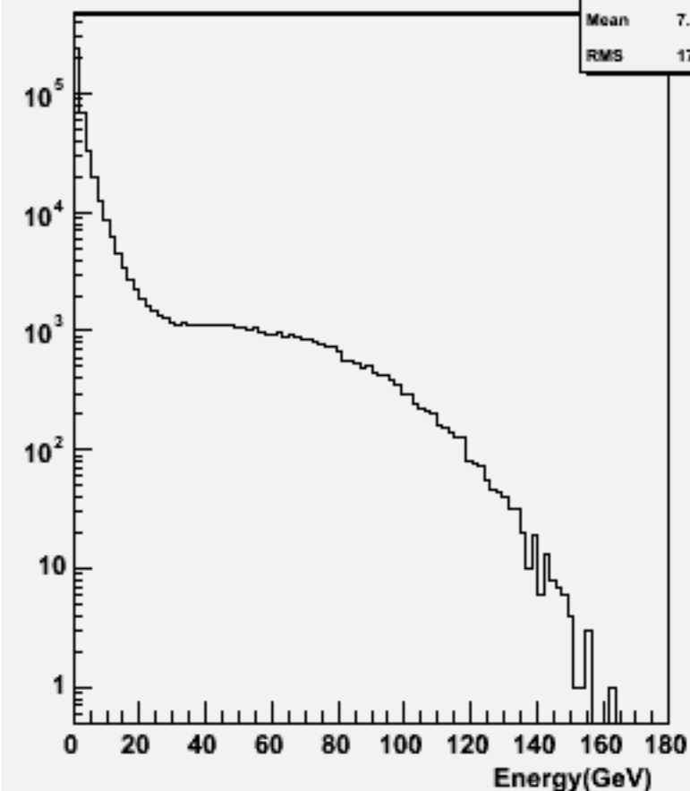
Particle Energy : w101716 ccn2e2e1n1_o
