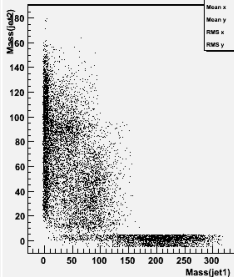
Jet mass for forced 2-jets : w101716 ccn2e2e1n1_o
