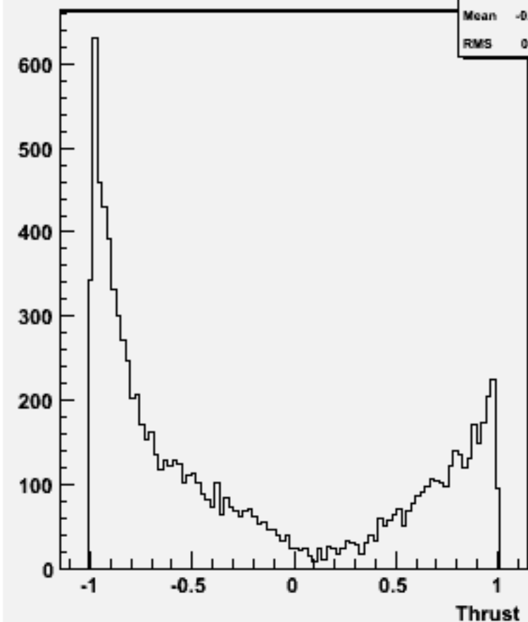
cos \Theta (thrust) w101716 ccn2e2e1n1_o
