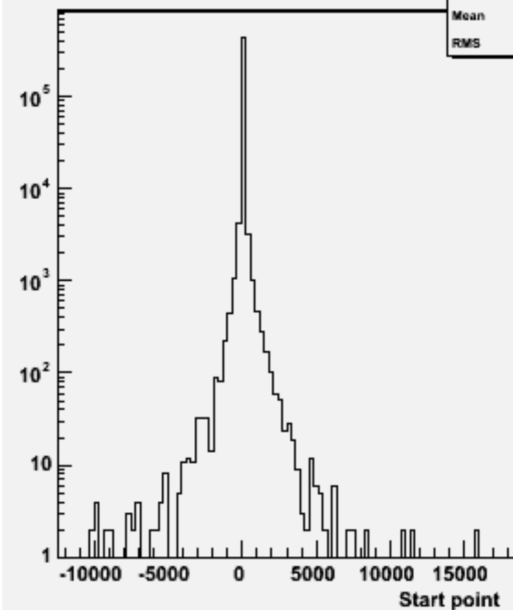
Start point Z : w101716 ccn2e2e1n1_o
