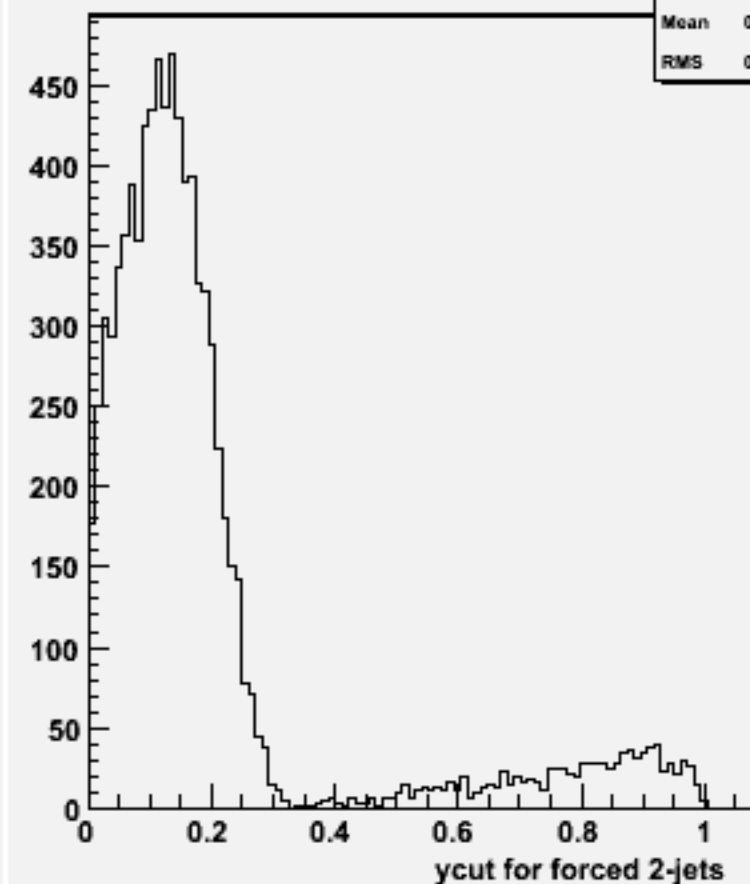
Ycut for 2-jets :w101716 ccn2e2e1n1_o
