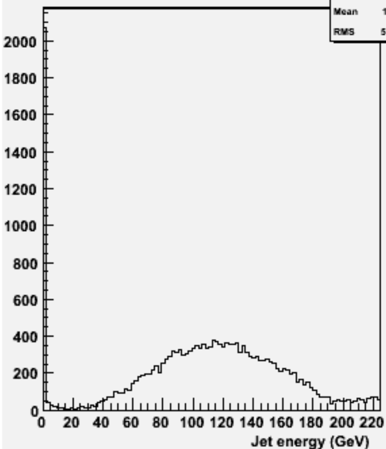
energy for 2-jets :w101716 ccn2e2e1n1_o
