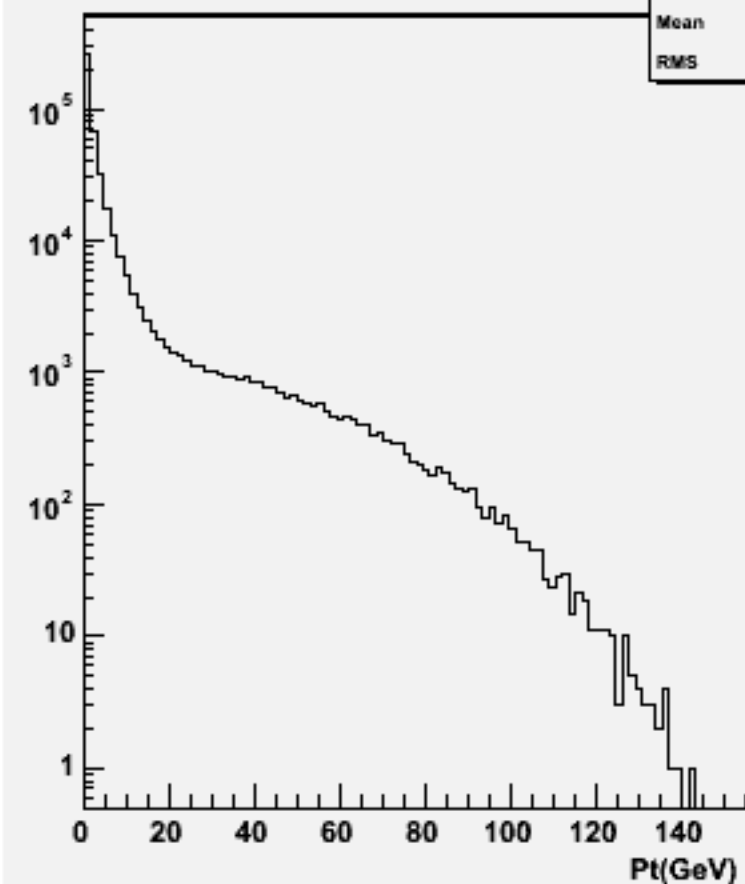
Particle Pt : w101716 ccn2e2e1n1_o
