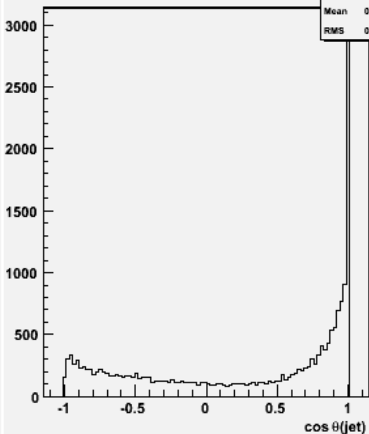
cos \theta for 2-jets :w101716 ccn2e2e1n1_o
