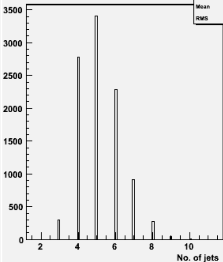
No. jets (ycut=0.001) : w101716 ccn2e2e1n1_o
