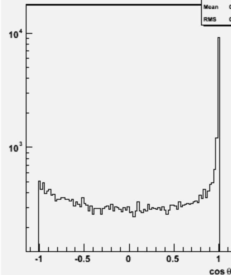
Jet cos \theta (All jets)w101716 ccn2e2e1n1_o
