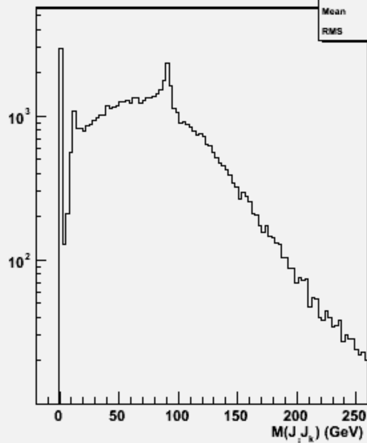
2jets mass(All comb)w101716 ccn2e2e1n1_o
