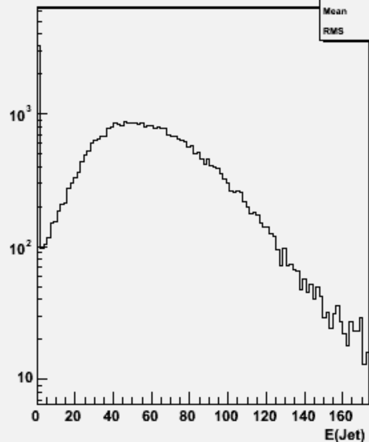
Jet energies(All jets)w101716 ccn2e2e1n1_o
