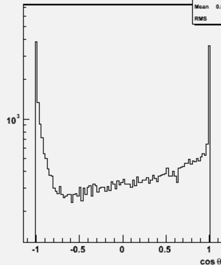
Jet cosθ (All jets)w101712 ccn1e1sc_o
