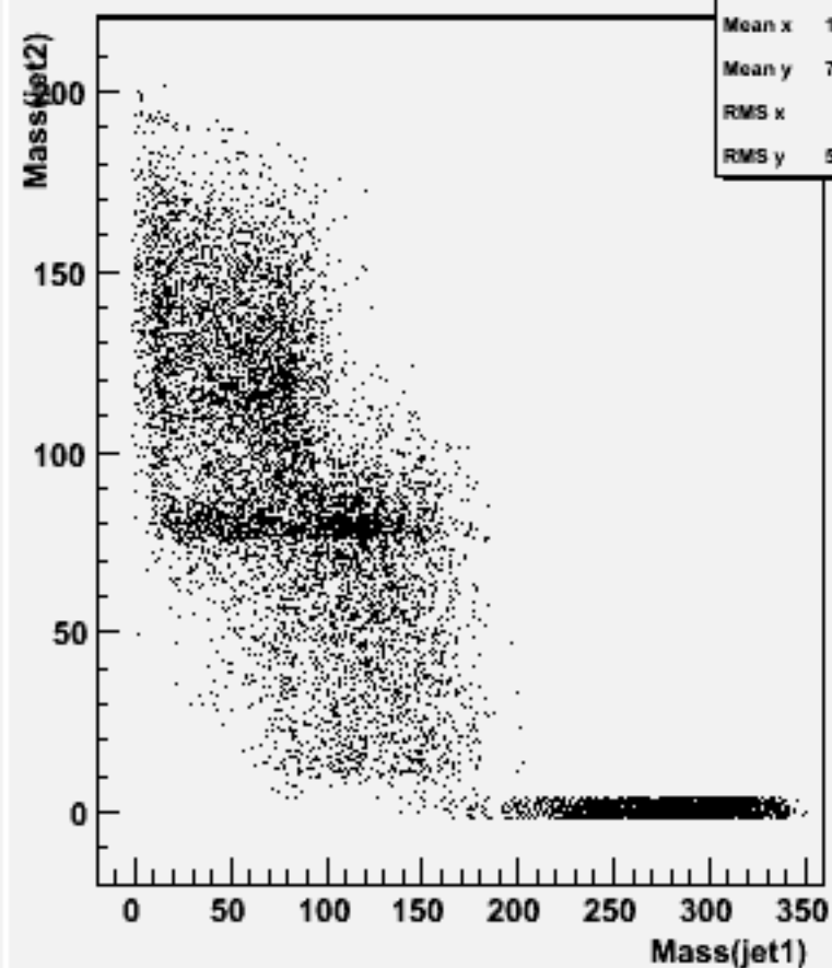
Jet mass for forced 2-jets : w101712 ccn1e1sc_o
