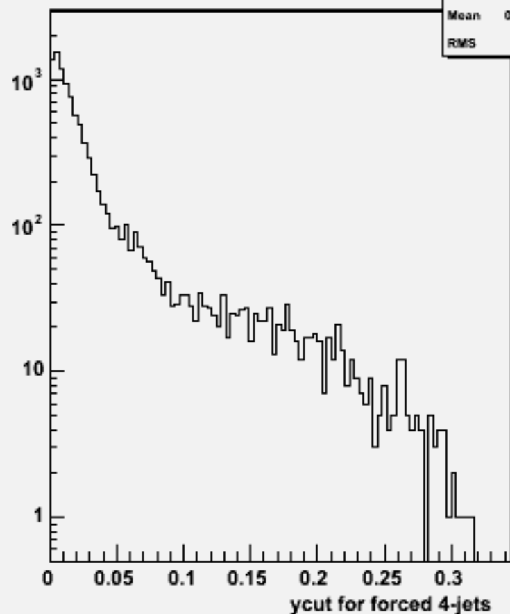
Ycut for 4-jets :w101712 ccn1e1sc_o
