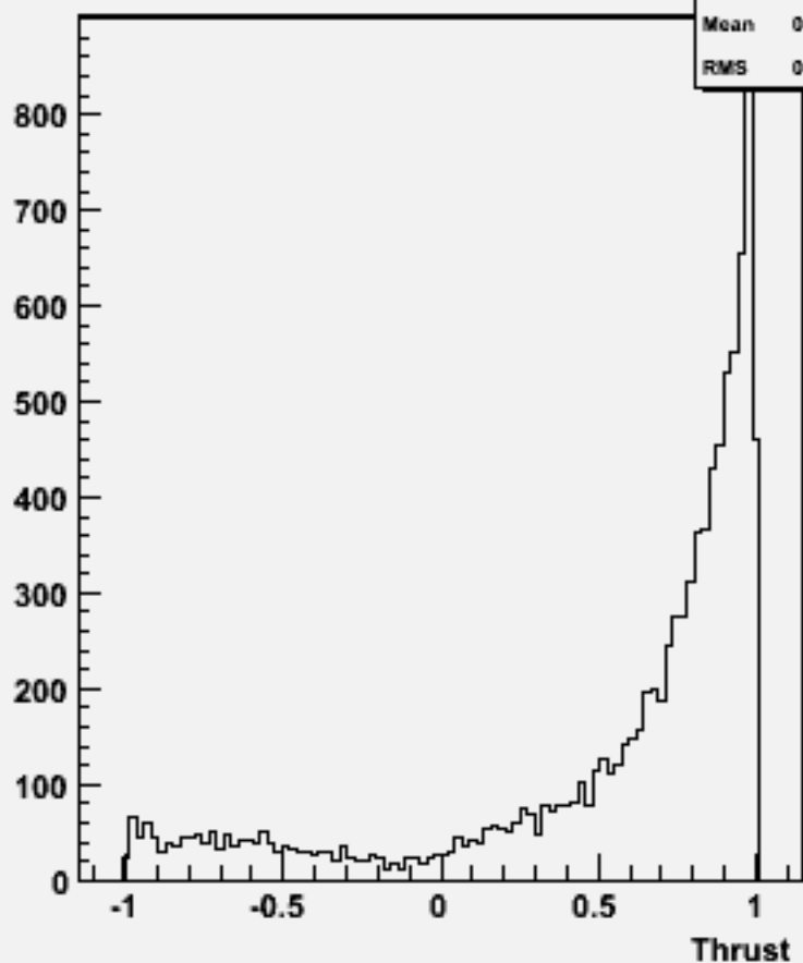
cos \Theta (thrust) w101712 ccn1e1sc_o
