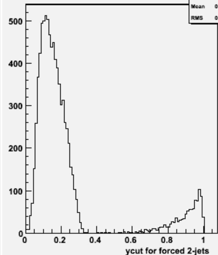
Ycut for 2-jets :w101712 ccn1e1sc_o
