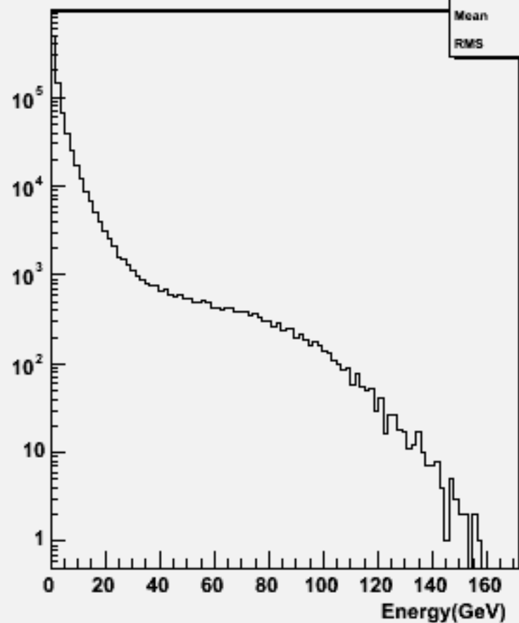
Particle Energy : w101712 ccn1e1sc_o
