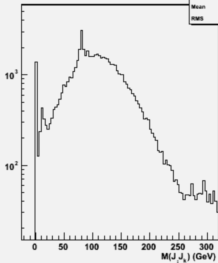
2jets mass(All comb)w101712 ccn1e1sc_o
