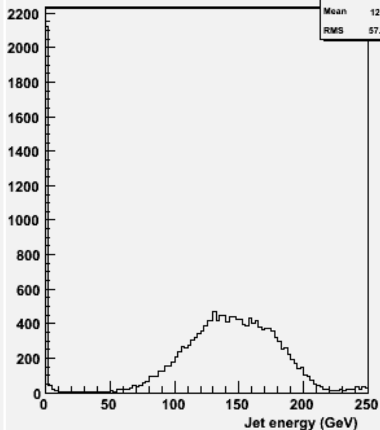
energy for 2-jets :w101712 ccn1e1sc_o
