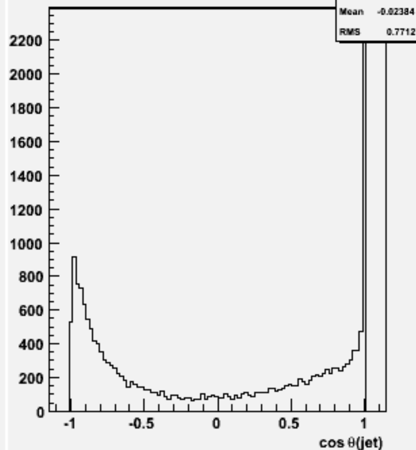
cos \theta for 2-jets :w101712 ccn1e1sc_o
