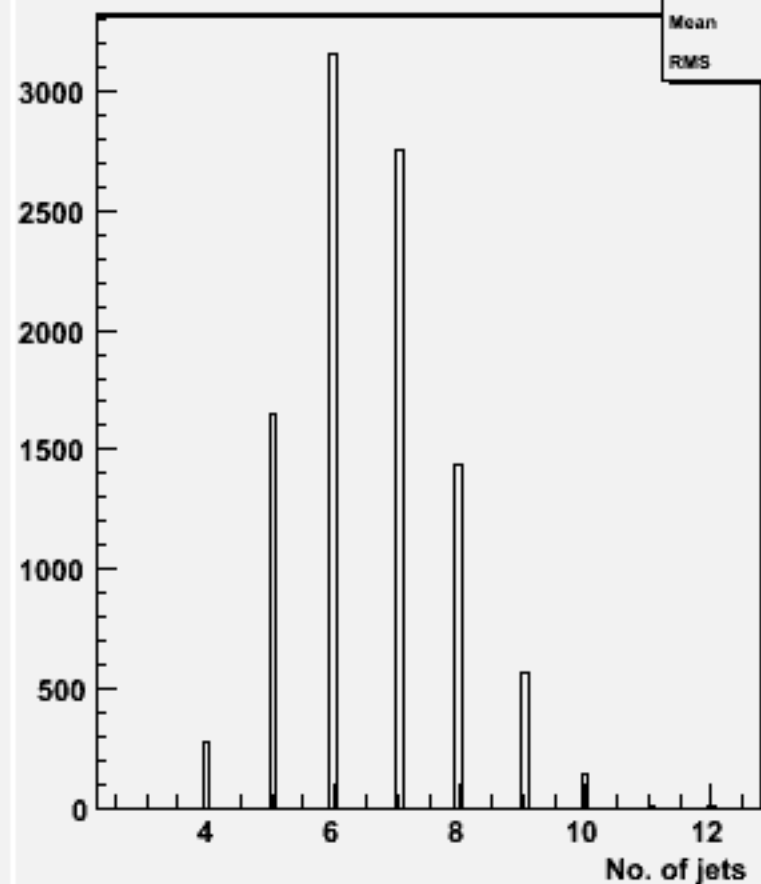
No. jets (ycut=0.001) : w101712 ccn1e1sc_o
