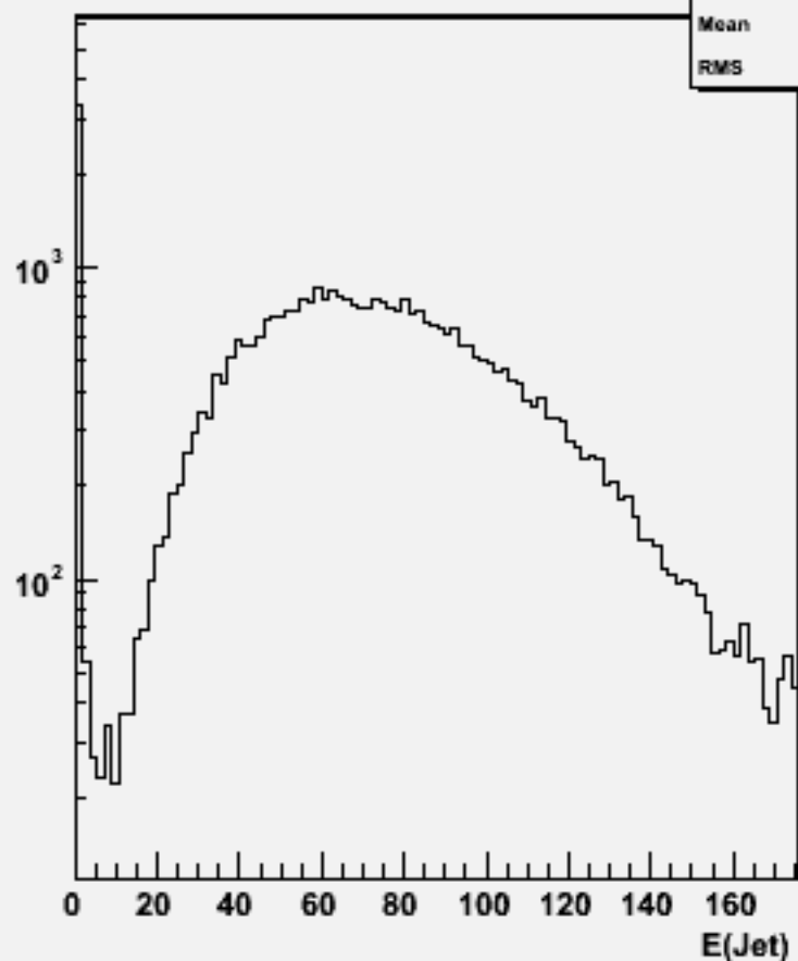
Jet energies(All jets)w101712 ccn1e1sc_o
