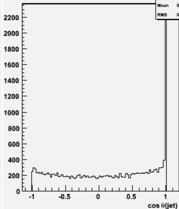
cos \Theta for 2-jets :w101705 ccn1e1e3n3_o
