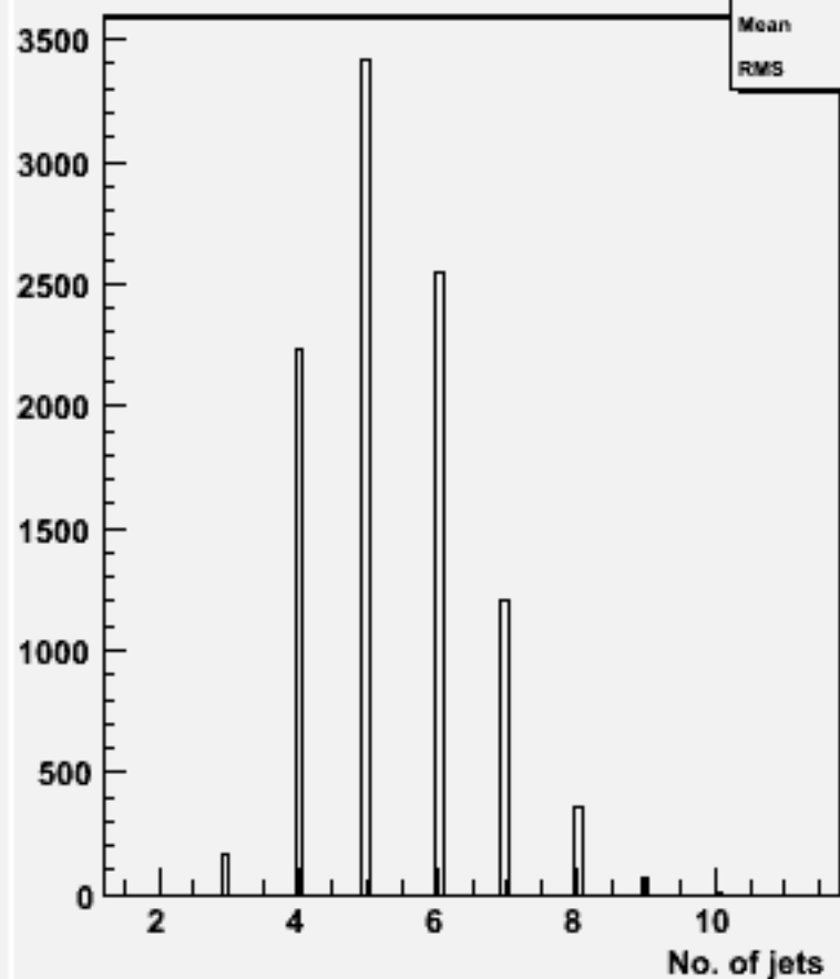
No. jets (ycut=0.001) : w101705 ccn1e1e3n3_o
