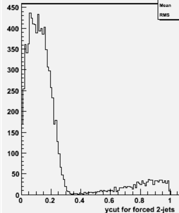
Ycut for 2-jets :w101705 ccn1e1e3n3_o
