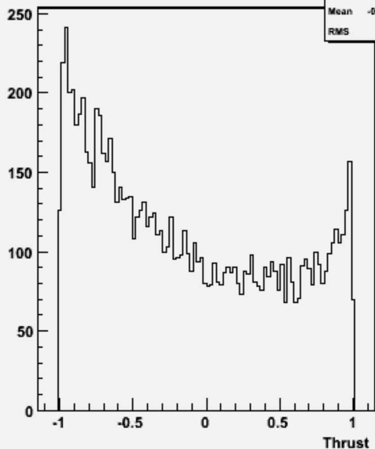
cos \Theta (thrust) w101705 ccn1e1e3n3_o
