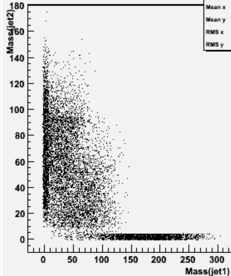
Jet mass for forced 2-jets : w101705 ccn1e1e3n3_o
