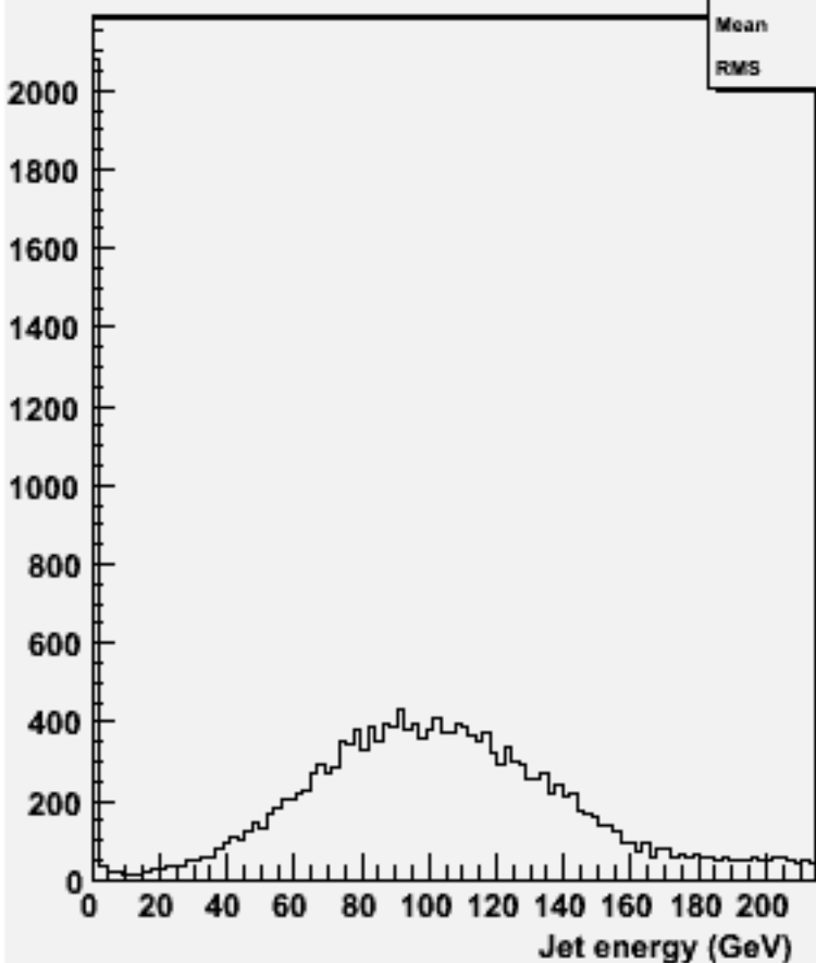
energy for 2-jets :w101705 ccn1e1e3n3_o
