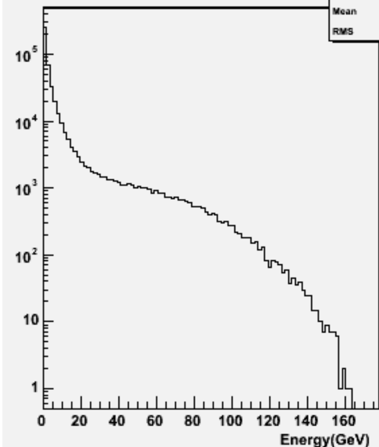
Particle Energy : w101705 ccn1e1e3n3_o
