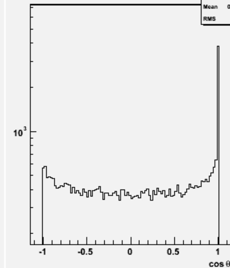
Jet cos \theta (All jets)w101701 ccn1e1e2n2_o
