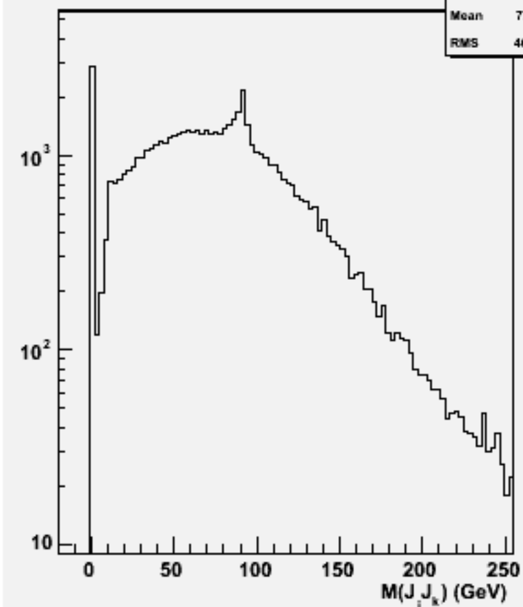
2jets mass(All comb)w101701 ccn1e1e2n2_o
