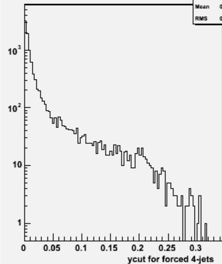
Ycut for 4-jets :w101701 ccn1e1e2n2_o
