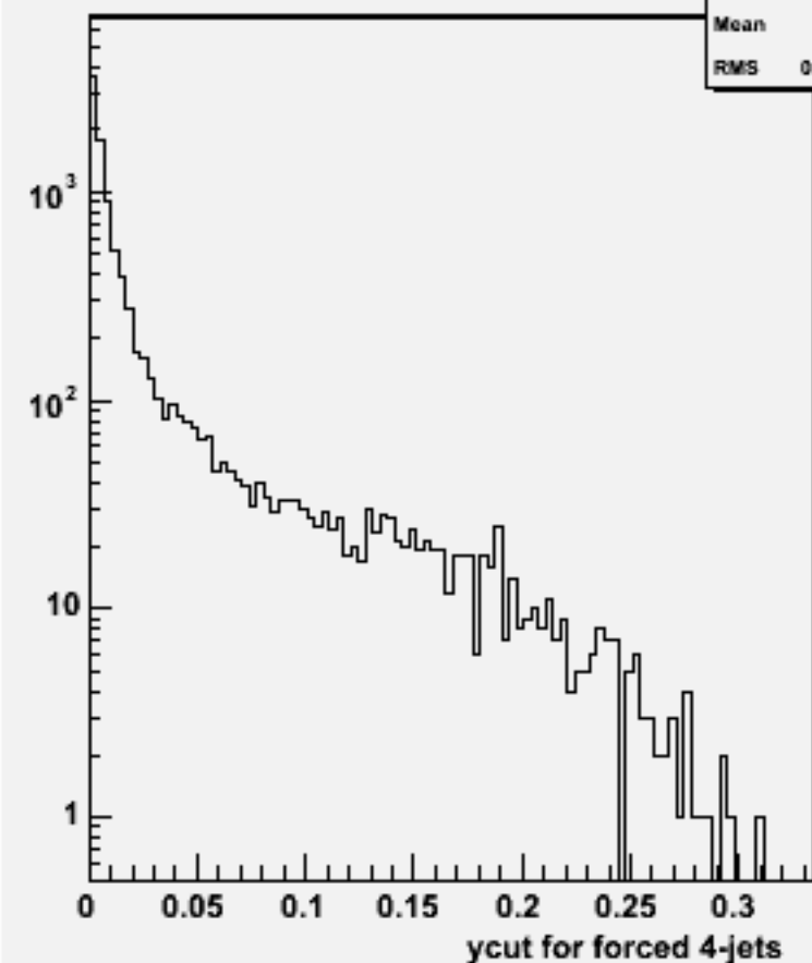
Ycut for 4-jets :w101700 ccn1e1e2n2_o
