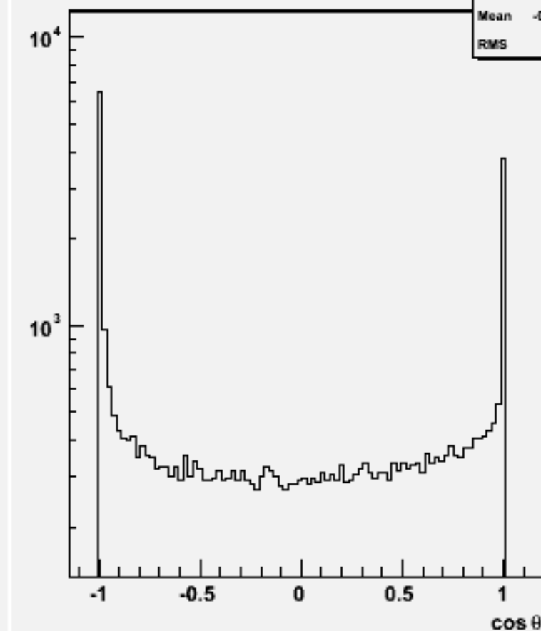
Jet cos \theta (All jets)w101700 ccn1e1e2n2_o
