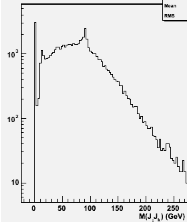
2jets mass(All comb)w101700 ccn1e1e2n2_o
