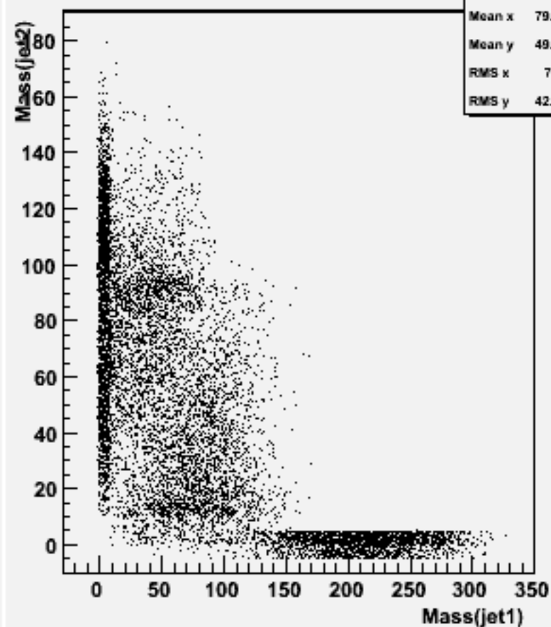
Jet mass for forced 2-jets : w101699 ccn1e1e2n2_o
