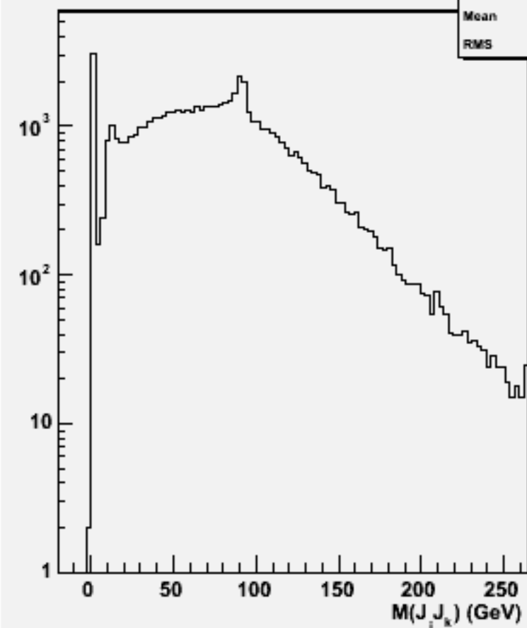
2jets mass(All comb)w101699 ccn1e1e2n2_o
