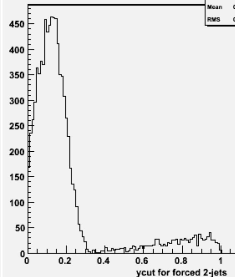
Ycut for 2-jets :w101699 ccn1e1e2n2_o
