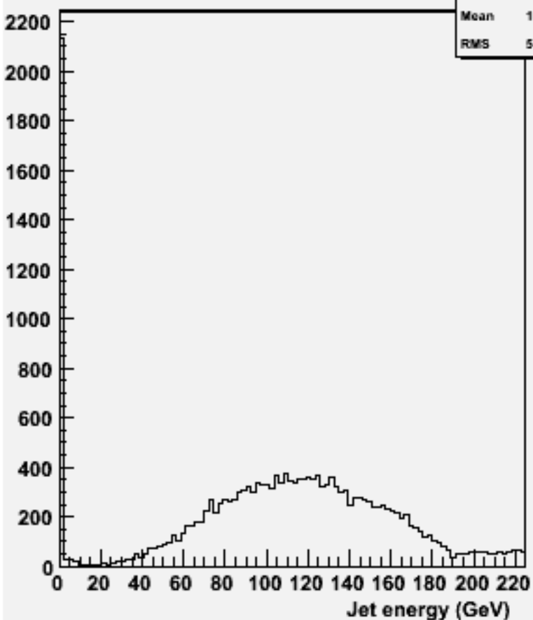
energy for 2-jets :w101699 ccn1e1e2n2_o
