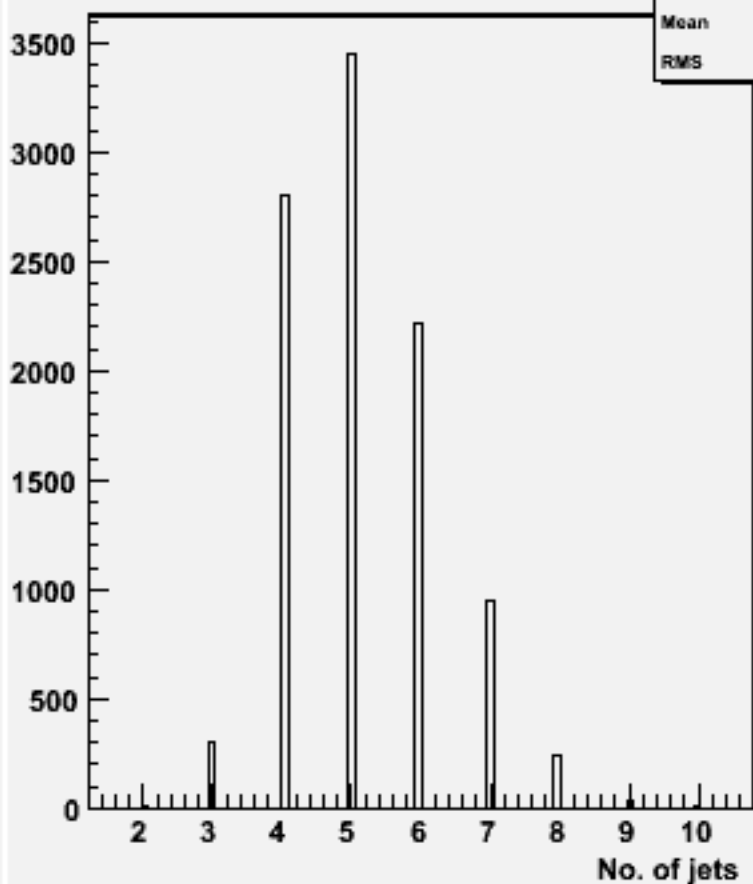
No. jets (ycut=0.001) : w101699 ccn1e1e2n2_o
