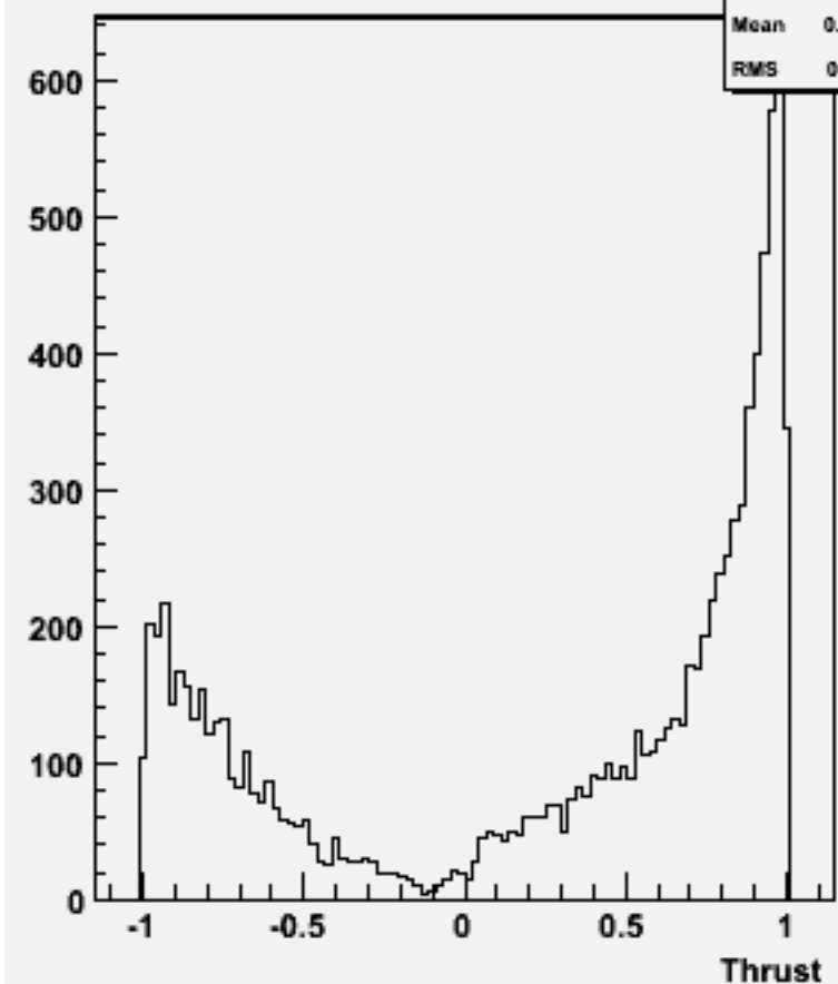
cos \Theta (thrust) w101699 ccn1e1e2n2_o
