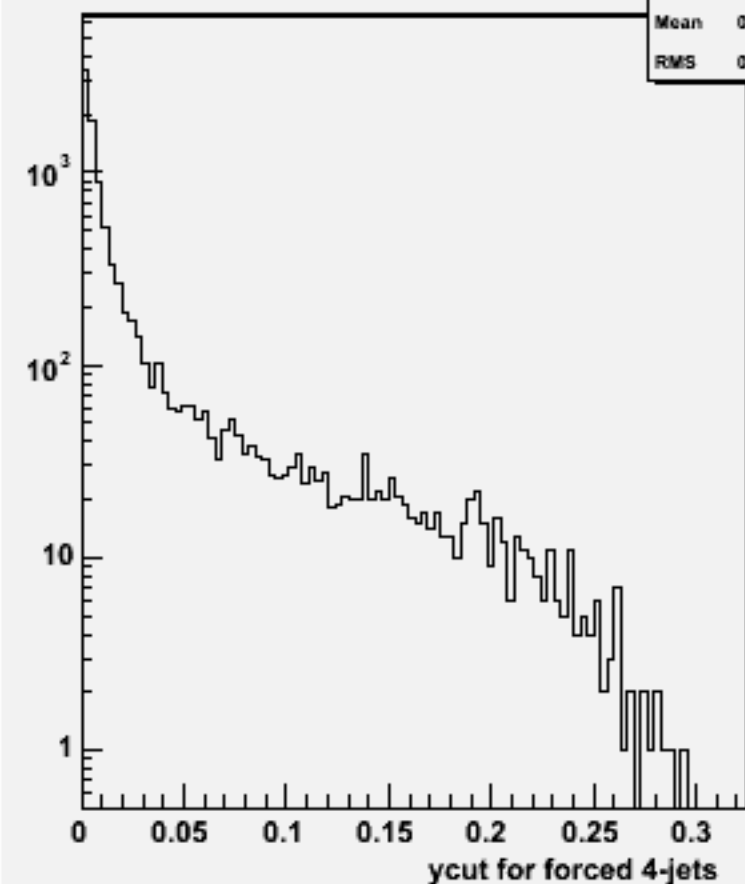
Ycut for 4-jets :w101699 ccn1e1e2n2_o
