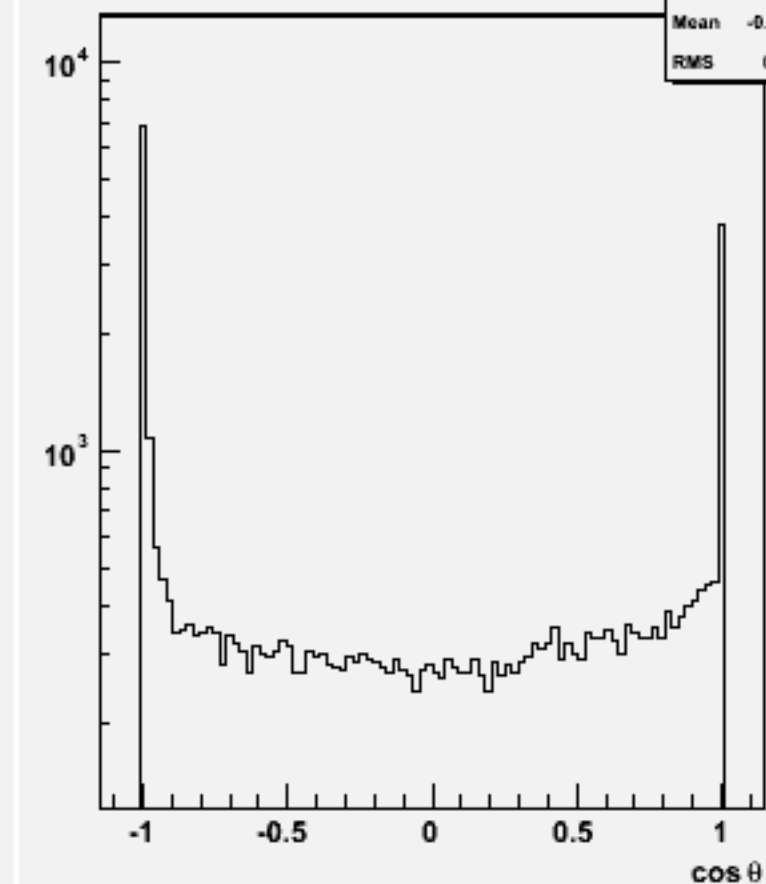
Jet cos \theta (All jets)w101699 ccn1e1e2n2_o
