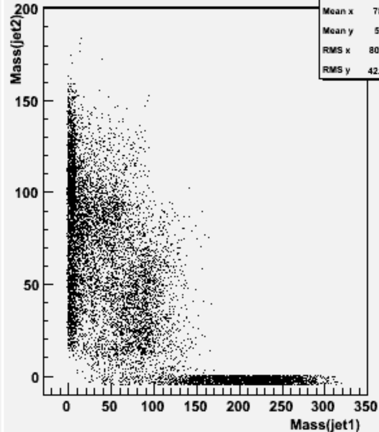
Jet mass for forced 2-jets : w101698 ccn1e1e1n1_o
