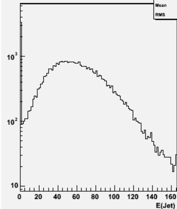
Jet energies(All jets)w101698 ccn1e1e1n1_o
