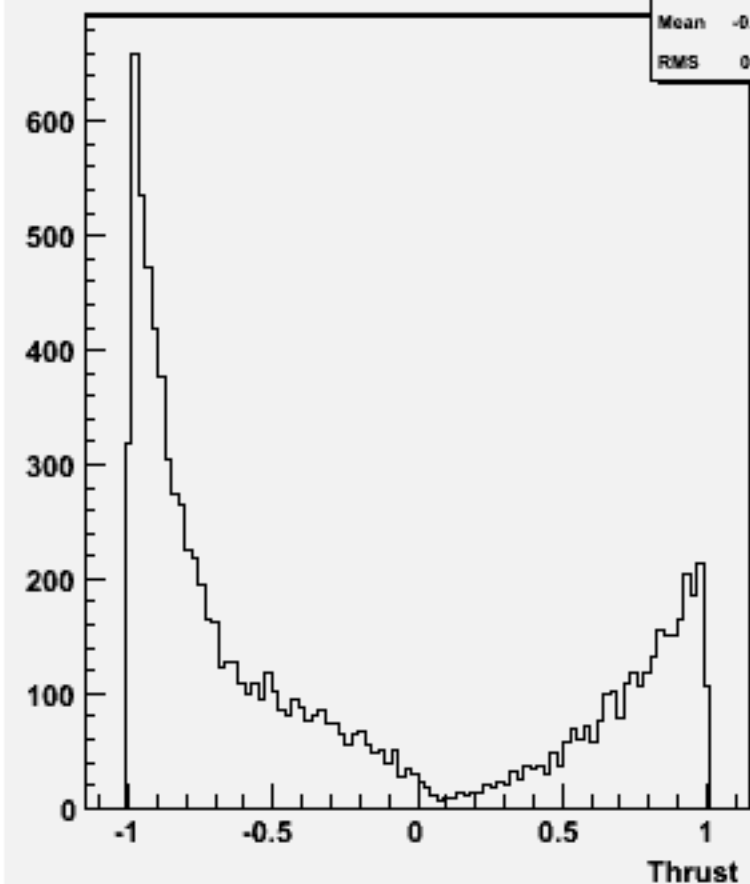
cos \Theta (thrust) w101698 ccn1e1e1n1_o
