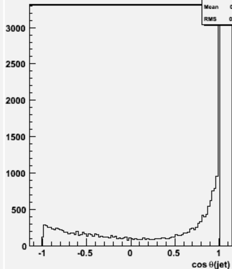
cos \theta for 2-jets :w101698 ccn1e1e1n1_o
