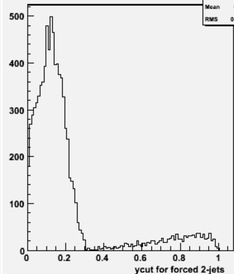
Ycut for 2-jets :w101698 ccn1e1e1n1_o
