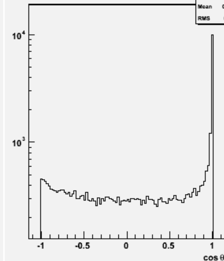
Jet cos \theta (All jets)w101698 ccn1e1e1n1_o
