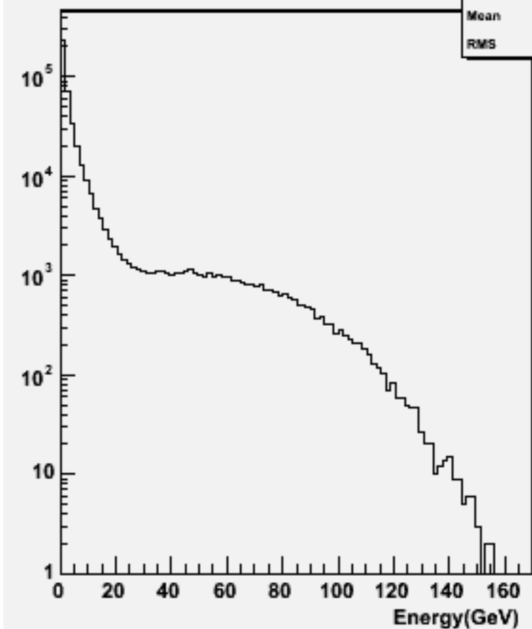
Particle Energy : w101698 ccn1e1e1n1_o
