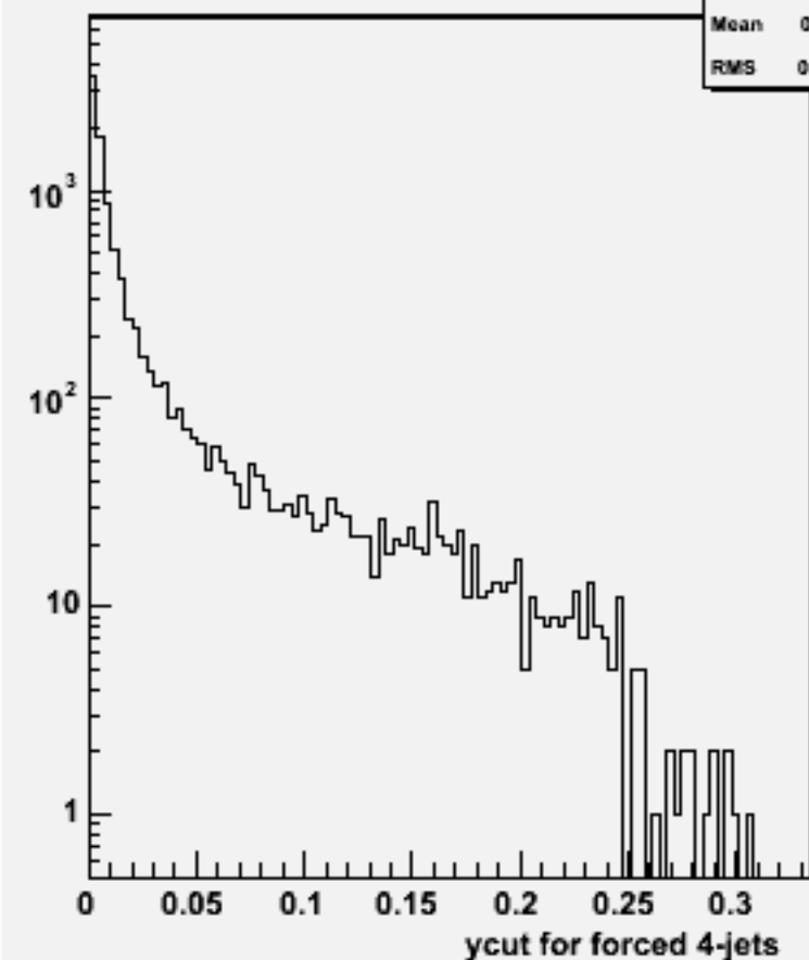
Ycut for 4-jets :w101698 ccn1e1e1n1_o
