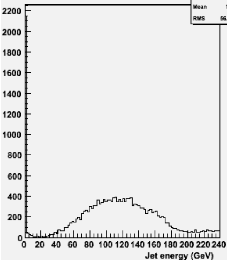
energy for 2-jets :w101698 ccn1e1e1n1_o
