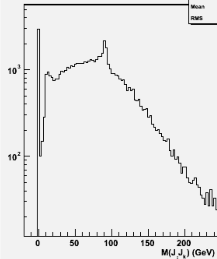
2jets mass(All comb)w101698 ccn1e1e1n1_o
