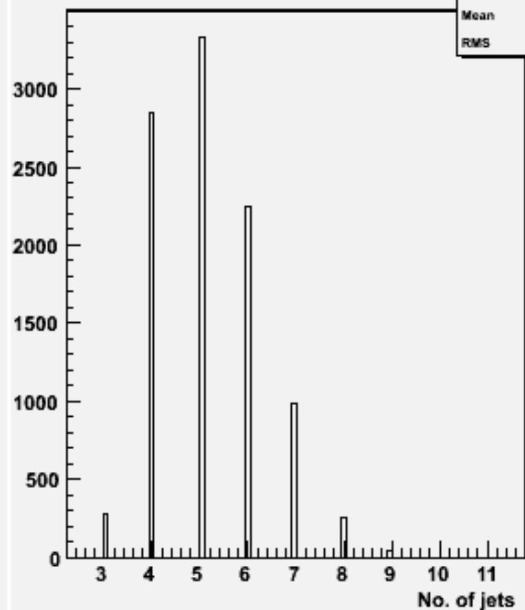
No. jets (ycut=0.001) : w101698 ccn1e1e1n1_o
