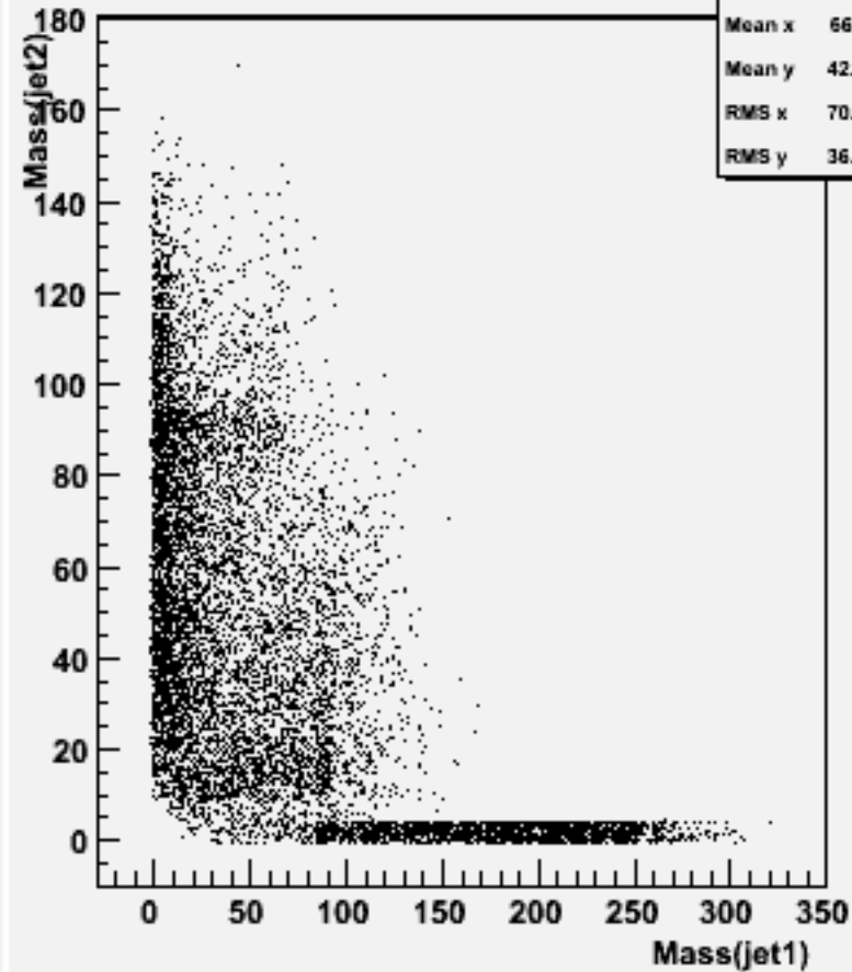
Jet mass for forced 2-jets : w101697 ccn1e1e1n1_o
