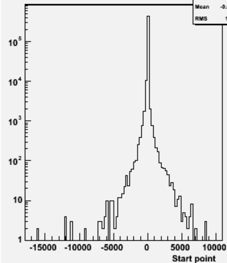
Start point Z : w101697 ccn1e1e1n1_o
