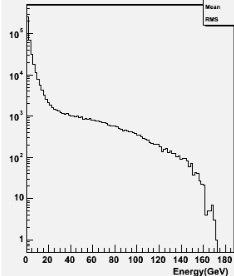
Particle Energy : w101697 ccn1e1e1n1_o
