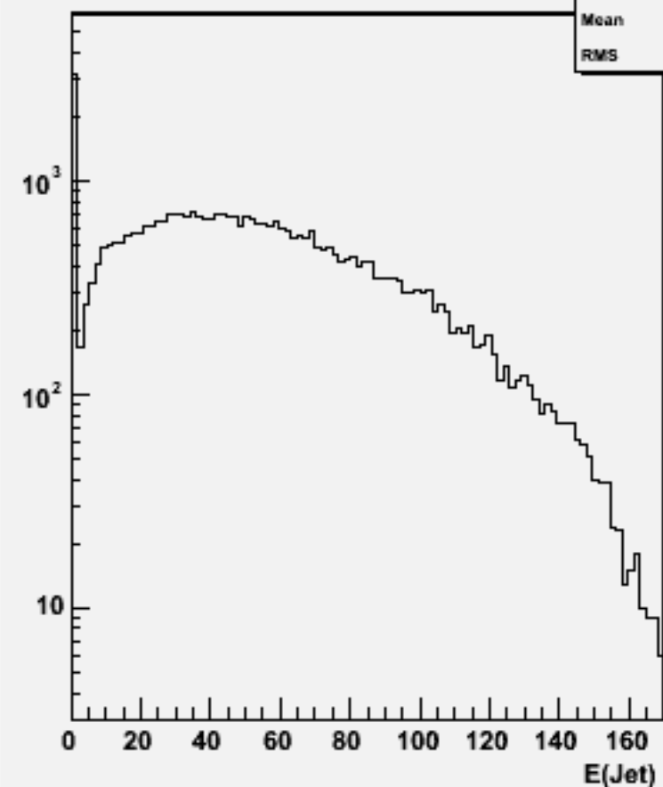
Jet energies(All jets)w101697 ccn1e1e1n1_o
