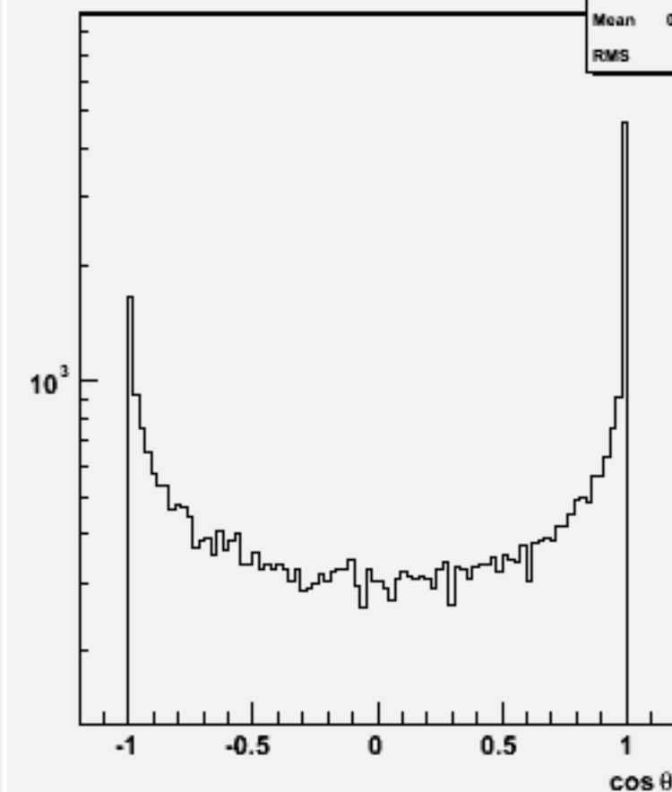
Jet cos \theta (All jets)w101697 ccn1e1e1n1_o
