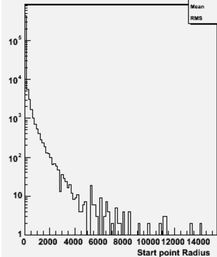
Start point R : w101697 ccn1e1e1n1_o
