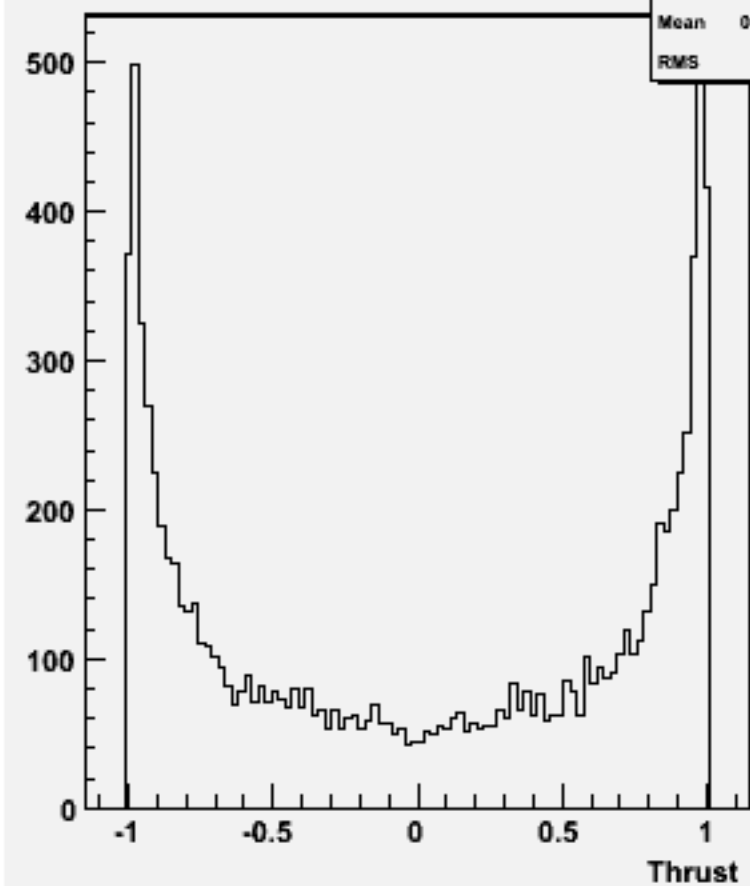
cos \Theta (thrust) w101697 ccn1e1e1n1_o
