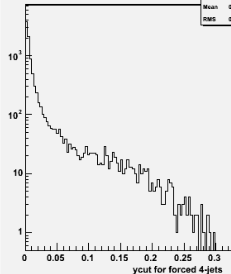
Ycut for 4-jets :w101697 ccn1e1e1n1_o
