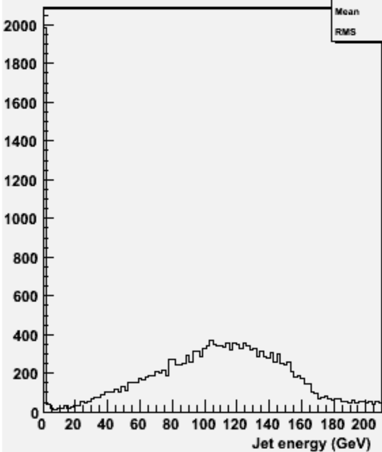
energy for 2-jets :w101697 ccn1e1e1n1_o
