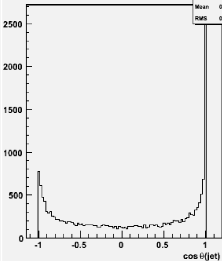
cos \theta for 2-jets :w101697 ccn1e1e1n1_o
