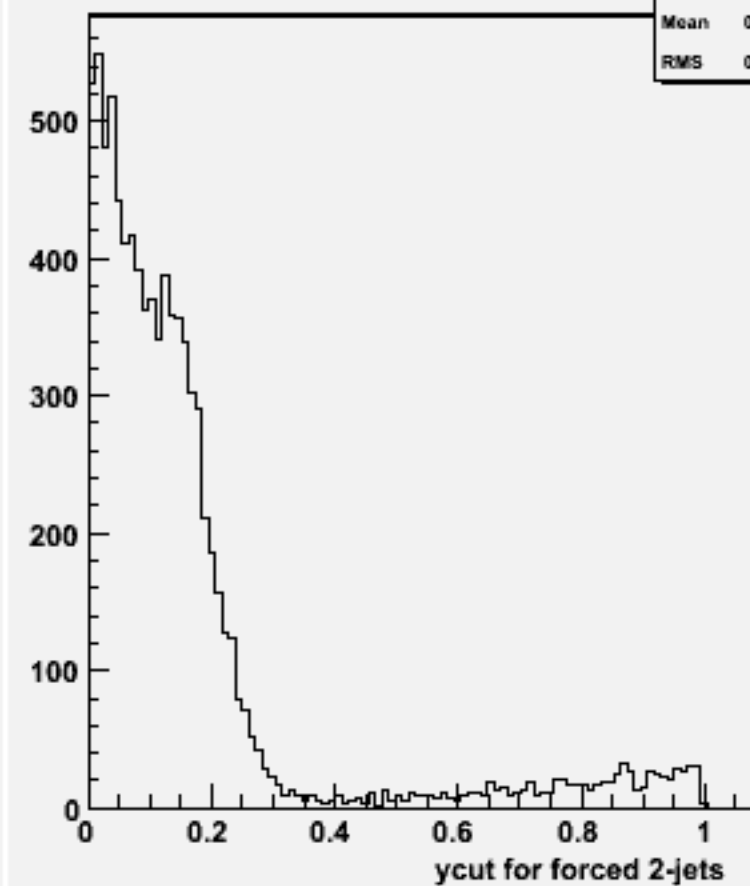
Ycut for 2-jets :w101697 ccn1e1e1n1_o
