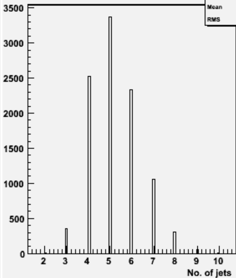
No. jets (ycut=0.001) : w101697 ccn1e1e1n1_o
