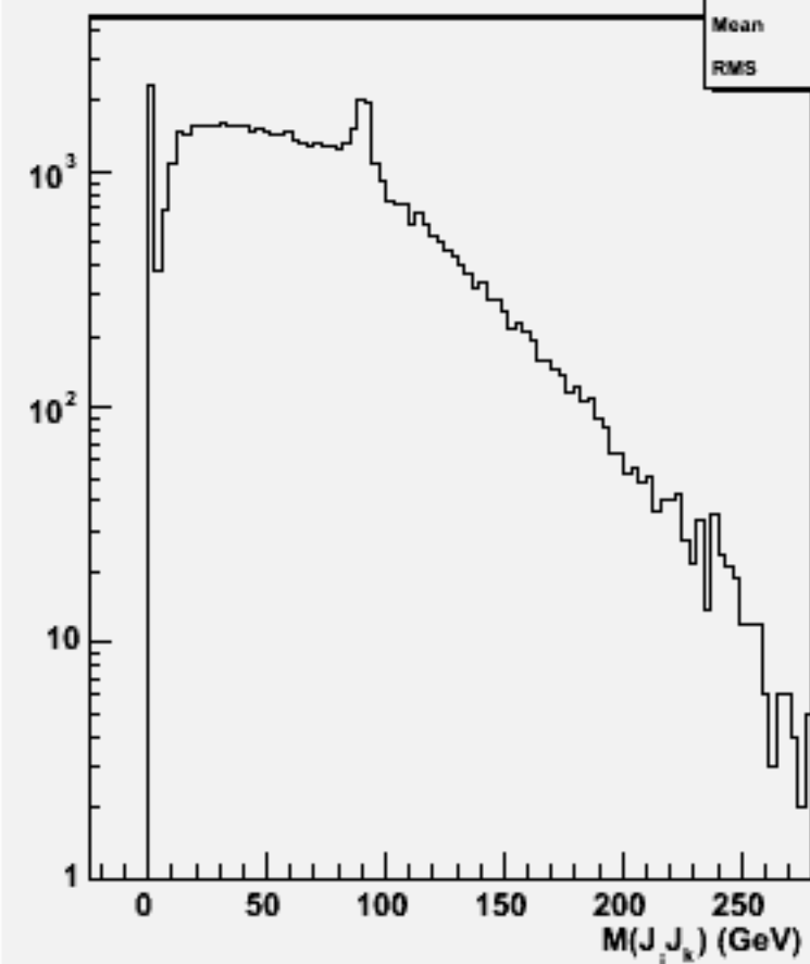
2jets mass(All comb)w101697 ccn1e1e1n1_o
