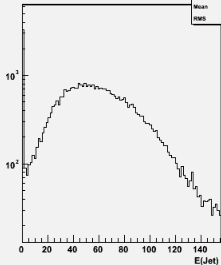
Jet energies(All jets)w101695 ccn1e1e1n1_o
