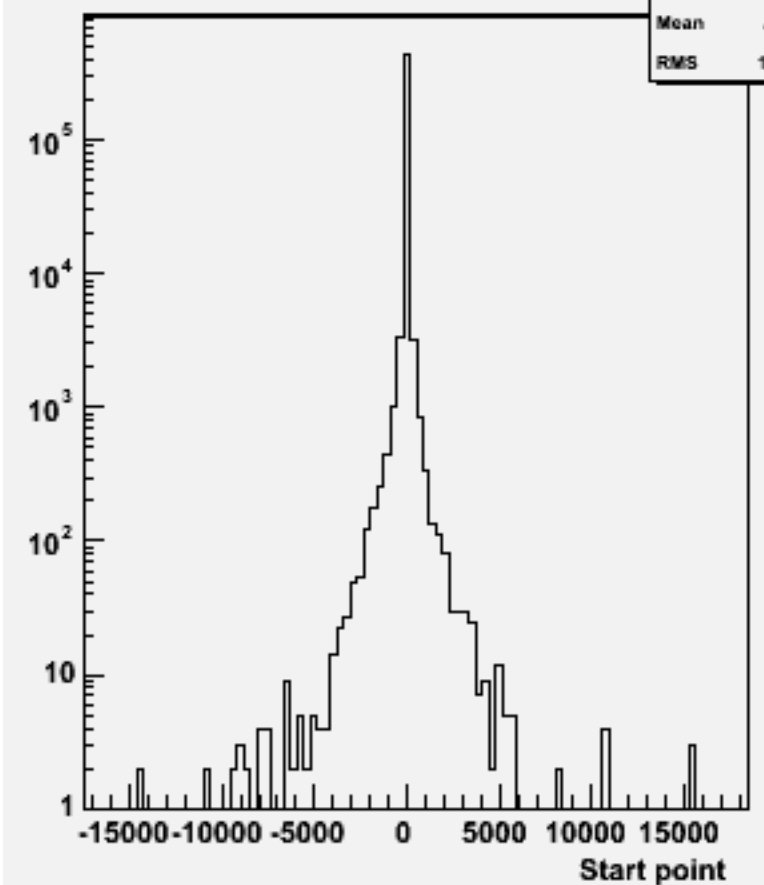
Start point Z : w101695 ccn1e1e1n1_o
