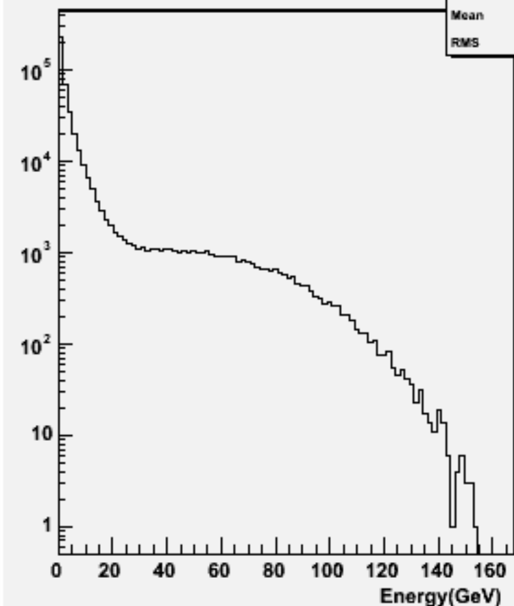
Particle Energy : w101695 ccn1e1e1n1_o
