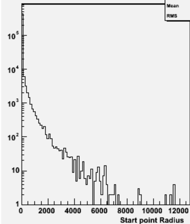
Start point R : w101695 ccn1e1e1n1_o
