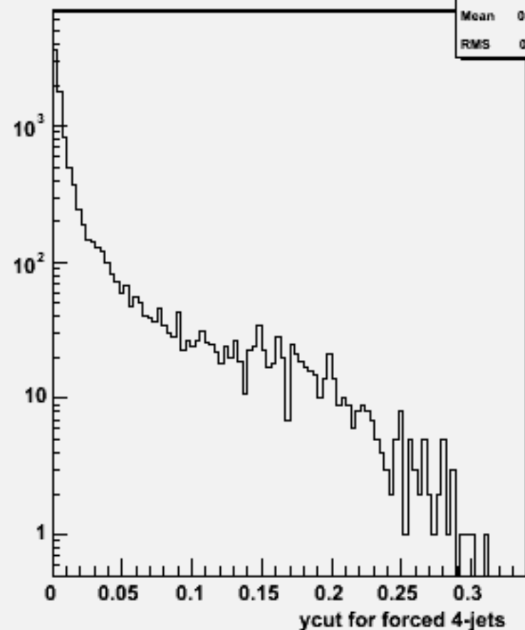
Ycut for 4-jets :w101695 ccn1e1e1n1_o
