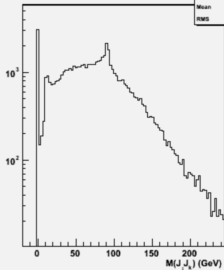
2jets mass(All comb)w101695 ccn1e1e1n1_o
