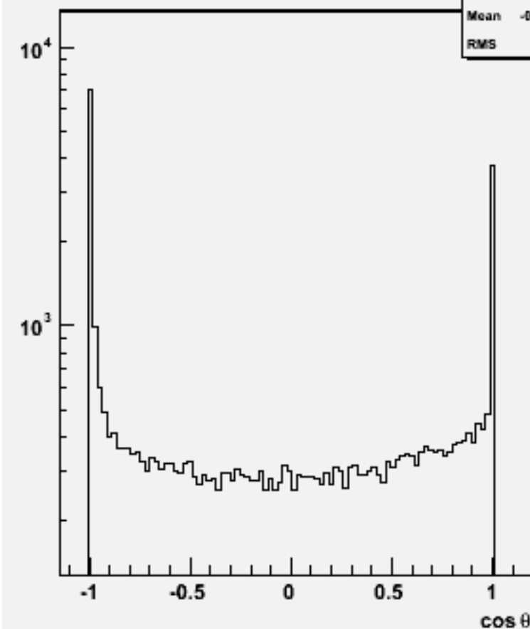
Jet cos \theta (All jets)w101695 ccn1e1e1n1_o
