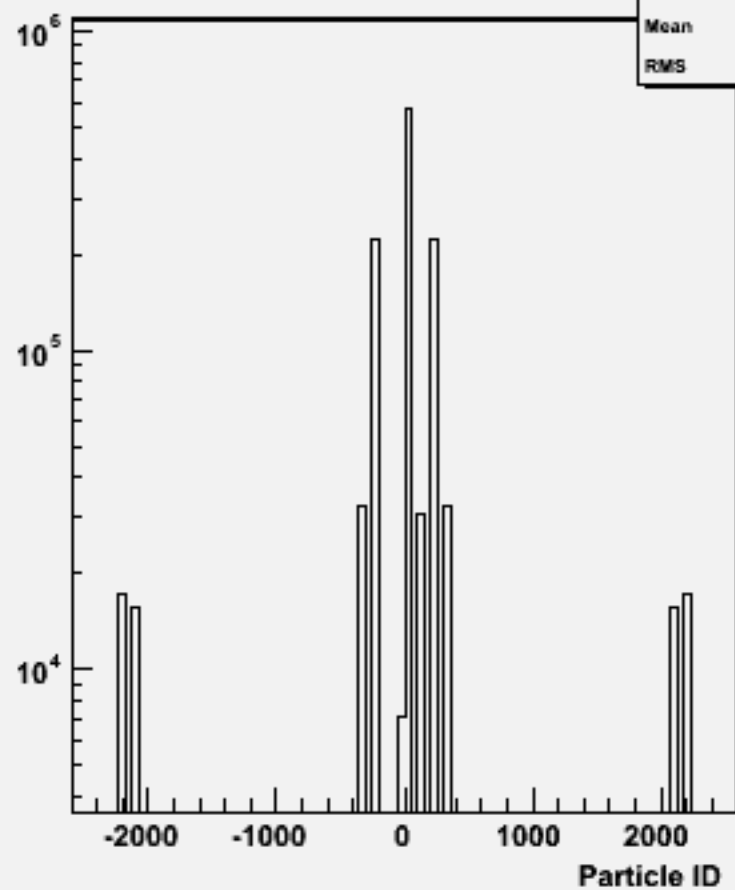
Particle ID : w101693 uucssc_o
