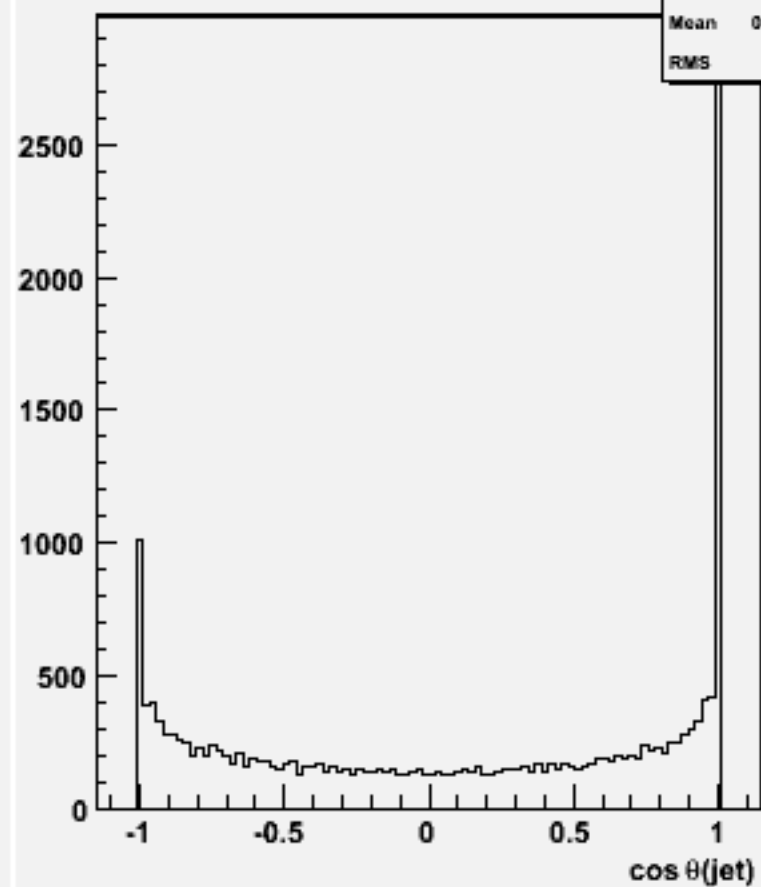
cos \theta for 2-jets :w101693 uucssc_o
