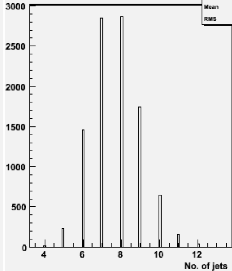
No. jets (ycut=0.001) : w101693 uucssc_o
