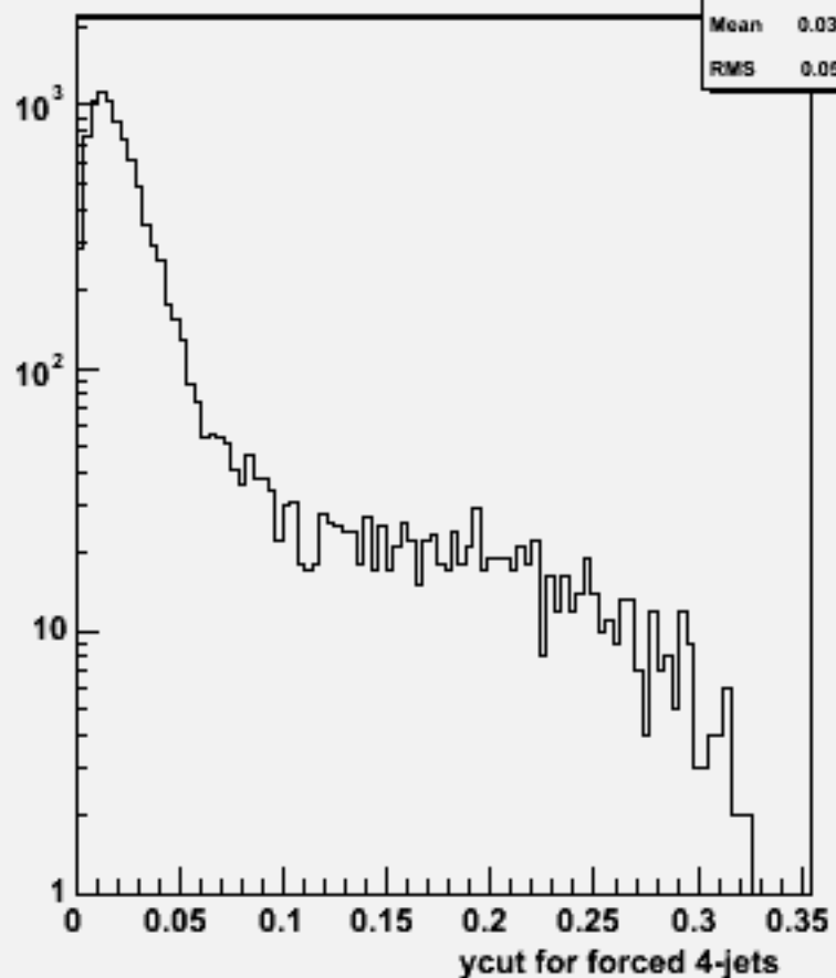
Ycut for 4-jets :w101693 uucssc_o
