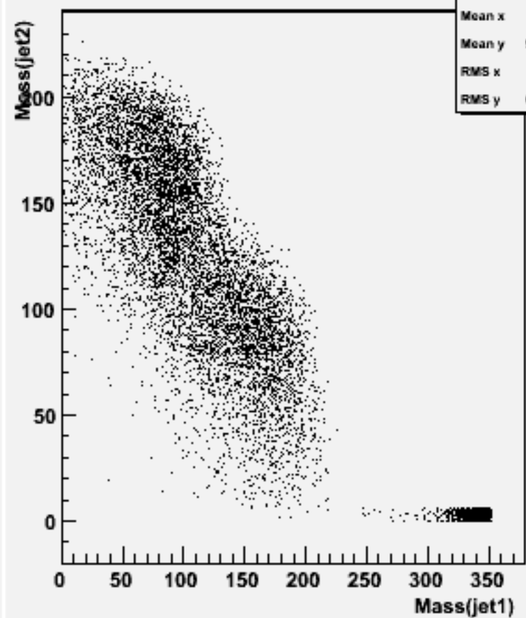
Jet mass for forced 2-jets : w101693 uucssc_o
