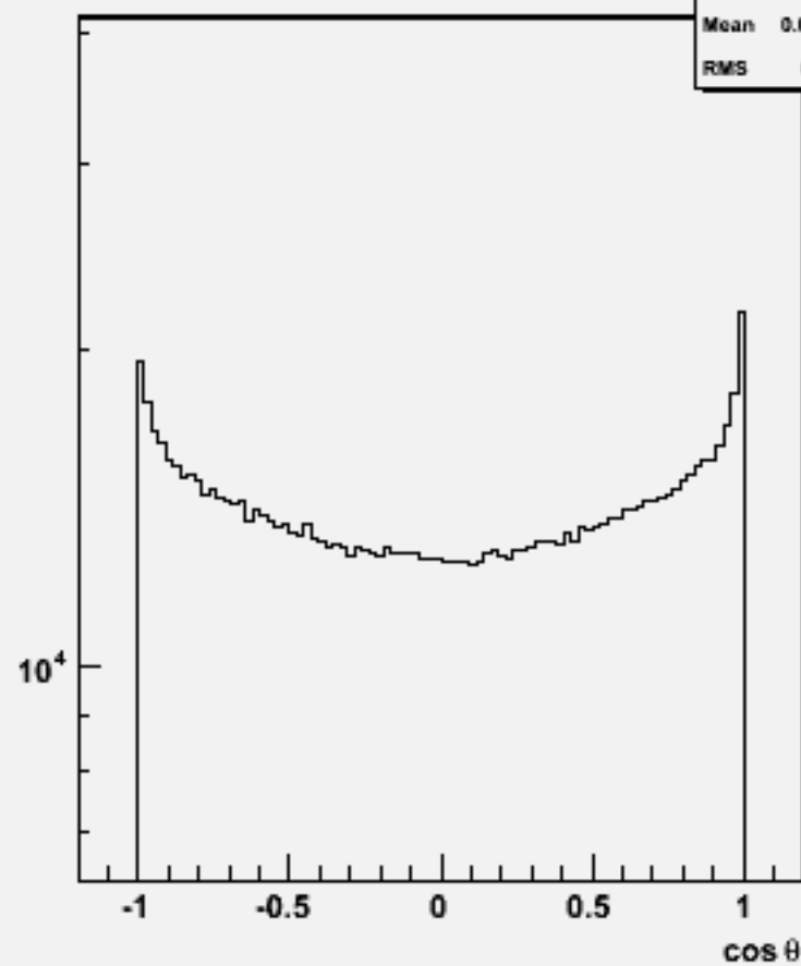
Particle cos \theta : w101693 uucssc_o
