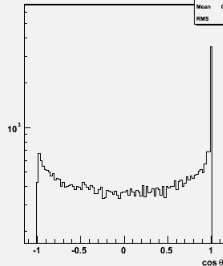
Jet cos \theta (All jets)w101693 uucssc_o
