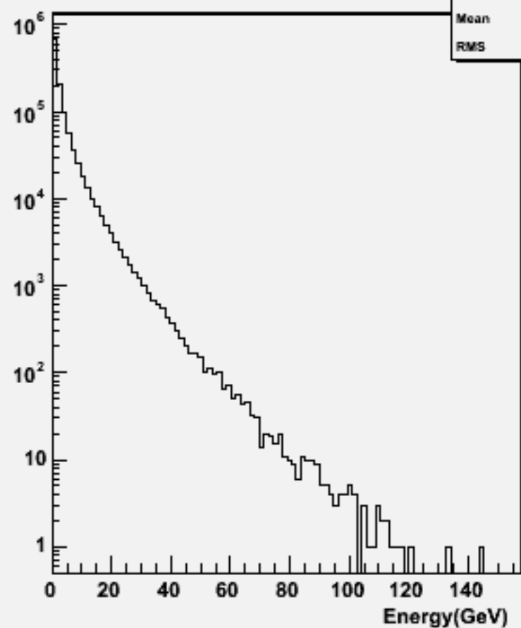
Particle Energy : w101693 uucssc_o
