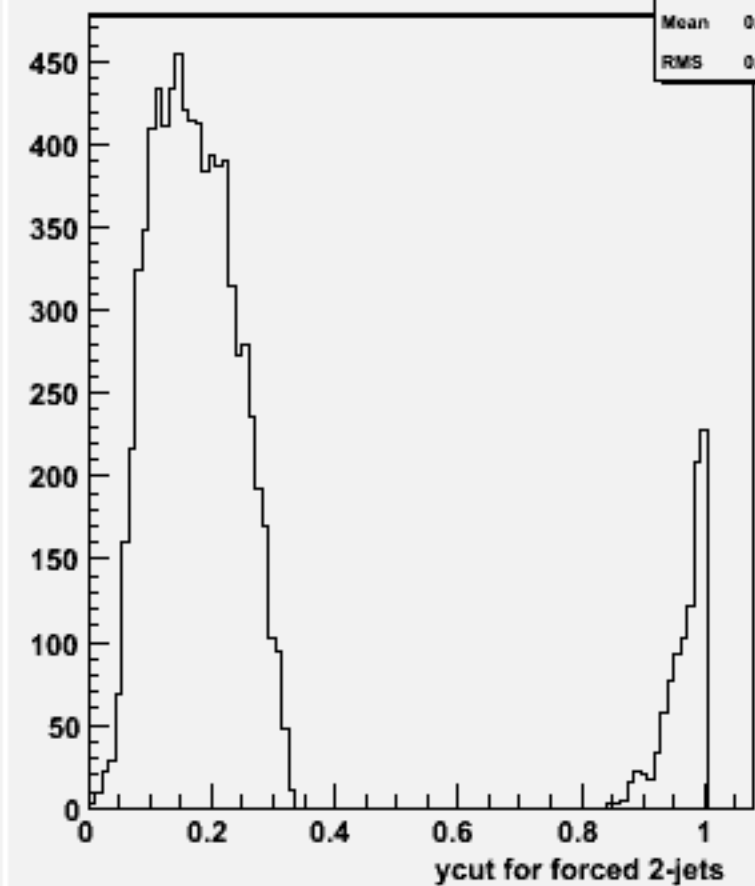
Ycut for 2-jets :w101693 uucssc_o
