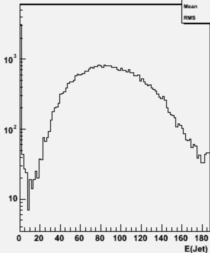
Jet energies(All jets)w101693 uucssc_o
