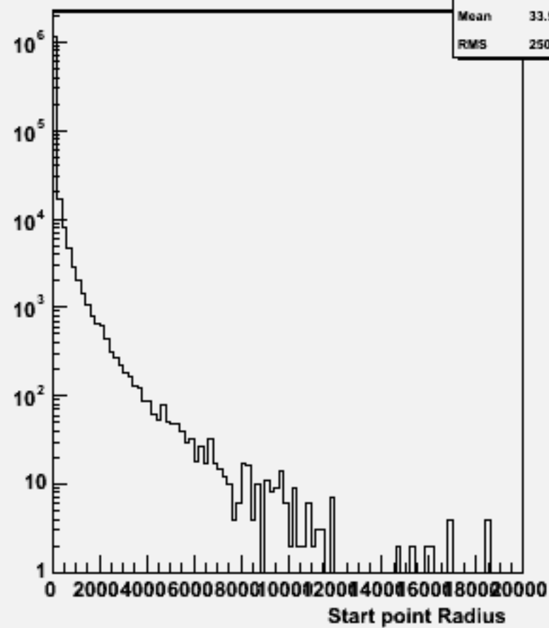
Start point R : w101693 uucssc_o
