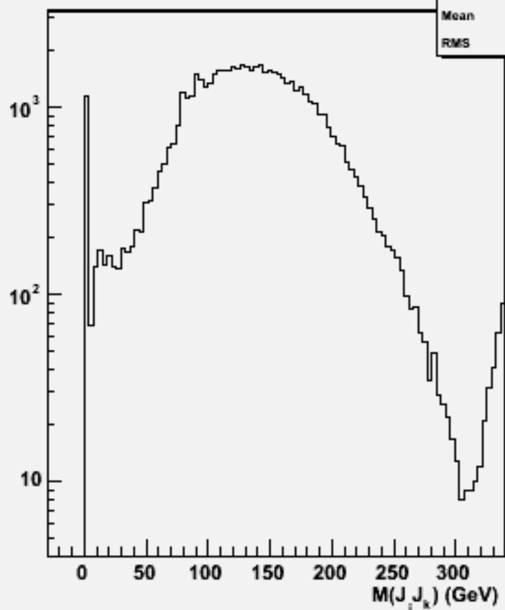
2jets mass(All comb)w101693 uucssc_o
