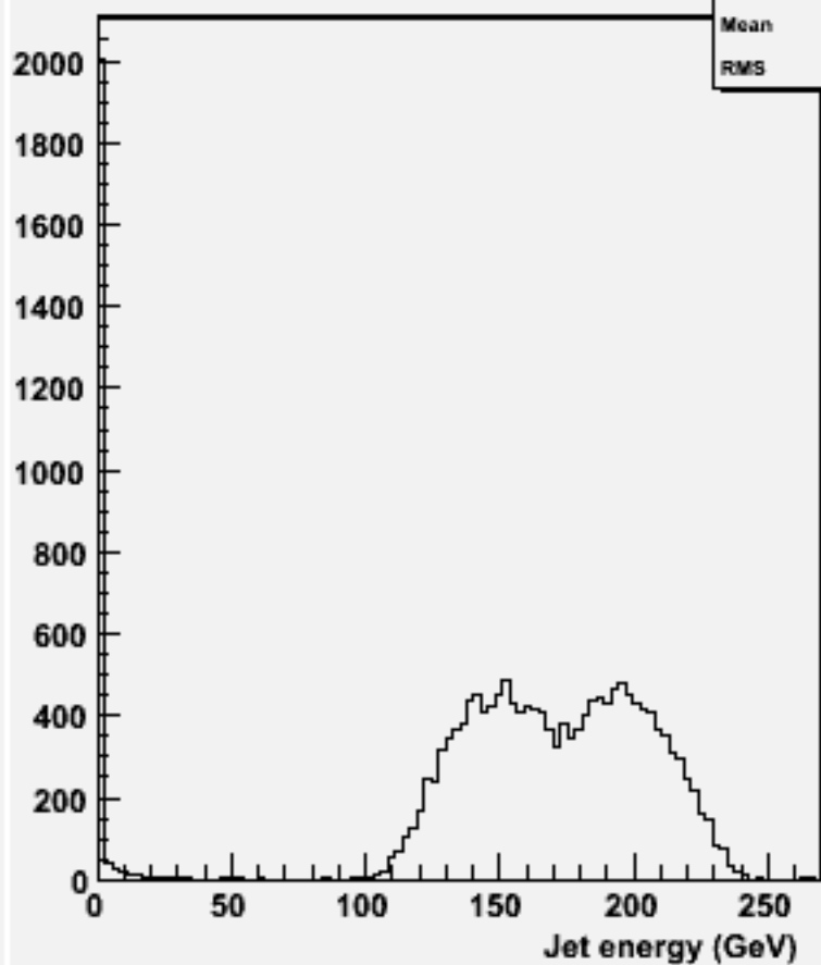
energy for 2-jets :w101693 uucssc_o
