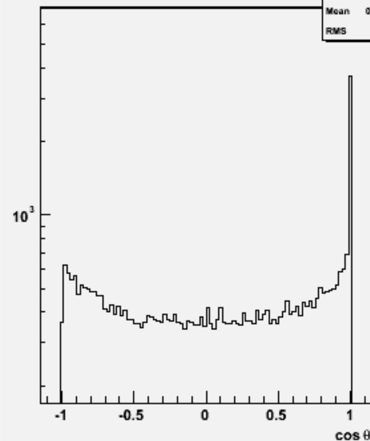
Jet cos \theta (All jets)w101692 uucssc_o
