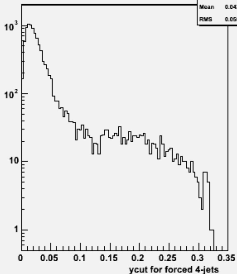
Ycut for 4-jets :w101692 uucssc_o
