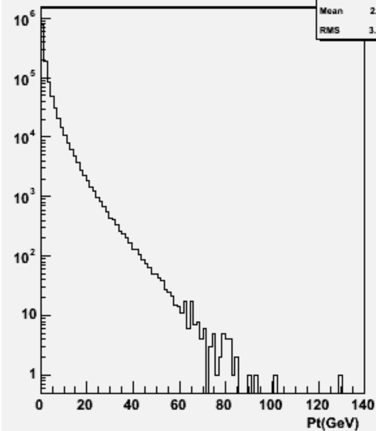
Start point Z : w101692 uucssc_o
