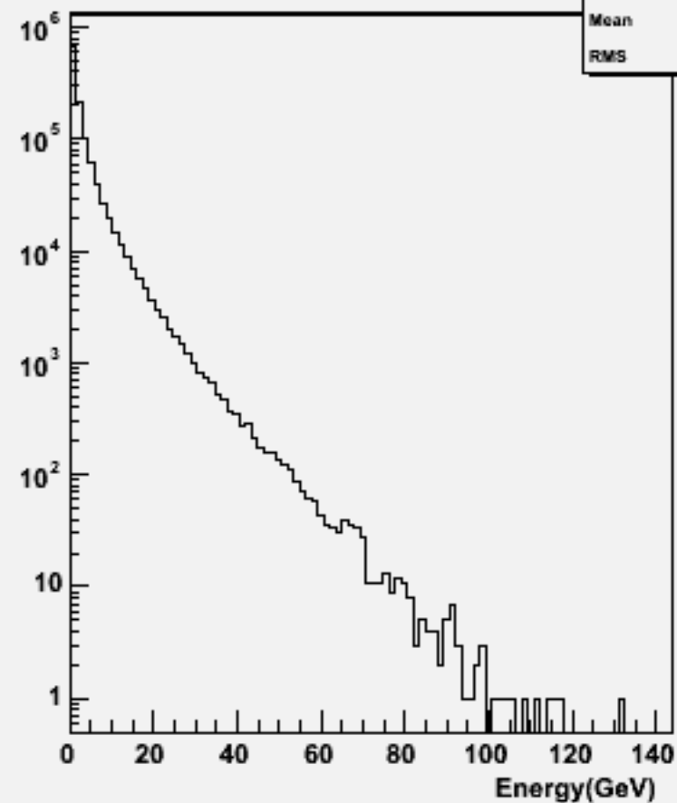
Start point R : w101692 uucssc_o
