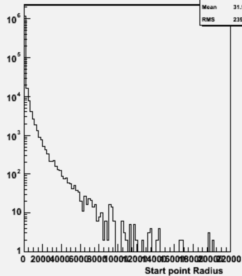
Start point R : w101692 uucssc_o
