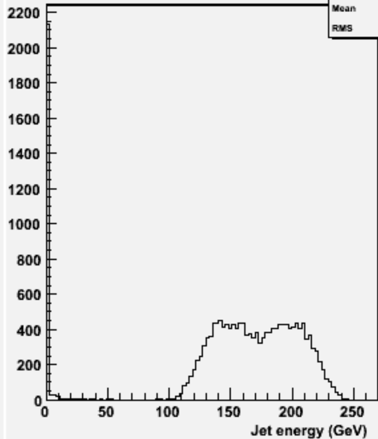
energy for 2-jets :w101692 uucssc_o
