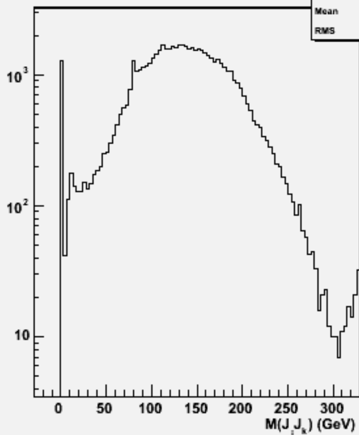
2jets mass(All comb)w101692 uucssc_o
