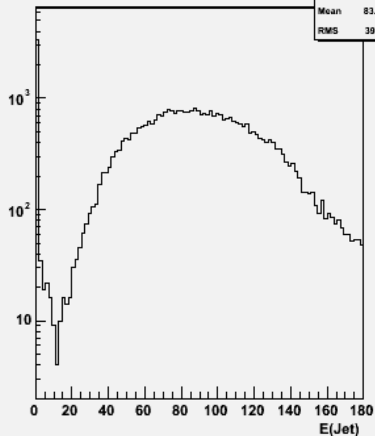
Jet energies(All jets)w101692 uucssc_o
