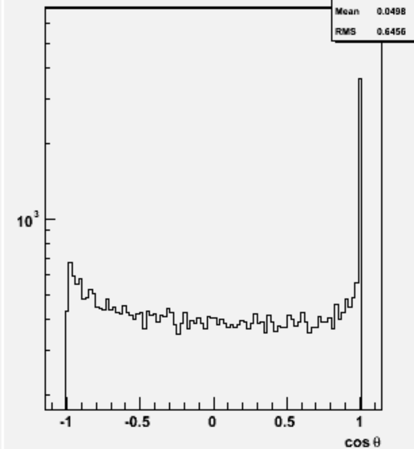
Jet cos \theta (All jets)w101685 uucse3n3_o
