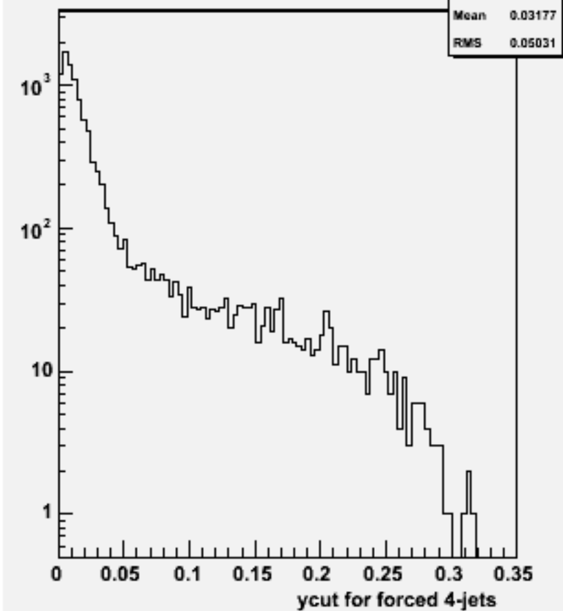
Ycut for 4-jets :w101685 uucse3n3_o
