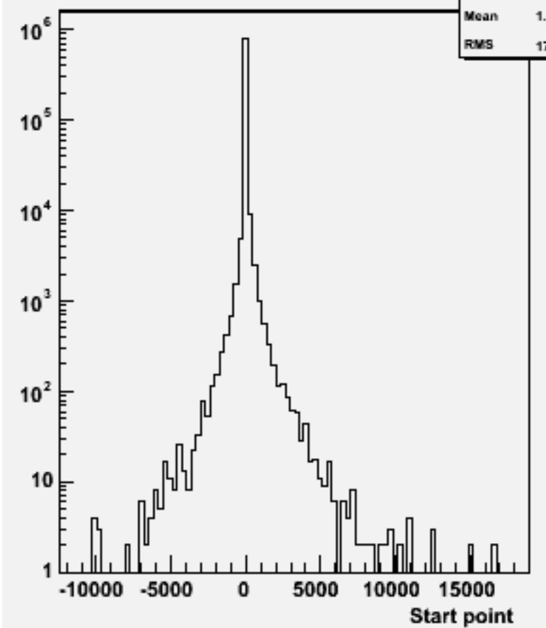
Start point Z : w101685 uucse3n3_o
