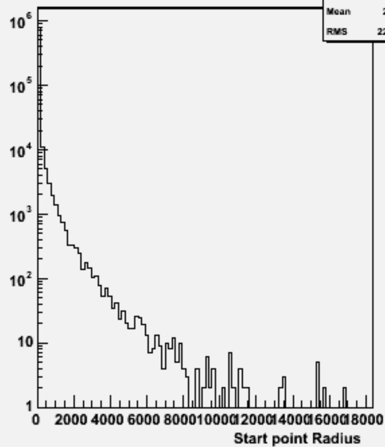
Start point R : w101685 uucse3n3_o
