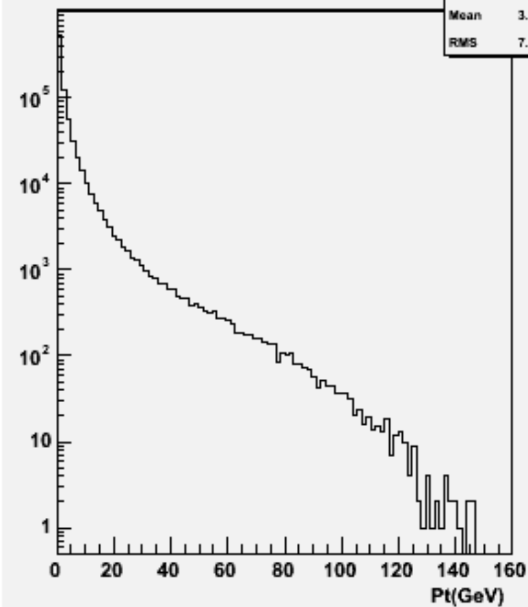
Particle Pt : w101685 uucse3n3_o
