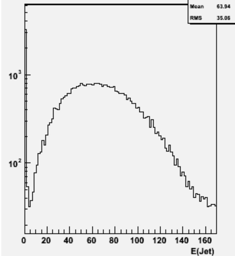
Jet energies(All jets)w101685 uucse3n3_o
