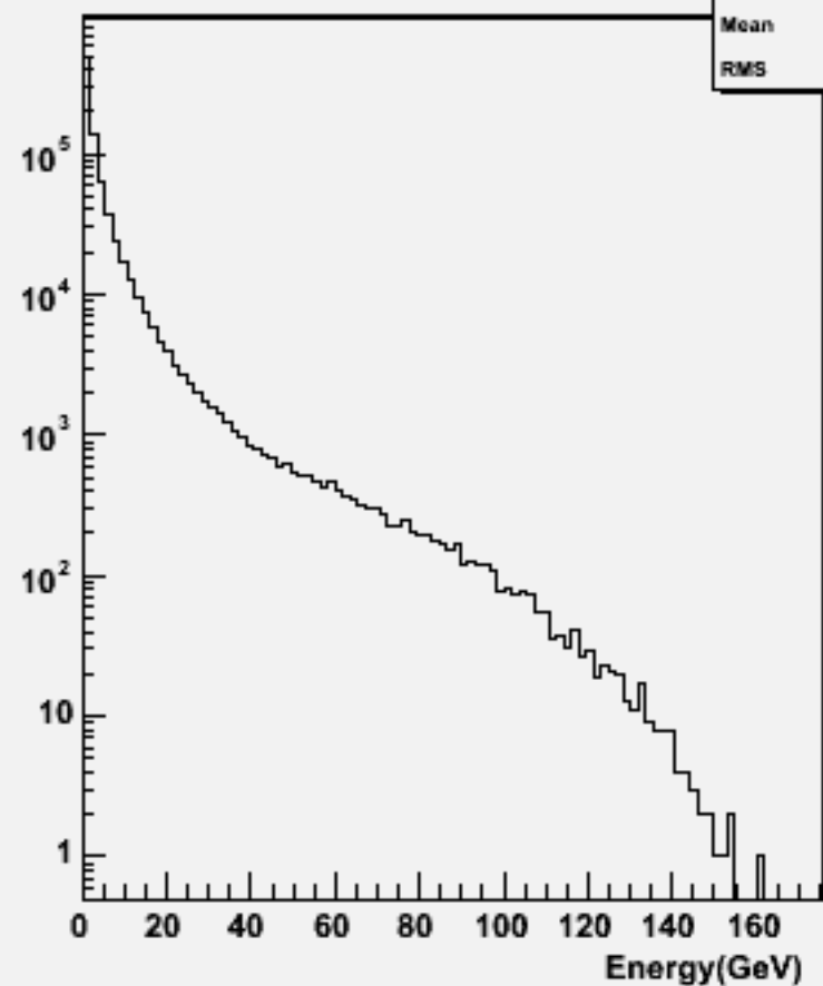
Particle Energy : w101685 uucse3n3_o
