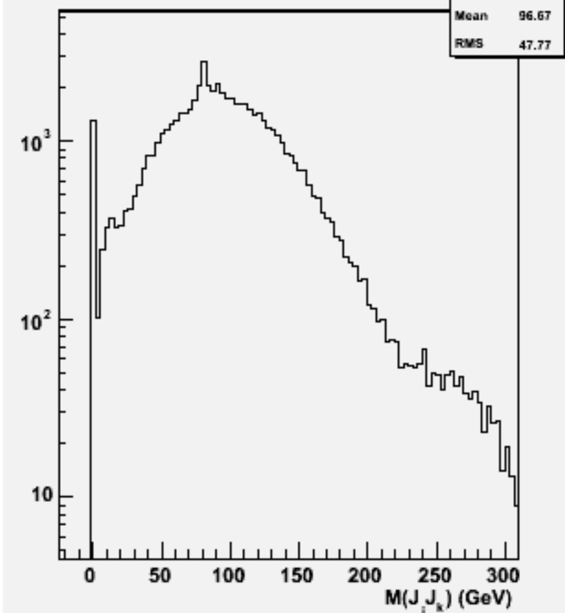
2jets mass(All comb)w101685 uucse3n3_o
