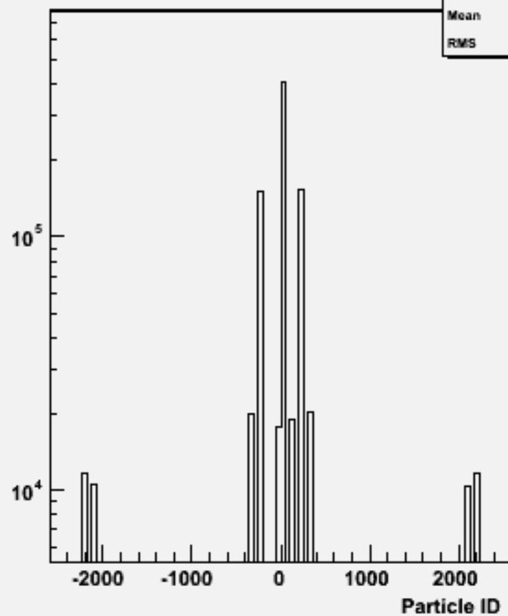
Particle ID : w101685 uucse3n3_o
