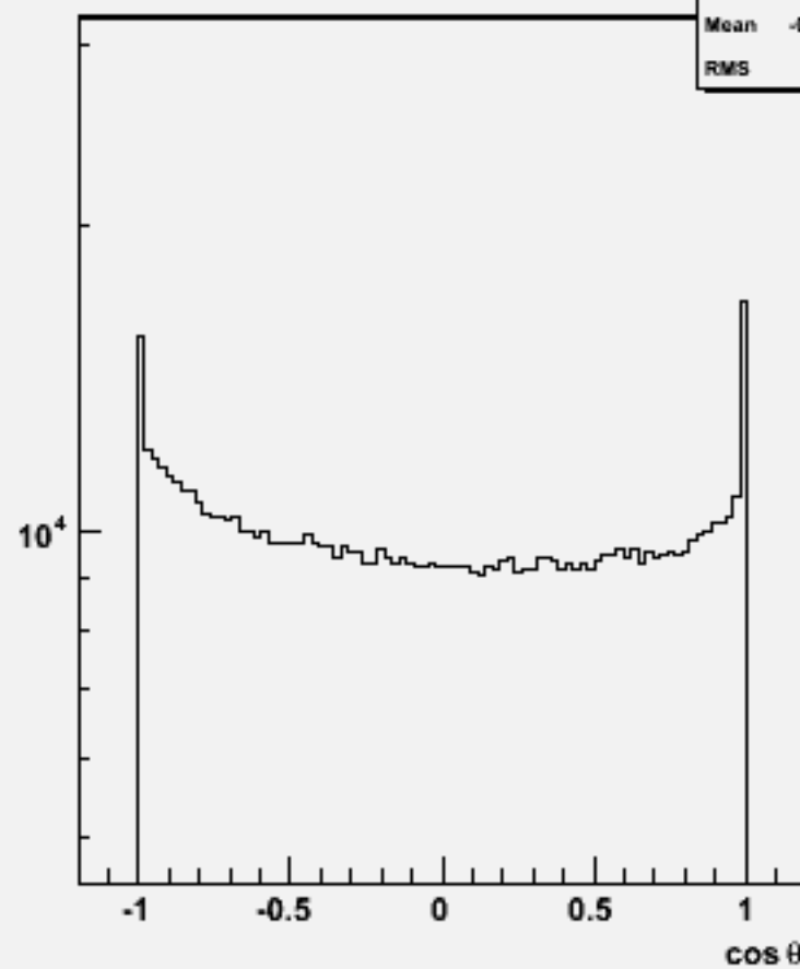
Particle cos \theta : w101685 uucse3n3_o
