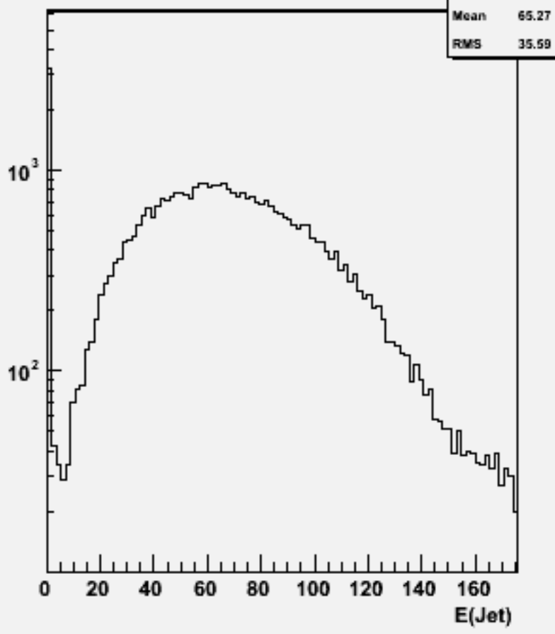
Jet energies(All jets)w101684 uucse3n3_o
