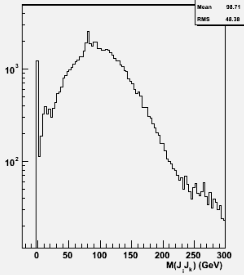
2jets mass(All comb)w101684 uucse3n3_o
