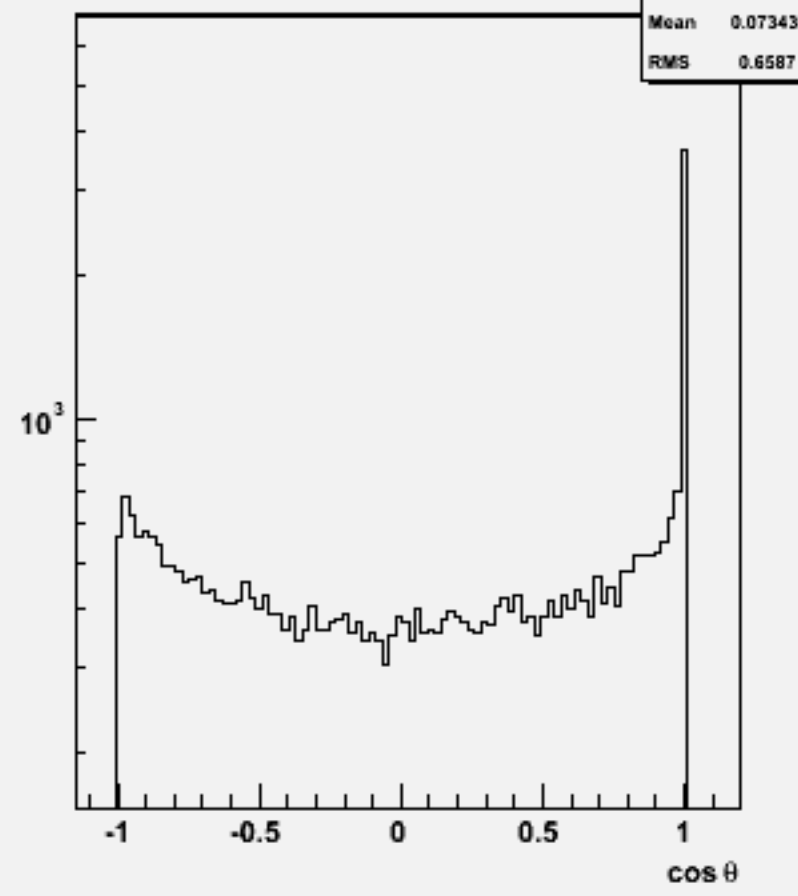
Jet cosθ (All jets)w101684 uucse3n3_o
