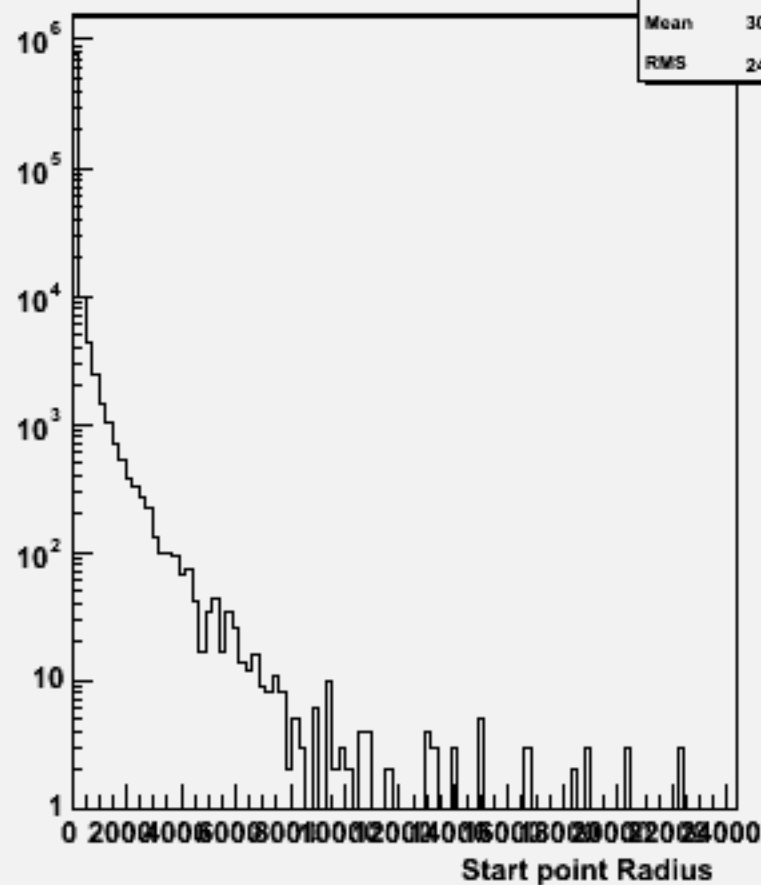
Start point R : w101681 uucse2n2_o
