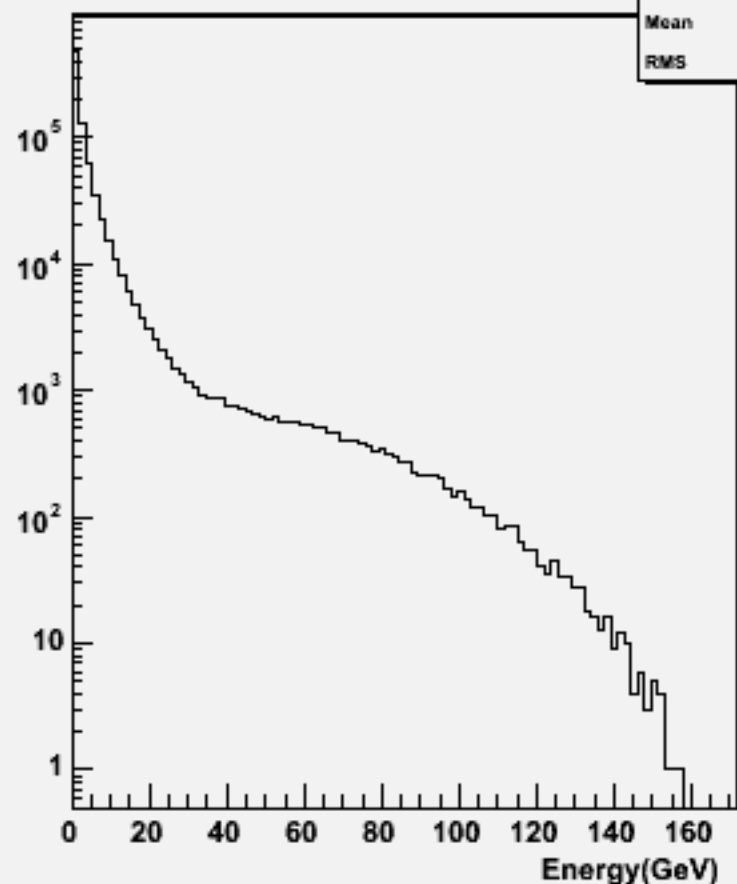
Particle Energy : w101681 uucse2n2_o
