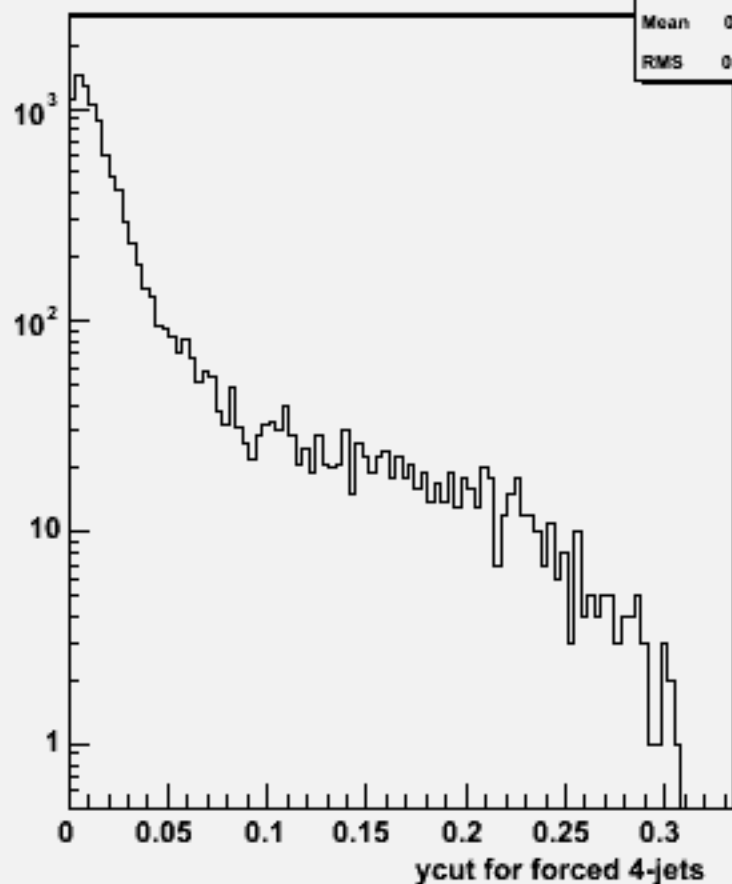
Ycut for 4-jets :w101681 uucse2n2_o
