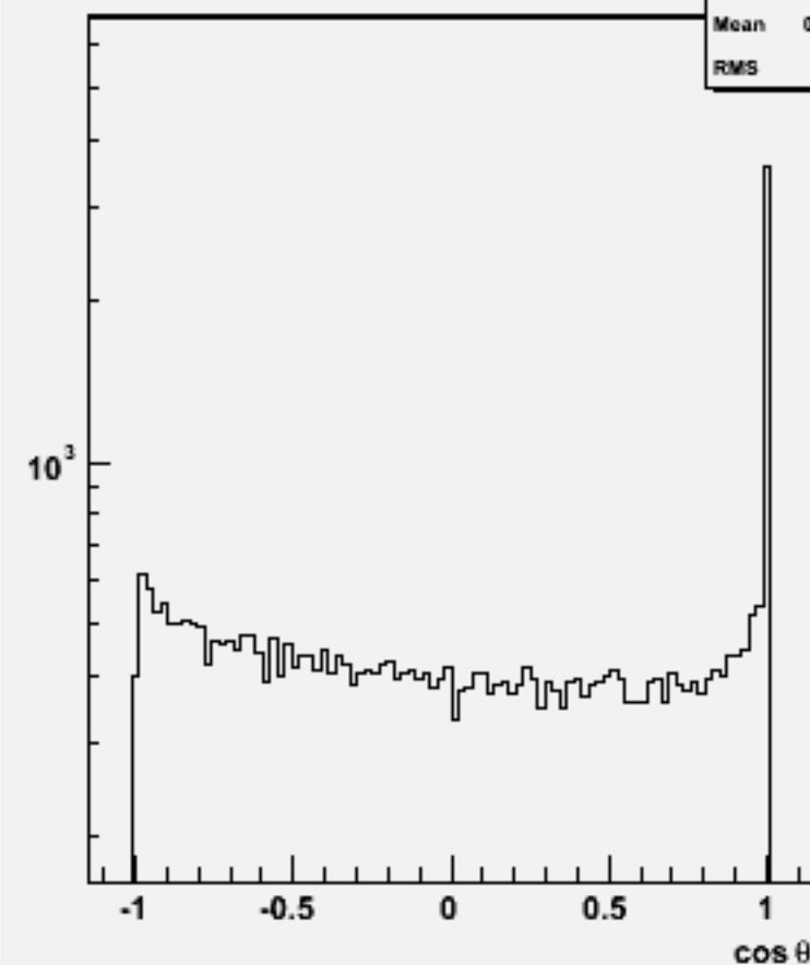
Jet cosθ (All jets)w101681 uucse2n2_o
