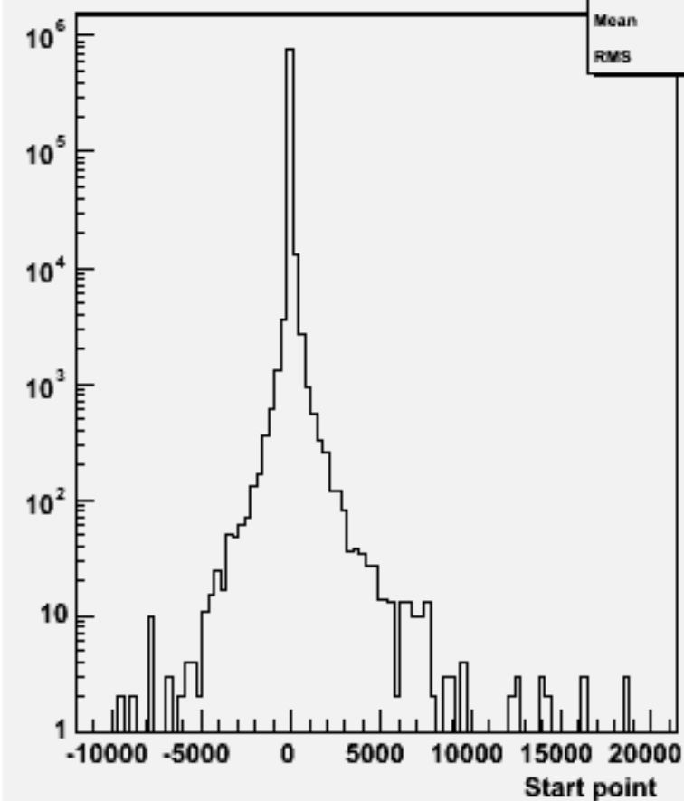
Start point Z : w101681 uucse2n2_o
