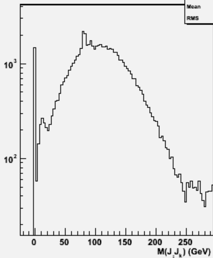
2jets mass(All comb)w101681 uucse2n2_o
