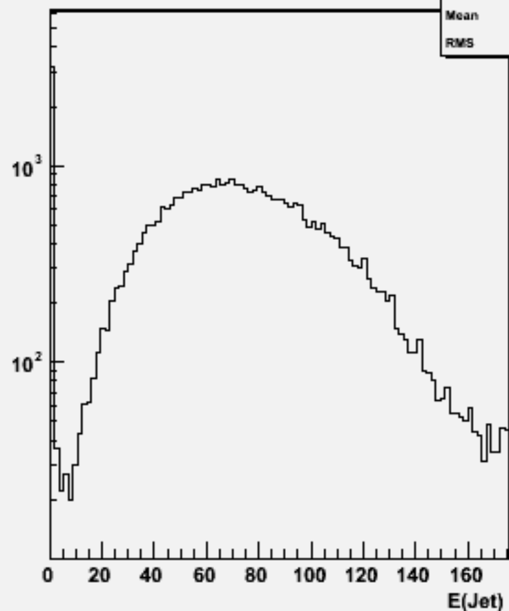
Jet energies(All jets)w101681 uucse2n2_o
