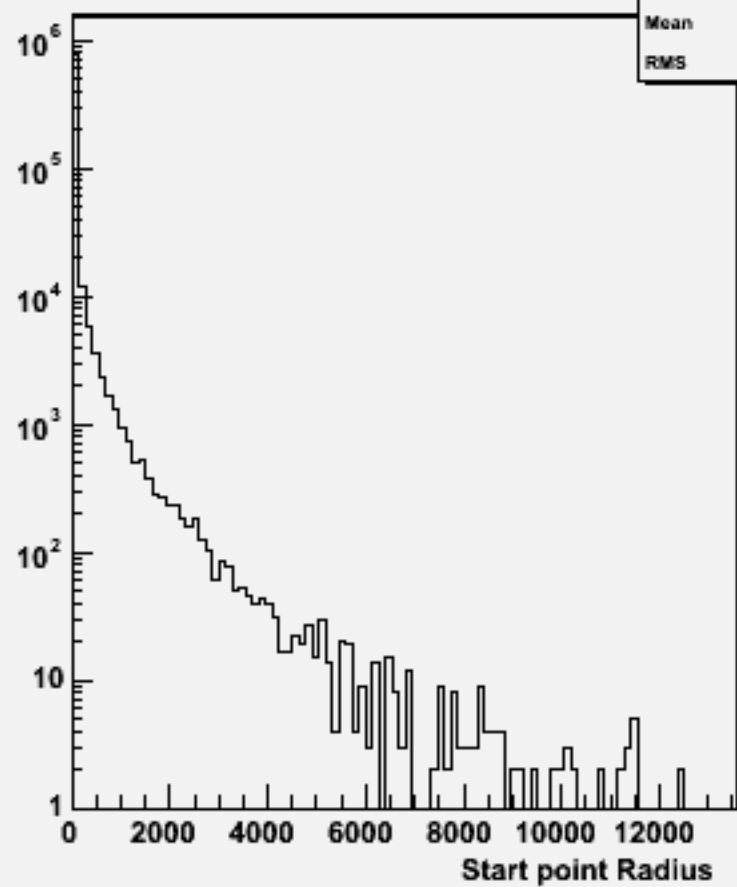
Start point R : w101680 uucse2n2_o
