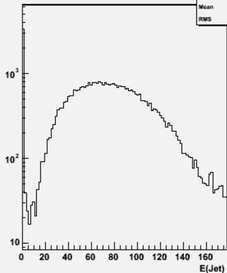
Jet energies(All jets)w101680 uucse2n2_o
