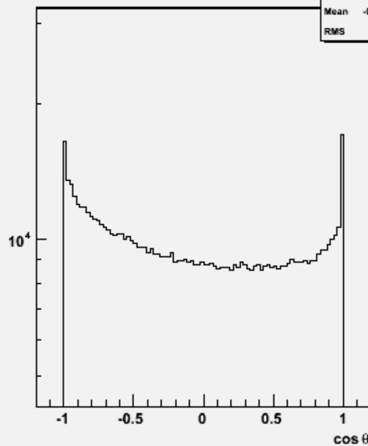
Particle cos \theta : w101680 uucse2n2_o
