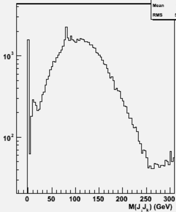
2jets mass(All comb)w101680 uucse2n2_o
