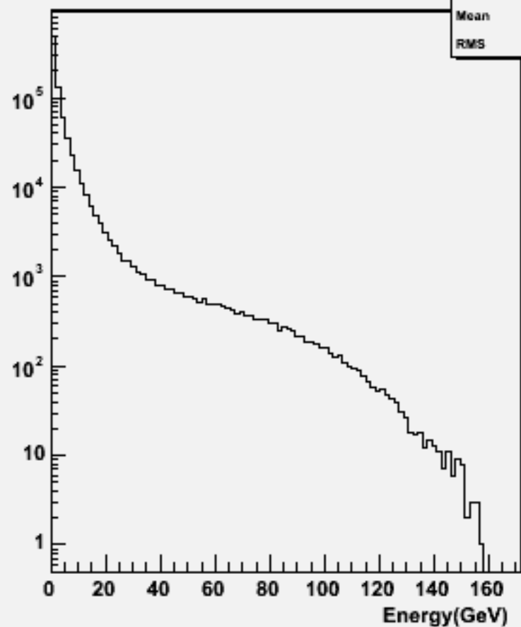
Particle Energy : w101680 uucse2n2_o
