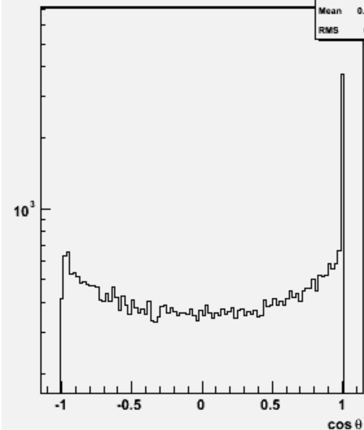
Jet cos \theta (All jets)w101680 uucse2n2_o
