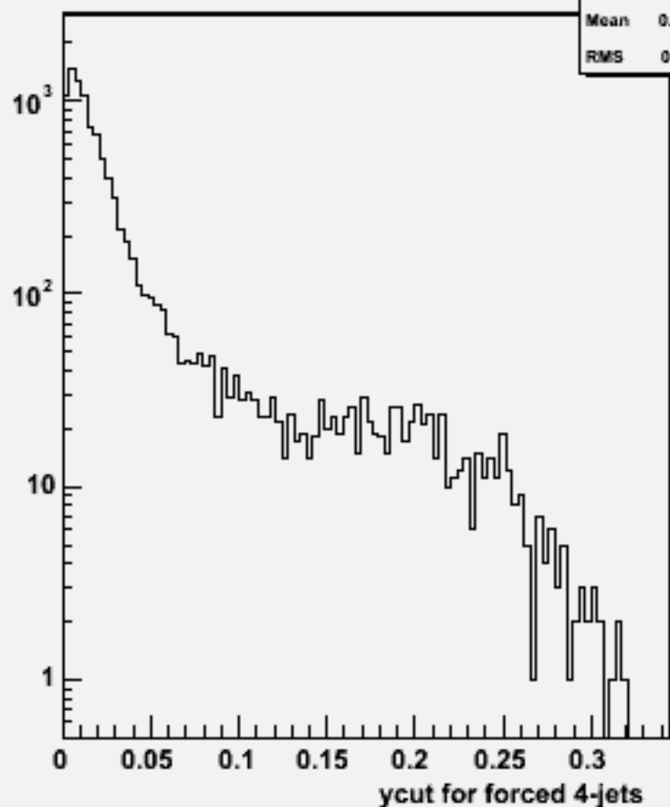
Ycut for 4-jets :w101680 uucse2n2_o
