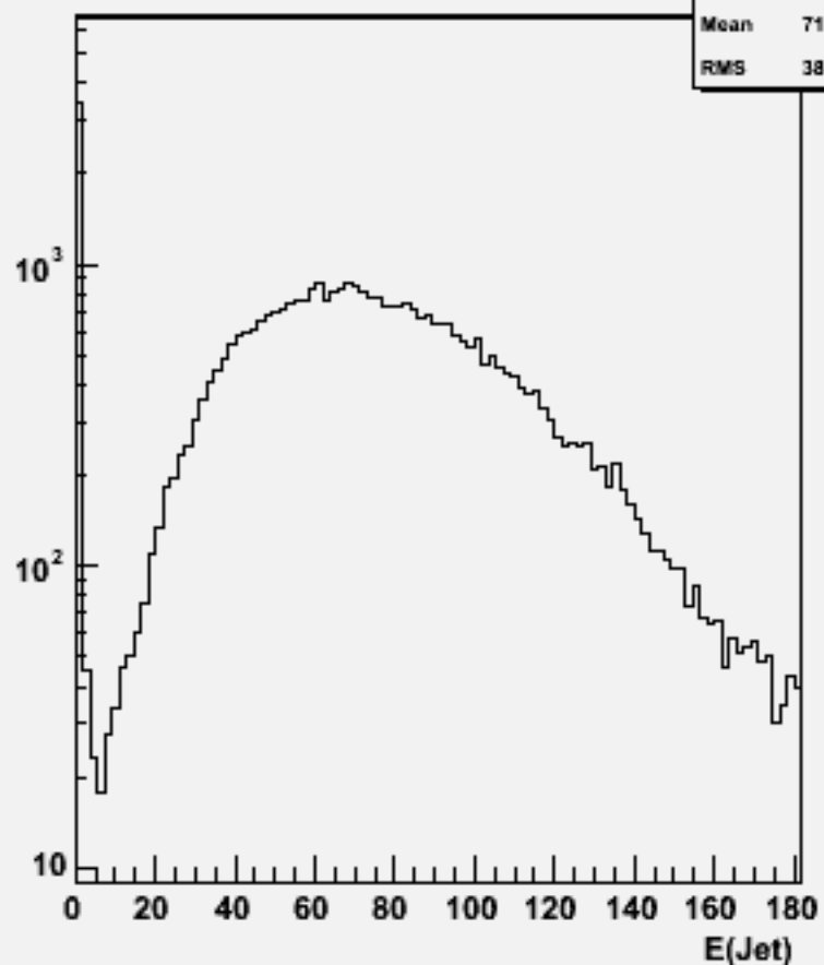
Jet energies(All jets)w101678 uucse1n1_o
