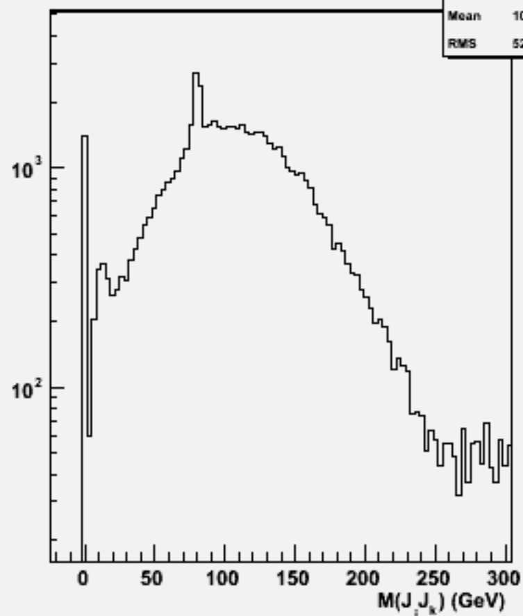
2jets mass(All comb)w101678 uucse1n1_o
