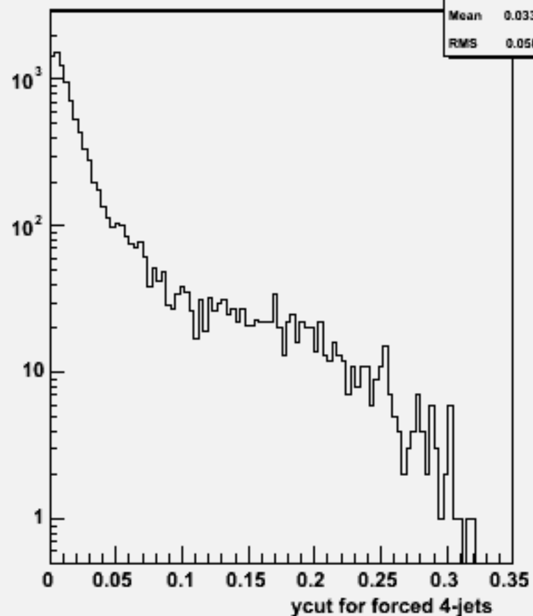
Ycut for 4-jets :w101678 uucse1n1_o
