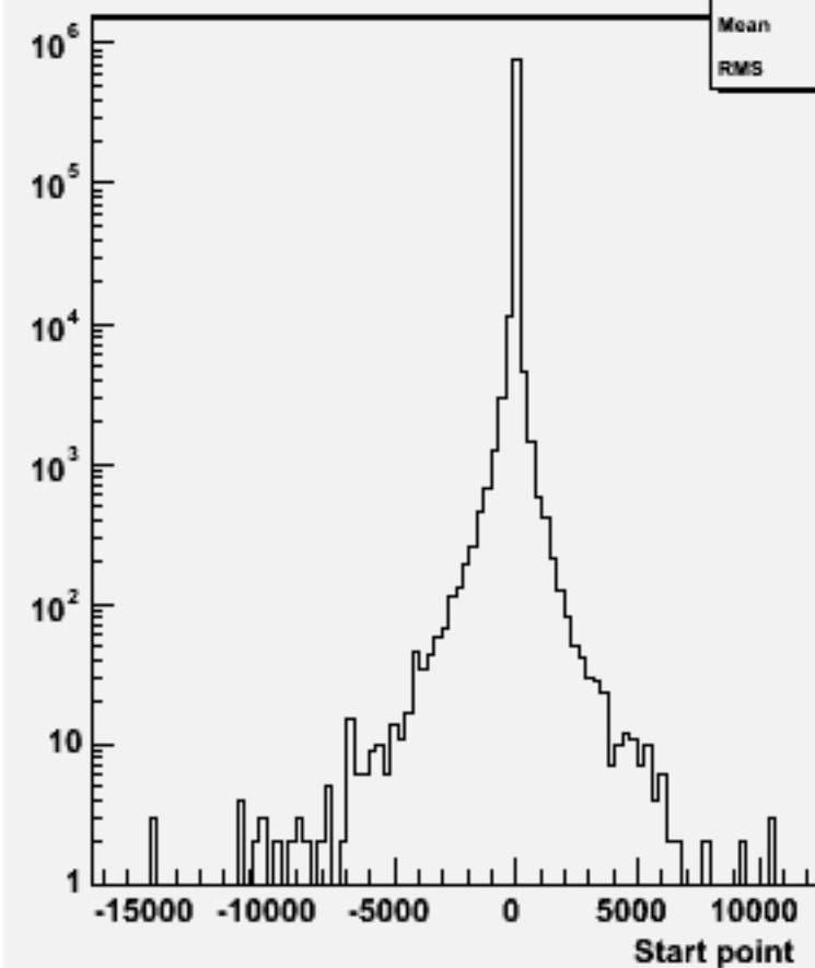
Start point Z : w101678 uucse1n1_o
