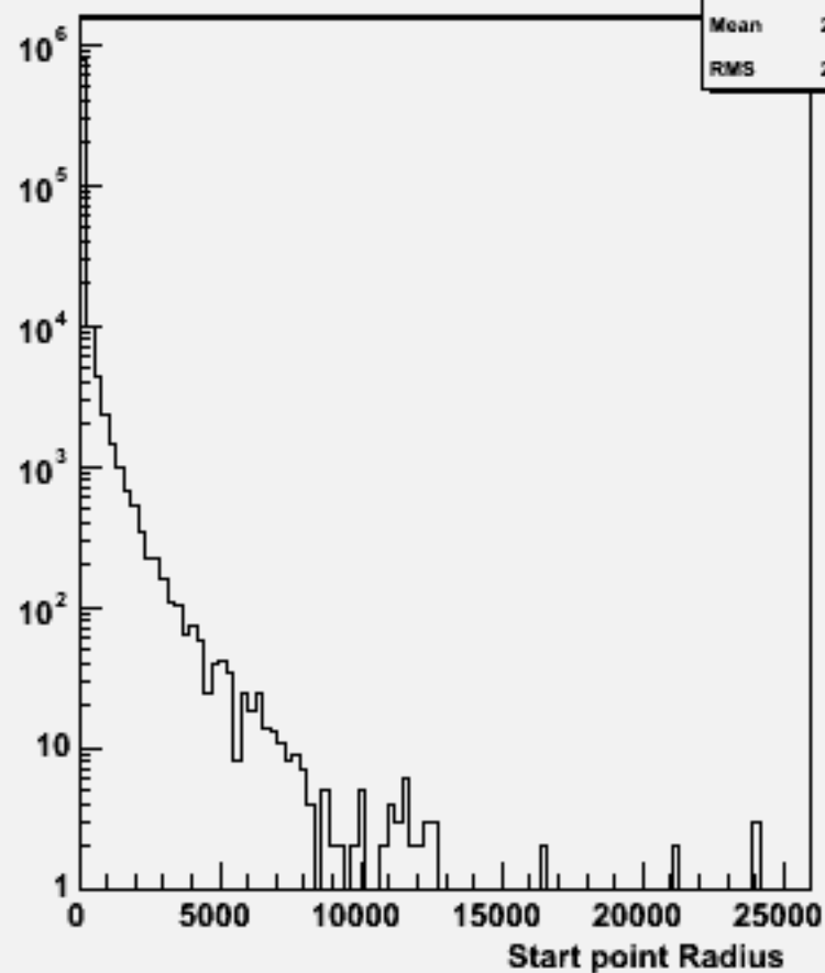
Start point R : w101678 uucse1n1_o
