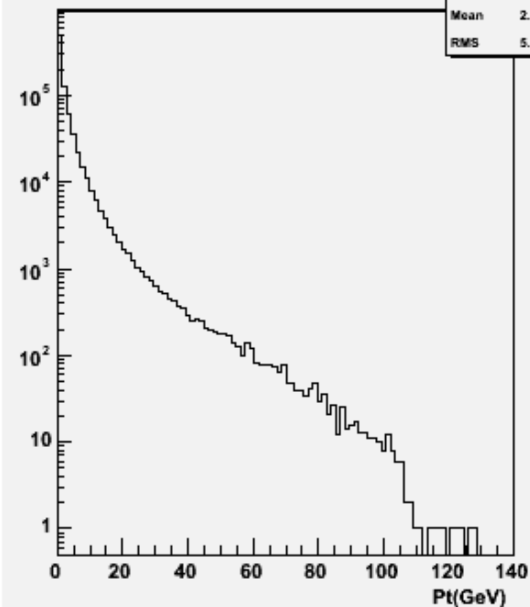
Particle Pt : w101678 uucse1n1_o
