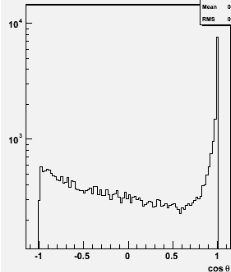
Jet cos \theta (All jets)w101678 uucse1n1_o
