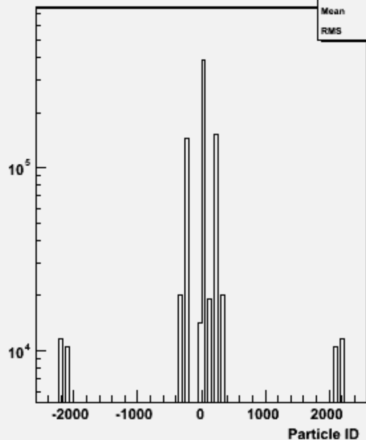
Particle ID : w101678 uucse1n1_o
