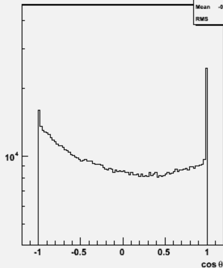
Particle cos \theta : w101678 uucse1n1_o
