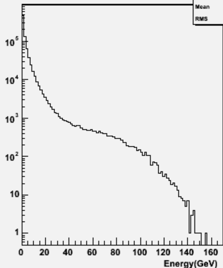
Particle Energy : w101678 uucse1n1_o
