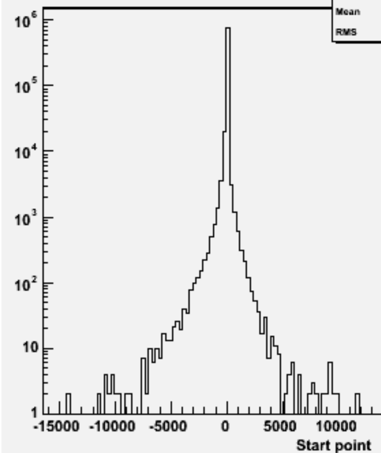
Start point Z : w101676 uucse1n1_o
