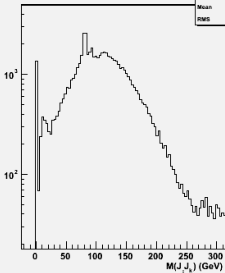
2jets mass(All comb)w101676 uucse1n1_o
