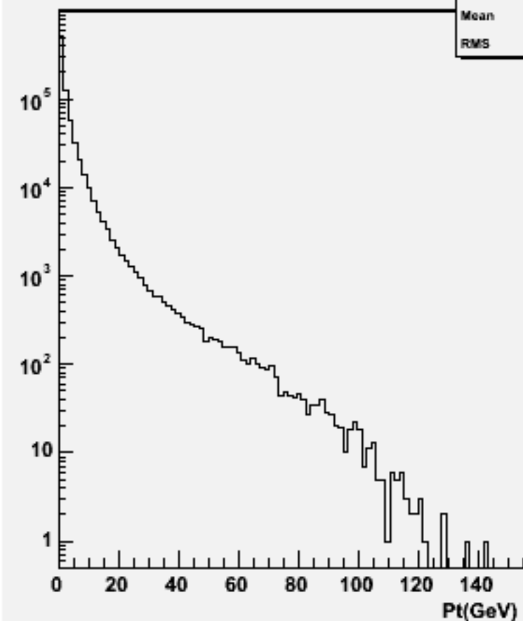
Particle Pt : w101676 uucse1n1_o
