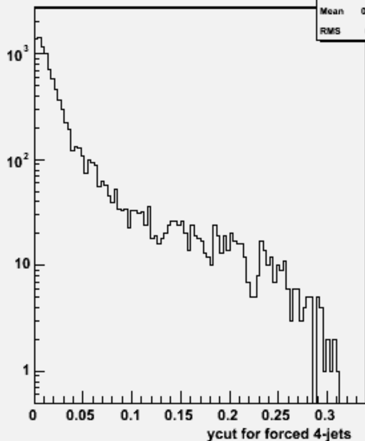
Ycut for 4-jets :w101676 uucse1n1_o
