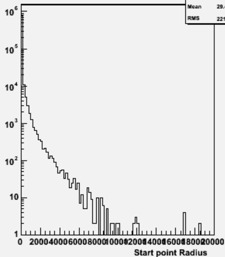
Start point R : w101676 uucse1n1_o
