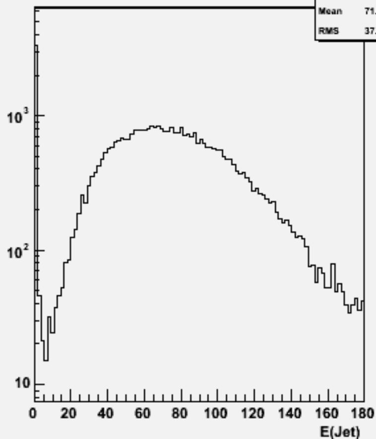
Jet energies(All jets)w101676 uucse1n1_o
