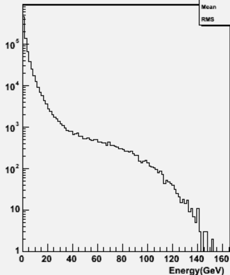
Particle Energy : w101676 uucse1n1_o
