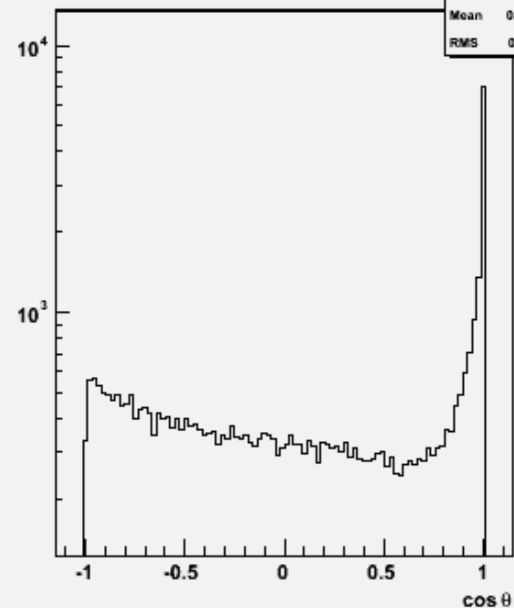
Jet cos \theta (All jets)w101676 uucse1n1_o
