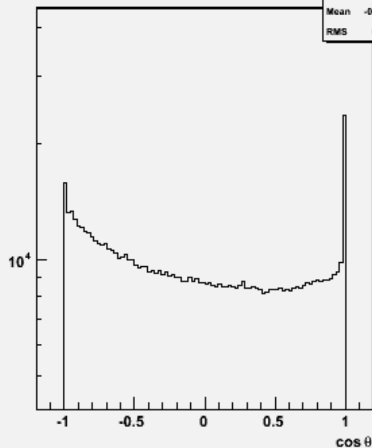
Particle cos \theta : w101676 uucse1n1_o
