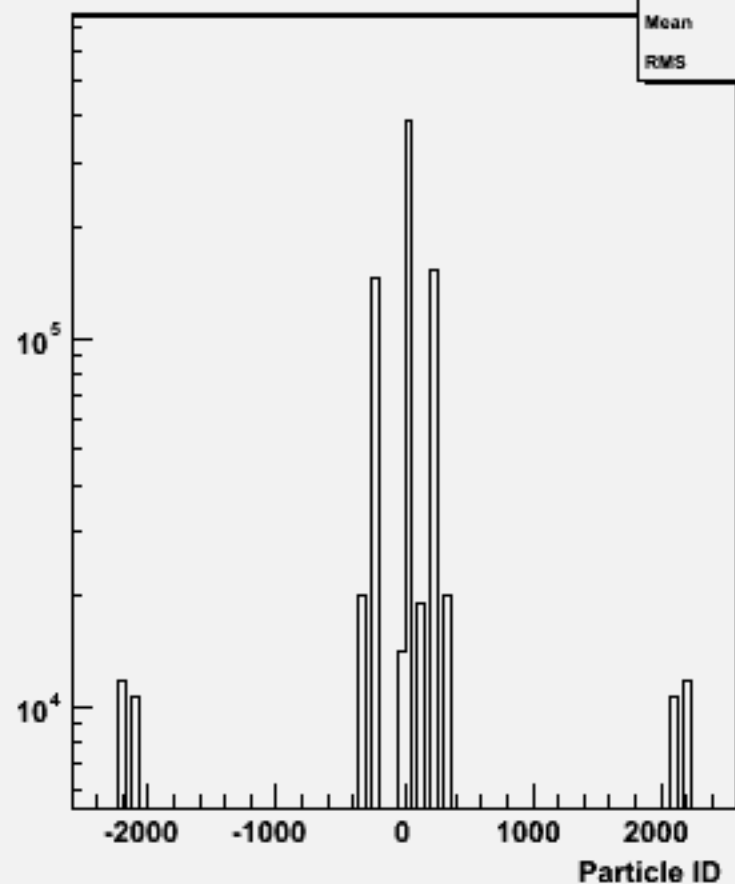
Particle ID : w101676 uucse1n1_o
