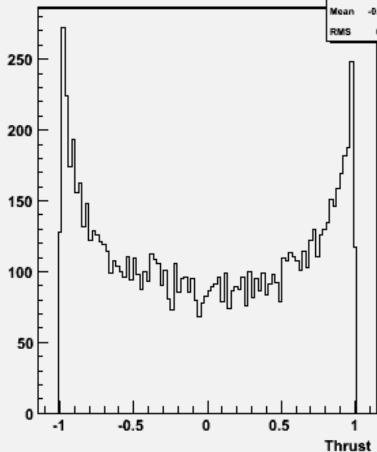
cos \Theta (thrust) w101672 uuudsc_o
