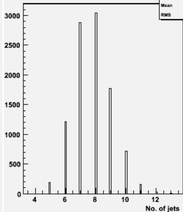
No. jets (ycut=0.001) : w101672 uuudsc_o
