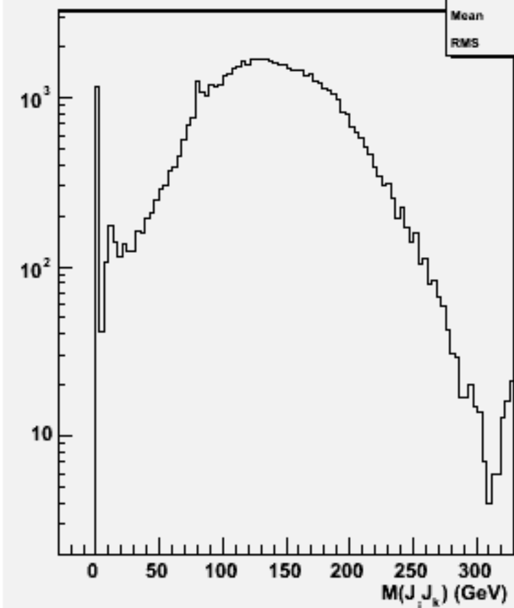
2jets mass(All comb)w101672 uuudsc_o
