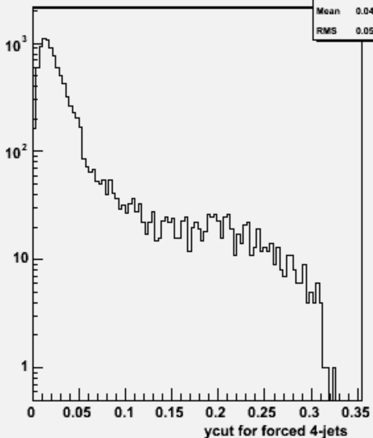
Ycut for 4-jets :w101672 uuudsc_o
