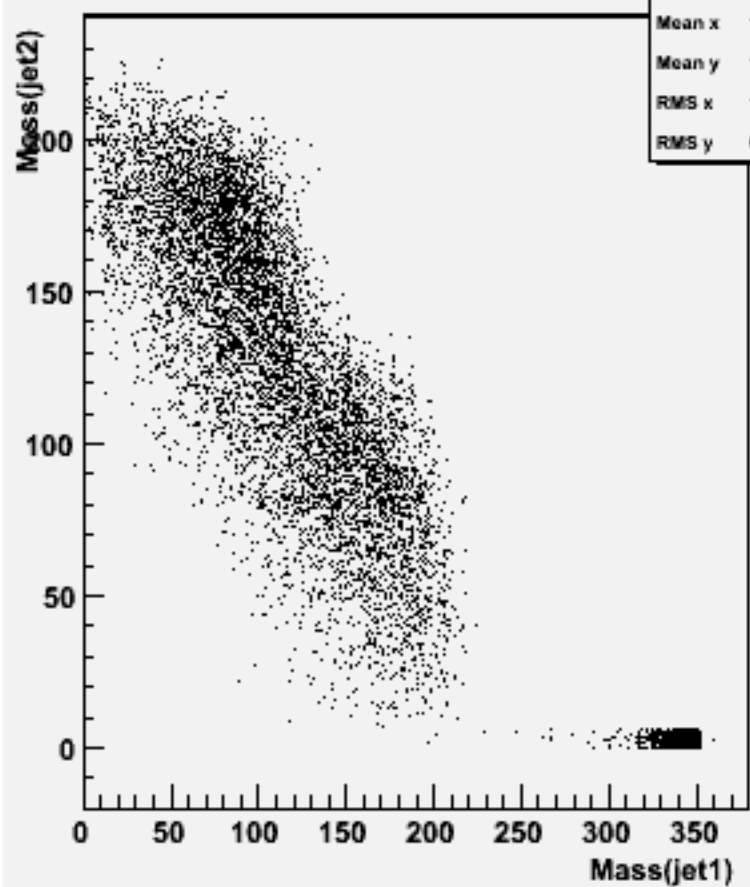
Jet mass for forced 2-jets : w101672 uuudsc_o
