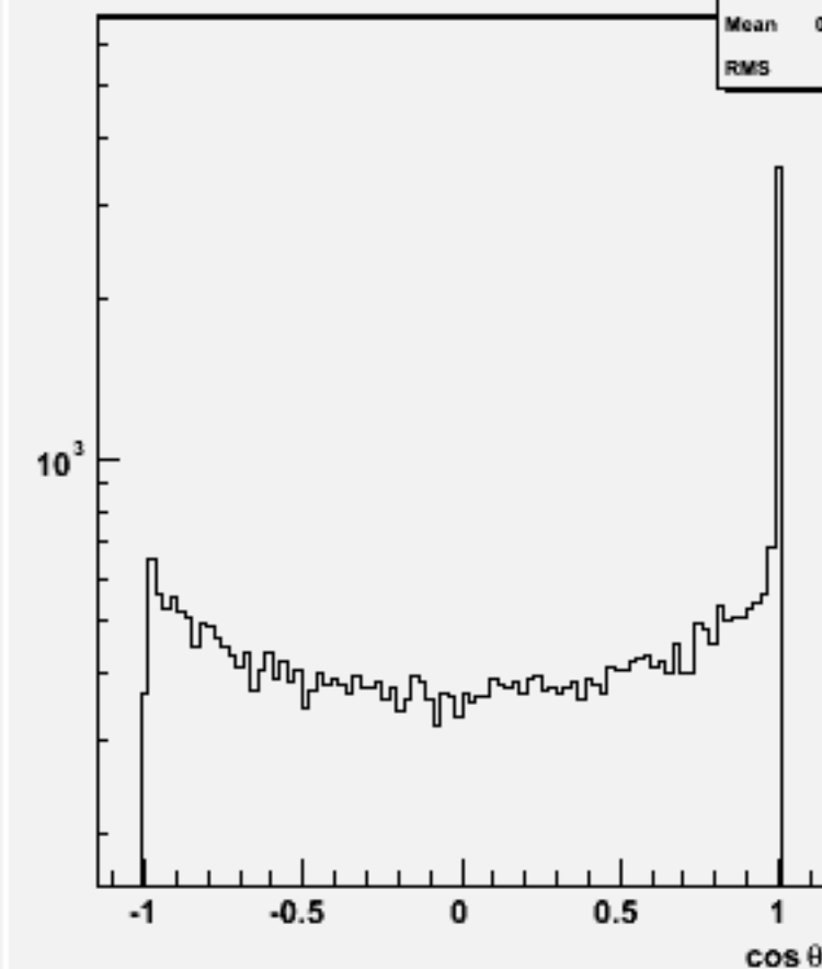
Jet cos \theta (All jets)w101672 uuudsc_o
