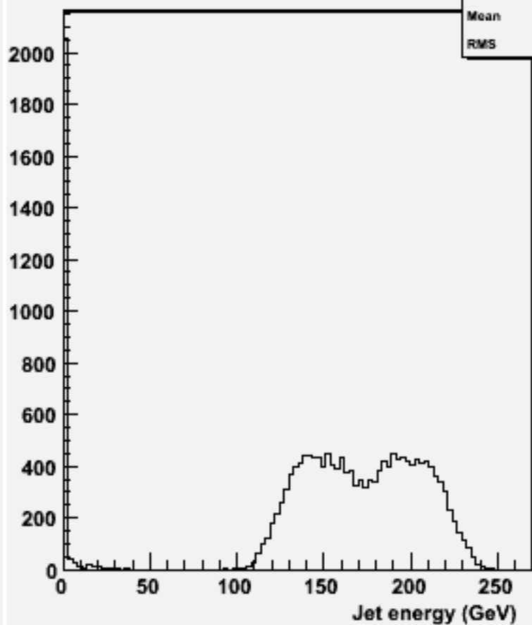
energy for 2-jets :w101672 uuudsc_o
