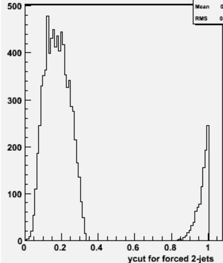
Ycut for 2-jets :w101672 uuudsc_o
