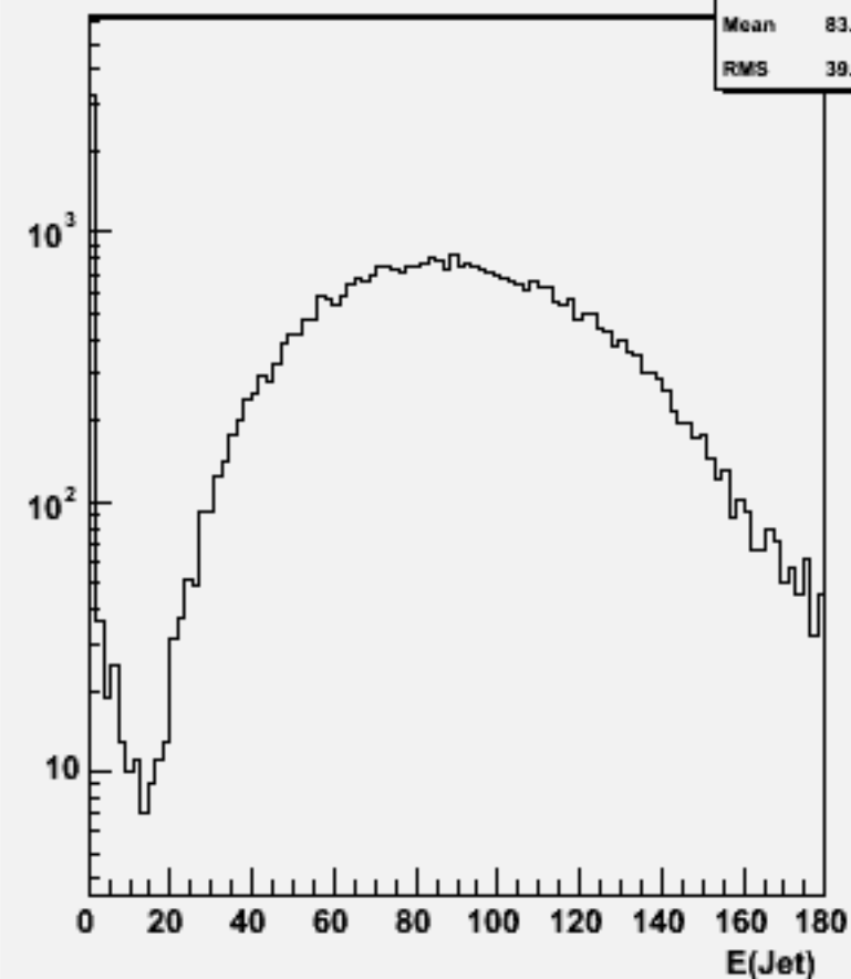
Jet energies(All jets)w101668 uuuddu_o
