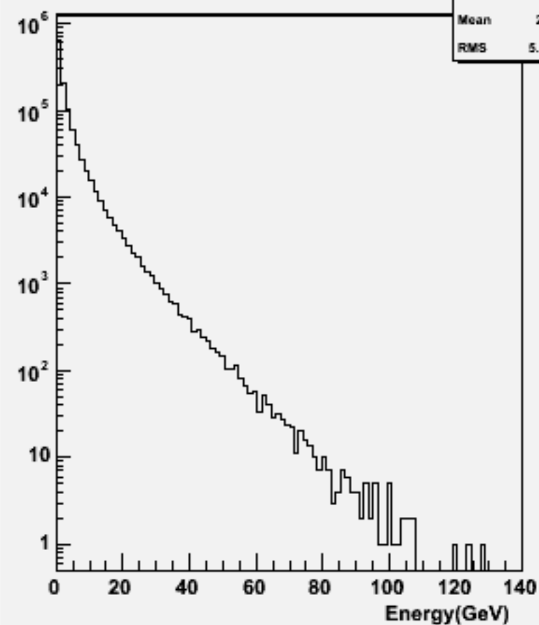
Particle Energy : w101668 uuuddu_o
