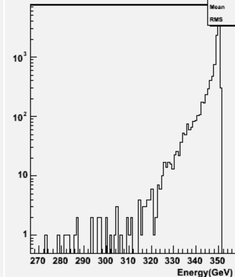
Total Energy (w/o \nu ): w101668 uuuddu_o
