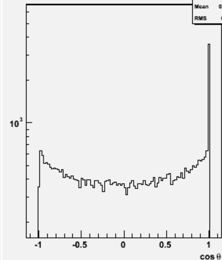
Jet cos \theta (All jets)w101668 uuuddu_o
