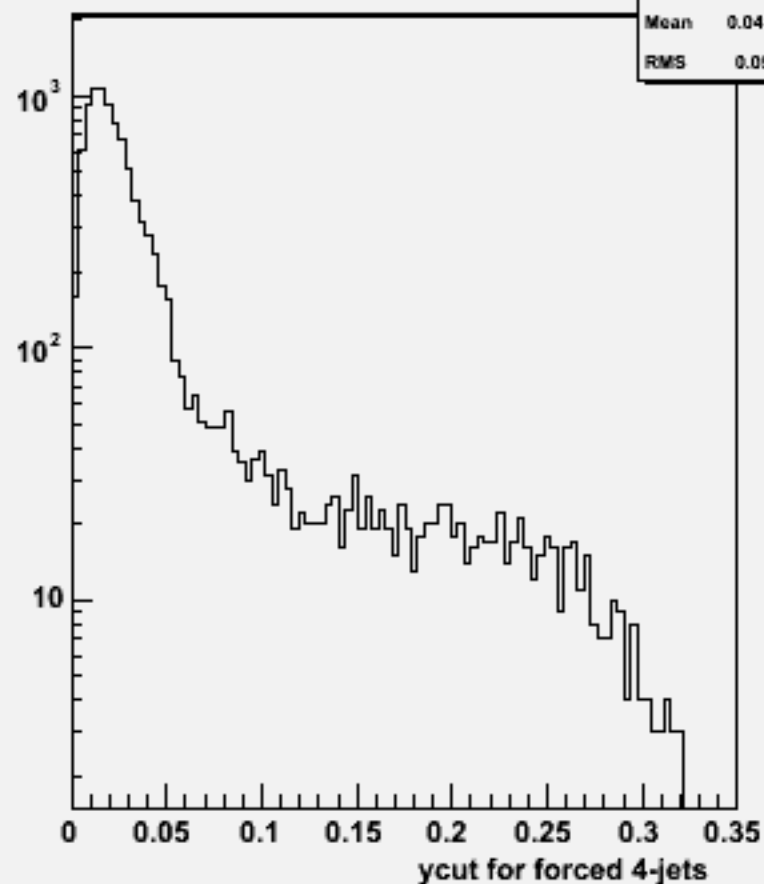
Ycut for 4-jets :w101668 uuuddu_o
