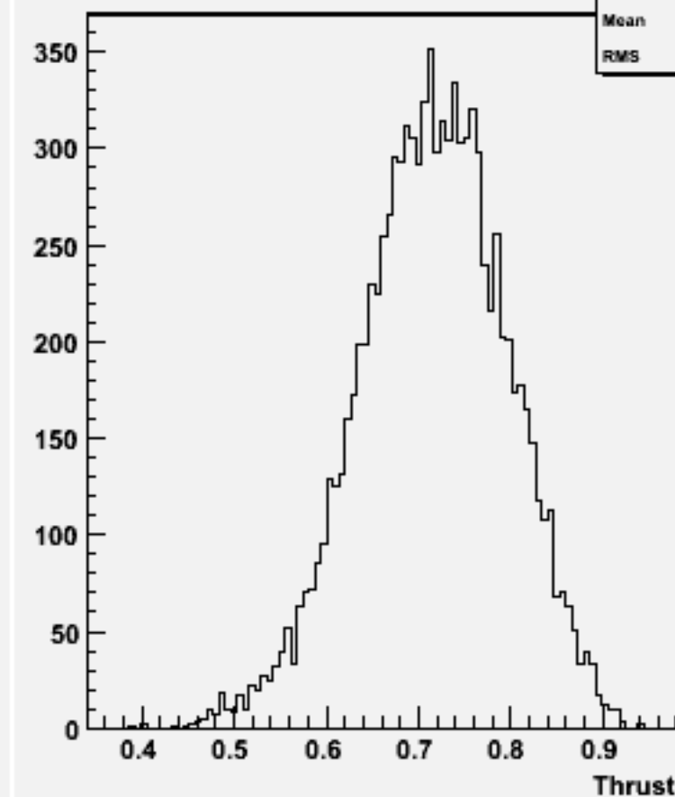
Thrust w101668 uuuddu_o
