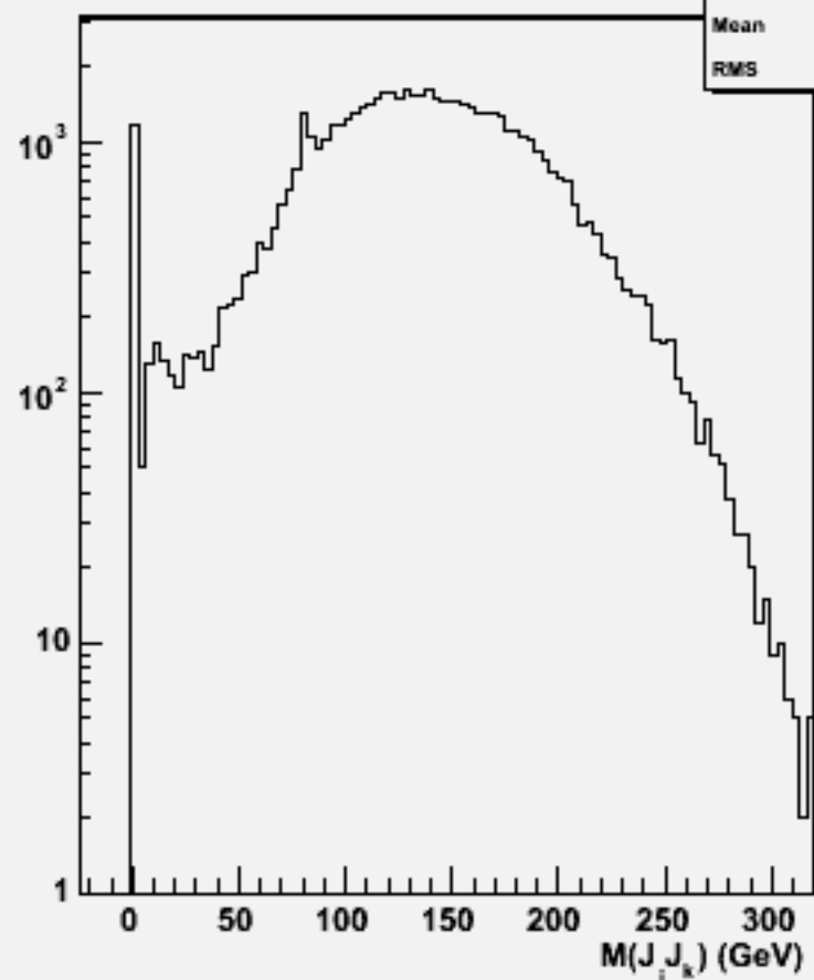
2jets mass(All comb)w101668 uuuddu_o
