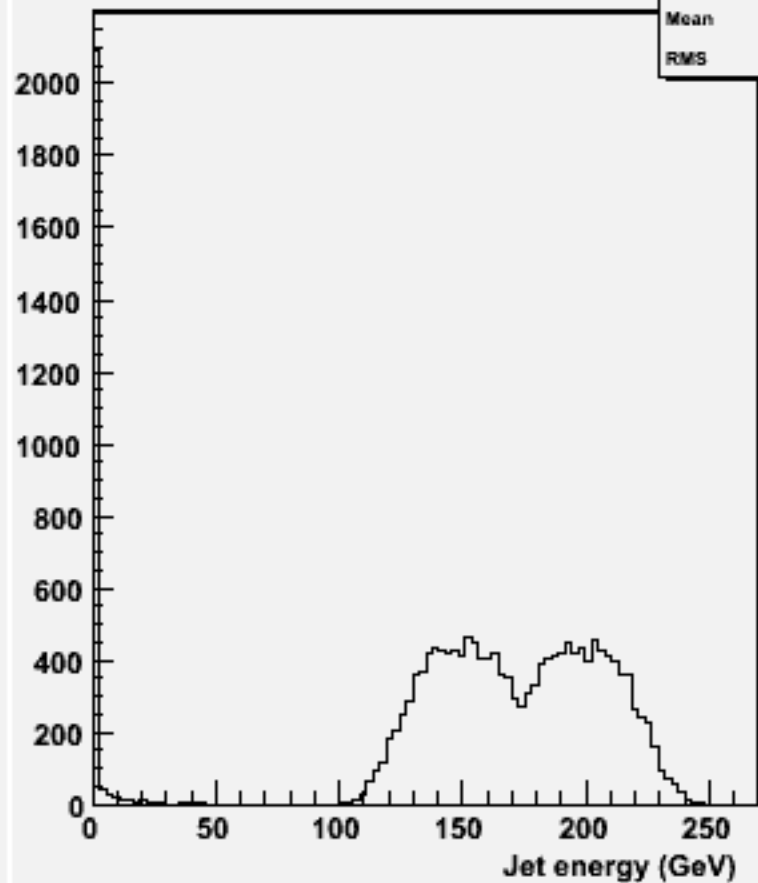
energy for 2-jets :w101668 uuuddu_o
