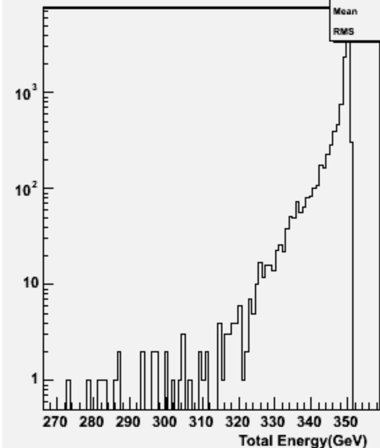
Total Energy (inc. \nu ): w101668 uuuddu_o
