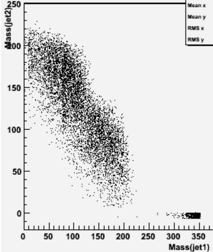
Jet mass for forced 2-jets : w101668 uuuddu_o
