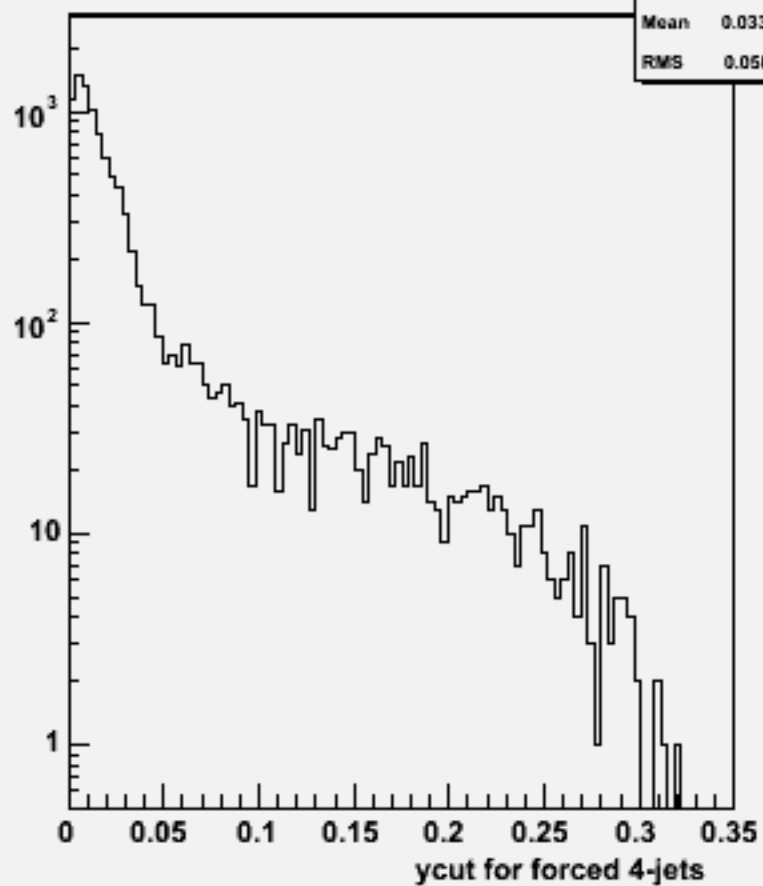
Ycut for 4-jets :w101657 uuude1n1_o
