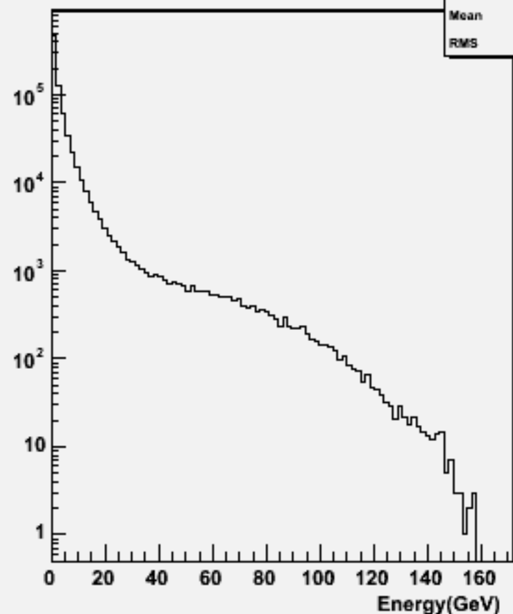
Particle Energy : w101657 uuude1n1_o
