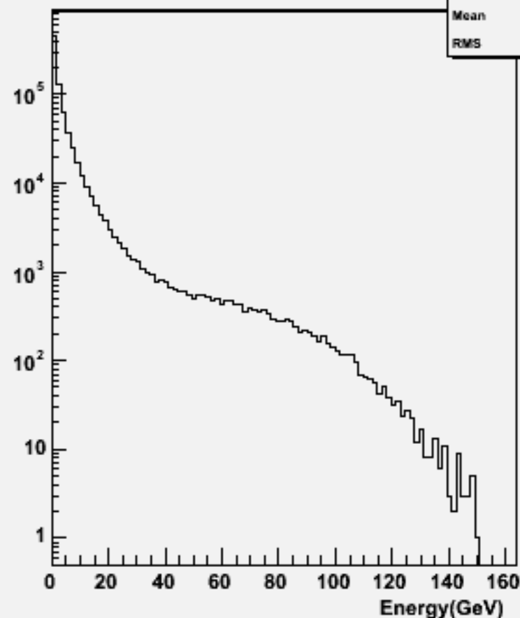
Particle Energy : w101656 uuude1n1_o
