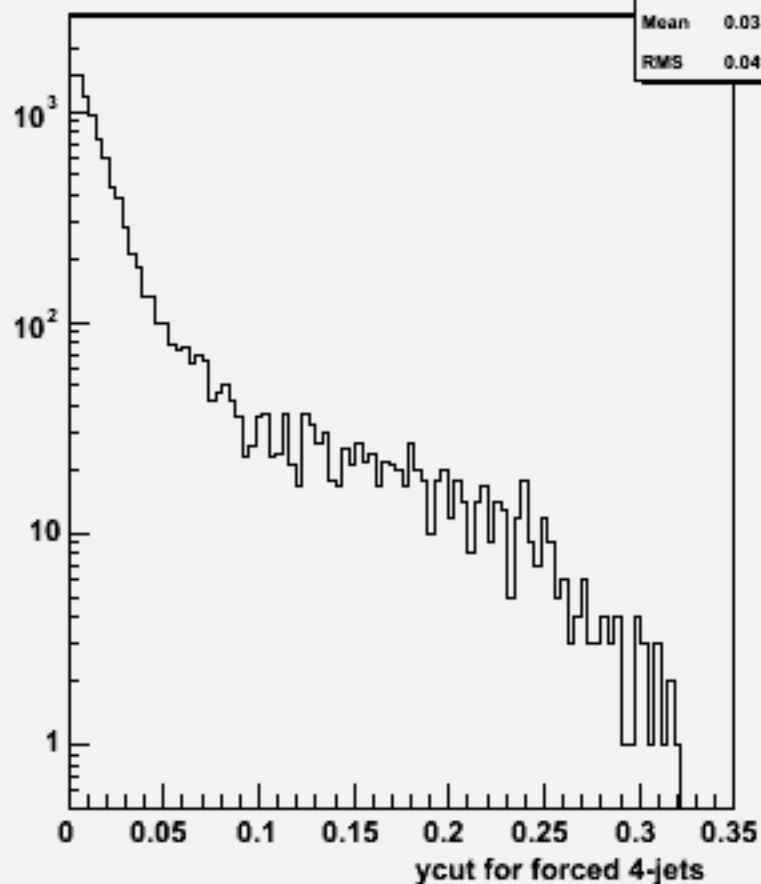
Ycut for 4-jets :w101656 uuude1n1_o
