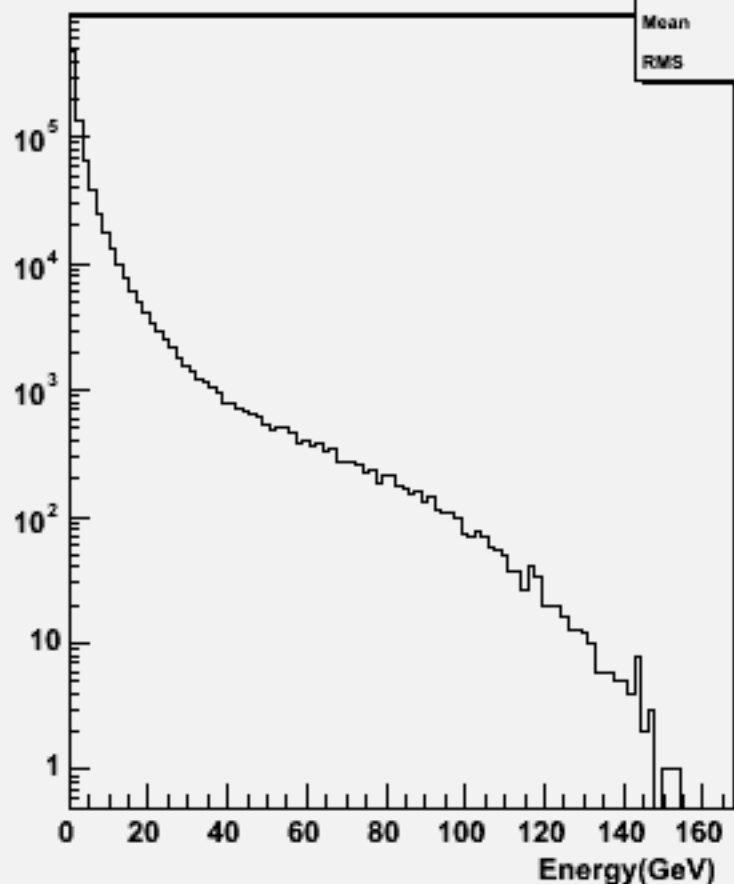
Particle Energy : w101653 uun3e3sc_o
