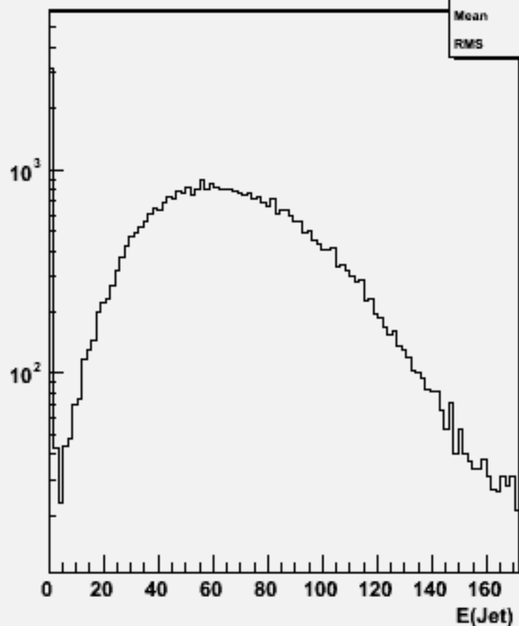
Jet energies(All jets)w101653 uun3e3sc_o
