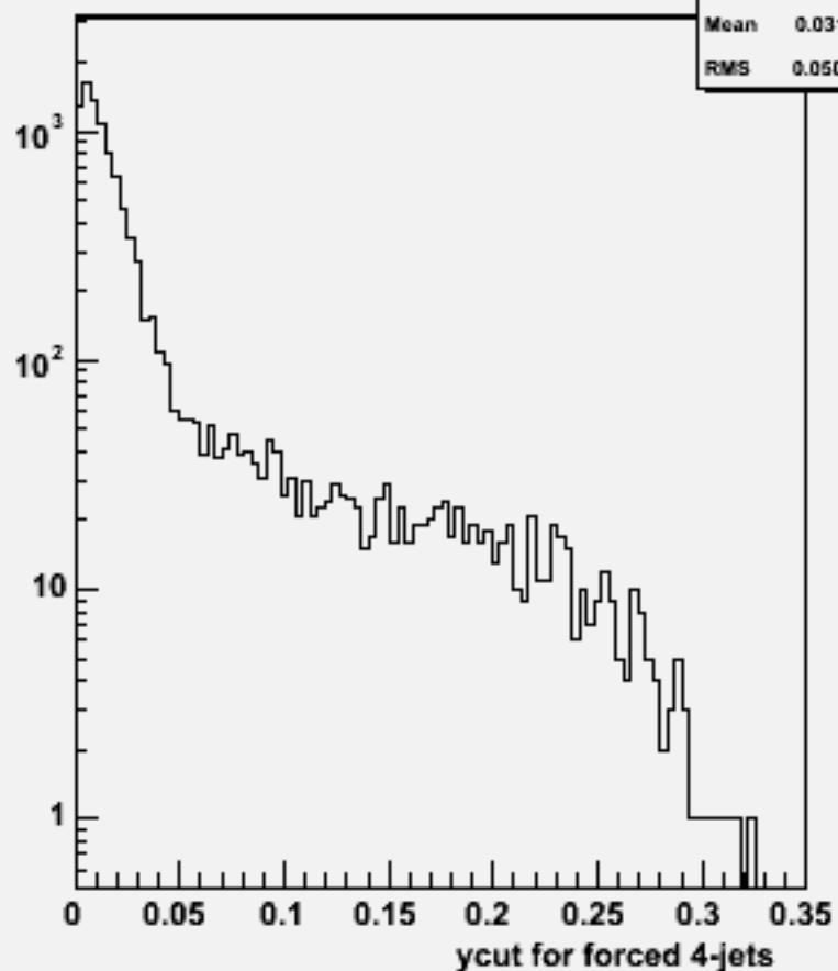
Ycut for 4-jets :w101653 uun3e3sc_o
