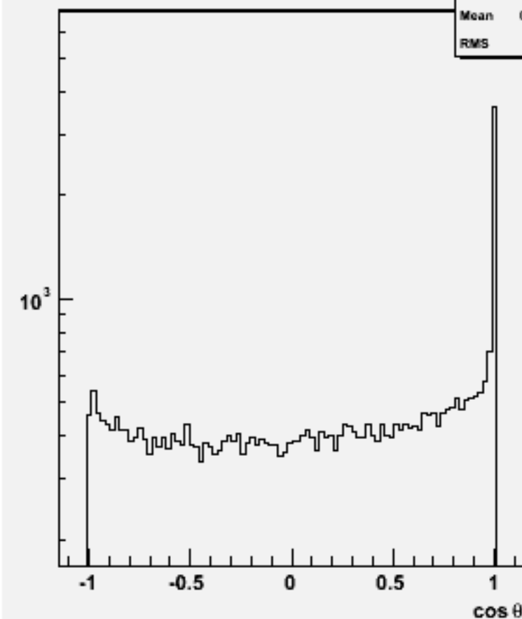
Jet cosθ (All jets)w101653 uun3e3sc_o
