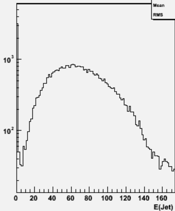
Jet energies(All jets)w101652 uun3e3sc_o
