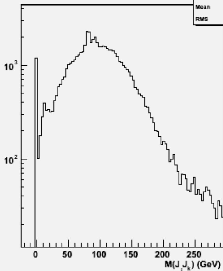
2jets mass(All comb)w101652 uun3e3sc_o
