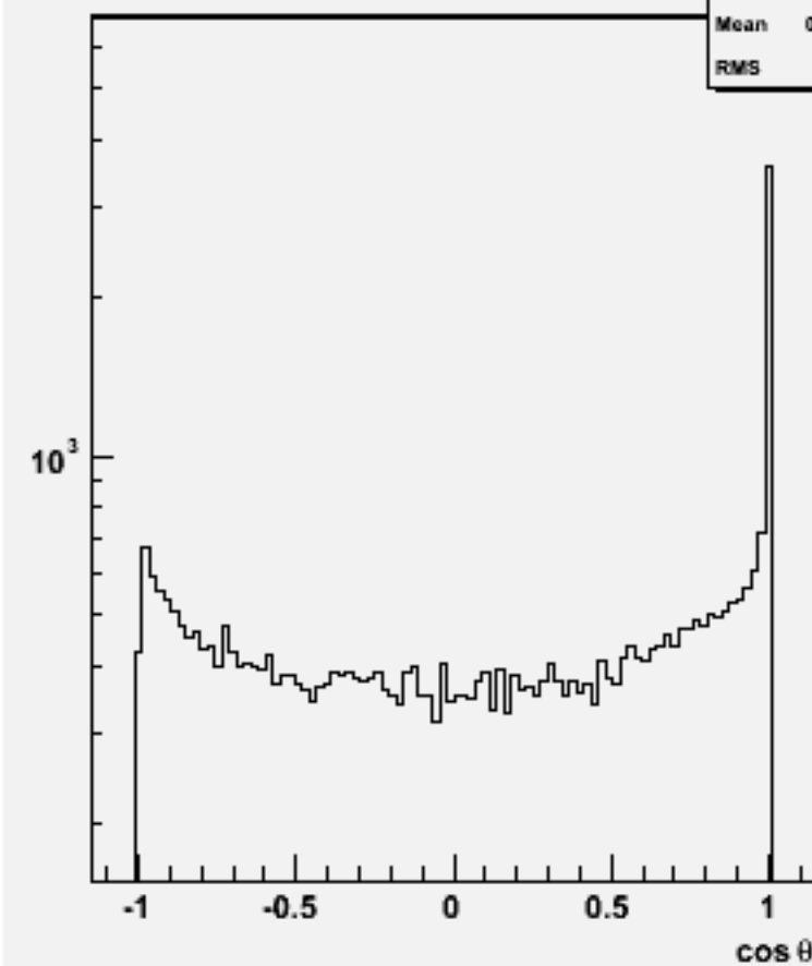
Jet cos \theta (All jets)w101652 uun3e3sc_o
