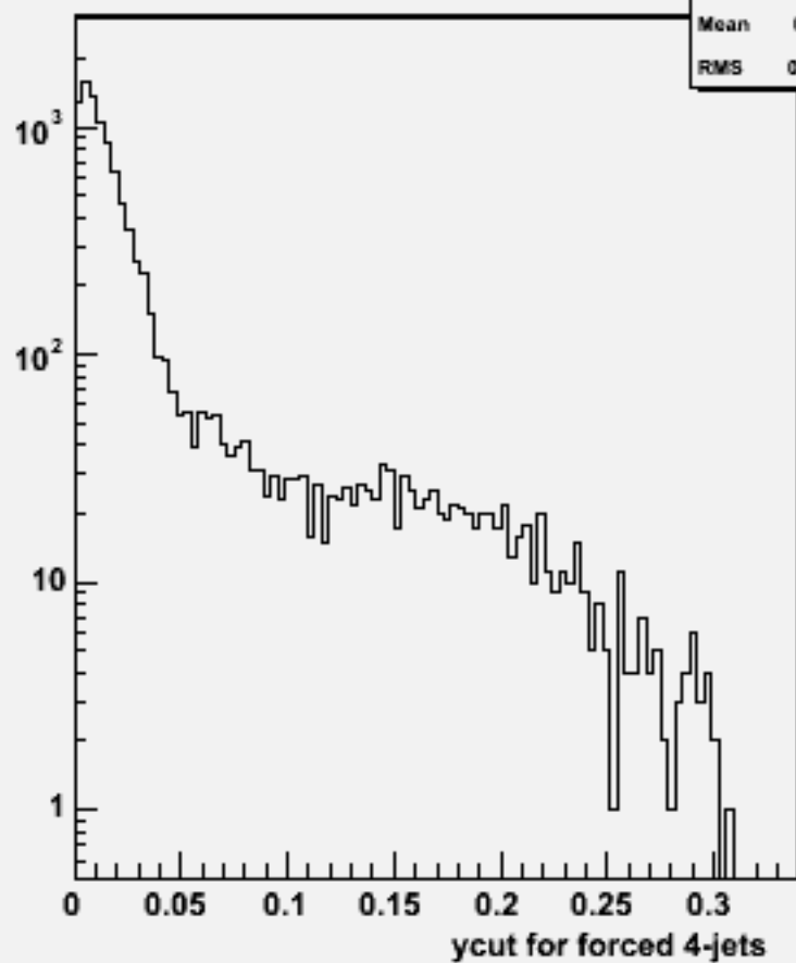
Ycut for 4-jets :w101652 uun3e3sc_o
