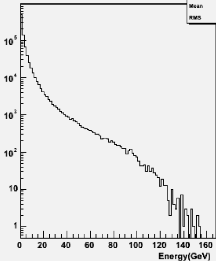
Particle Energy : w101652 uun3e3sc_o
