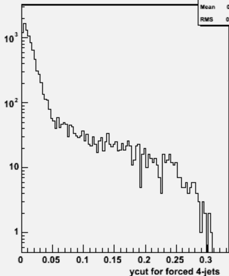
Ycut for 4-jets :w101648 uun3e3du_o
