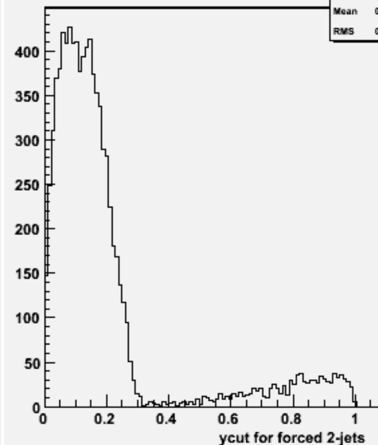
Ycut for 2-jets :w101641 uun3e3e2n2_o
