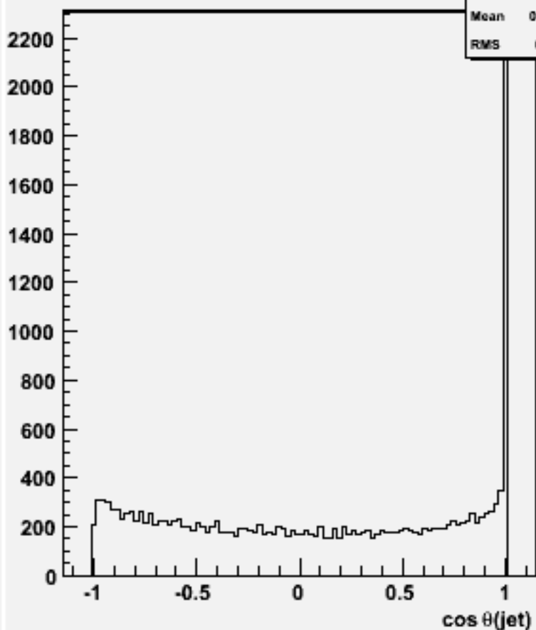
cos \theta for 2-jets :w101641 uun3e3e2n2_o
