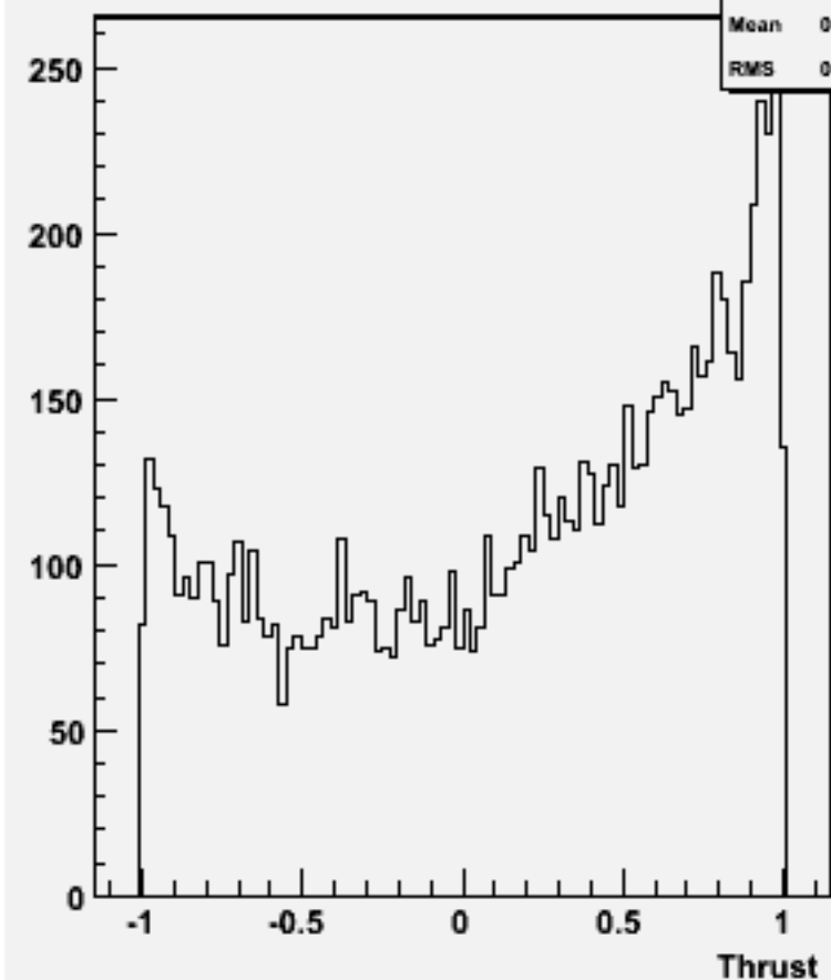
cos \Theta (thrust) w101641 uun3e3e2n2_o
