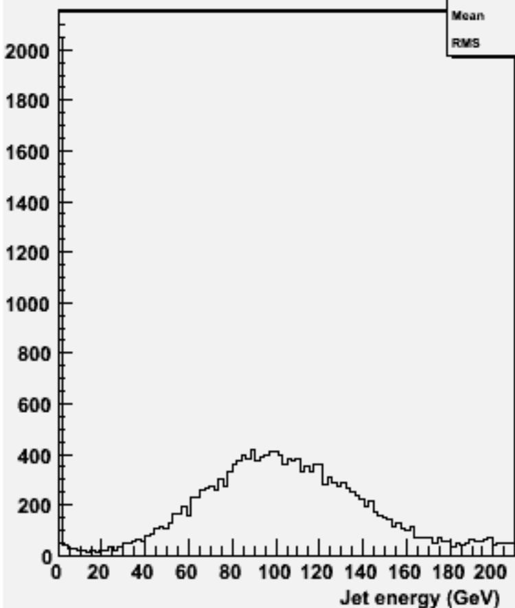
energy for 2-jets :w101641 uun3e3e2n2_o
