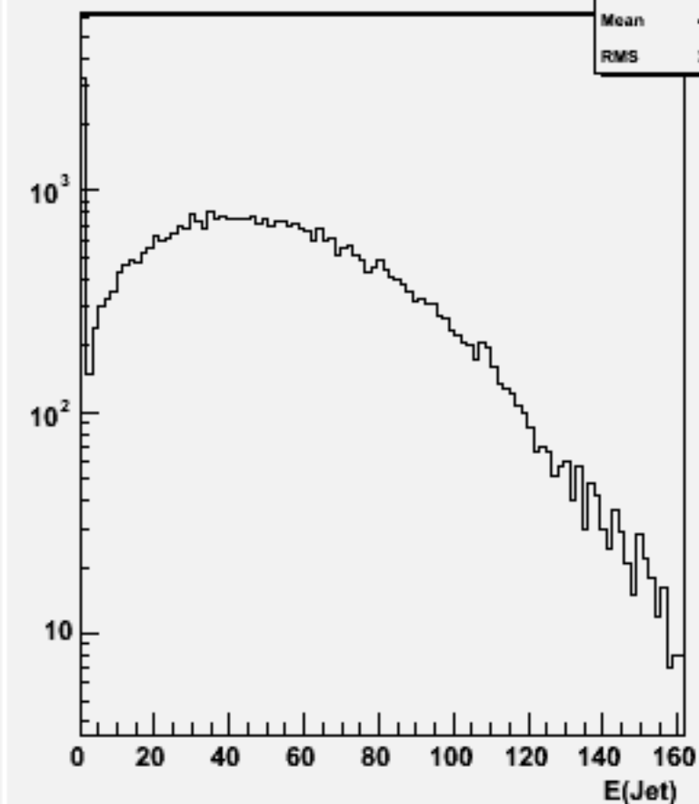
Jet energies(All jets)w101641 uun3e3e2n2_o
