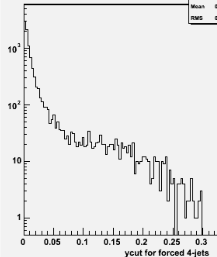
Ycut for 4-jets :w101641 uun3e3e2n2_o
