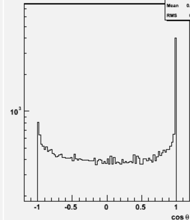
Jet cos \theta (All jets)w101641 uun3e3e2n2_o
