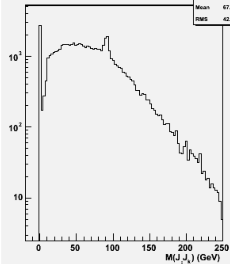
2jets mass(All comb)w101641 uun3e3e2n2_o
