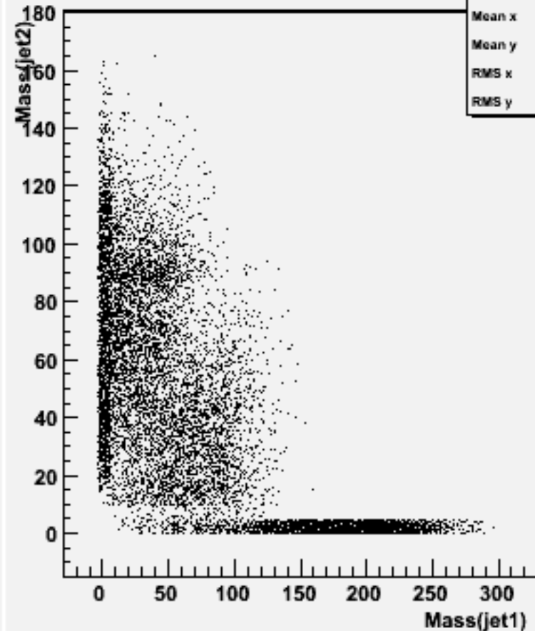
Jet mass for forced 2-jets : w101641 uun3e3e2n2_o
