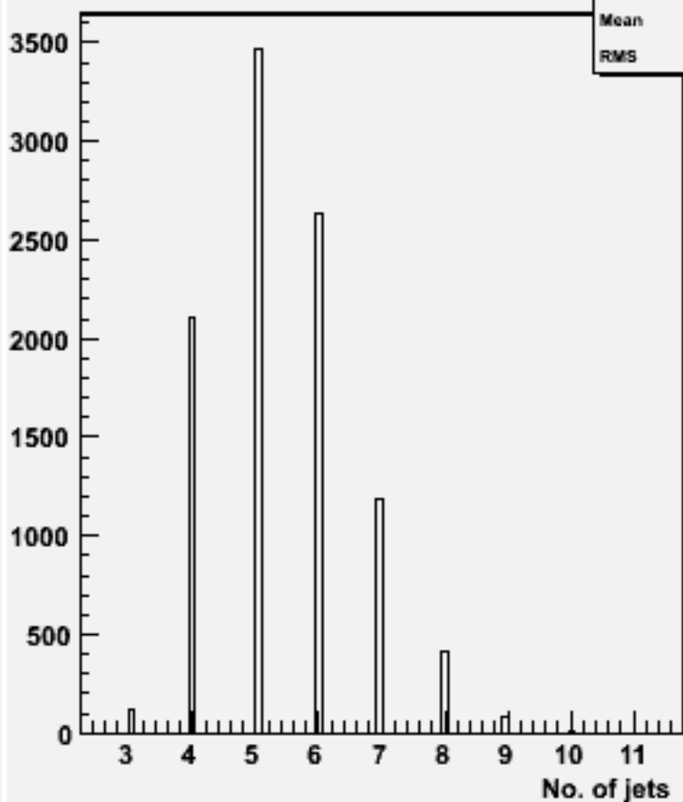
No. jets (ycut=0.001) : w101641 uun3e3e2n2_o
