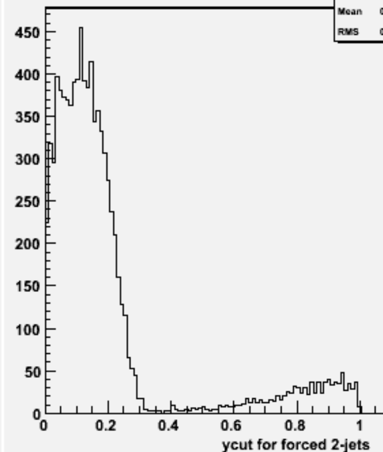
Ycut for 2-jets :w101640 uun3e3e2n2_o
