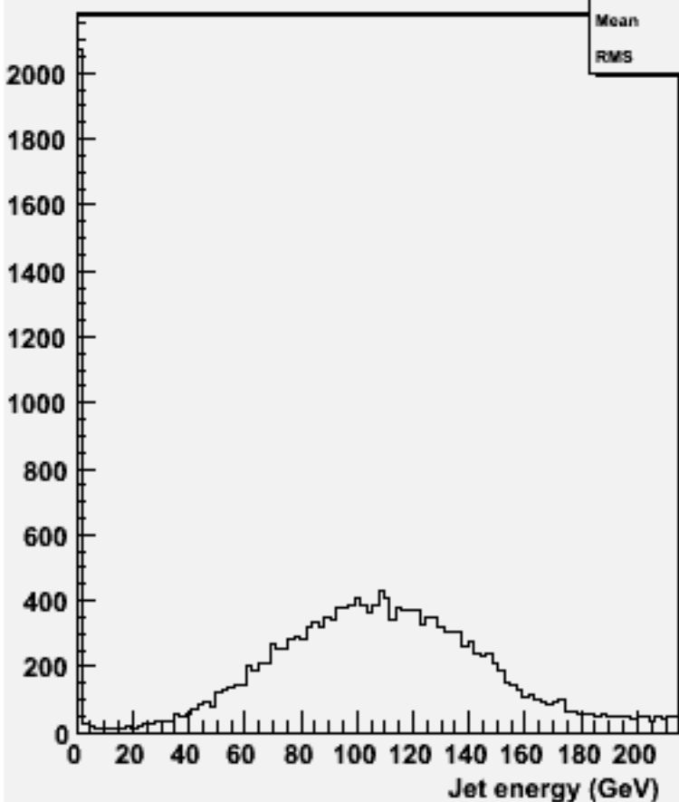
energy for 2-jets :w101640 uun3e3e2n2_o
