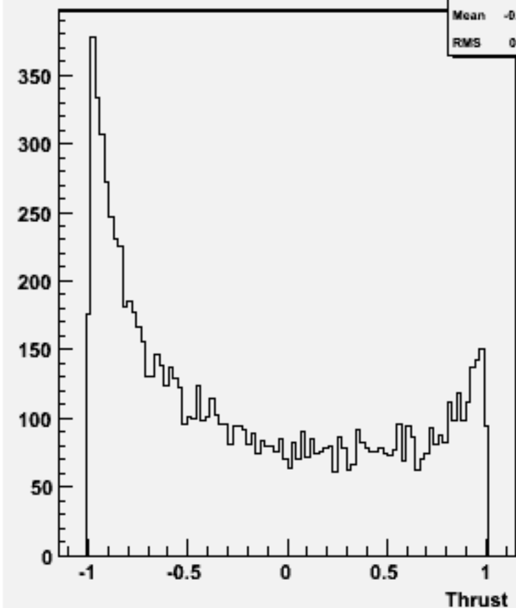
cos \Theta (thrust) w101640 uun3e3e2n2_o
