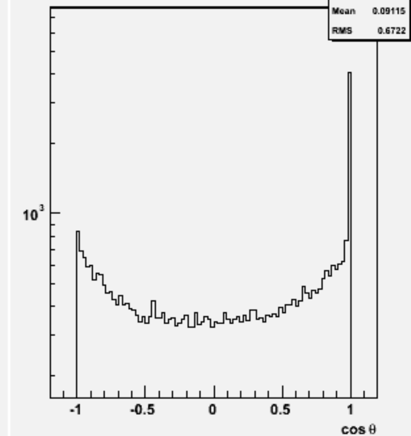
Jet cos \theta (All jets)w101640 uun3e3e2n2_o
