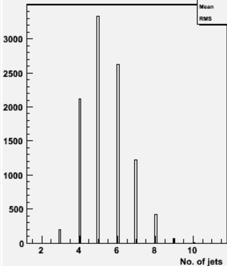
No. jets (ycut=0.001) : w101640 uun3e3e2n2_o
