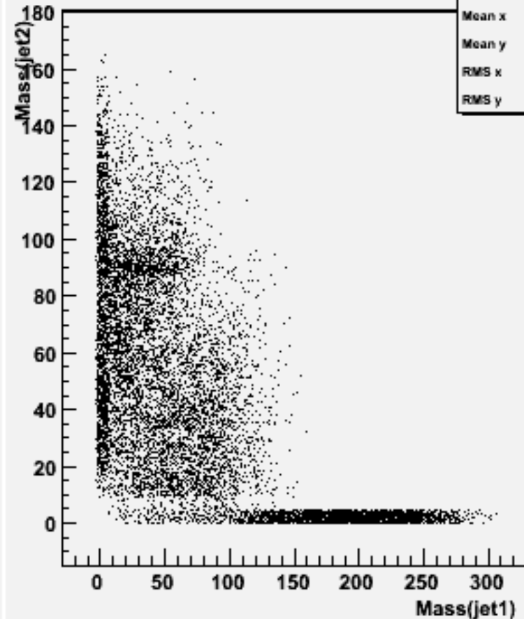
Jet mass for forced 2-jets : w101640 uun3e3e2n2_o
