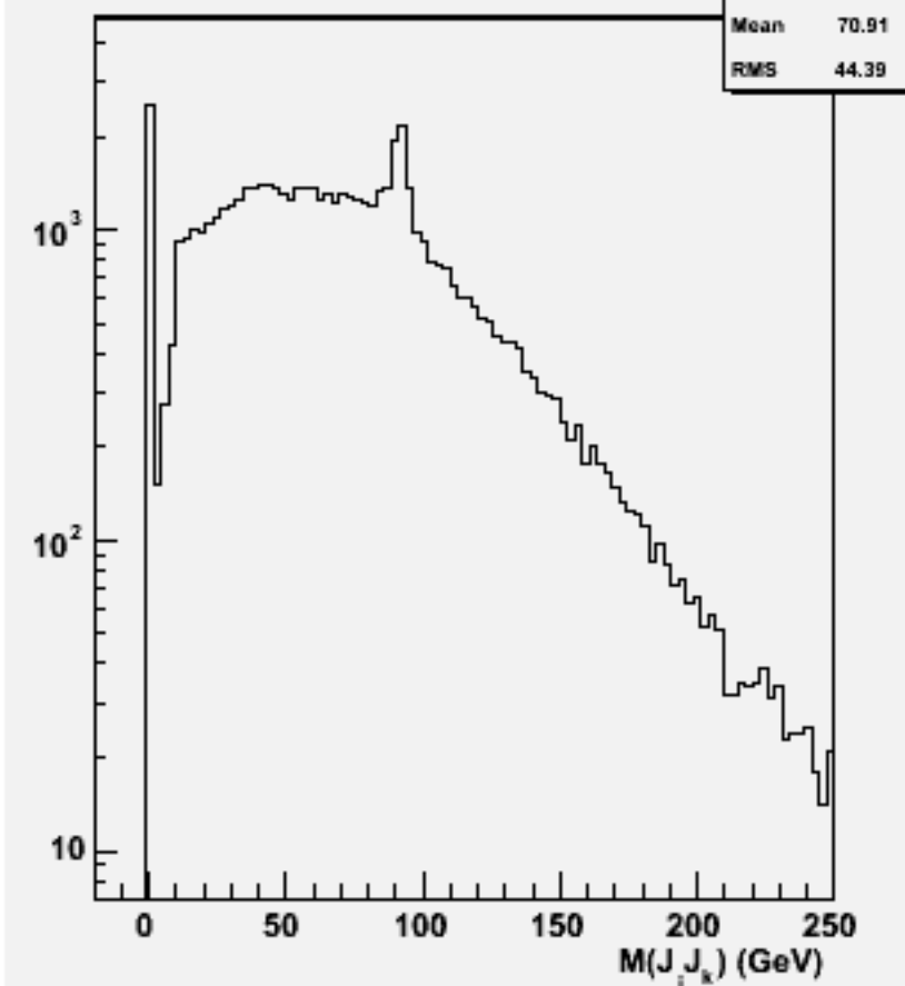
2jets mass(All comb)w101640 uun3e3e2n2_o
