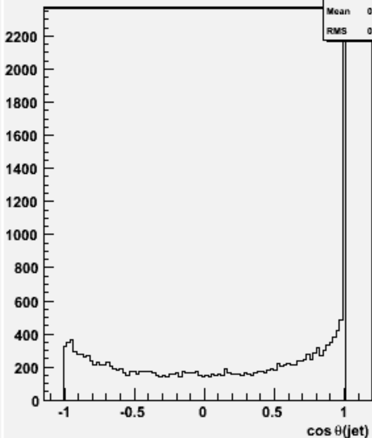
cos \theta for 2-jets :w101640 uun3e3e2n2_o
