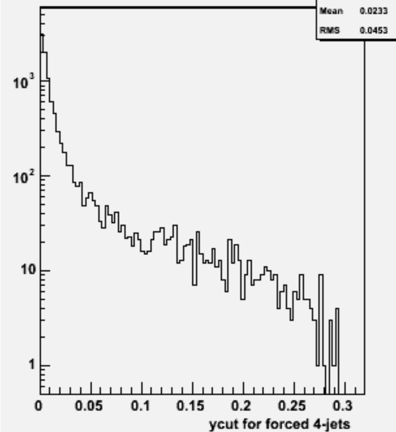
Ycut for 4-jets :w101640 uun3e3e2n2_o
