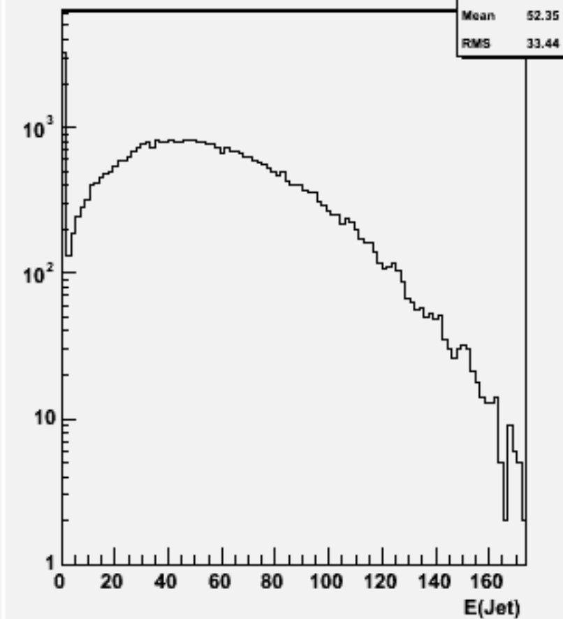
Jet energies(All jets)w101640 uun3e3e2n2_o
