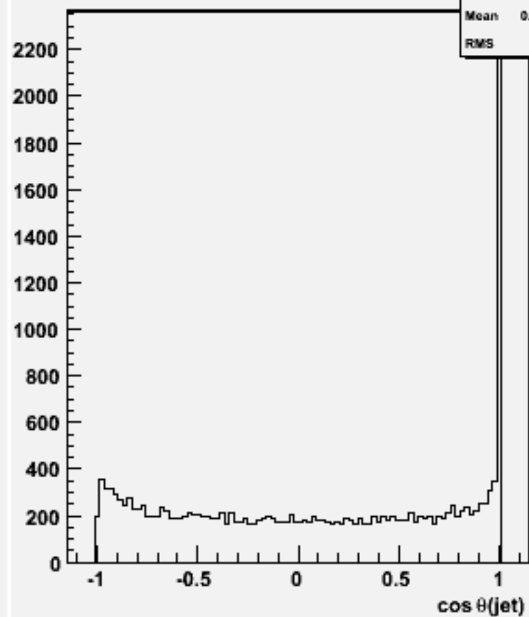
cos \theta for 2-jets :w101637 uun3e3e1n1_o
