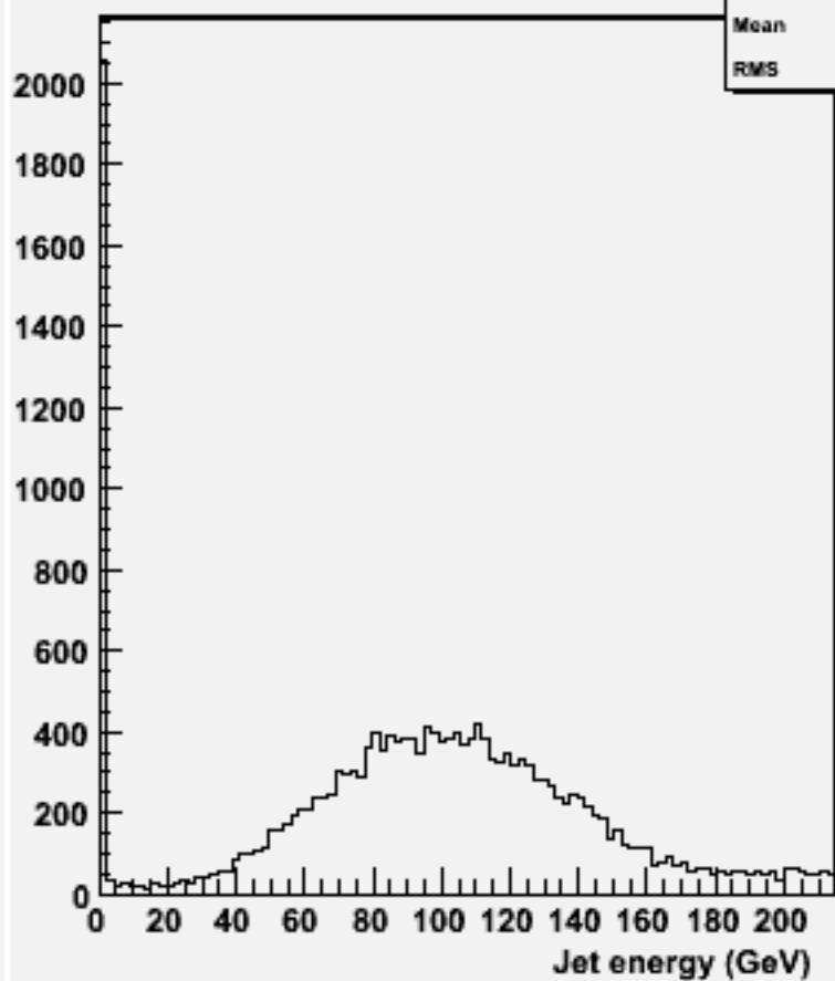
energy for 2-jets :w101637 uun3e3e1n1_o
