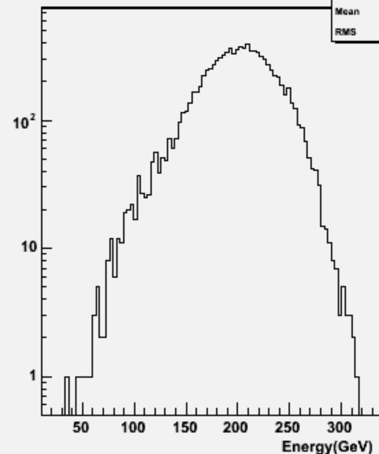
Thrust w101637 uun3e3e1n1_o
