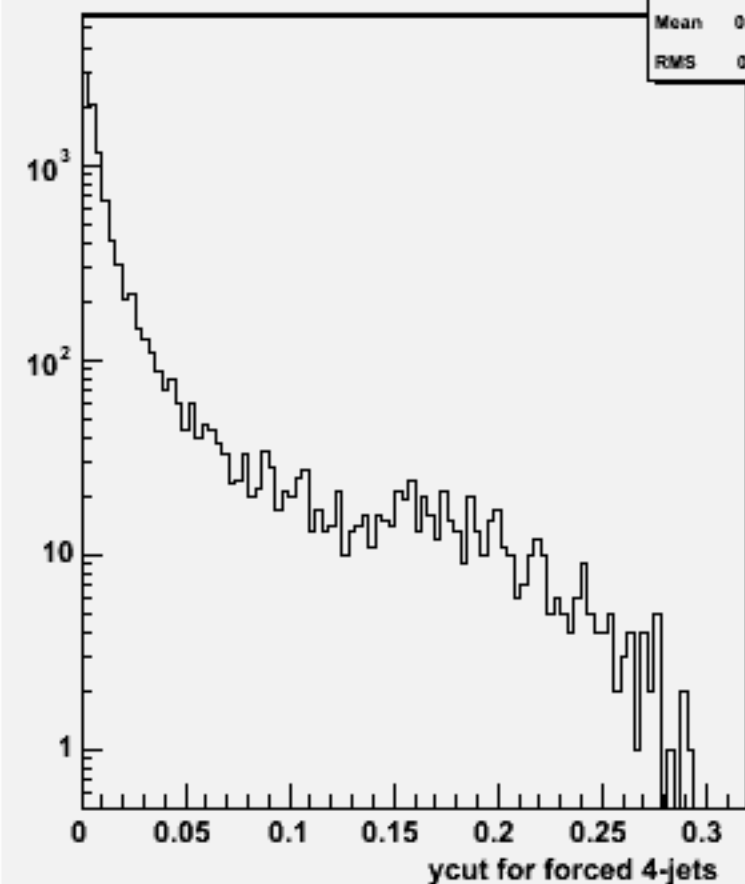
Ycut for 4-jets :w101637 uun3e3e1n1_o
