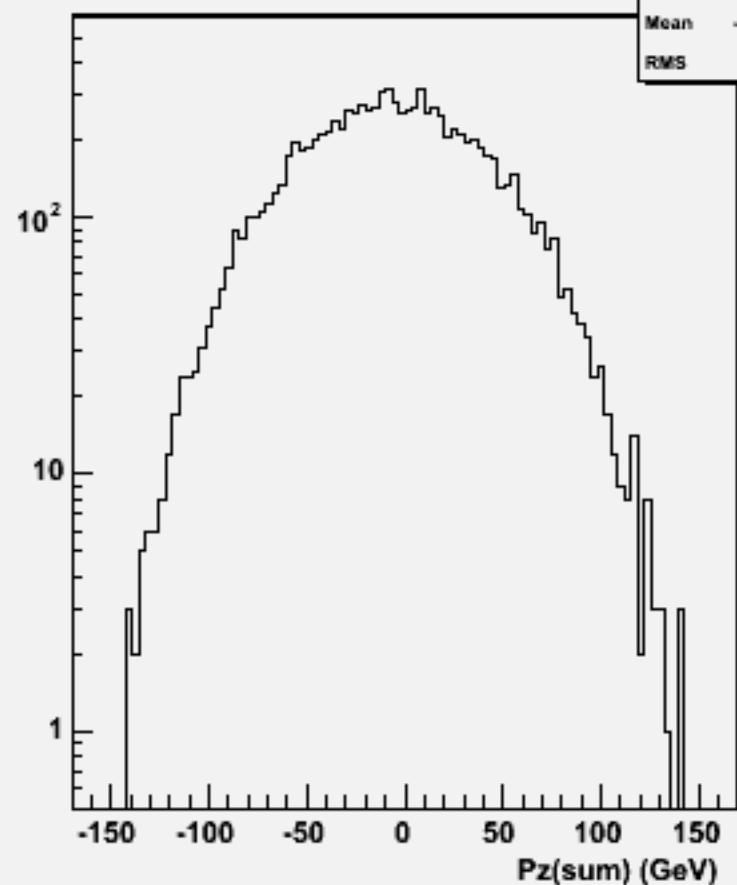
Pz Sum: w101637 uun3e3e1n1_o
