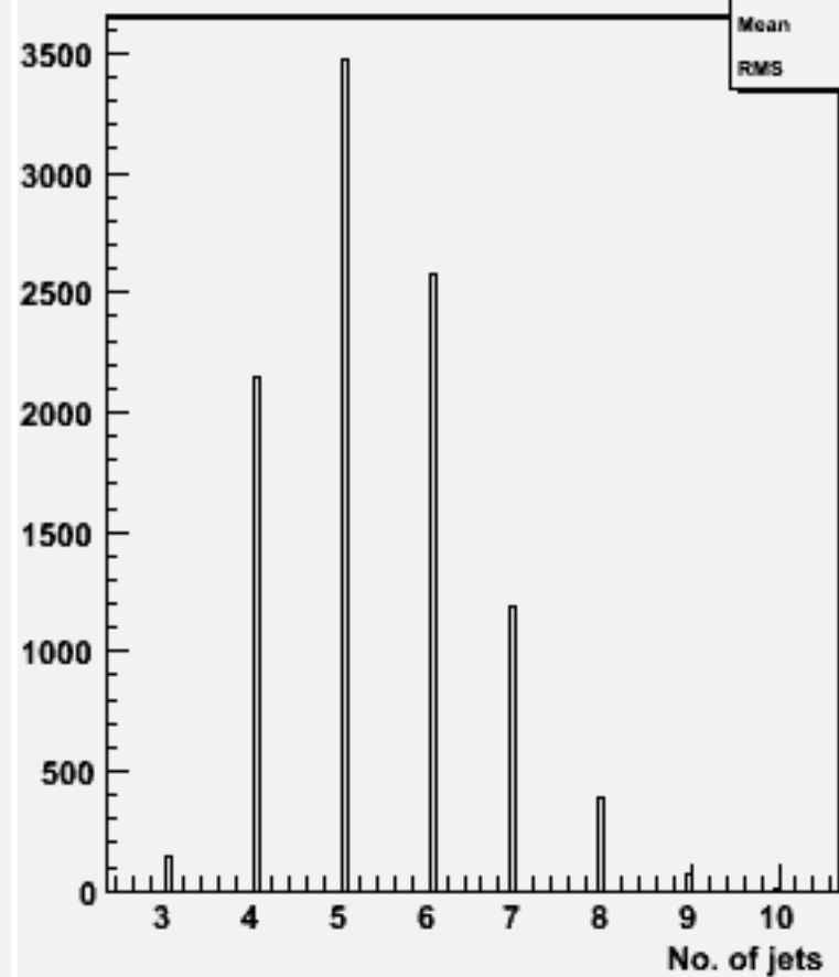
No. jets (ycut=0.001) : w101637 uun3e3e1n1_o
