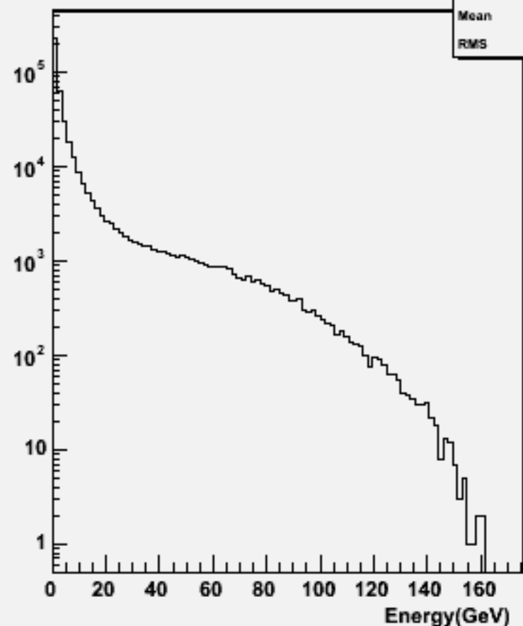
Particle Energy : w101637 uun3e3e1n1_o
