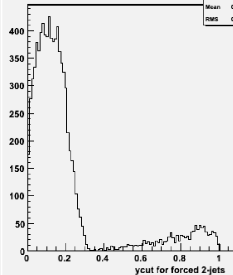
Ycut for 2-jets :w101637 uun3e3e1n1_o
