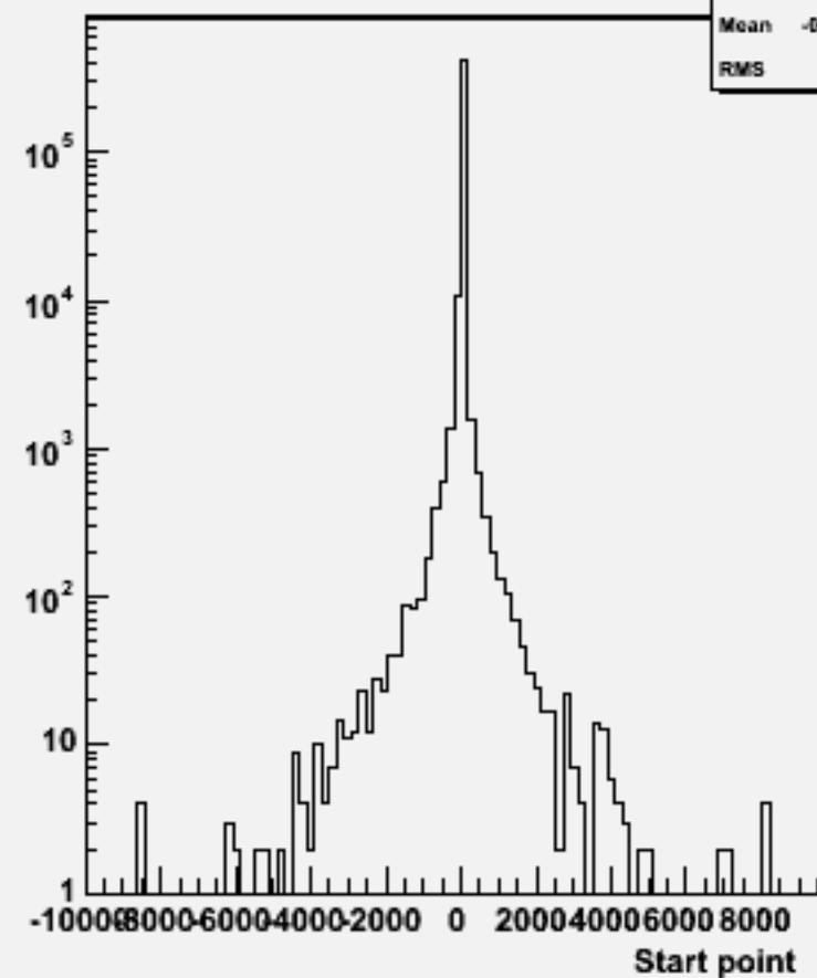
Start point Z : w101637 uun3e3e1n1_o
