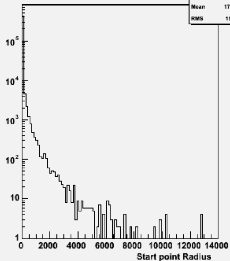
Start point R : w101637 uun3e3e1n1_o
