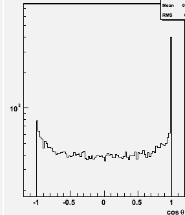
Jet cos \theta (All jets)w101637 uun3e3e1n1_o
