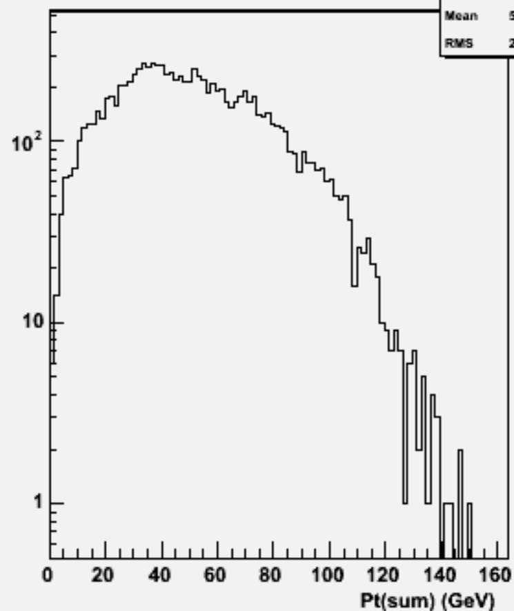
Pt Sum: w101637 uun3e3e1n1_o
