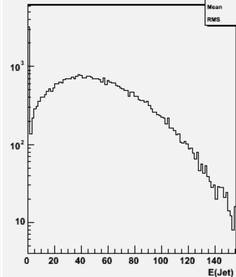
Jet energies(All jets)w101637 uun3e3e1n1_o
