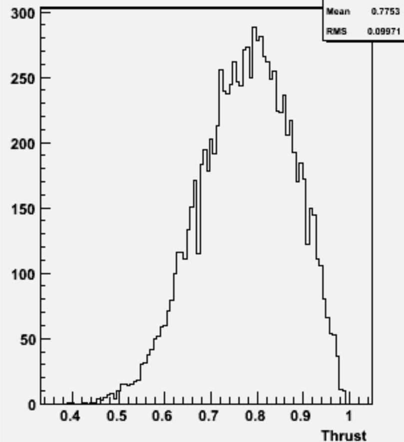
Thrust w101637 uun3e3e1n1_o
