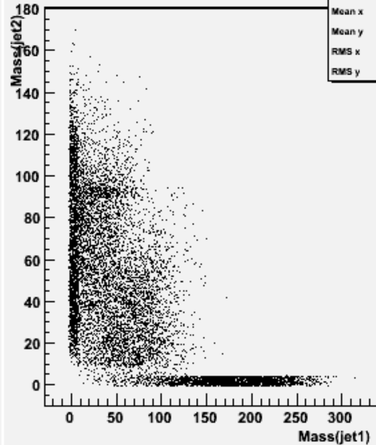
Jet mass for forced 2-jets : w101637 uun3e3e1n1_o
