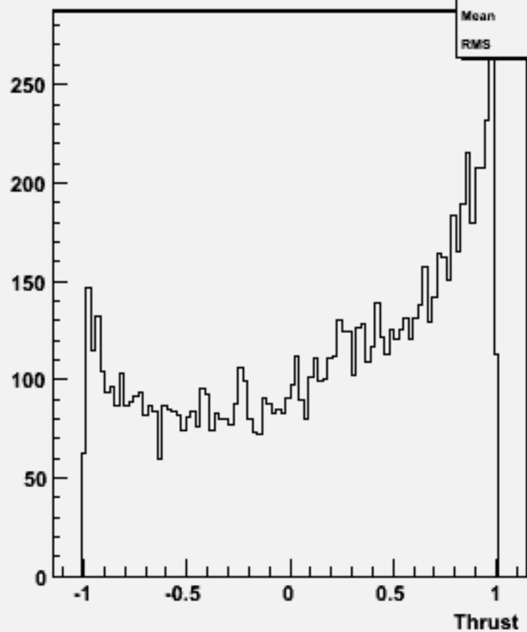
cos \Theta (thrust) w101637 uun3e3e1n1_o
