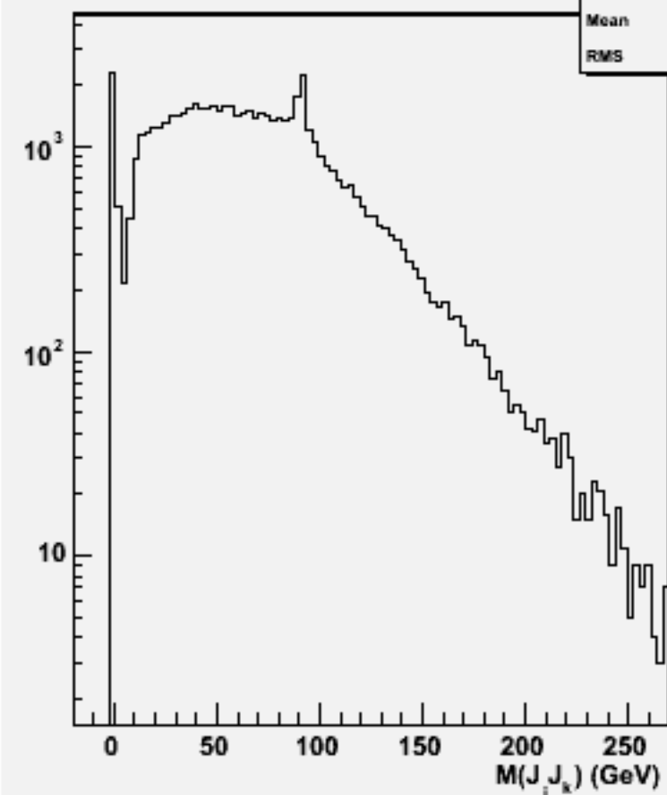
2jets mass(All comb)w101637 uun3e3e1n1_o
