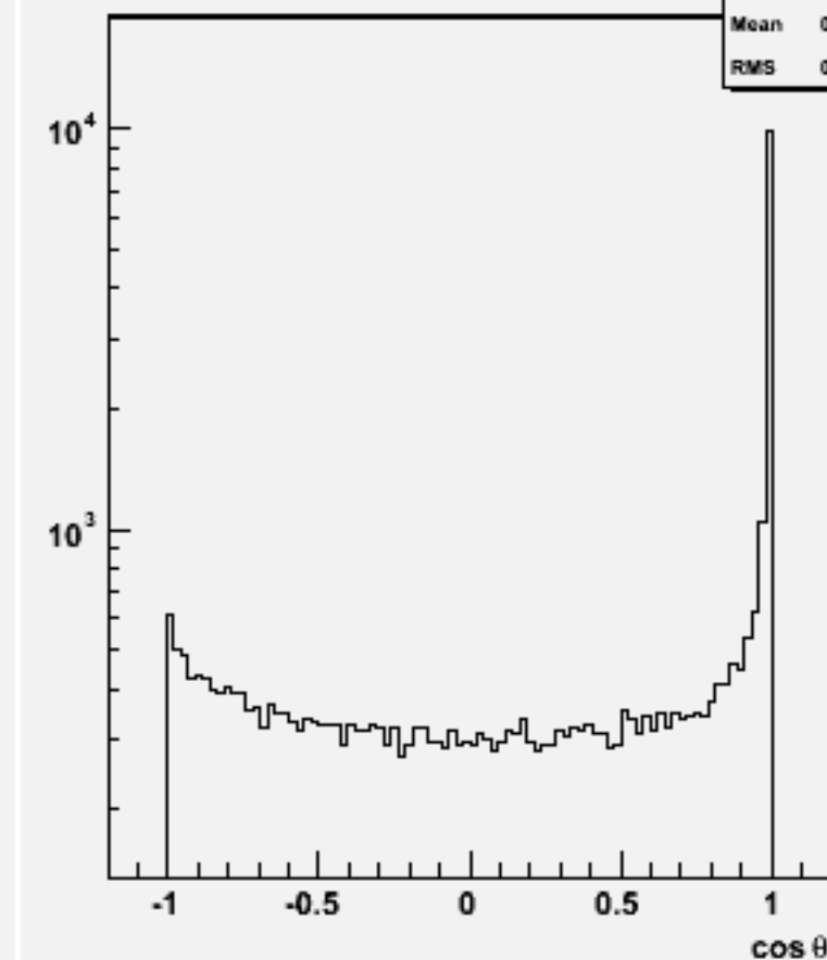
Jet cos \theta (All jets)w101636 uun3e3e1n1_o
