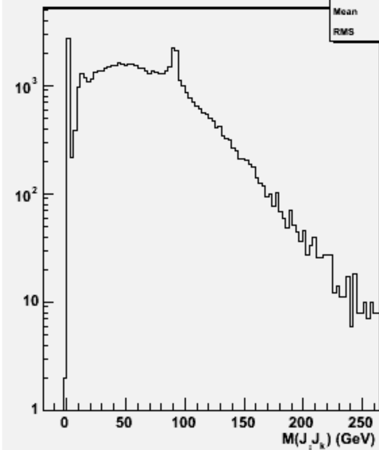
2jets mass(All comb)w101636 uun3e3e1n1_o
