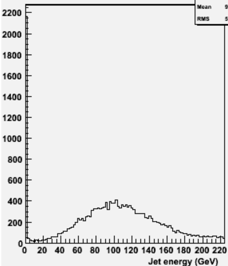
energy for 2-jets :w101636 uun3e3e1n1_o
