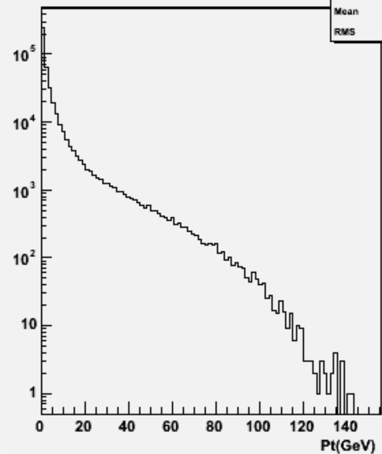
Start point Z : w101636 uun3e3e1n1_o
