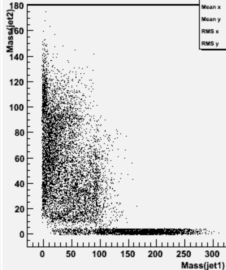
Jet mass for forced 2-jets : w101636 uun3e3e1n1_o
