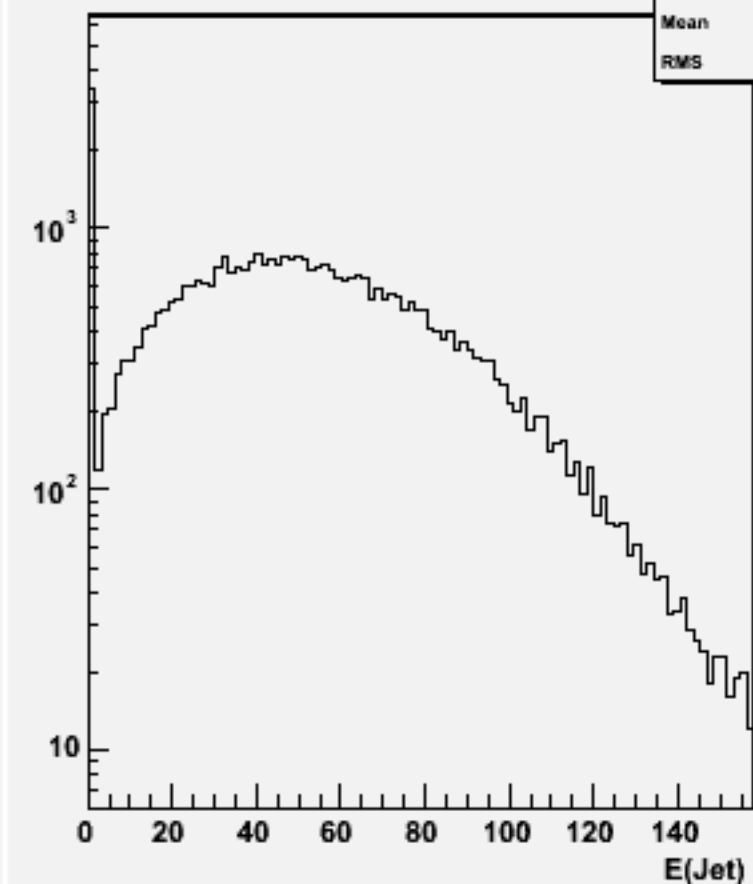
Jet energies(All jets)w101636 uun3e3e1n1_o
