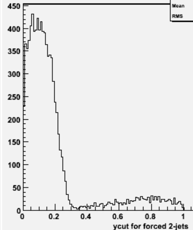
Ycut for 2-jets :w101636 uun3e3e1n1_o
