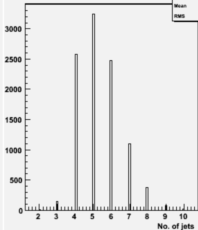
No. jets (ycut=0.001) : w101636 uun3e3e1n1_o
