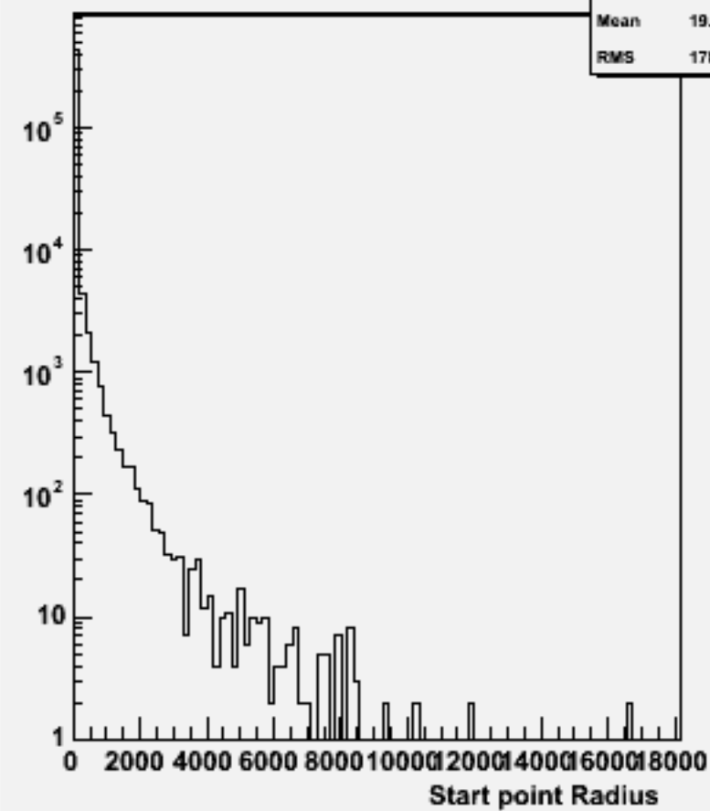
Start point R : w101636 uun3e3e1n1_o
