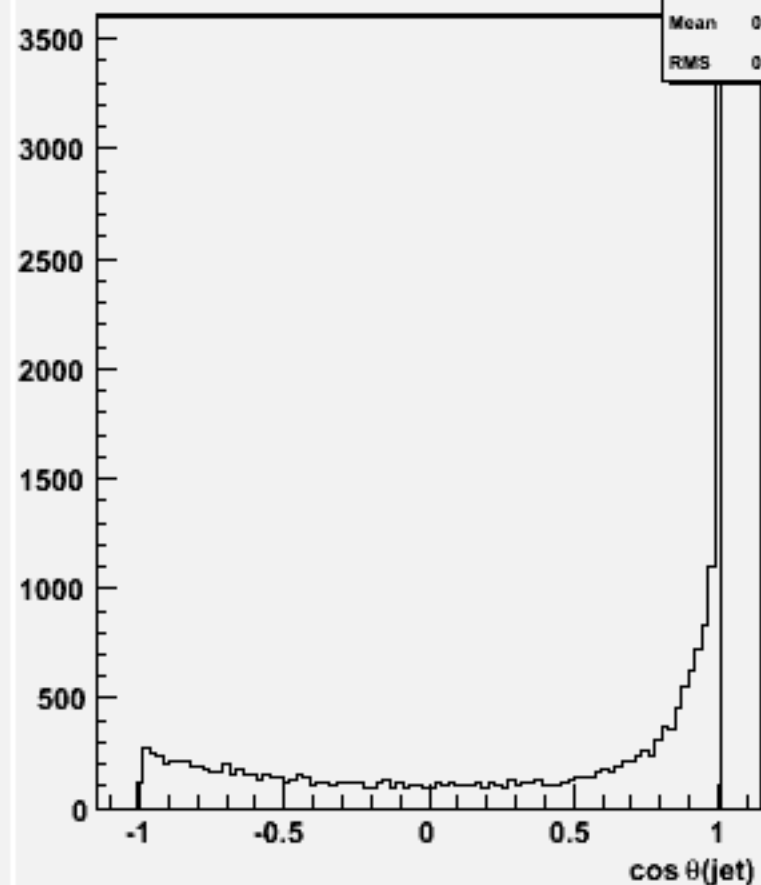
cos \theta for 2-jets :w101636 uun3e3e1n1_o
