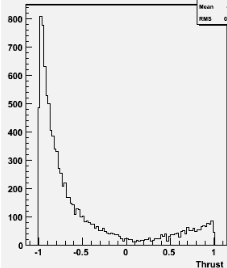
cos \Theta (thrust) w101636 uun3e3e1n1_o
