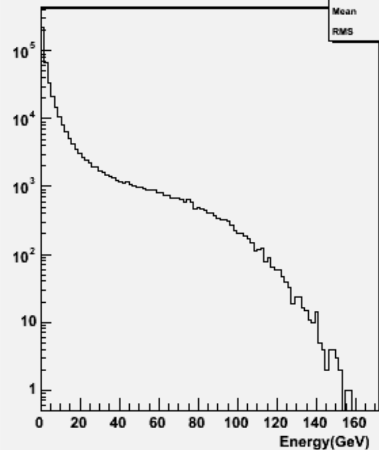
Start point R : w101636 uun3e3e1n1_o
