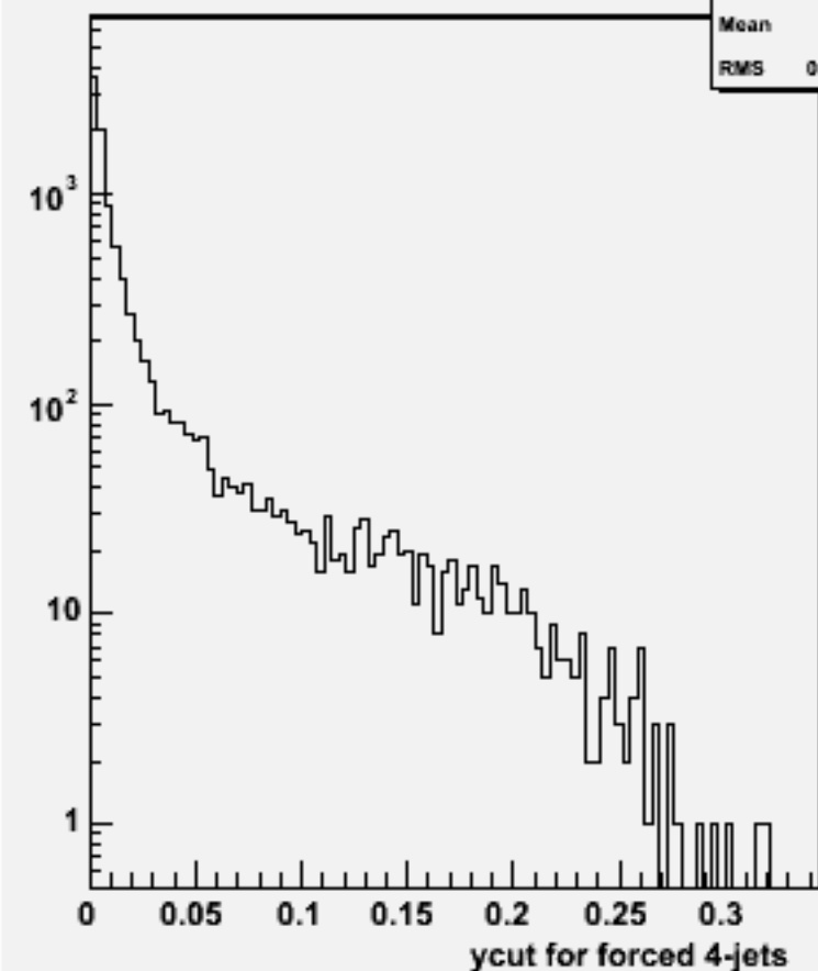
Ycut for 4-jets :w101636 uun3e3e1n1_o
