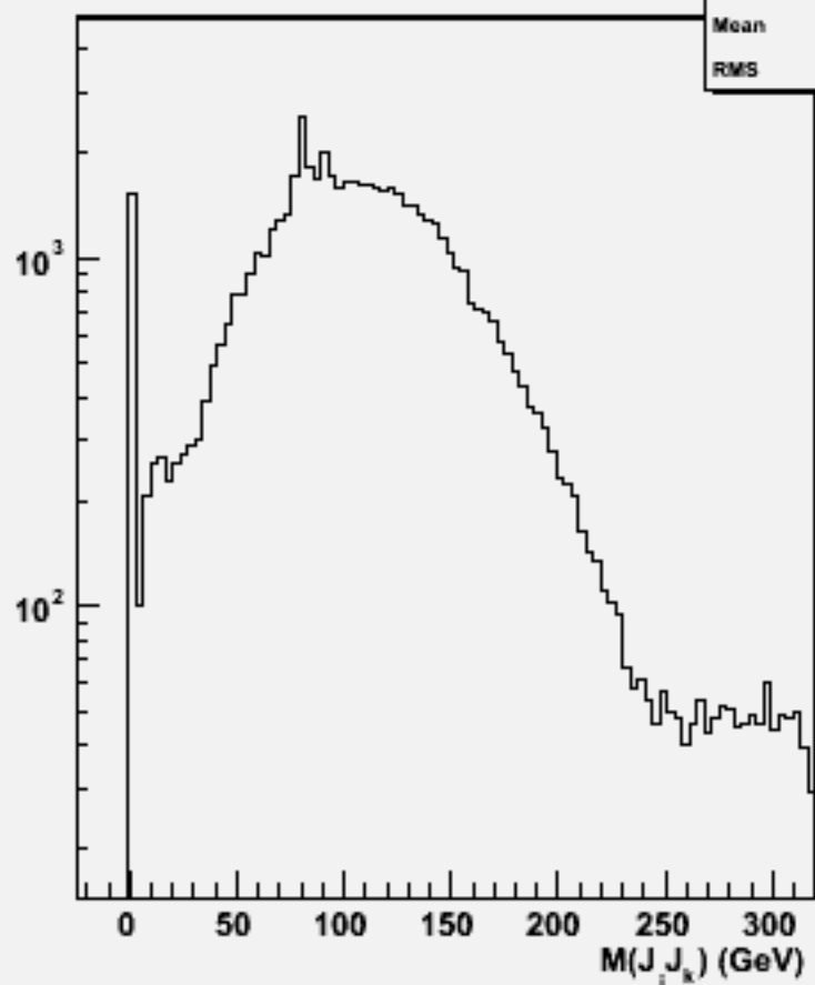
2jets mass(All comb)w101633 uun2e2sc_o
