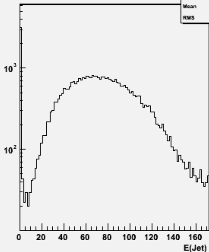
Jet energies(All jets)w101633 uun2e2sc_o
