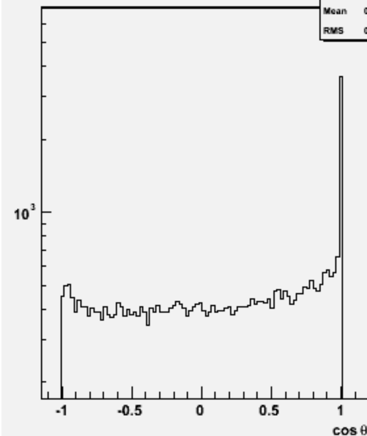
Jet cosθ (All jets)w101633 uun2e2sc_o
