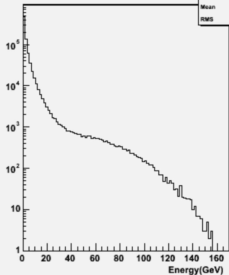
Particle Energy : w101633 uun2e2sc_o
