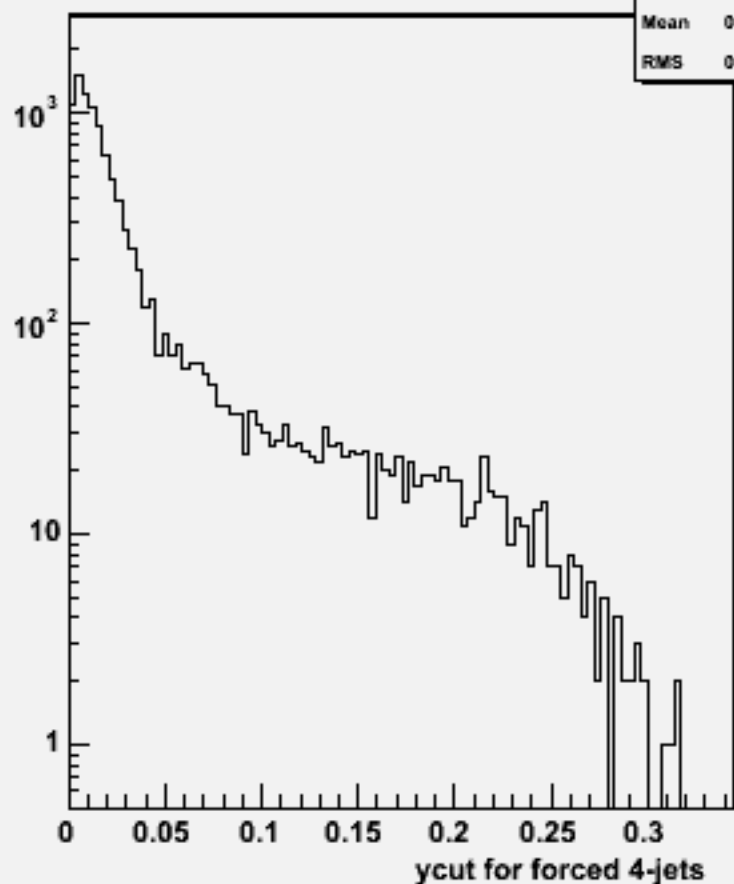
Ycut for 4-jets :w101633 uun2e2sc_o
