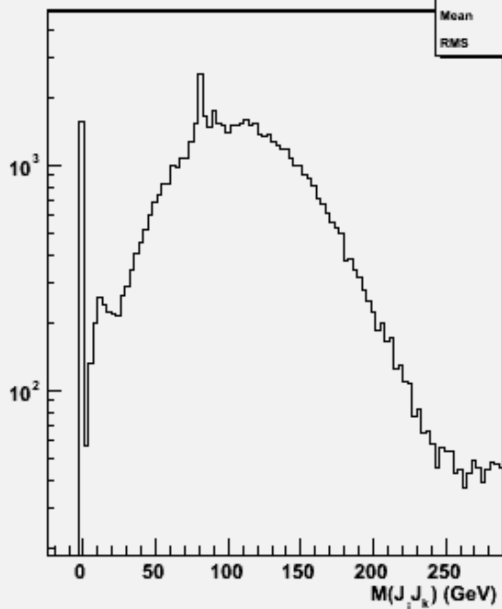
2jets mass(All comb)w101629 uun2e2du_o
