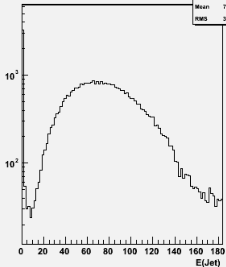
Jet energies(All jets)w101629 uun2e2du_o
