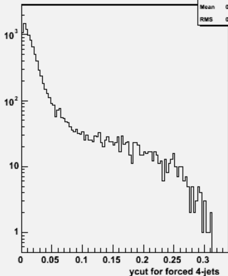
Ycut for 4-jets :w101629 uun2e2du_o
