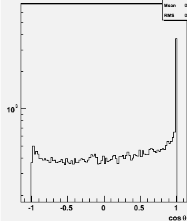
Jet cos \theta (All jets)w101629 uun2e2du_o
