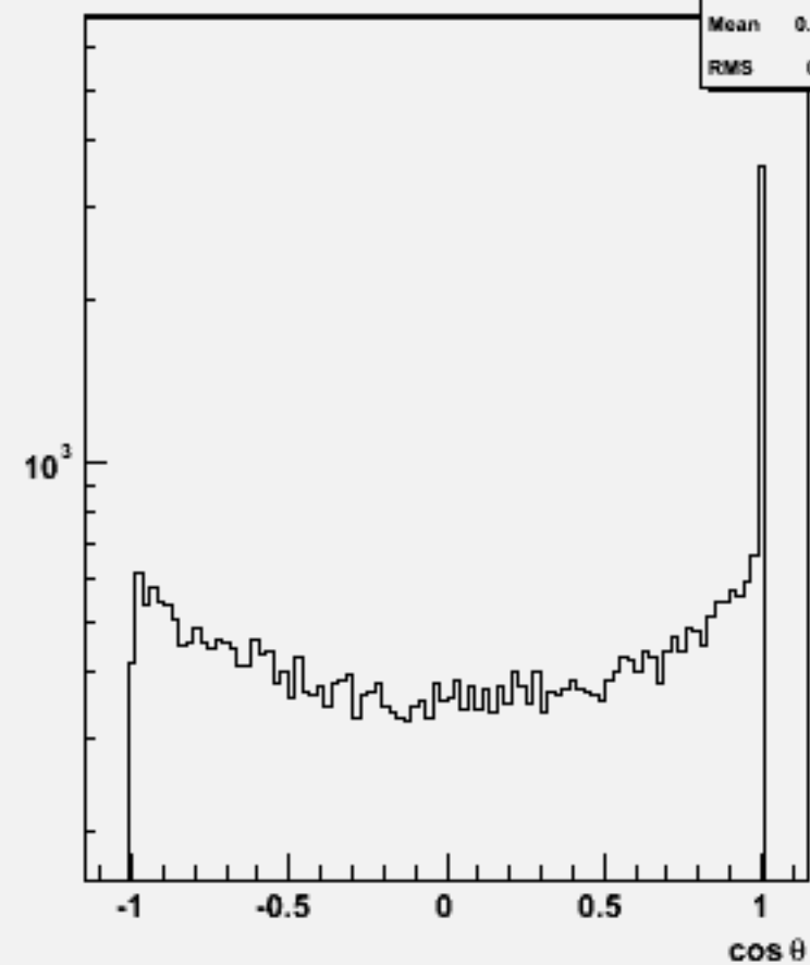
Jet cosθ (All jets)w101628 uun2e2du_o
