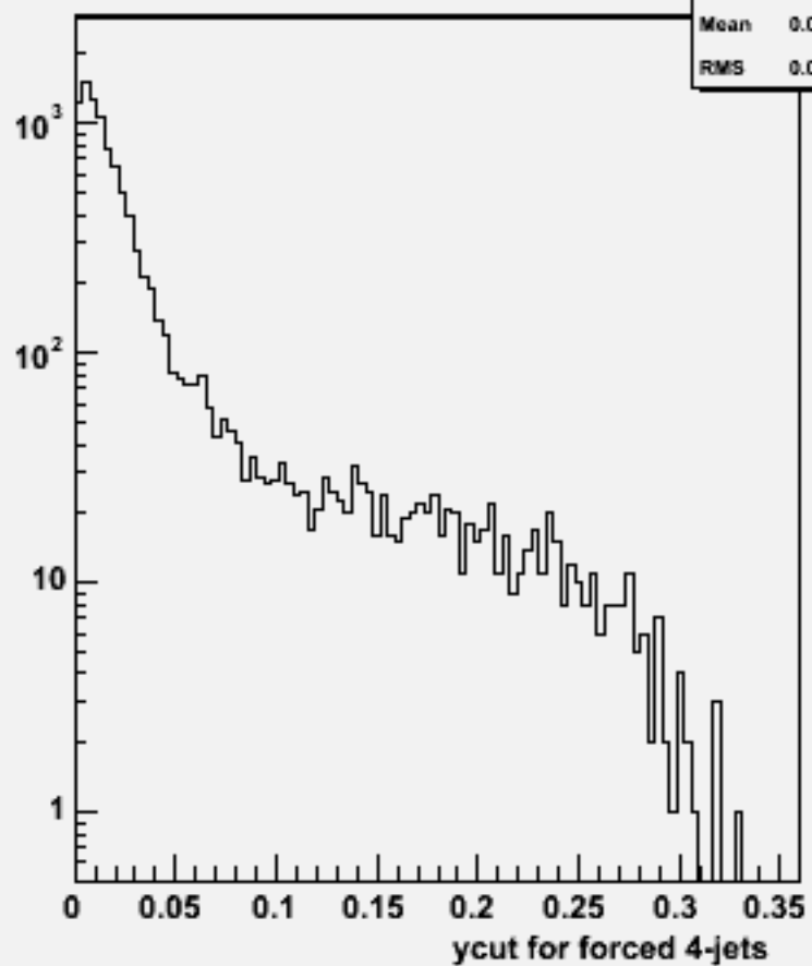
Ycut for 4-jets :w101628 uun2e2du_o
