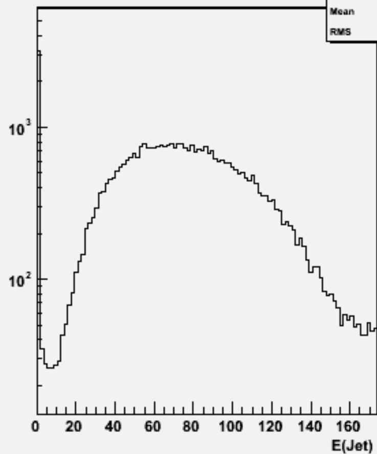
Jet energies(All jets)w101628 uun2e2du_o
