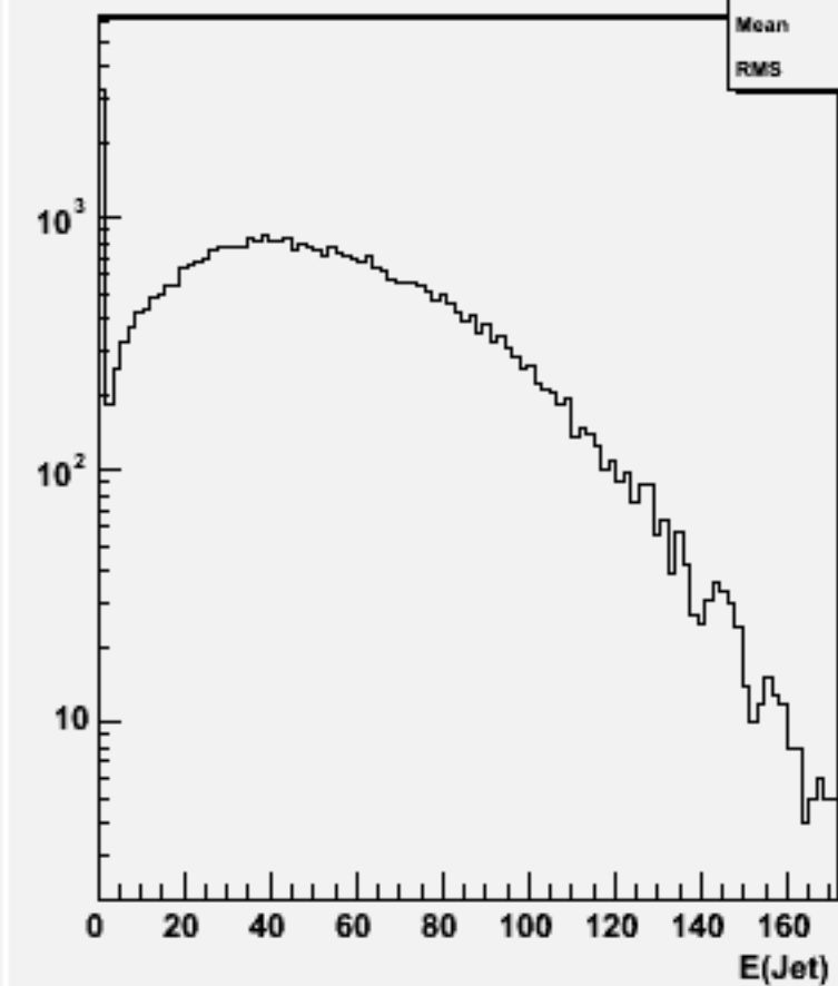
Jet energies(All jets)w101625 uun2e2e3n3_o
