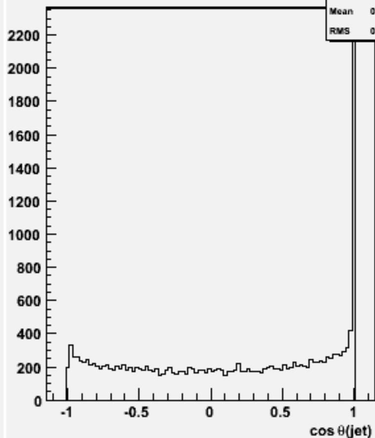
cos \theta for 2-jets :w101625 uun2e2e3n3_o
