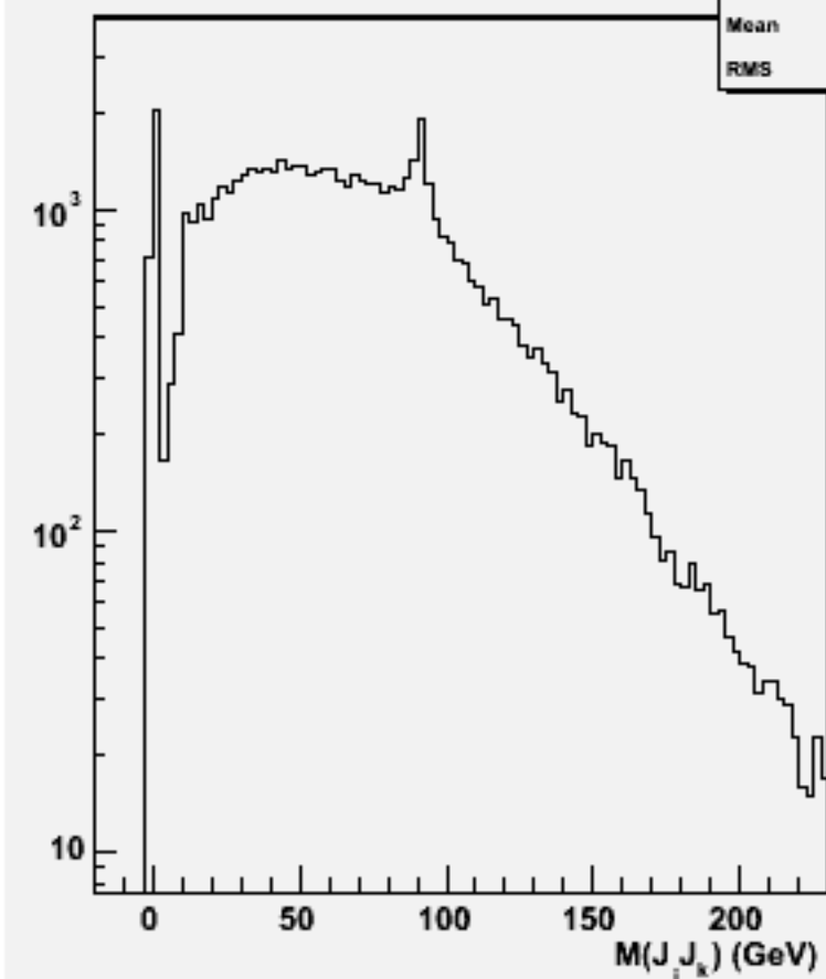
2jets mass(All comb)w101625 uun2e2e3n3_o
