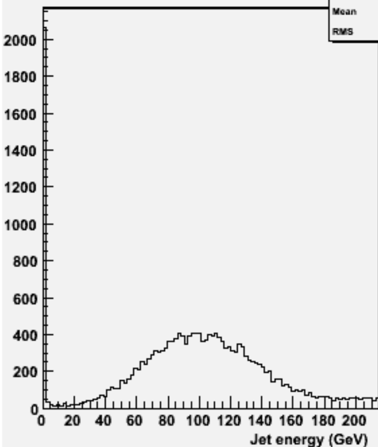
energy for 2-jets :w101625 uun2e2e3n3_o
