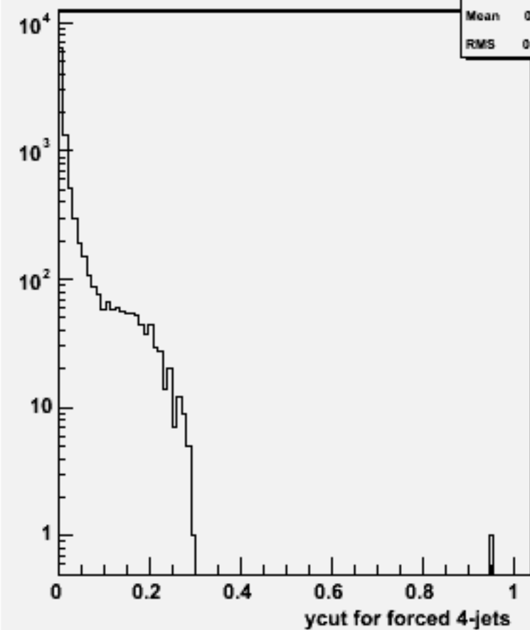
Ycut for 4-jets :w101625 uun2e2e3n3_o
