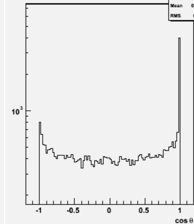
Jet cos \theta (All jets)w101625 uun2e2e3n3_o
