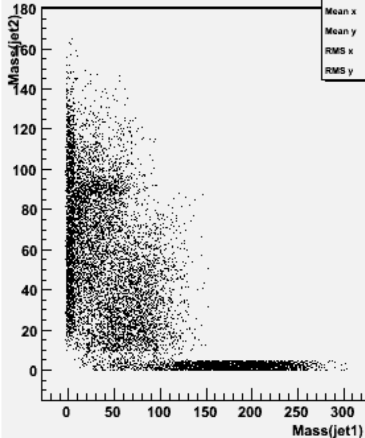
Jet mass for forced 2-jets : w101625 uun2e2e3n3_o
