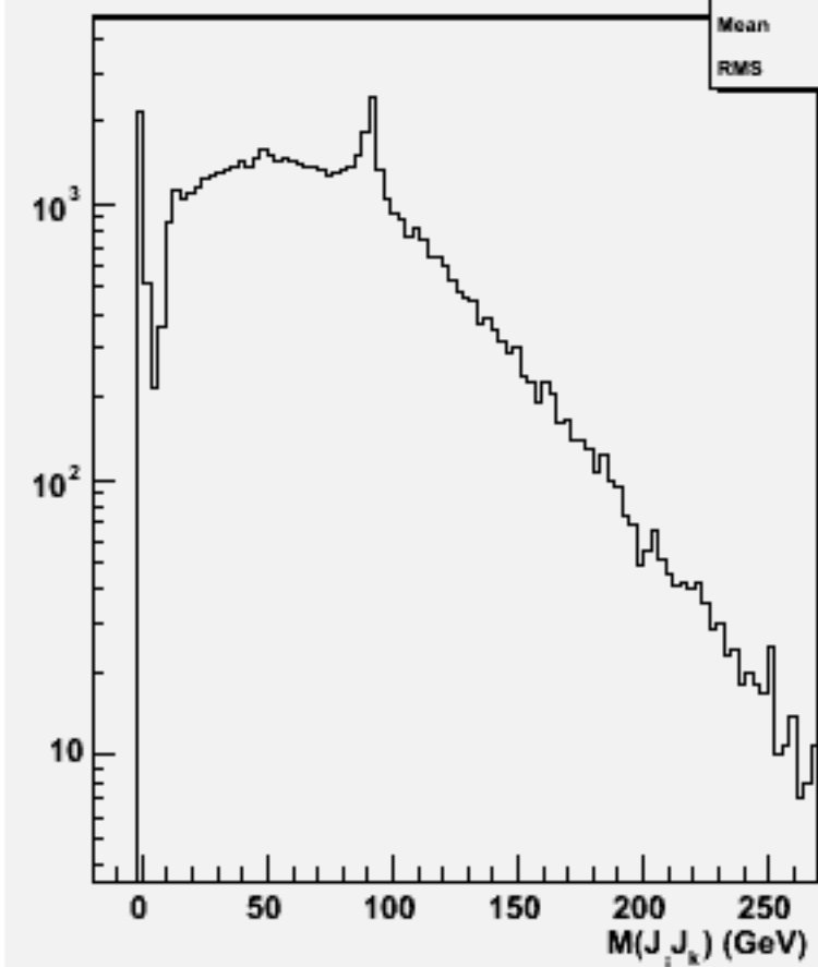
2jets mass(All comb)w101624 uun2e2e3n3_o
