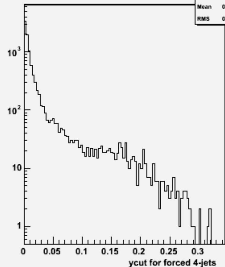
Ycut for 4-jets :w101624 uun2e2e3n3_o
