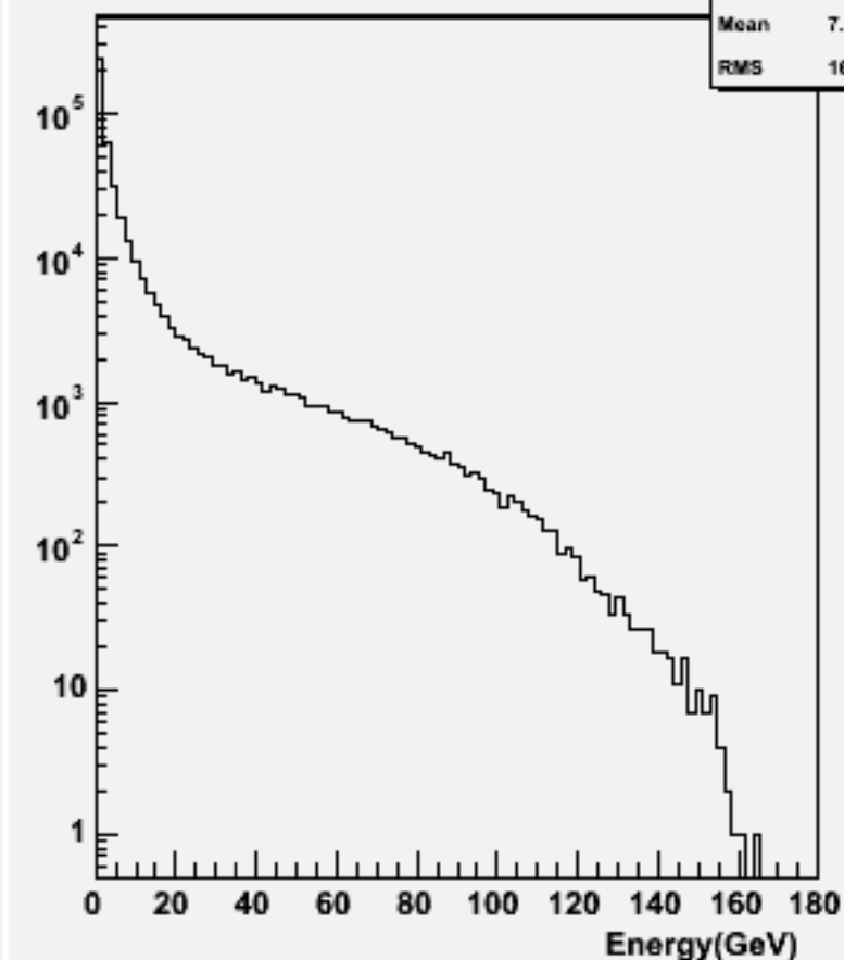
Particle Energy : w101624 uun2e2e3n3_o
