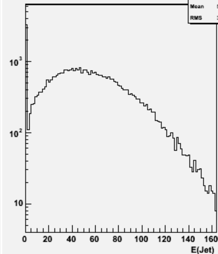
Jet energies(All jets)w101624 uun2e2e3n3_o
