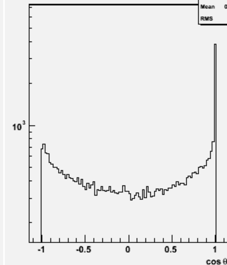
Jet cos \theta (All jets)w101624 uun2e2e3n3_o
